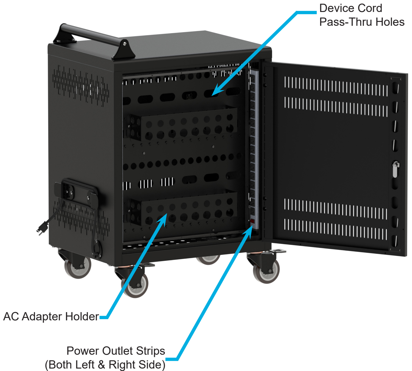
Rear View of Cart
