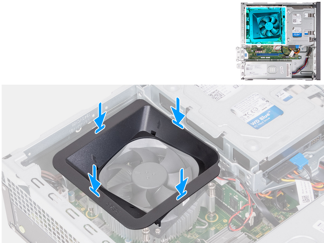
Figure 35. nstalling the fan shroud
