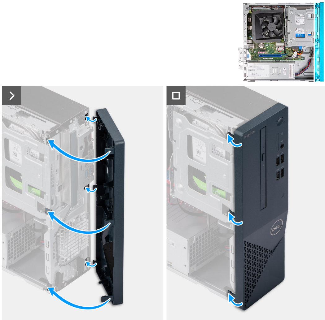
Figure 15. Installing the front cover
