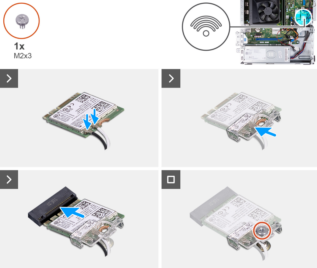
Figure 33. Installing the wireless card
