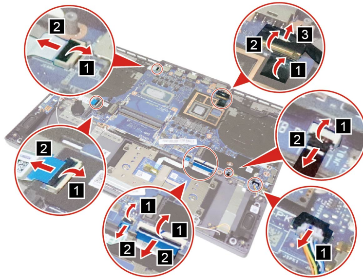
Figure 23. Disconnect cables
