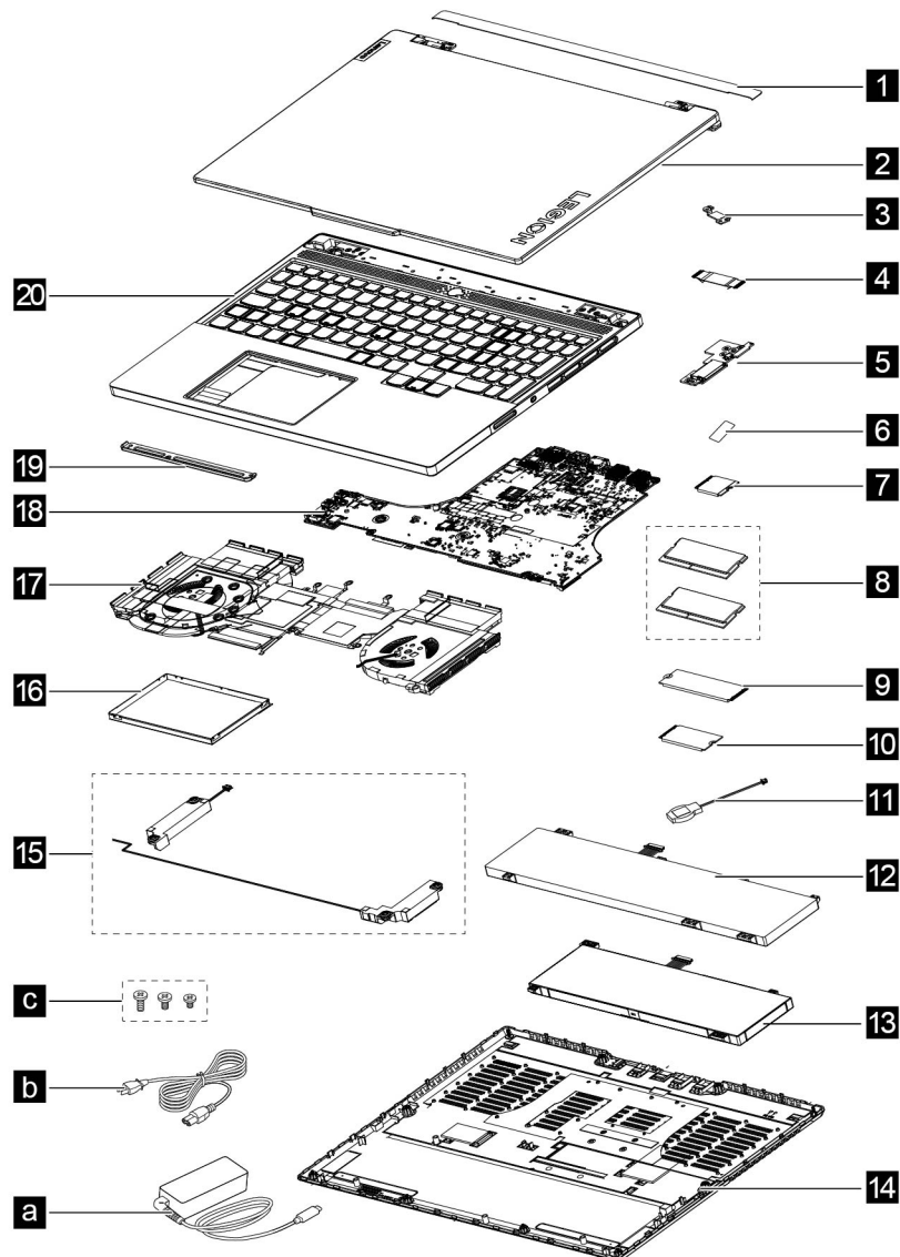
Figure 1. System exploded view
