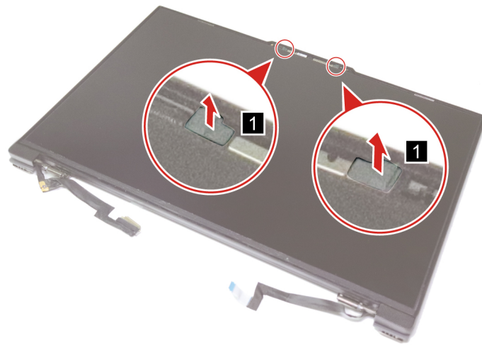
Figure 33. Remove the microphone rubbers
