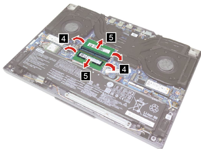
Figure 9. Remove the memory modules
