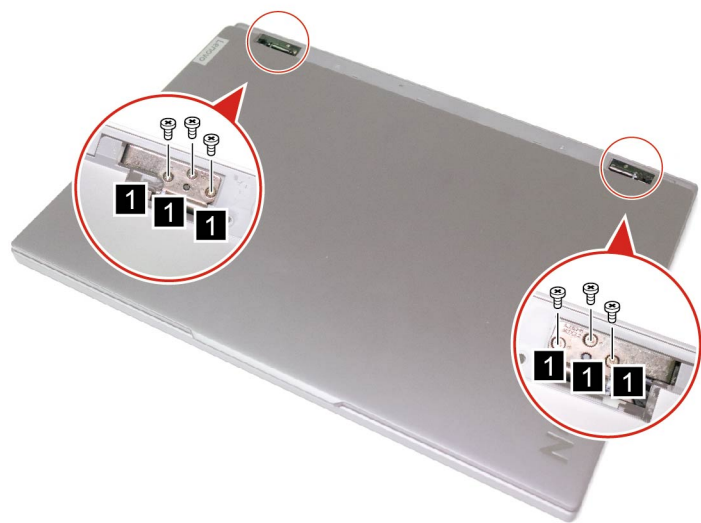
Figure 28. Remove six screws
