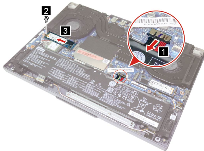
Figure 12. Remove the left SSD
