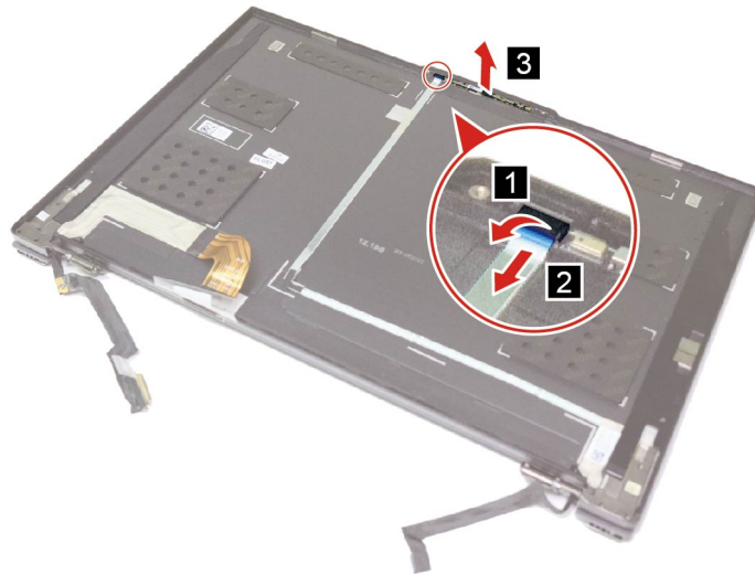
Figure 37. Disconnect the camera cable and remove the camera board
