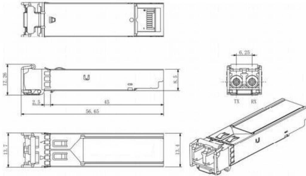
Mechanical Drawing
