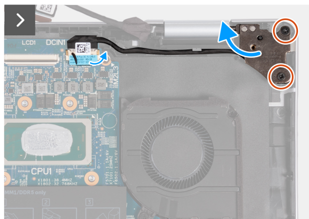
2x M2.5x5.5
