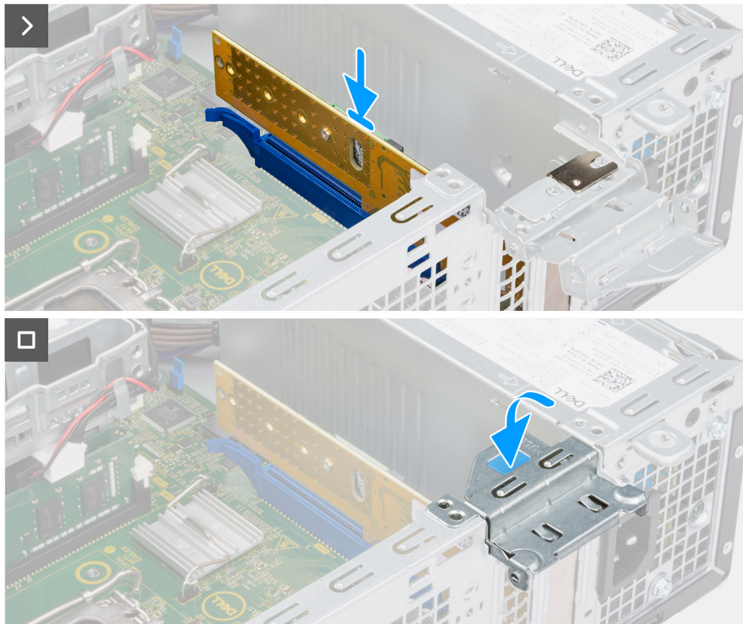
Figure 26. Installation de la carte Dell Ultra Speed Drive Gen 3
