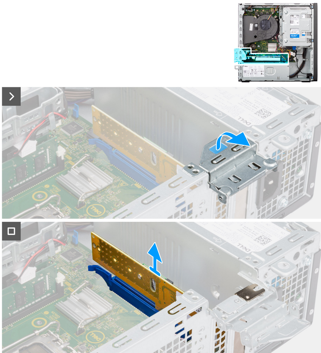
Figure 21. Retrait de la carte Dell Ultra Speed Drive Gen 3
