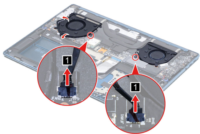
Figure 19. Disconnect the fan cable from the system board
