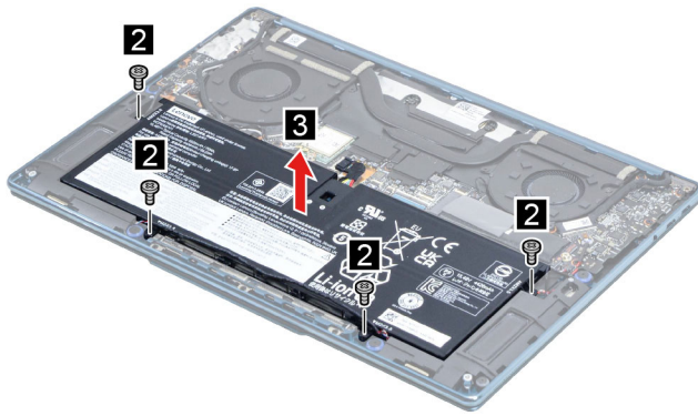
Figure 5. Remove the battery pack
