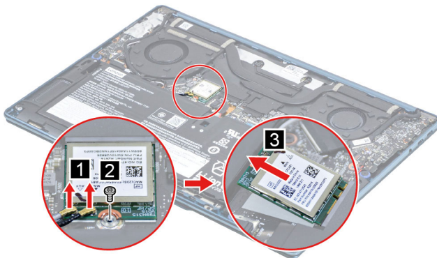
Figure 10. Remove the Wi-Fi card
