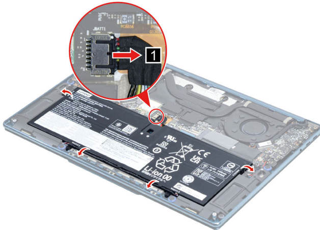
Figure 4. Disconnect the battery pack cable and release the speaker cable
