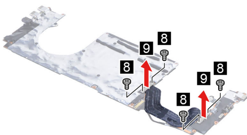
Figure 23. Remove the I/O board FPC
