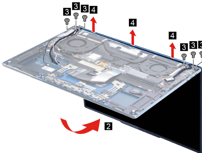
Figure 27. Remove the LCD module
