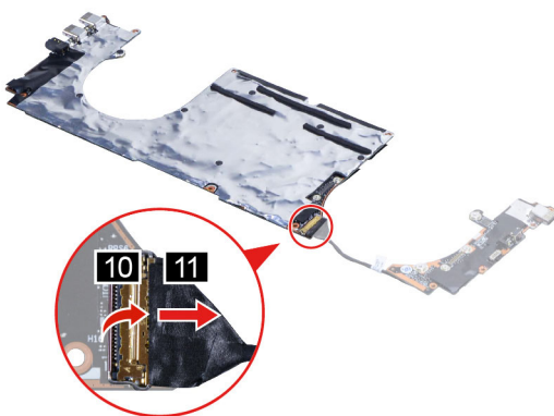
Figure 24. Disconnect the I/O board cable
