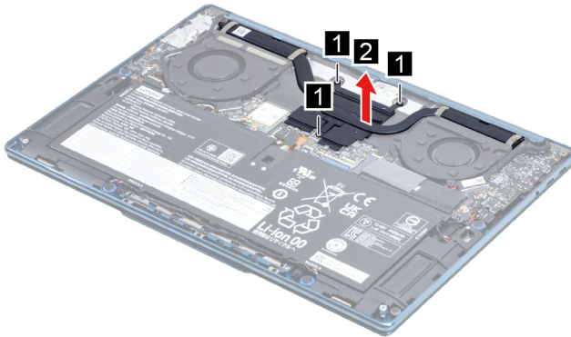
Figure 15. Remove the heat sink
