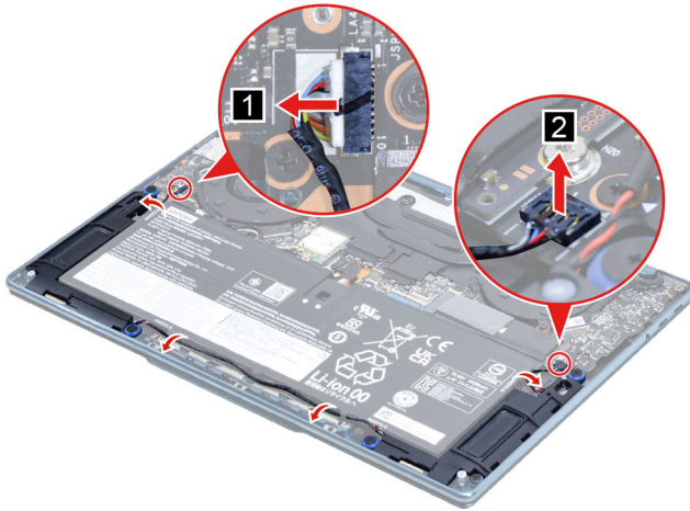
Figure 11. Detach the speaker cable connectors and release the speaker cable
