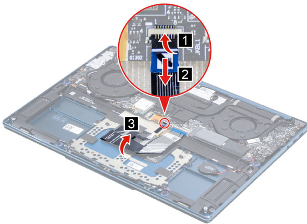
Figure 17. Disconnect the touchpad board cable and peel back the keyboard cable
