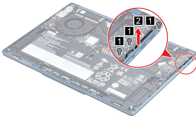
Figure 14. Remove the system board bracket
