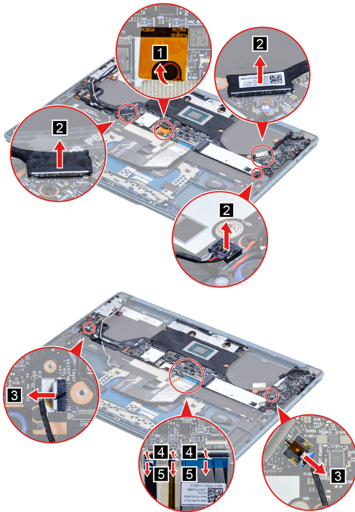
Figure 21. Peel off the tape and disconnect cables connected to the system board
