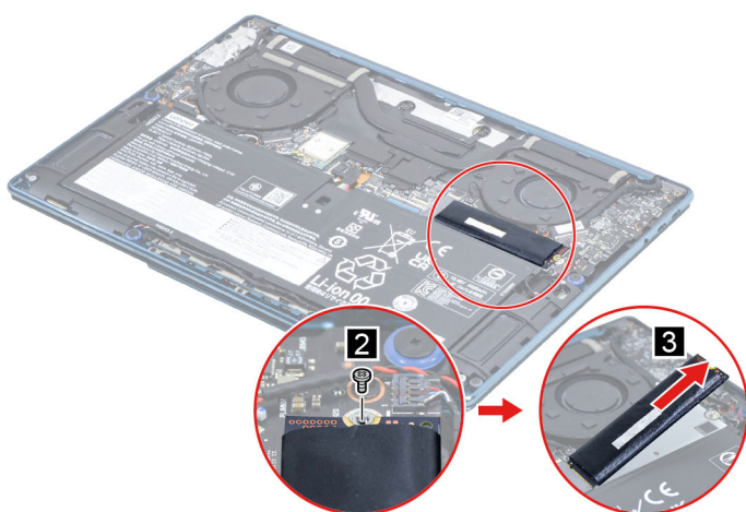
Figure 8. Remove the SSD
