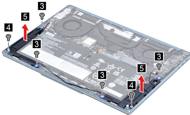
Figure 12. Remove the speakers
