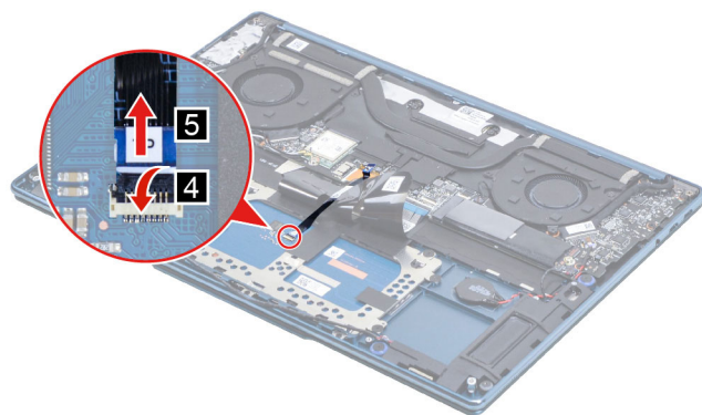
Figure 18. Remove the touchpad board cable
