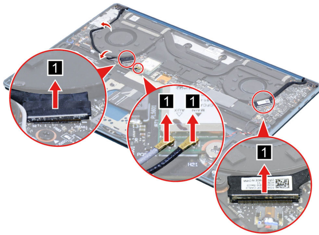
Figure 26. Disconnect the EDP cable, the sensor board cable and the antenna cable
