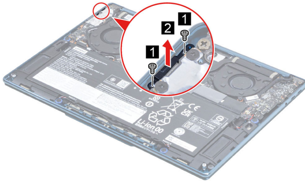
Figure 13. Remove the I/O board bracket
