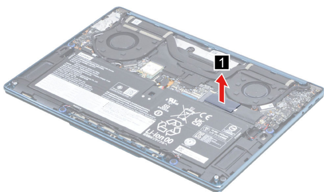
Figure 7. Remove the thermal pad
