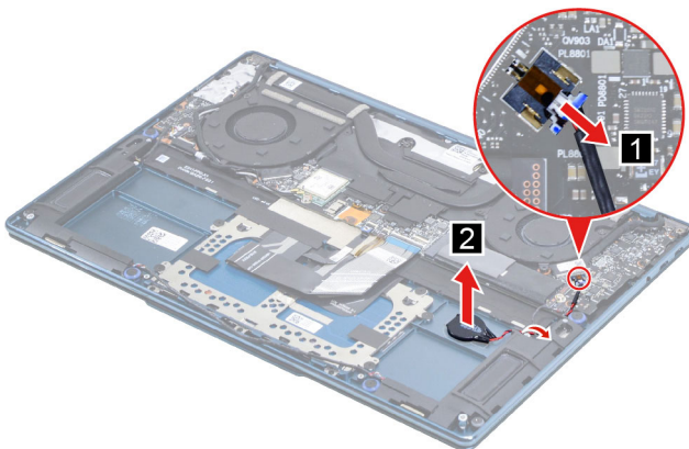
Figure 16. Remove the CMOS battery
