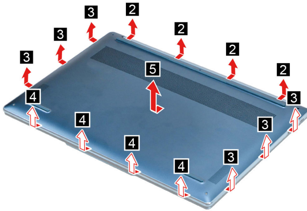
Figure 3. Pry up the latches and remove the lower case
