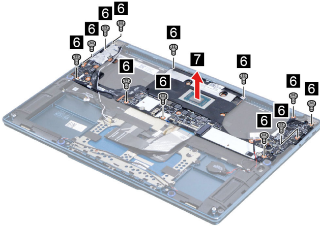
Figure 22. Remove the system board and the I/O board
