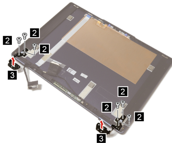
Figure 31. Remove six screws and hinges
