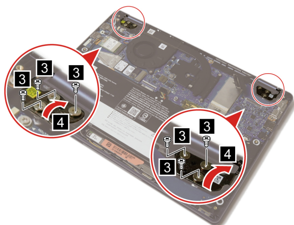
Figure 24. Remove six screws and open the hinges
