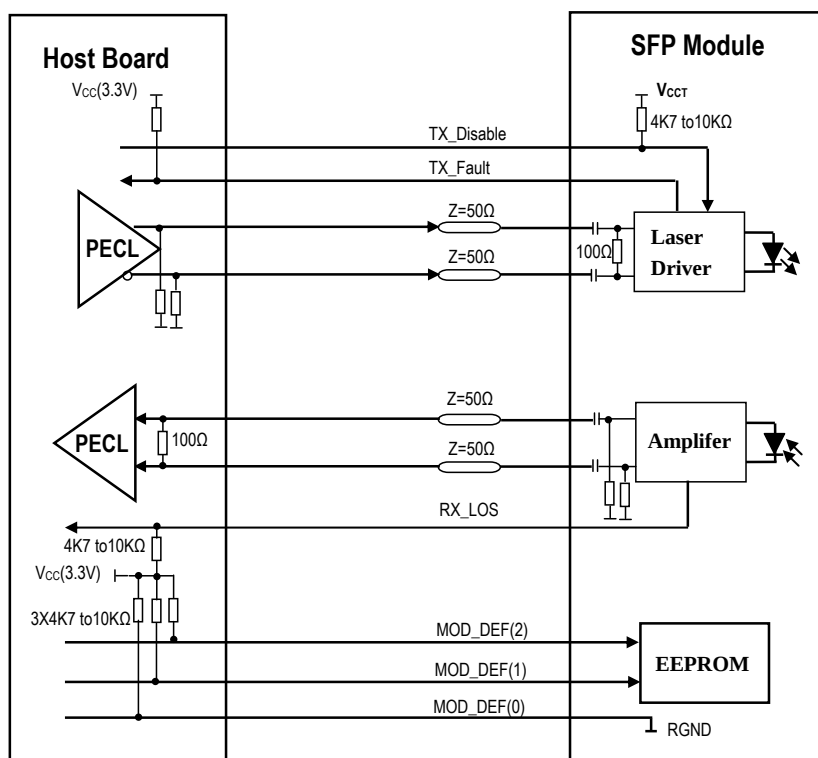
SFP Host Recommended Circuit
