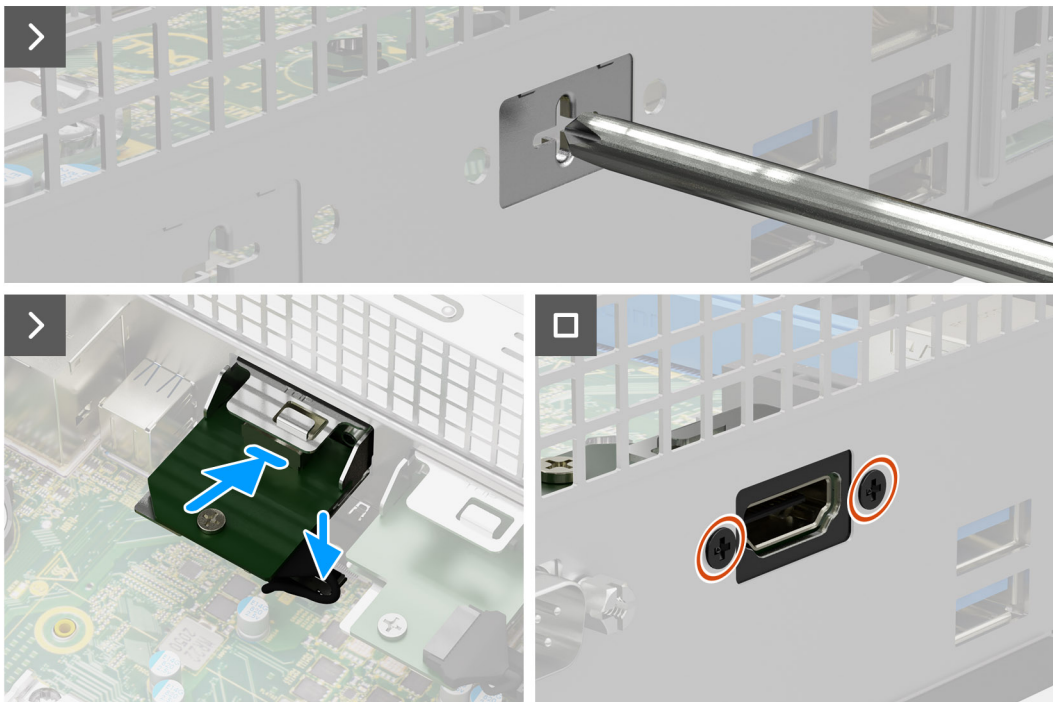
Figure 55. Installation du module HDMI
