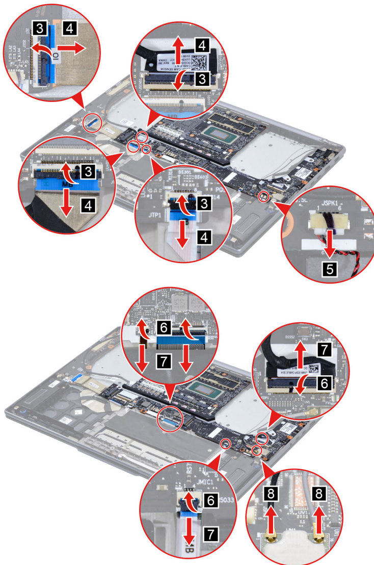
Figure 23. Disconnect cables connected to the system board
