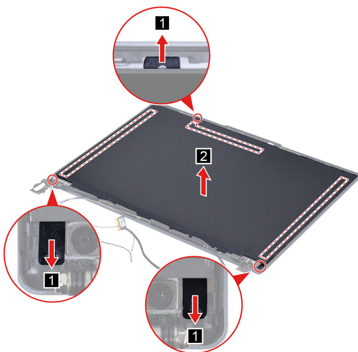
Figure 34. Remove the LCD panel
