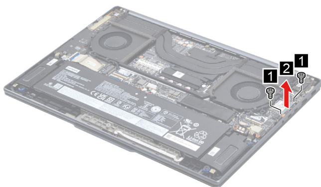
Figure 11. Remove the Type-C bracket
