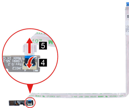
Figure 13. Remove the microphone cable
