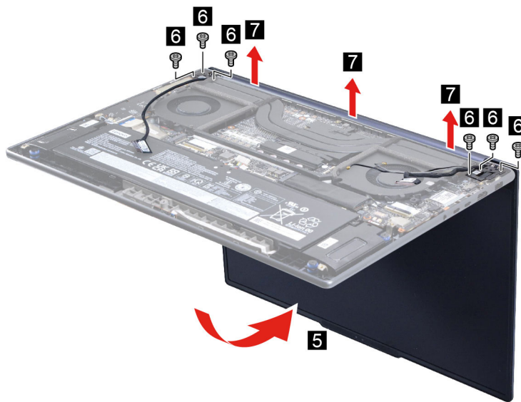
Figure 28. Remove the LCD module
