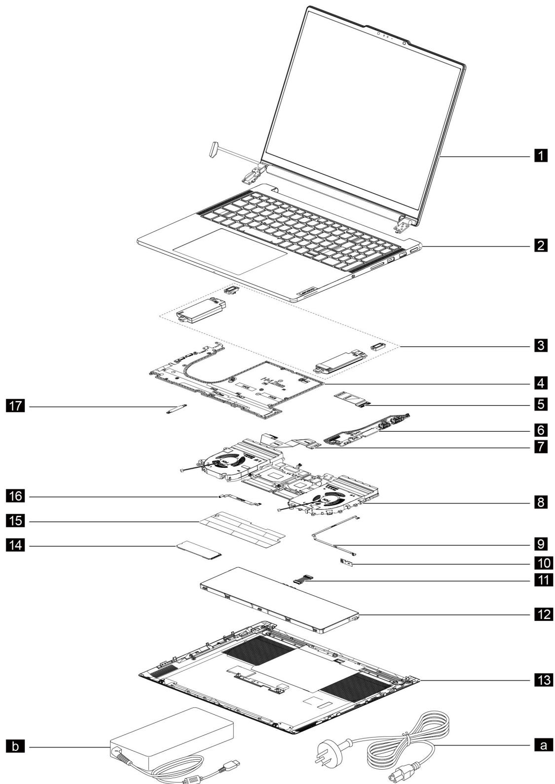
Figure 1. exploded view
