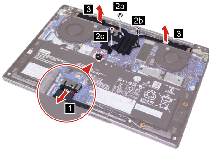
Figure 13. Remove the heat sink
