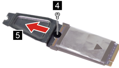
Figure 8. Remove the 2242 solid-state drive bracket
