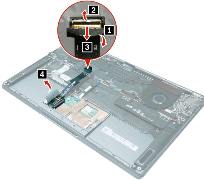
Figure 11. Disconnect the cable of the solid-state drive board
