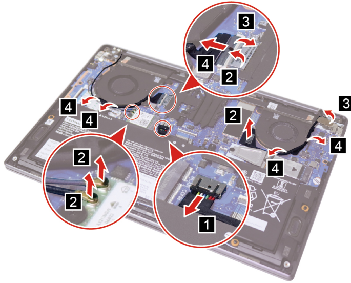
Figure 25. Disconnect cables
