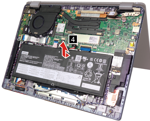
Figure 32. Remove the LCD unit
