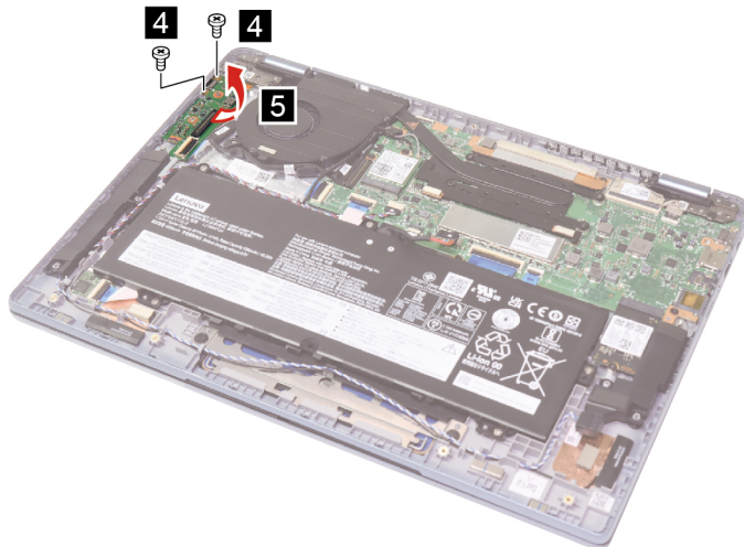
Figure 19. Remove three screws and the I/O board
