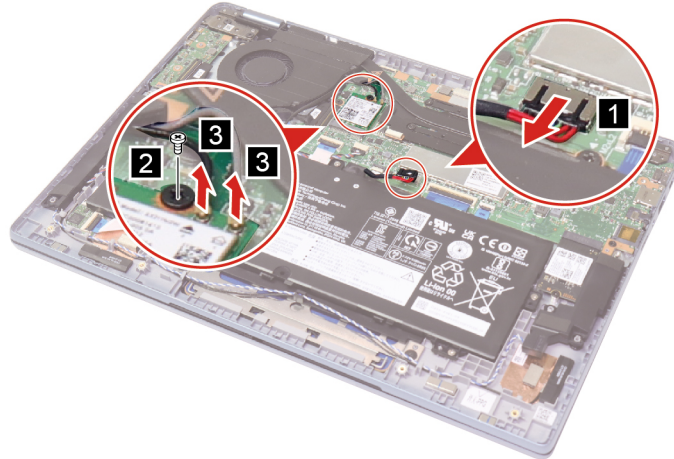
Figure 20. Disconnect cables and remove one screw
