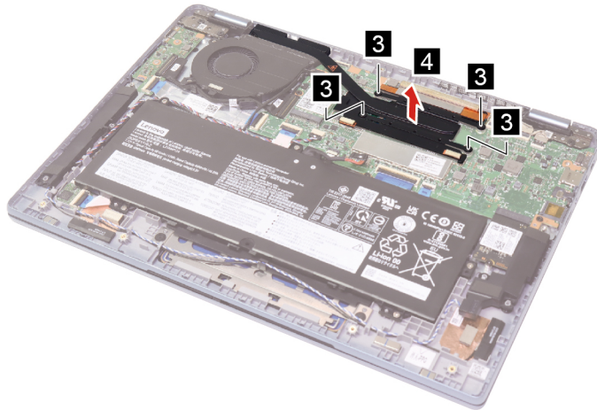
Figure 12. Loosen four screws and remove the heat sink
