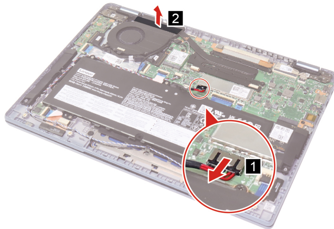
Figure 13. Disconnect the battery pack cable and peel off the tape
