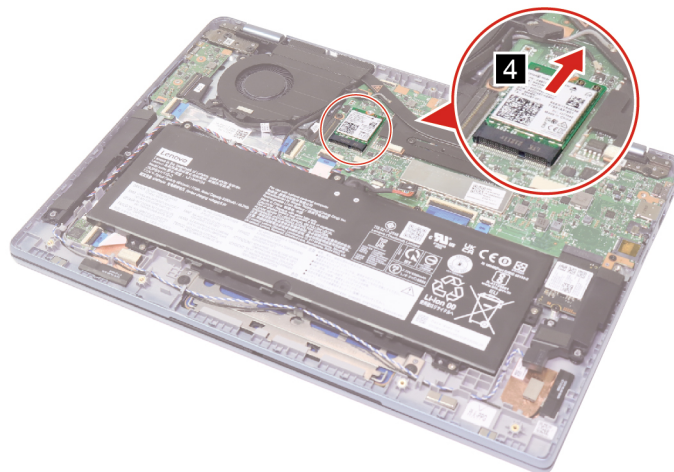
Figure 21. Remove the Wi-Fi card
