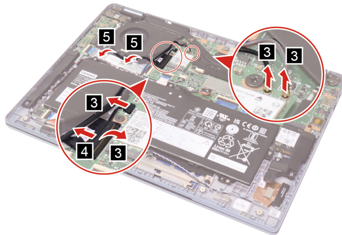
Figure 14. Disconnect cables
