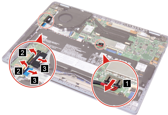
Figure 18. Disconnect the battery pack cable and the I/O board cables
