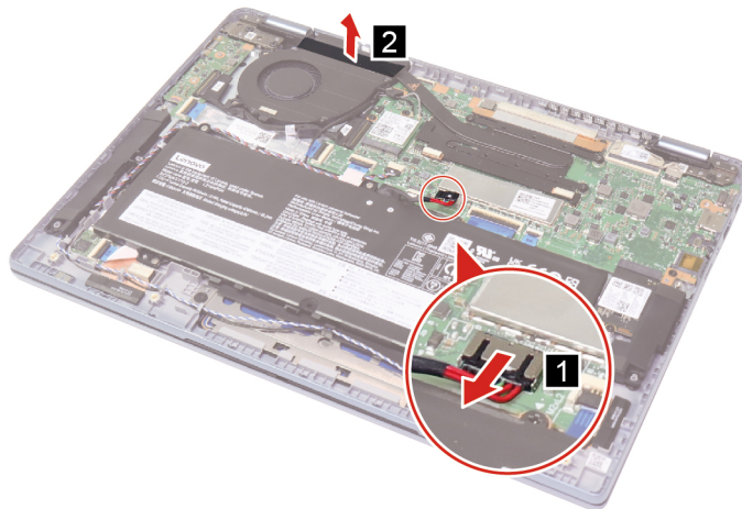
Figure 11. Disconnect the battery pack cable and peel off the tape
