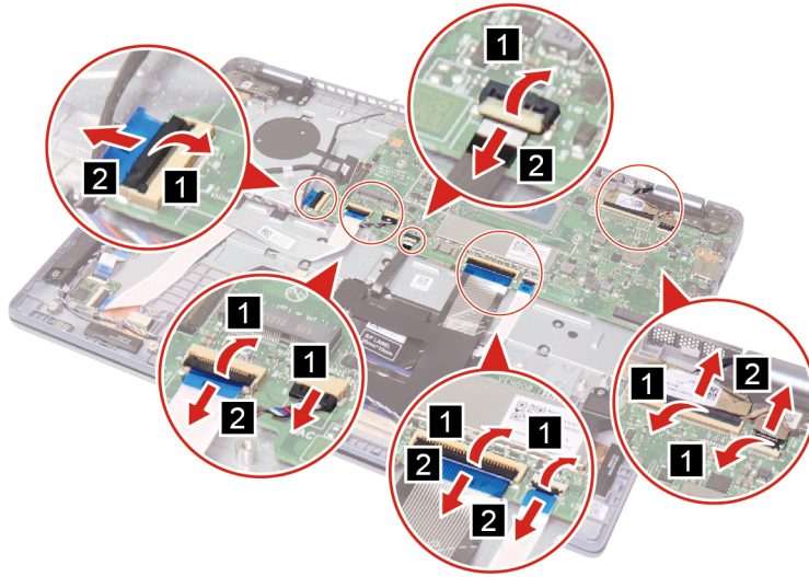
Figure 28. Disconnect all cables
