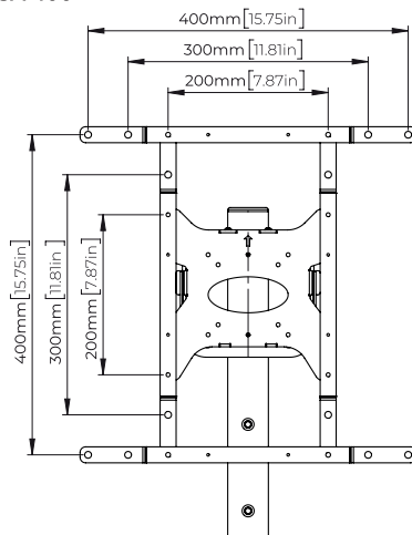
Mounting Plate VESA 400
