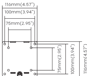
VESA Mount
