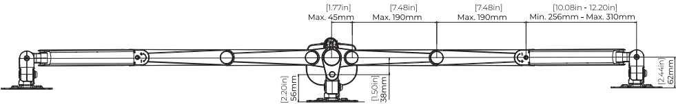
Top View
