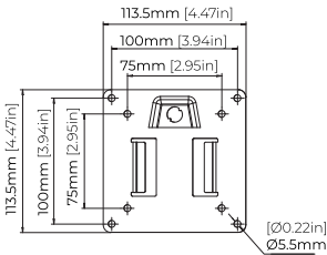
Interface Plate
