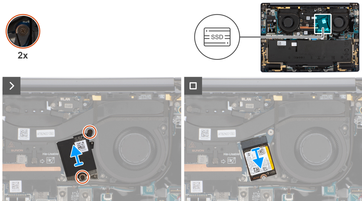
Figure 26. Removing the SSD
