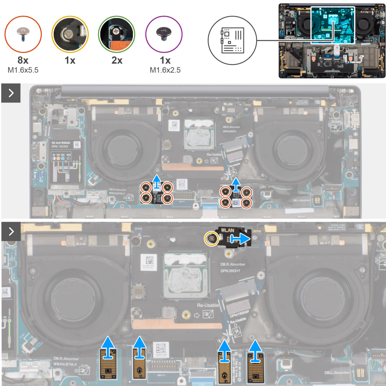
Figure 64. Removing the system board
