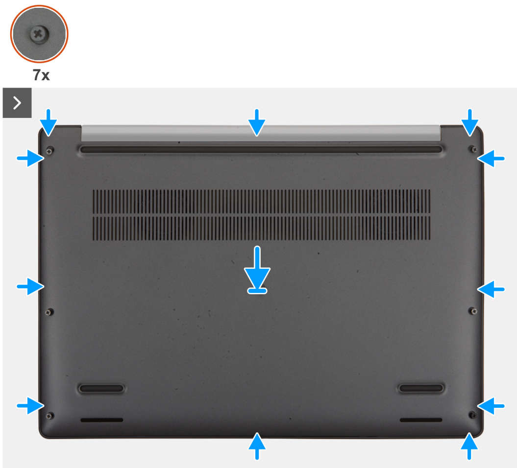
Figure 20. Installing the base cover
