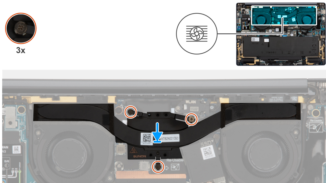
Figure 39. Installing the heat sink
