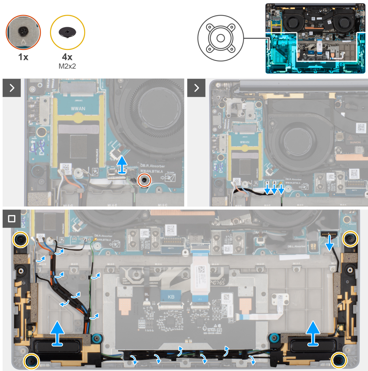
Figure 36. Removing the speakers with antennas (WWAN configuration)
