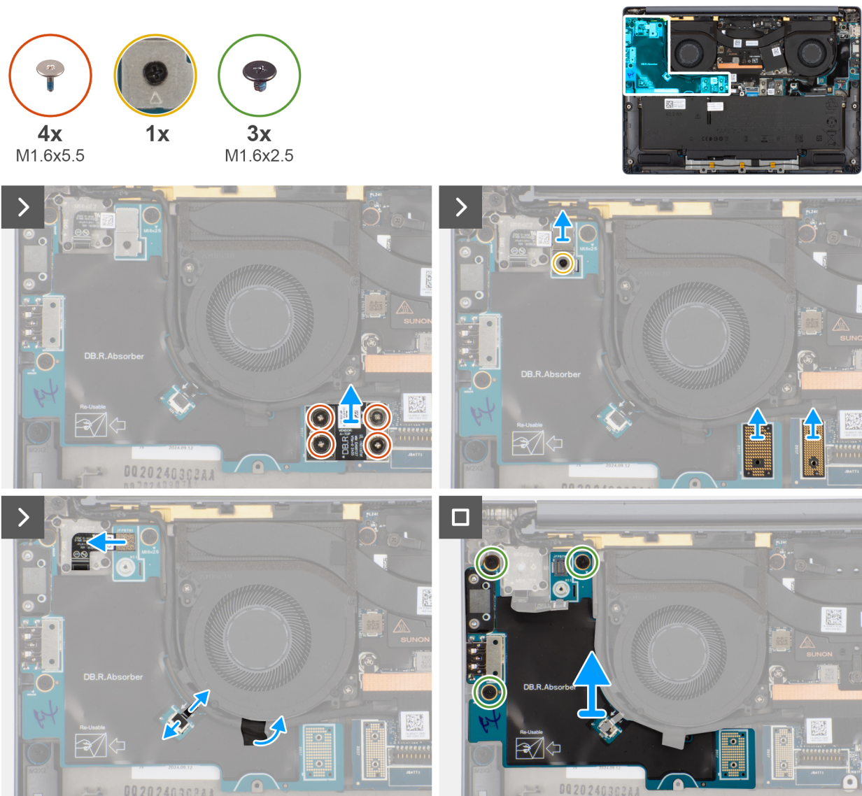
Figure 44. Removing the right I/O-board (without WWAN antennas)
