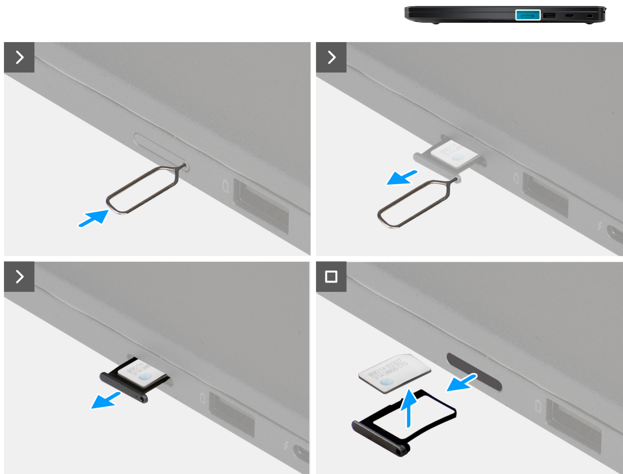
Figure 14. Removing the nano-SIM card
