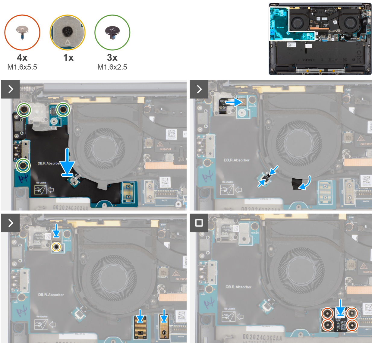
Figure 46. Installing the right I/O-board (without WWAN antennas)
