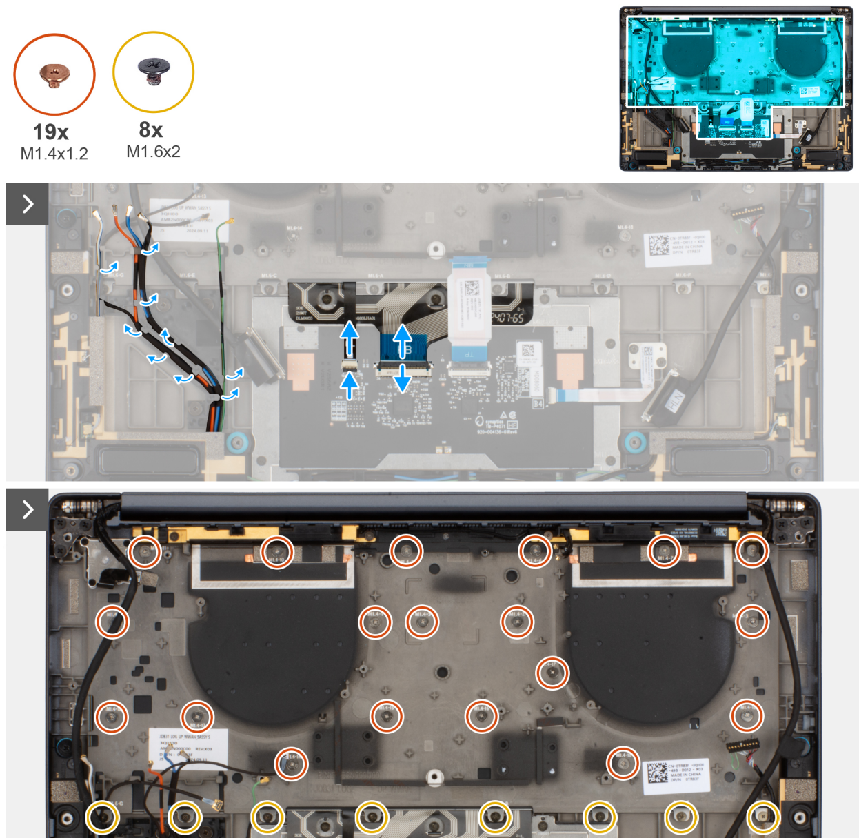
Figure 73. Removing the keyboard assembly
