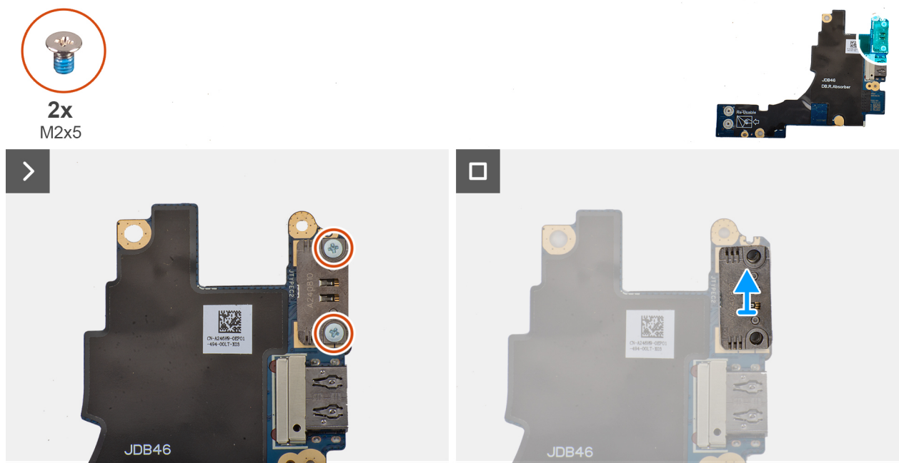
Figure 52. Removing the left USB Type-C module
