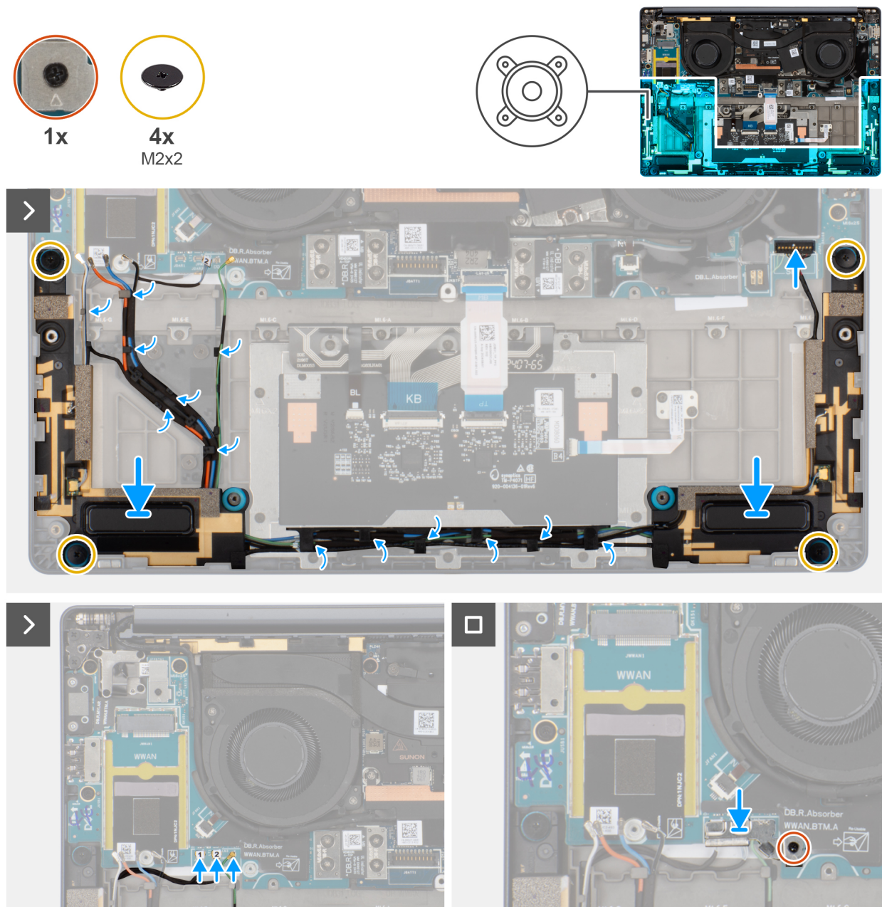
Figure 37. Installing the speakers with antennas (WWAN configuration)
