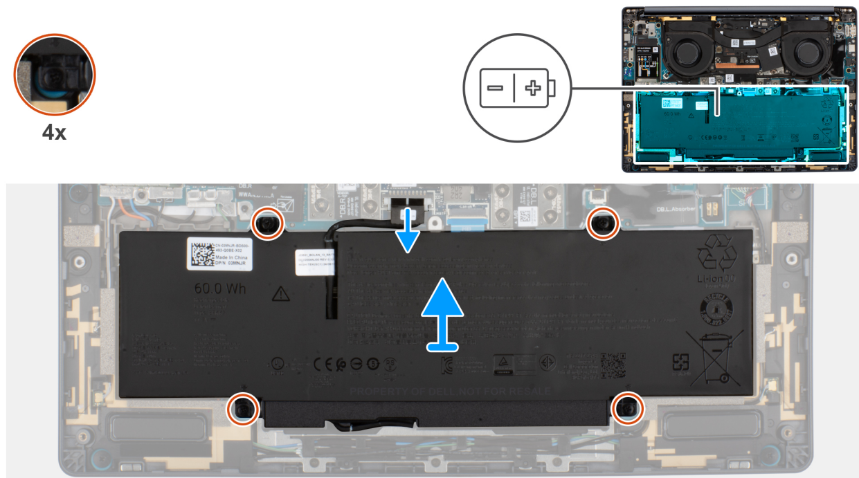
Figure 22. Loosen the captive screws
