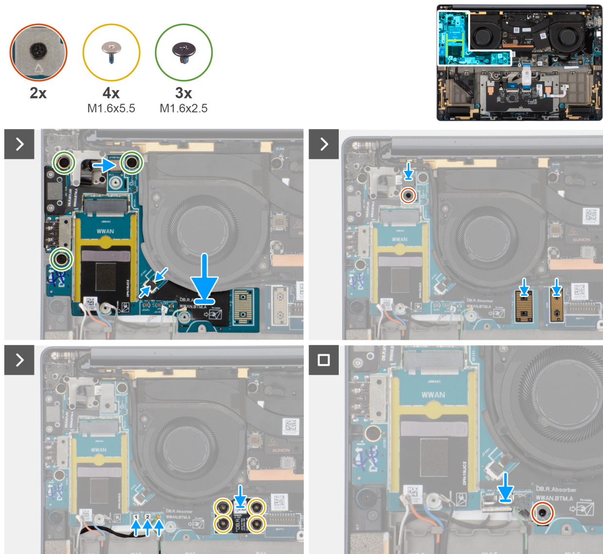
Figure 50. Installing the right I/O-board (with WWAN)
