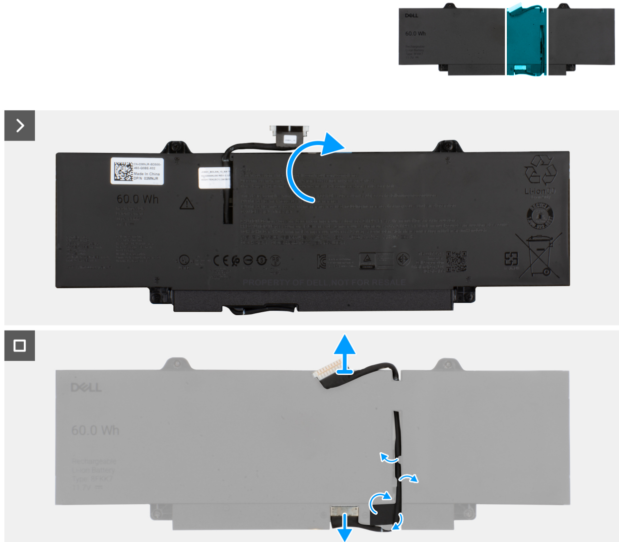
Figure 24. Removing and disconnecting the battery cable
