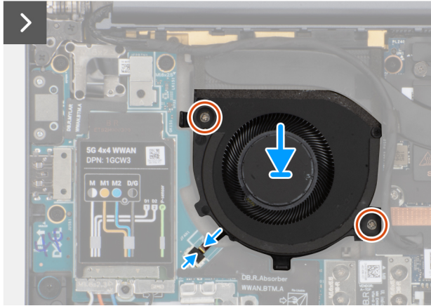
Figure 33. Installing the right fan
