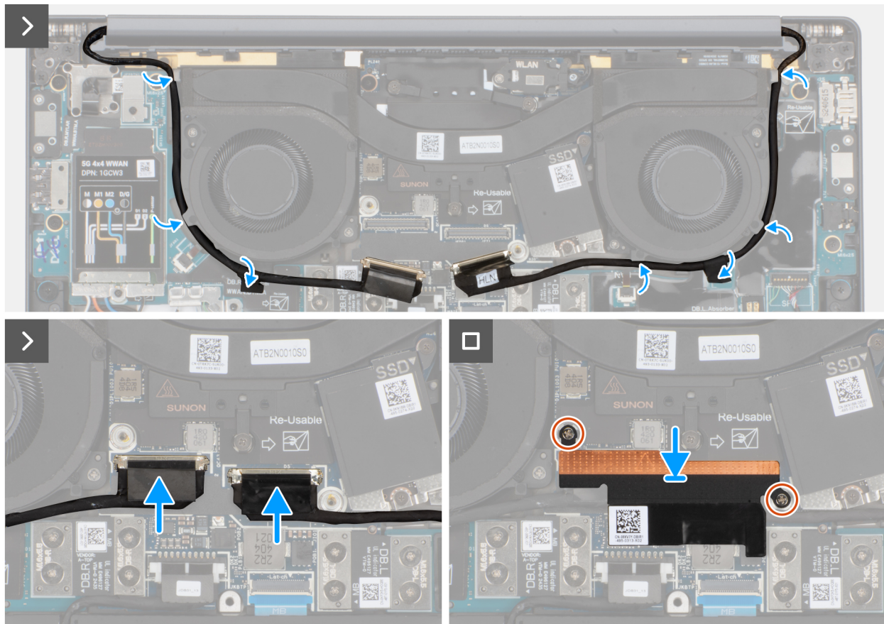
Figure 62. Connecting the display and camera cables
