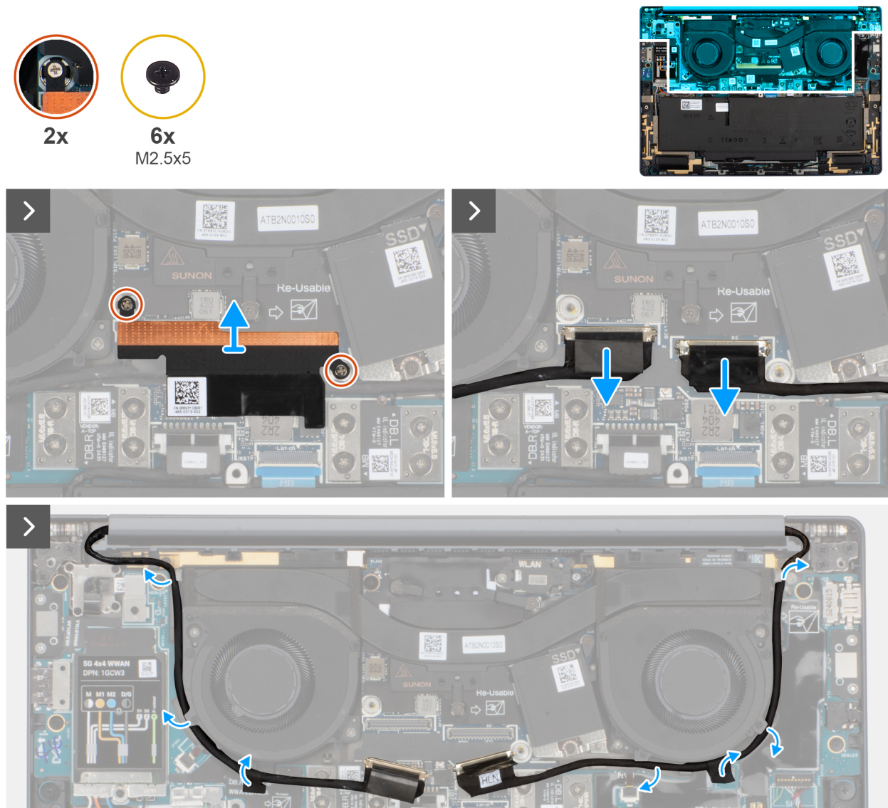
Figure 58. Disconnect the display and camera cables
