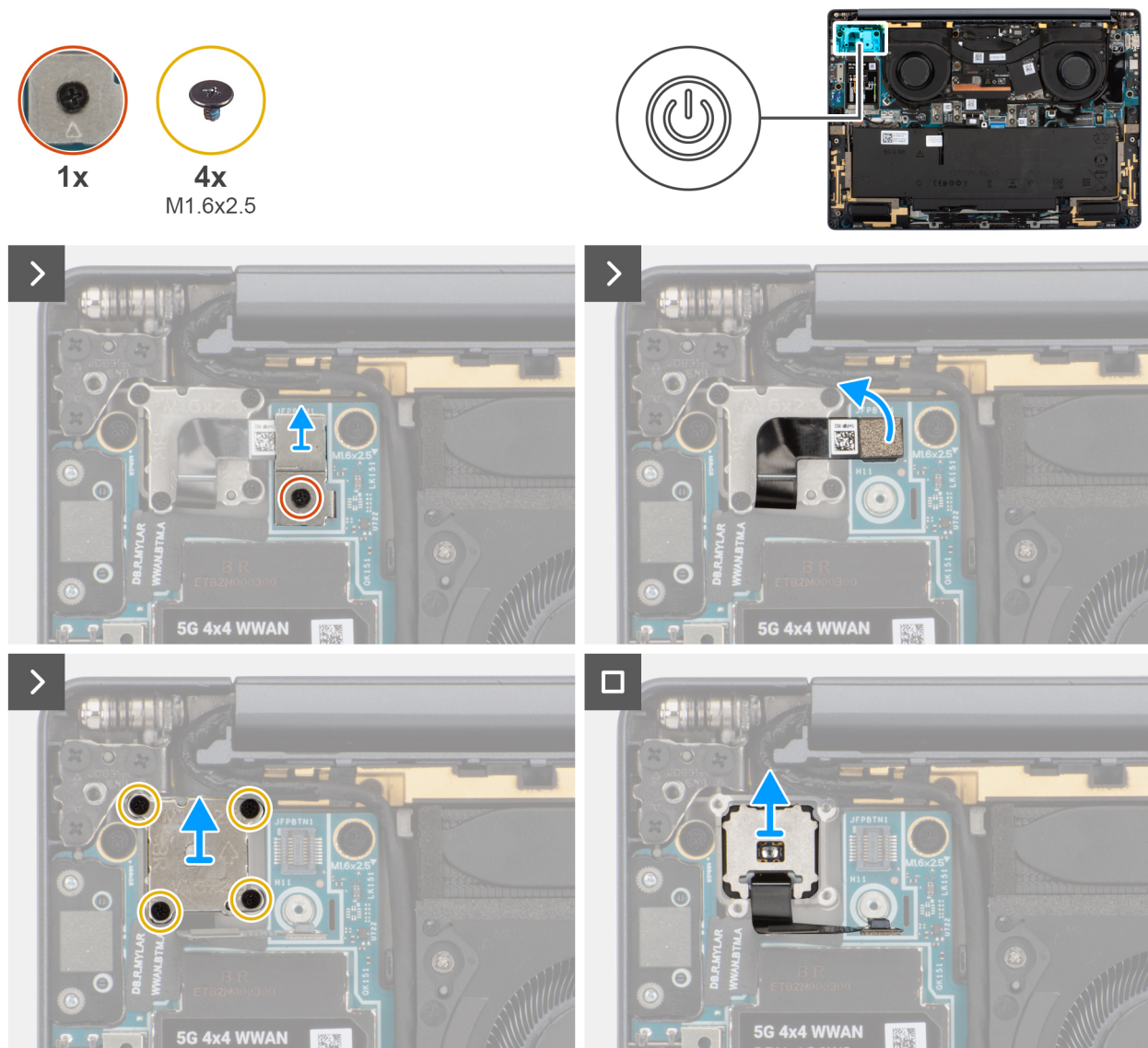
Figure 56. Removing the power button
