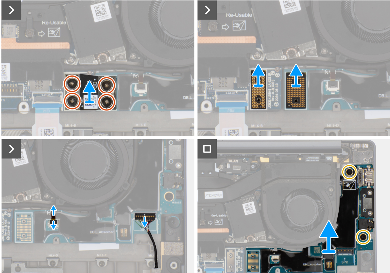
Figure 40. Removing the left I/O-board
