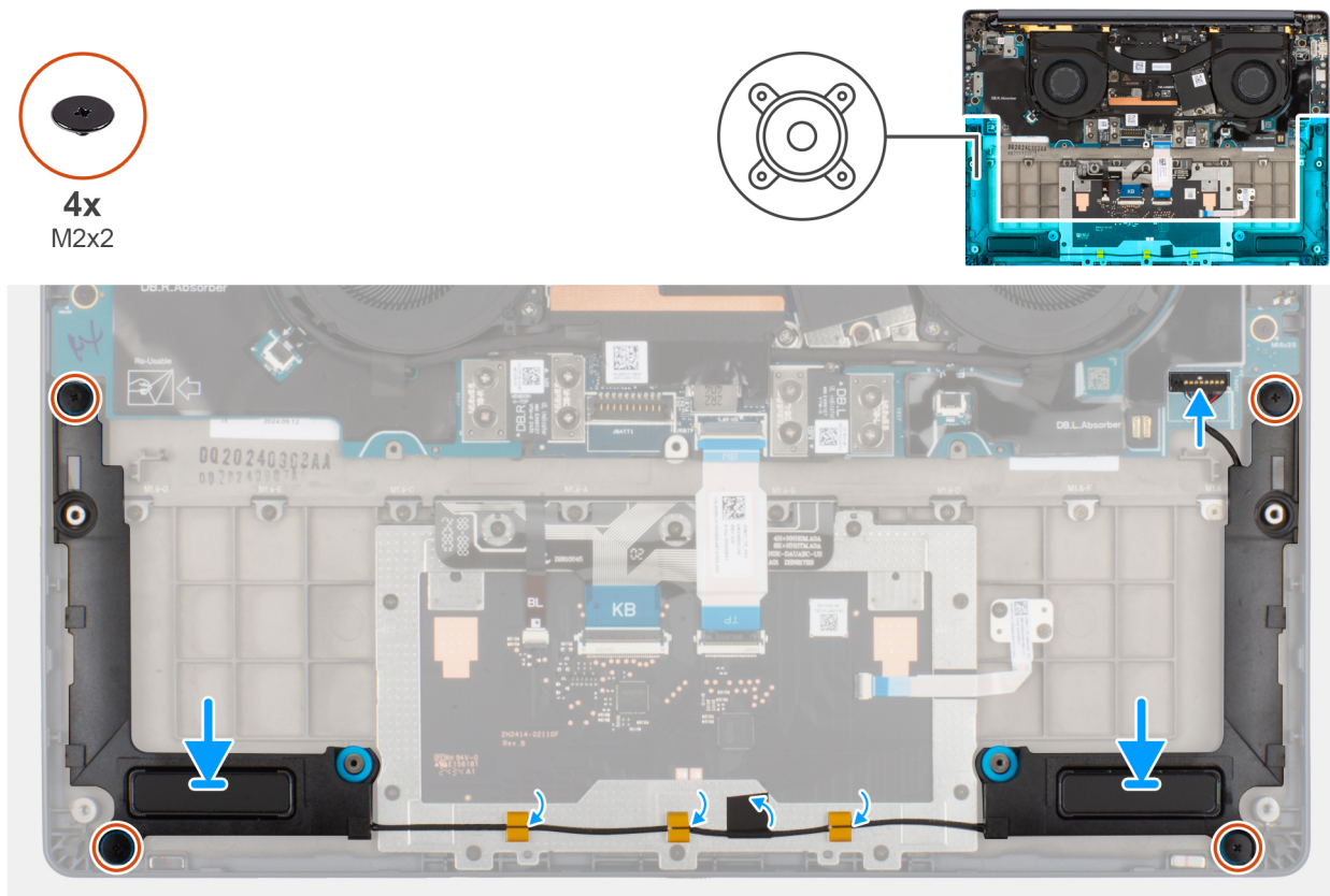
Figure 35. Installing the speakers (without WWAN)
