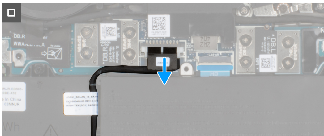
Figure 18. Disconnect the battery cable from the system board
