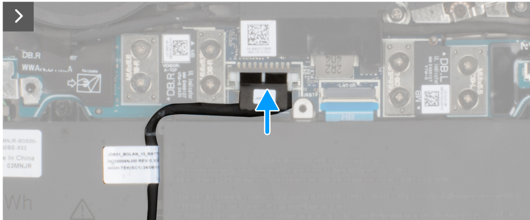
Figure 19. Connect the battery battery cable to the system board
