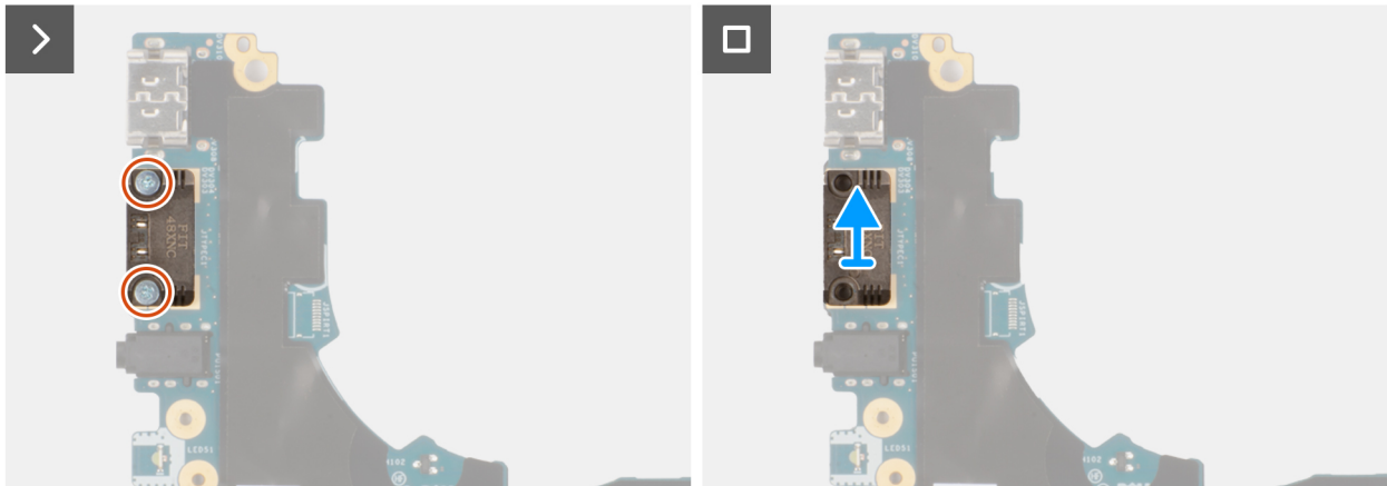
Figure 54. Removing the right USB Type-C module
