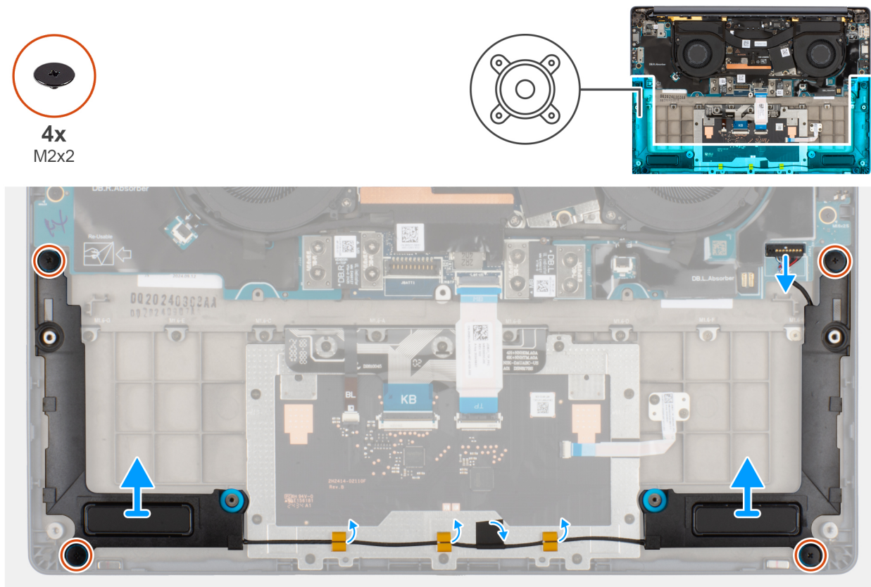
Figure 34. Removing the speakers without antenna (WLAN configuration)
