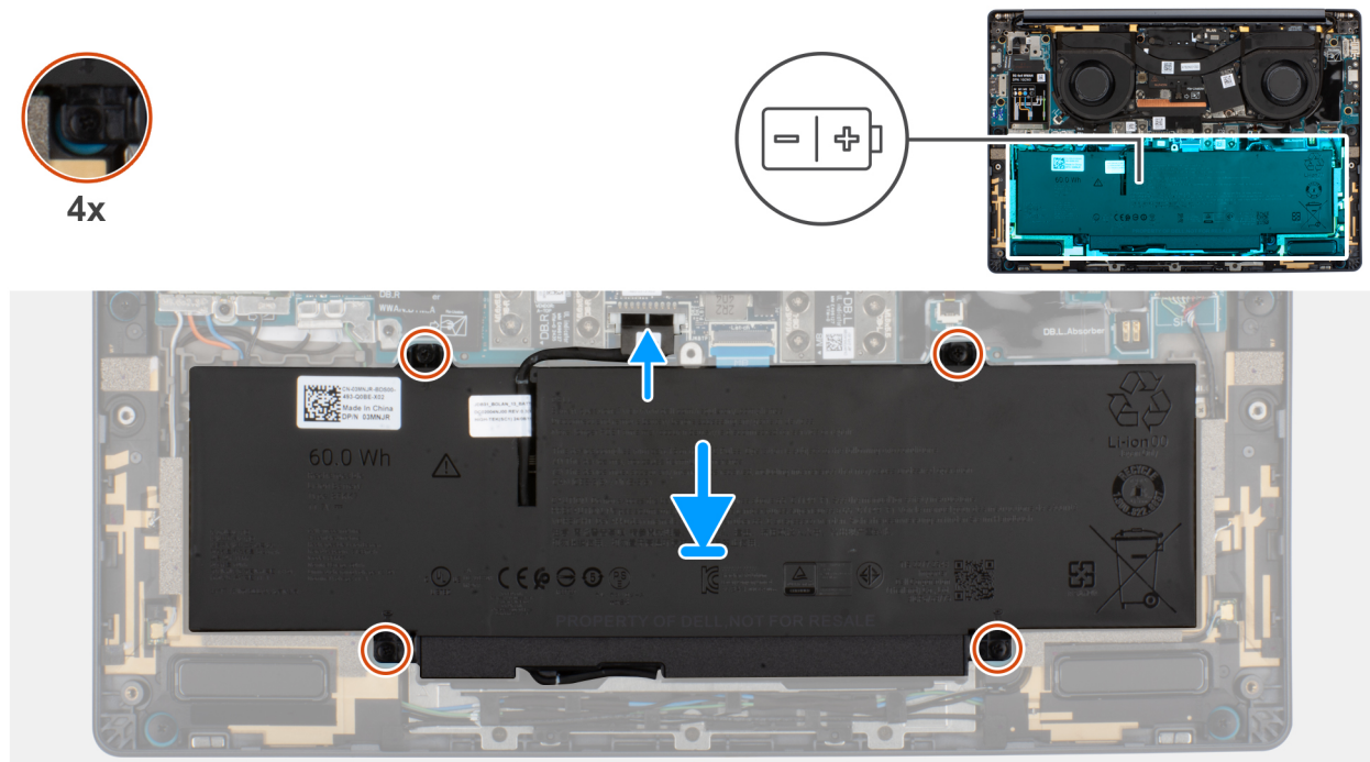
Figure 23. Installing the battery
