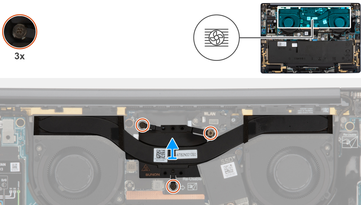
Figure 38. Removing the heat sink
