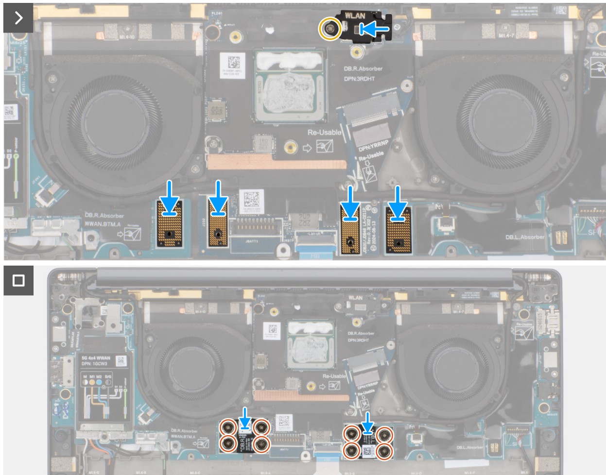
Figure 71. Installing the system board
