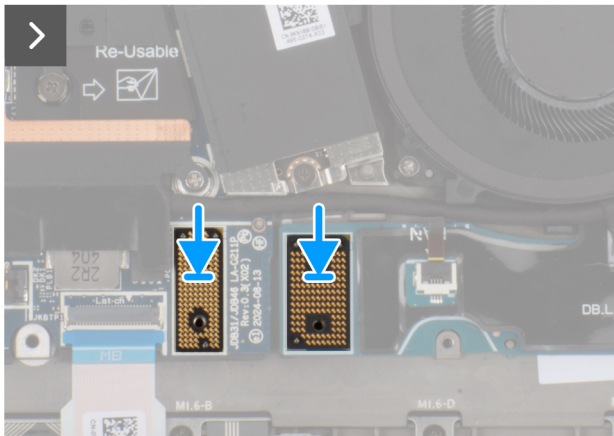
Figure 42. Installing the left I/O-board
