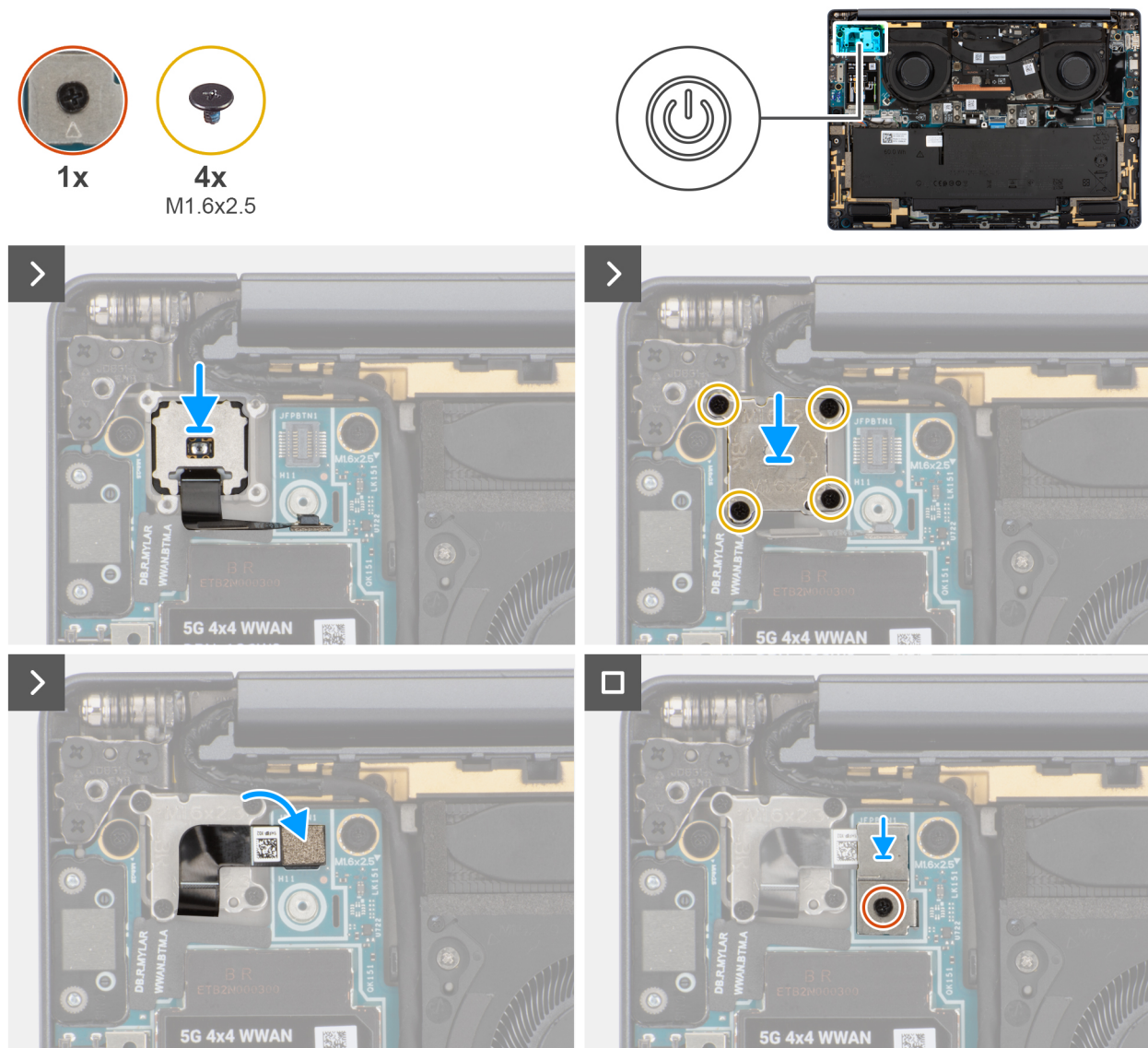
Figure 57. Installing the power button
