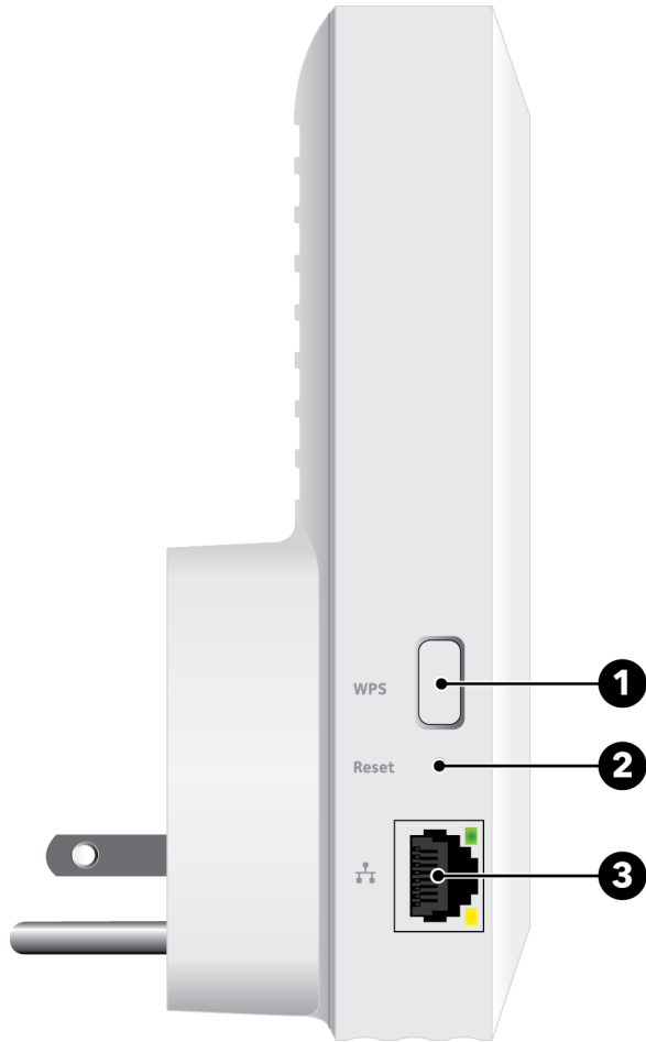
Figure 3. Back panel
