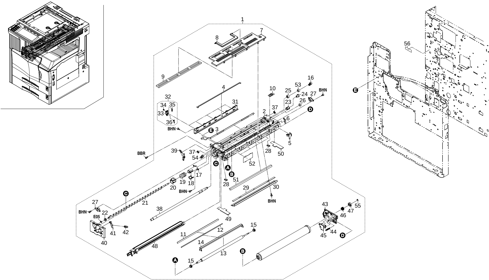
FIG. 15 CLEANING SECTION
