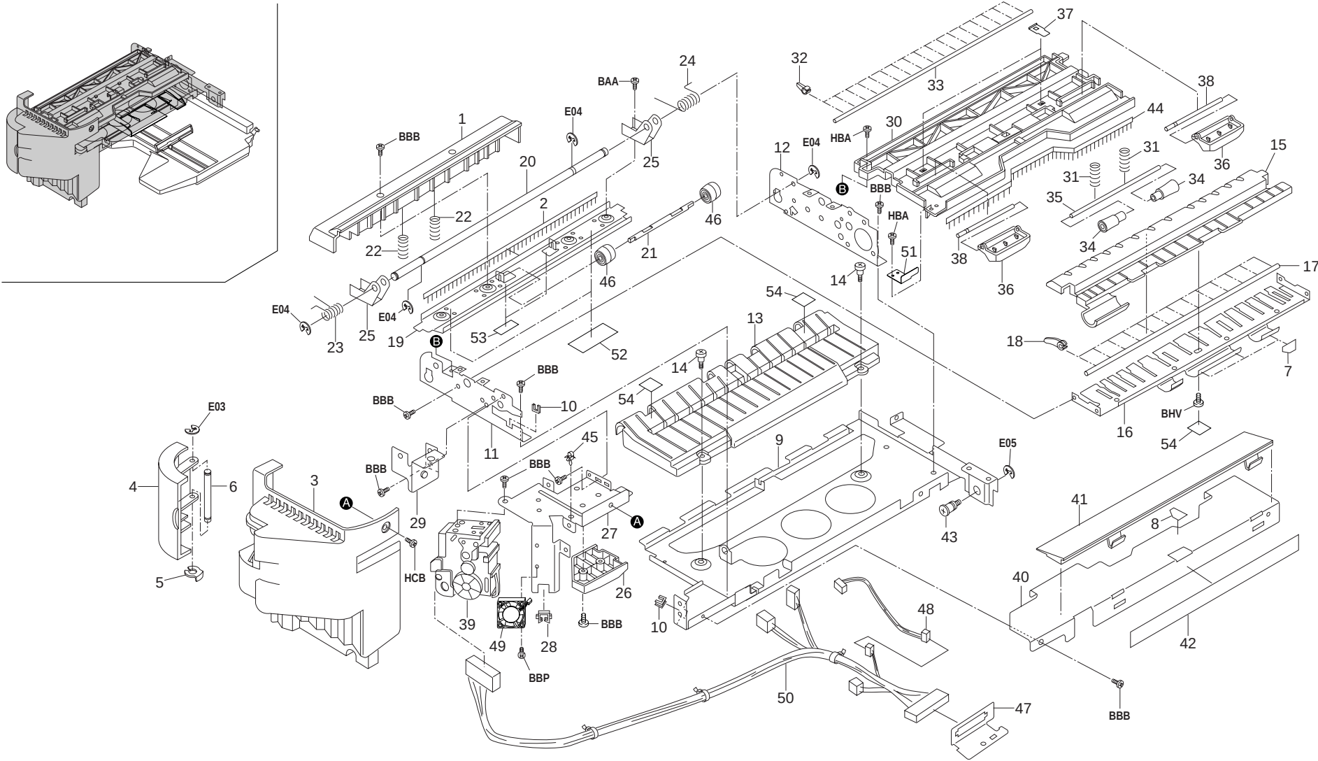
FIG. 1 EXTERIOR COVERS
