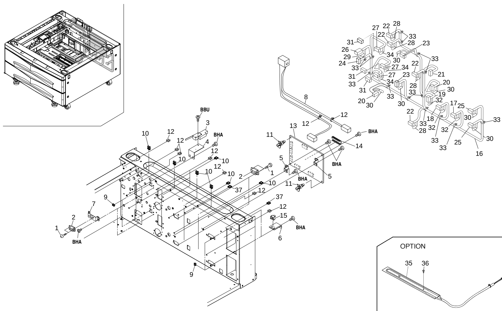
FIG. 6 ELECTRICAL COMPONENTS
