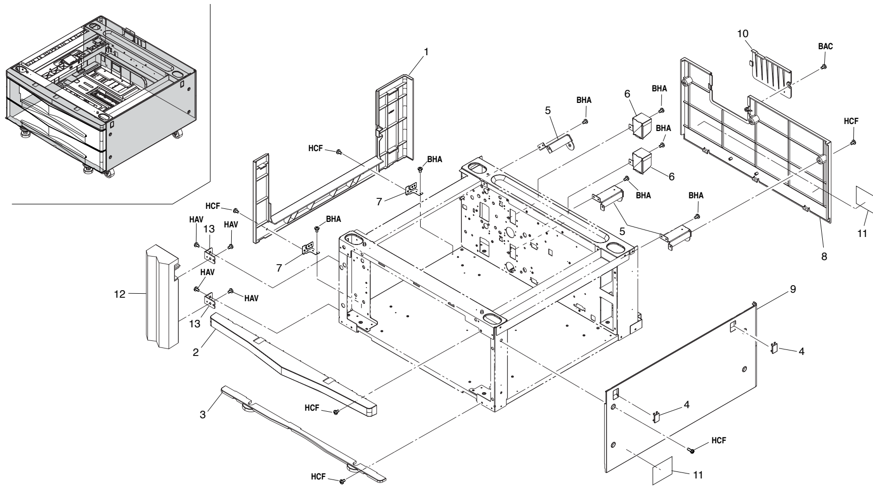
FIG. 1 COVER
