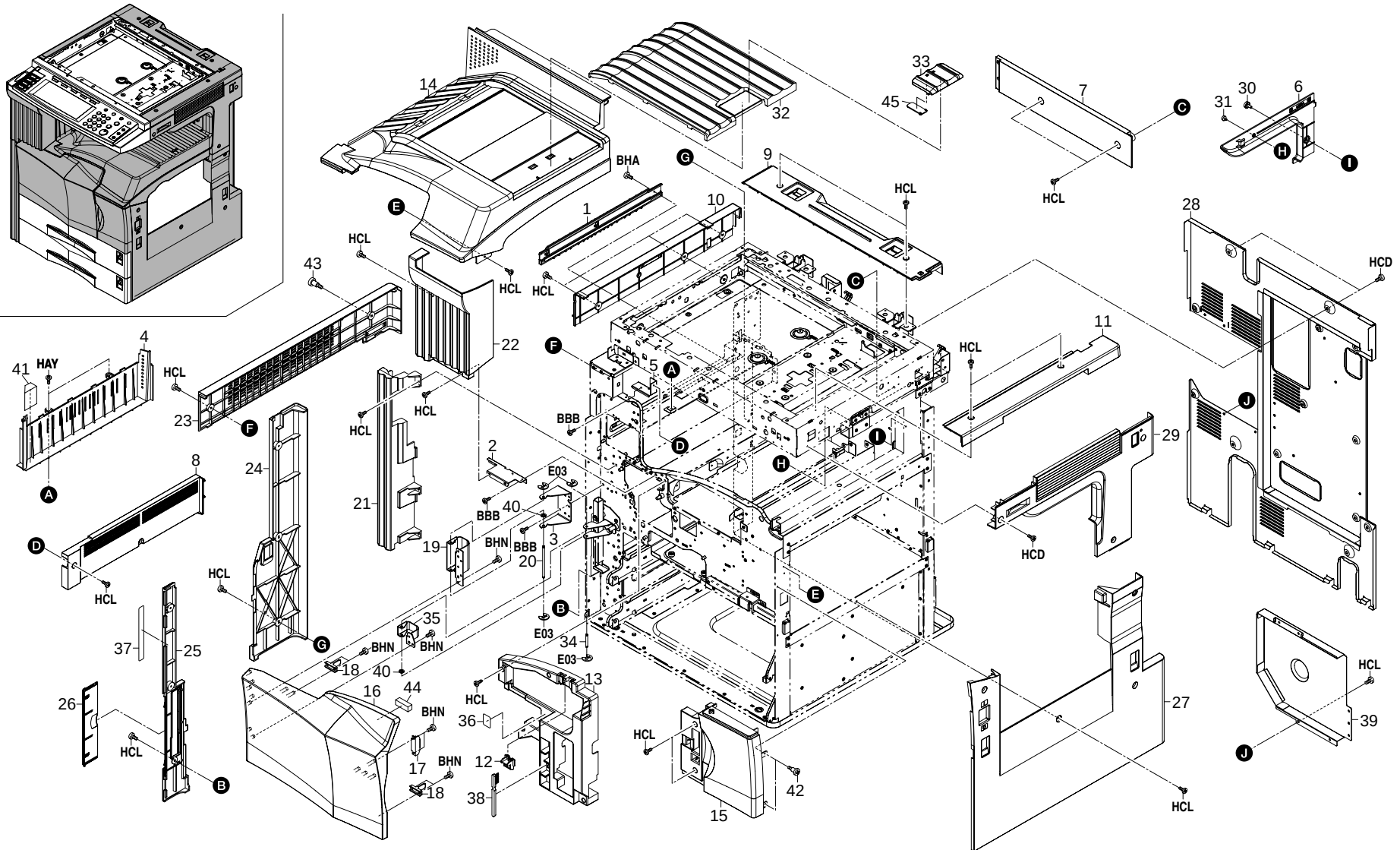
FIG. 1 EXTERIOR COVERS
