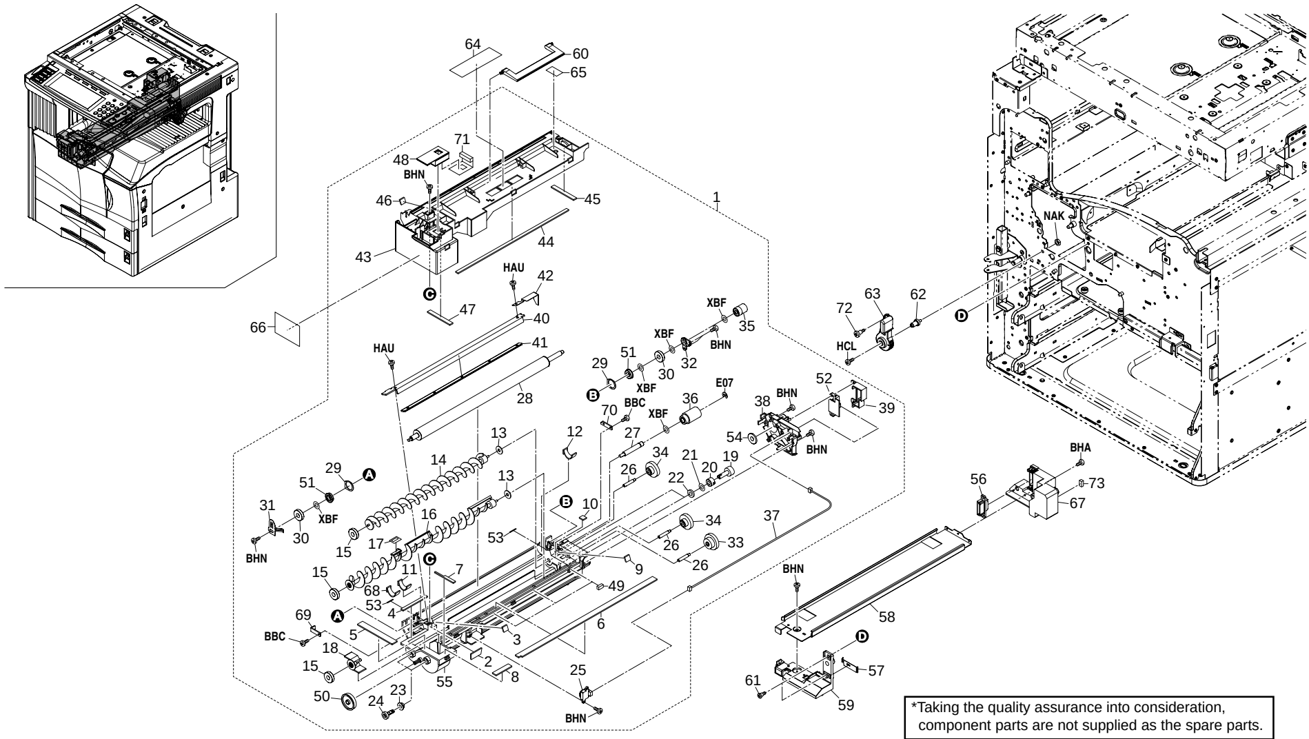
FIG. 13 DEVELOPING SECTION
