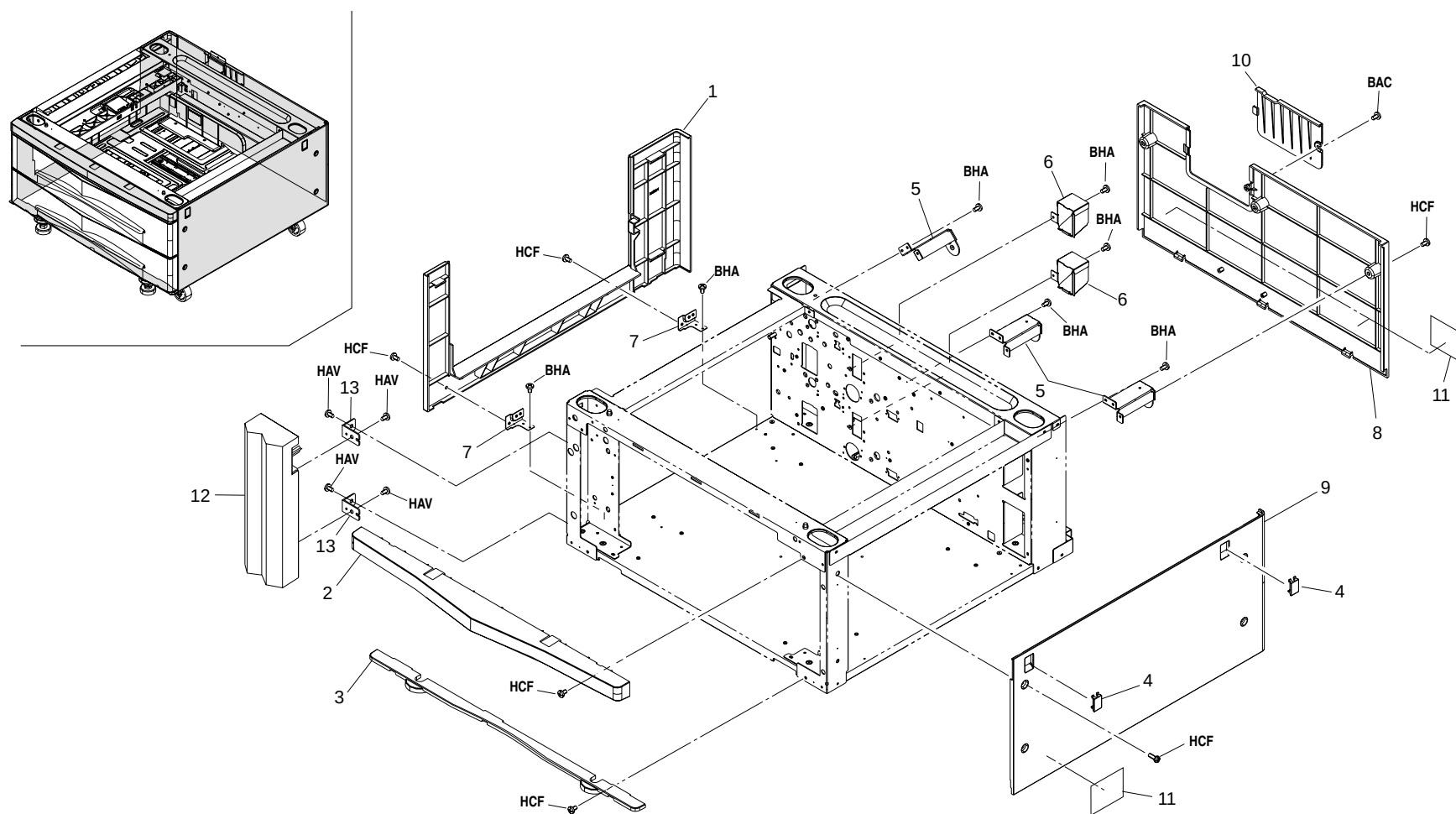
FIG. 1 COVER
