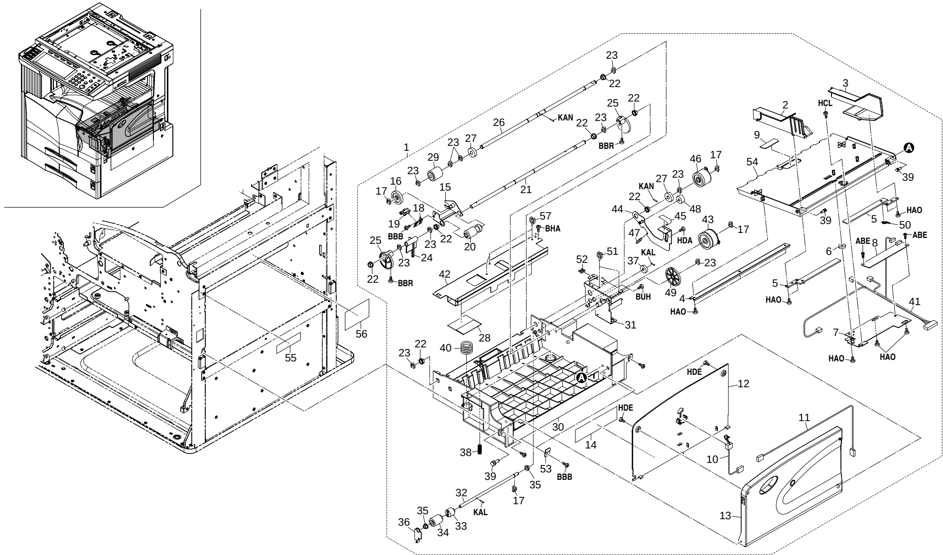
FIG. 10 BYPASS UNIT
