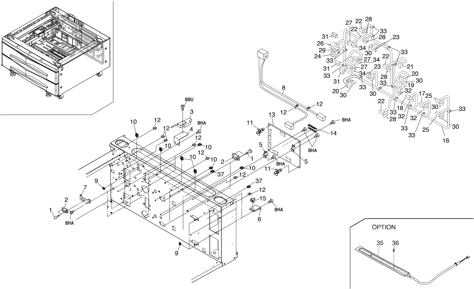
FIG. 6 ELECTRICAL COMPONENTS
