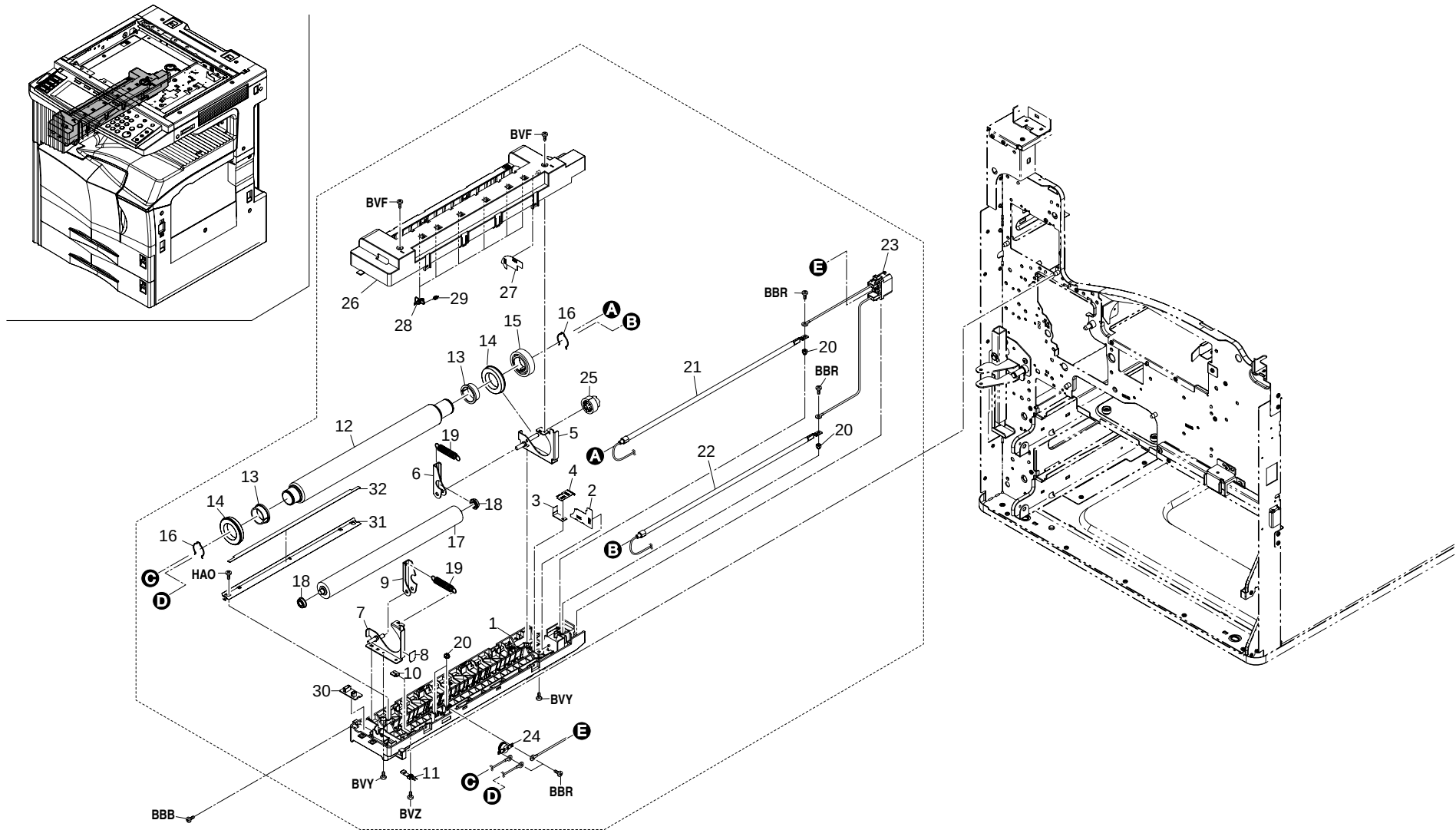
FIG. 14 FIXING SECTION
