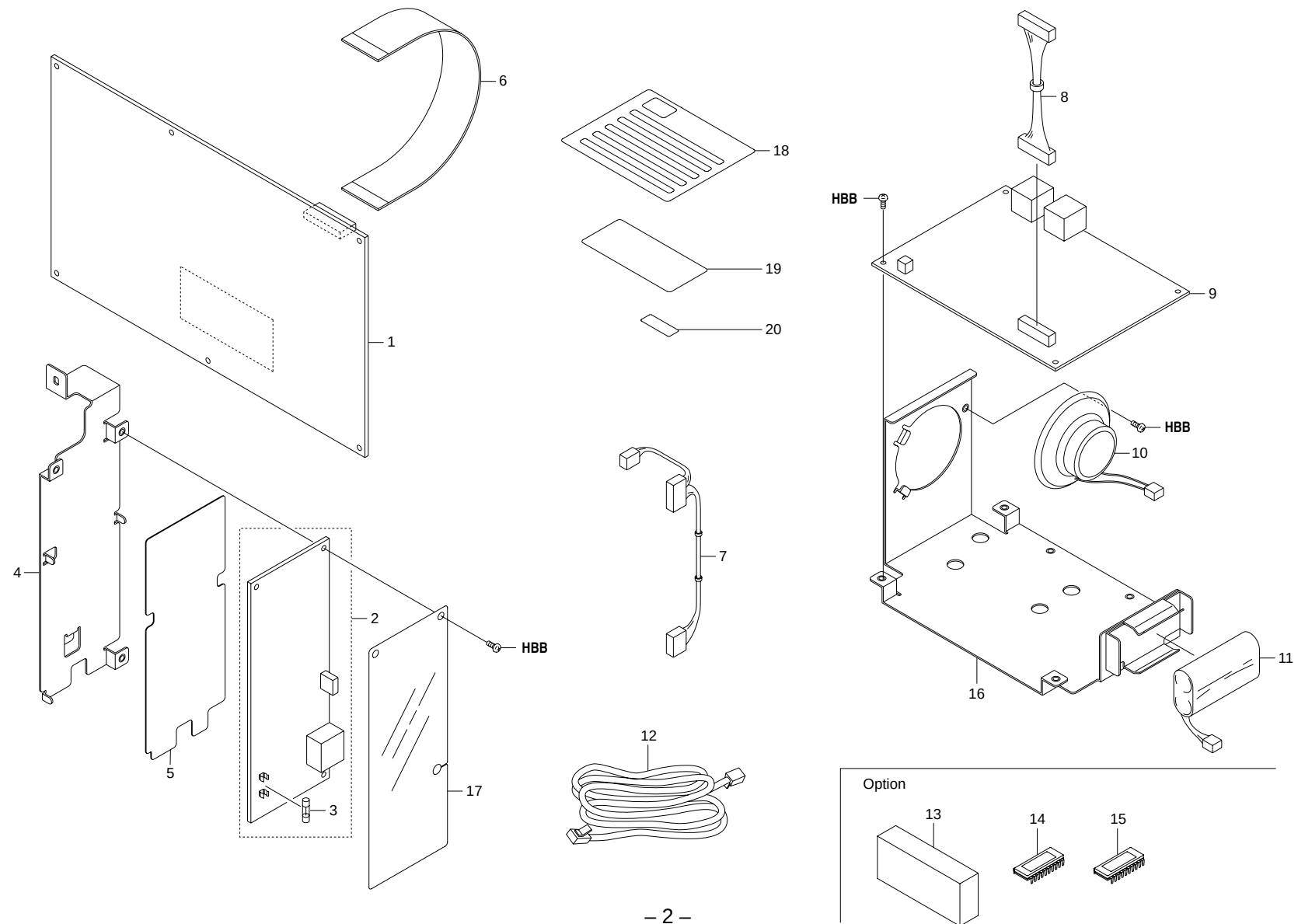
FIG. 1 FAX System(C)
