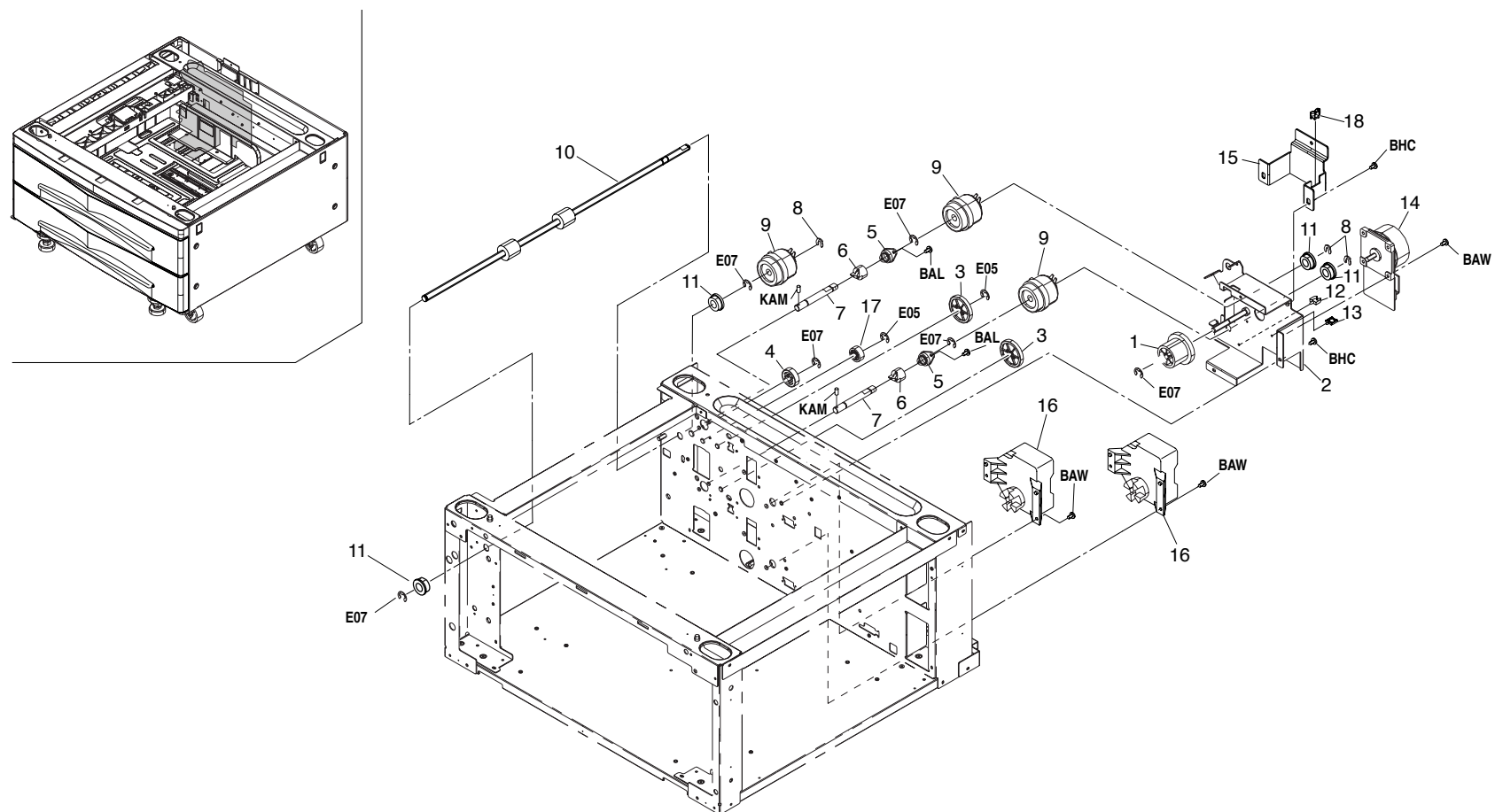
FIG. 5 DRIVING SECTION
