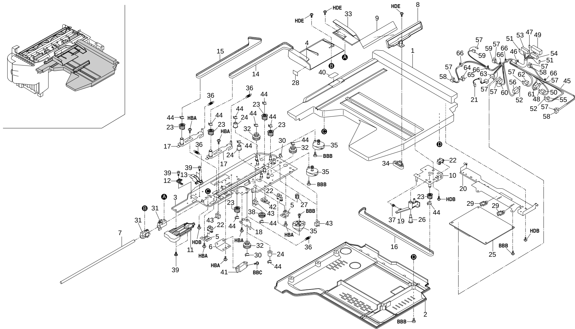
FIG. 3 TRAY SECTION
