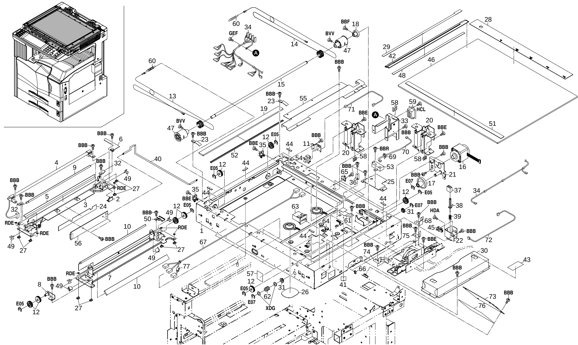
FIG. 9 OPTICAL SECTION
