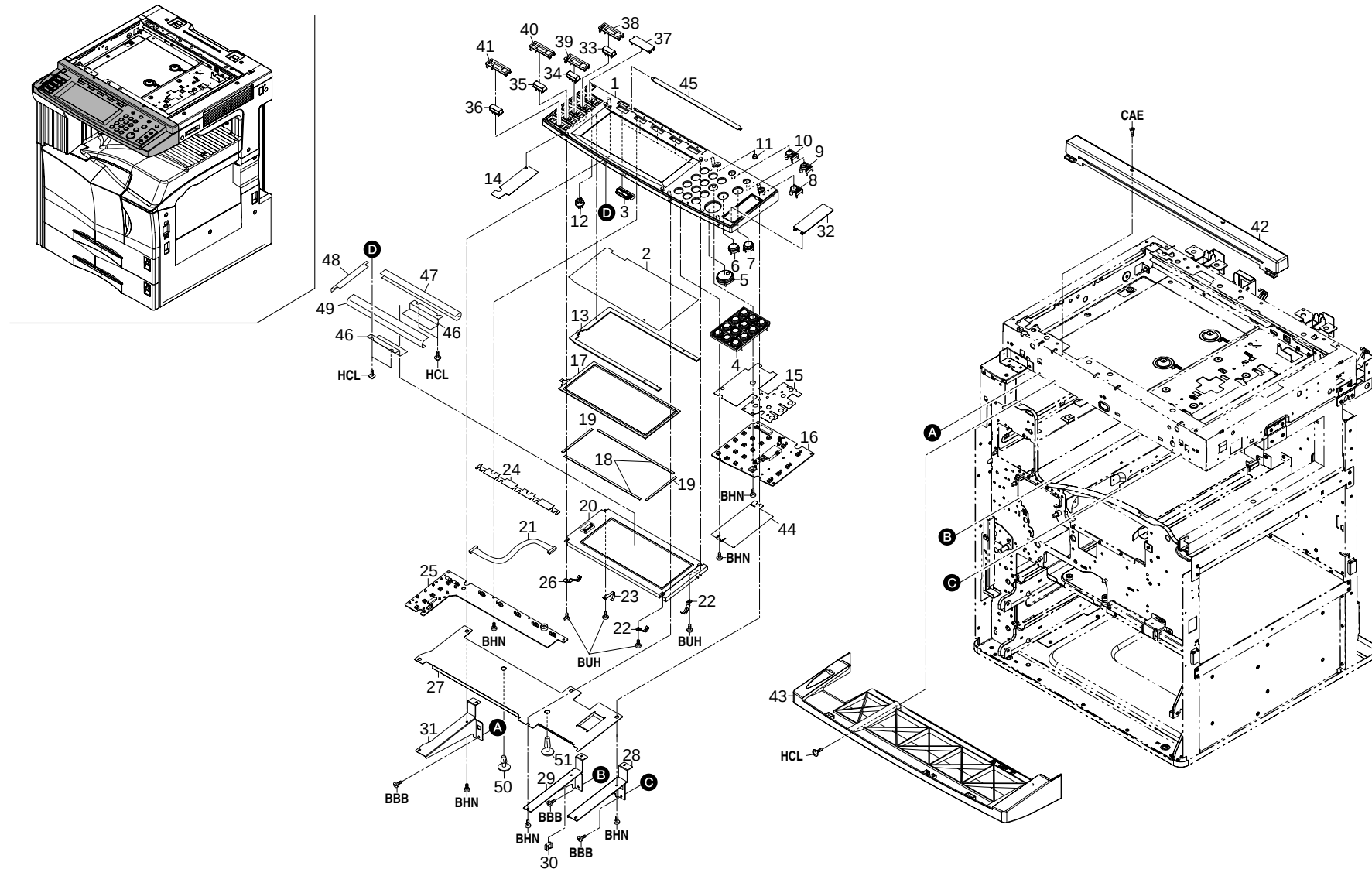
FIG. 19 OPERATION UNIT
