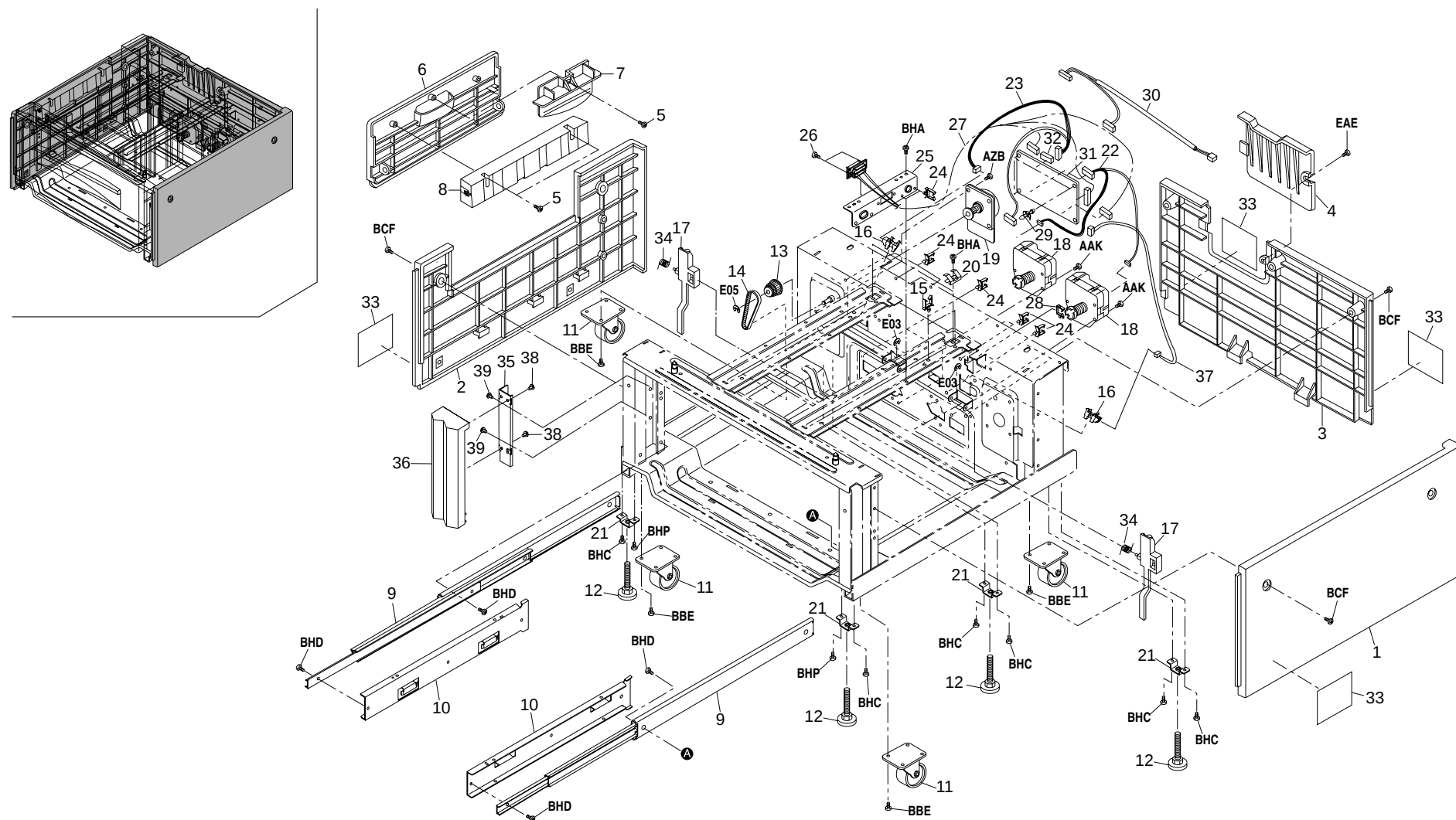
FIG. 1 EXTERIOR COVERS
