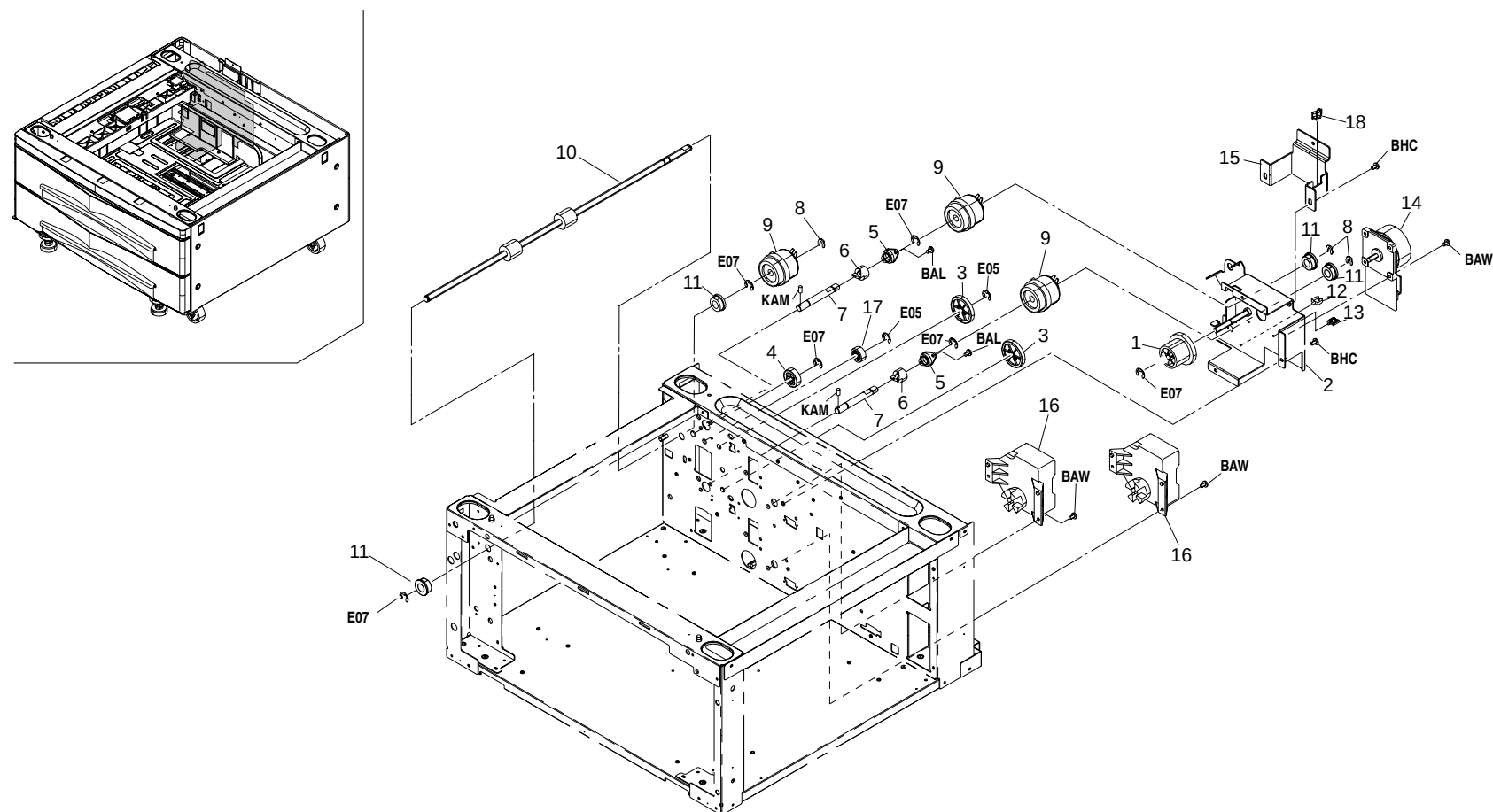
FIG. 5 DRIVING SECTION
