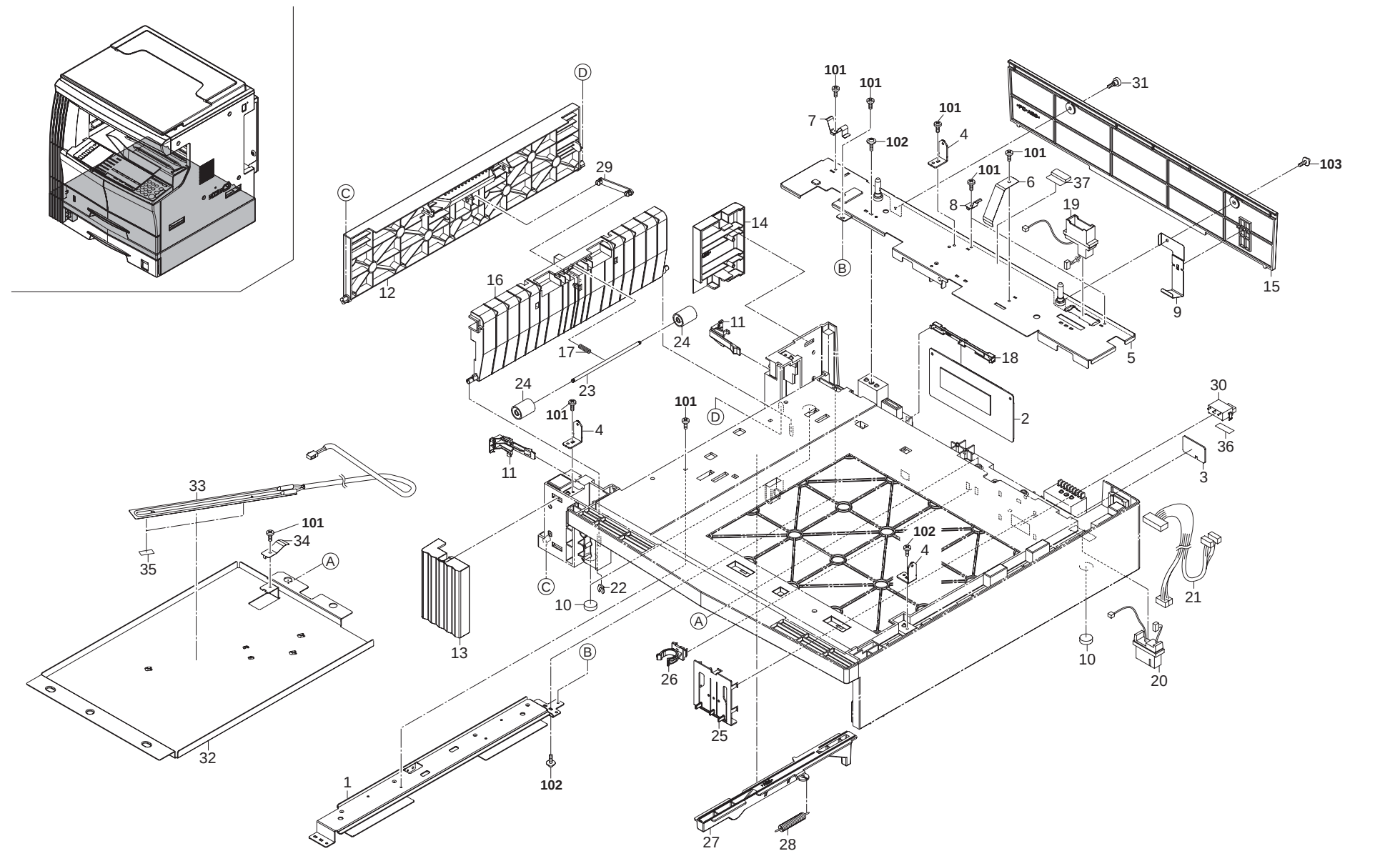
FIG. 3 Exterior Covers (Lower Cassette)
