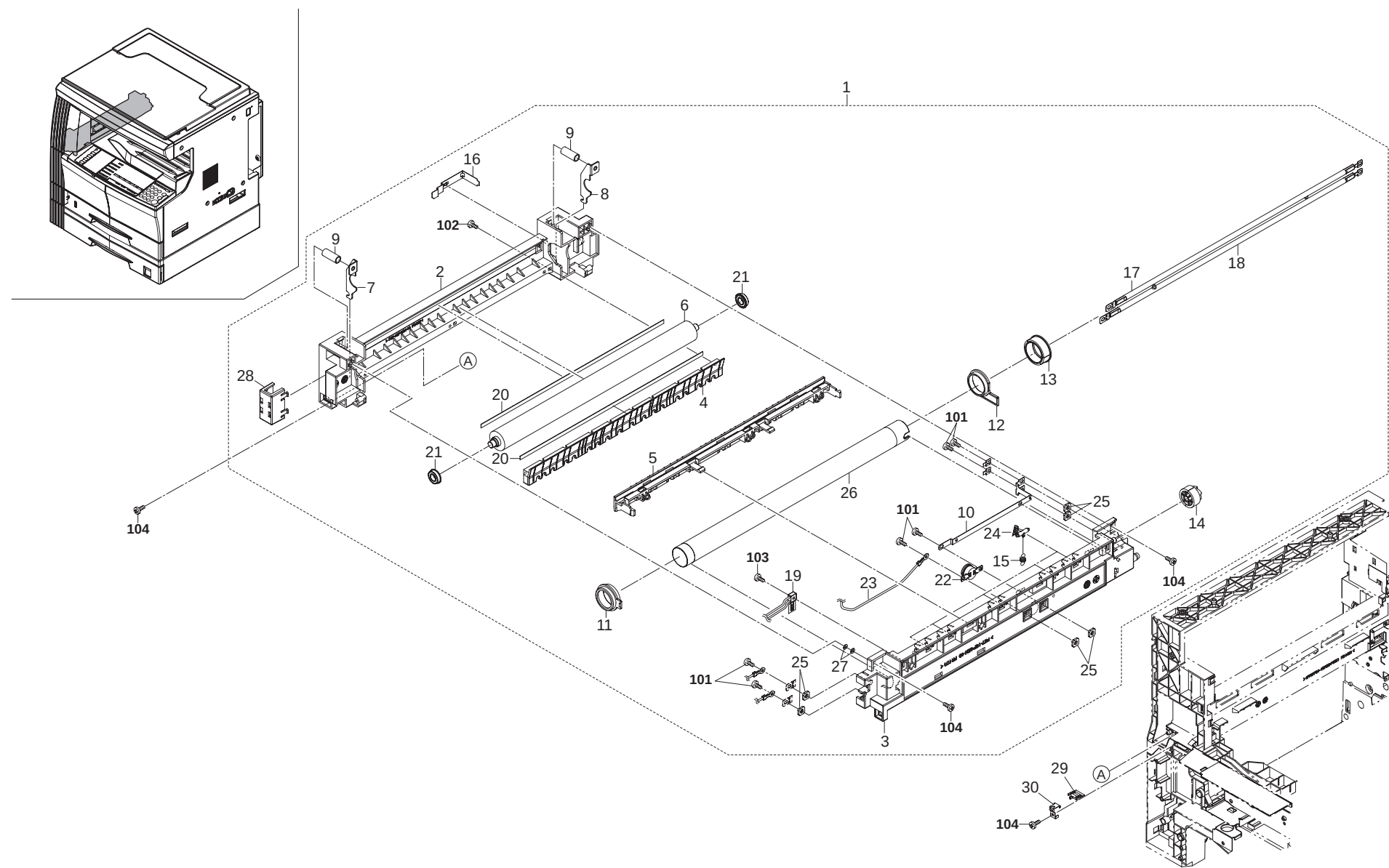
FIG. 12 Fuser Unit
