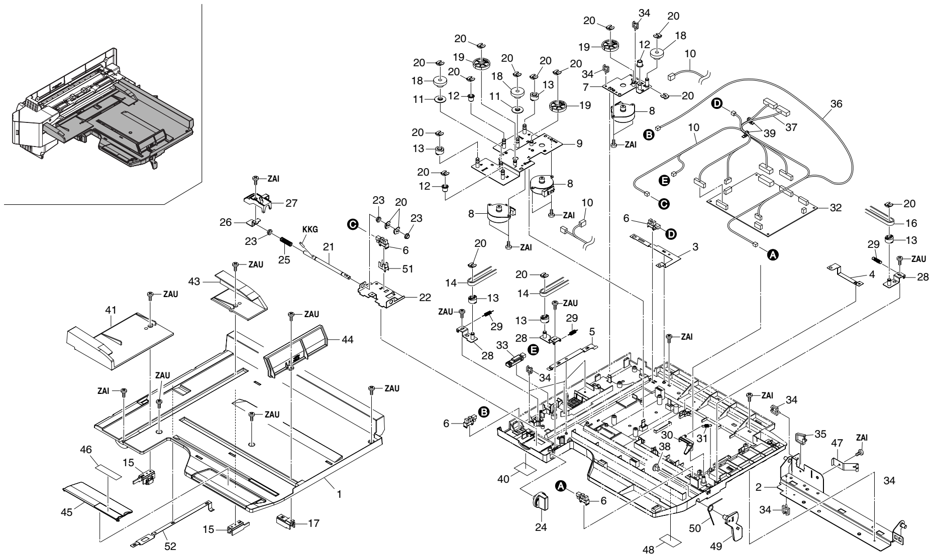
FIG. 3 TRAY SECTION
