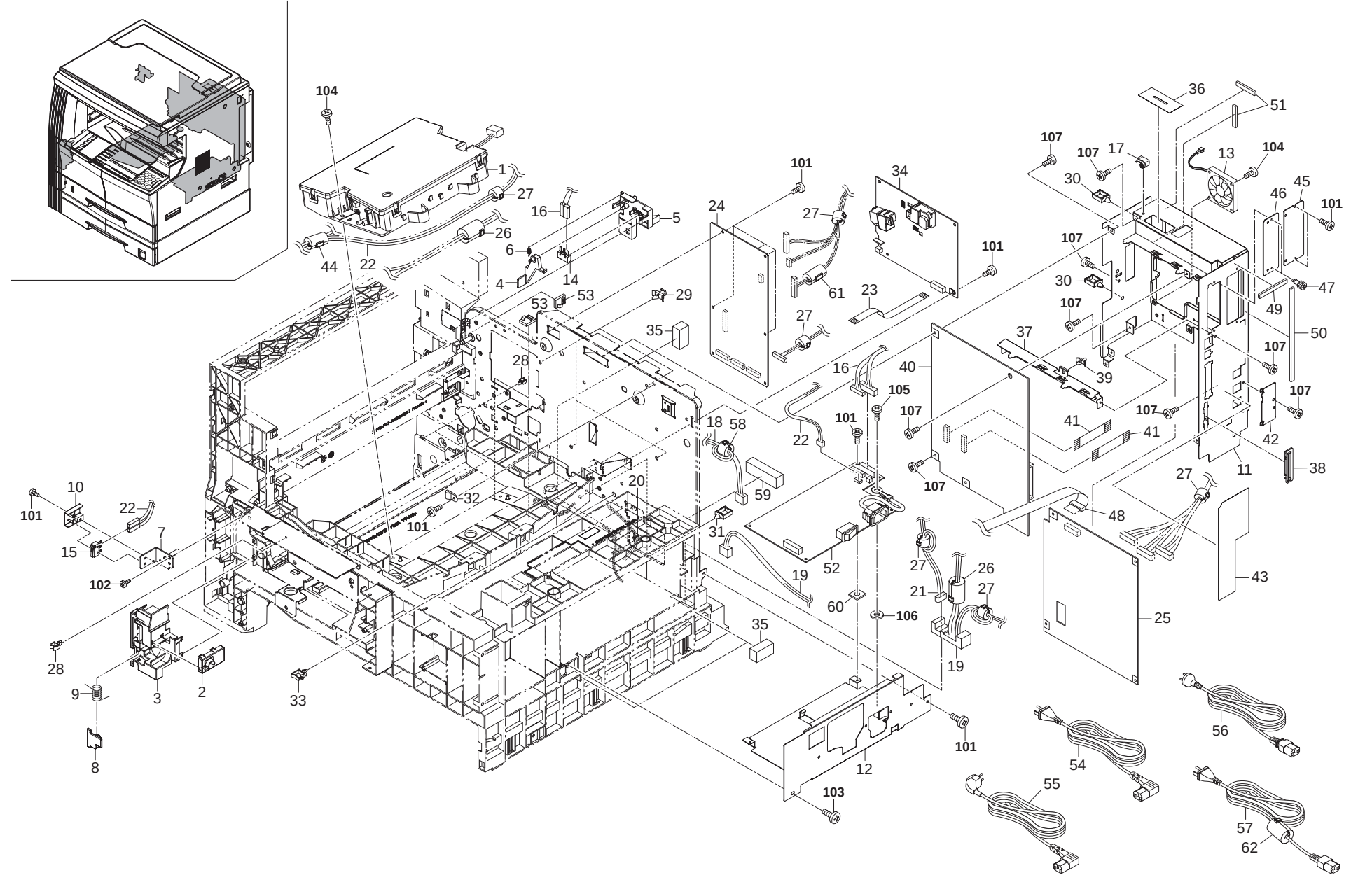
FIG. 14 Electrical Components
