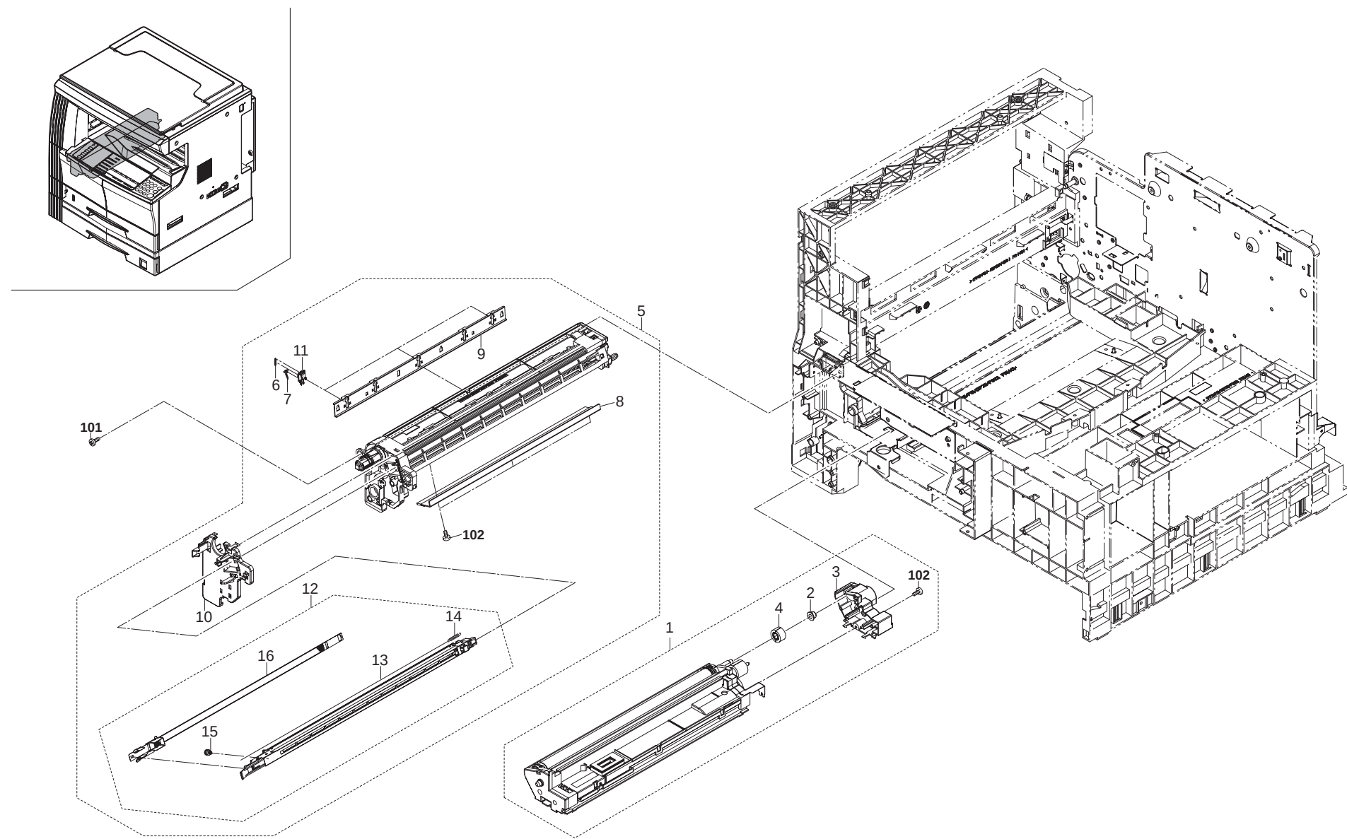
FIG. 11 Imaging Unit
