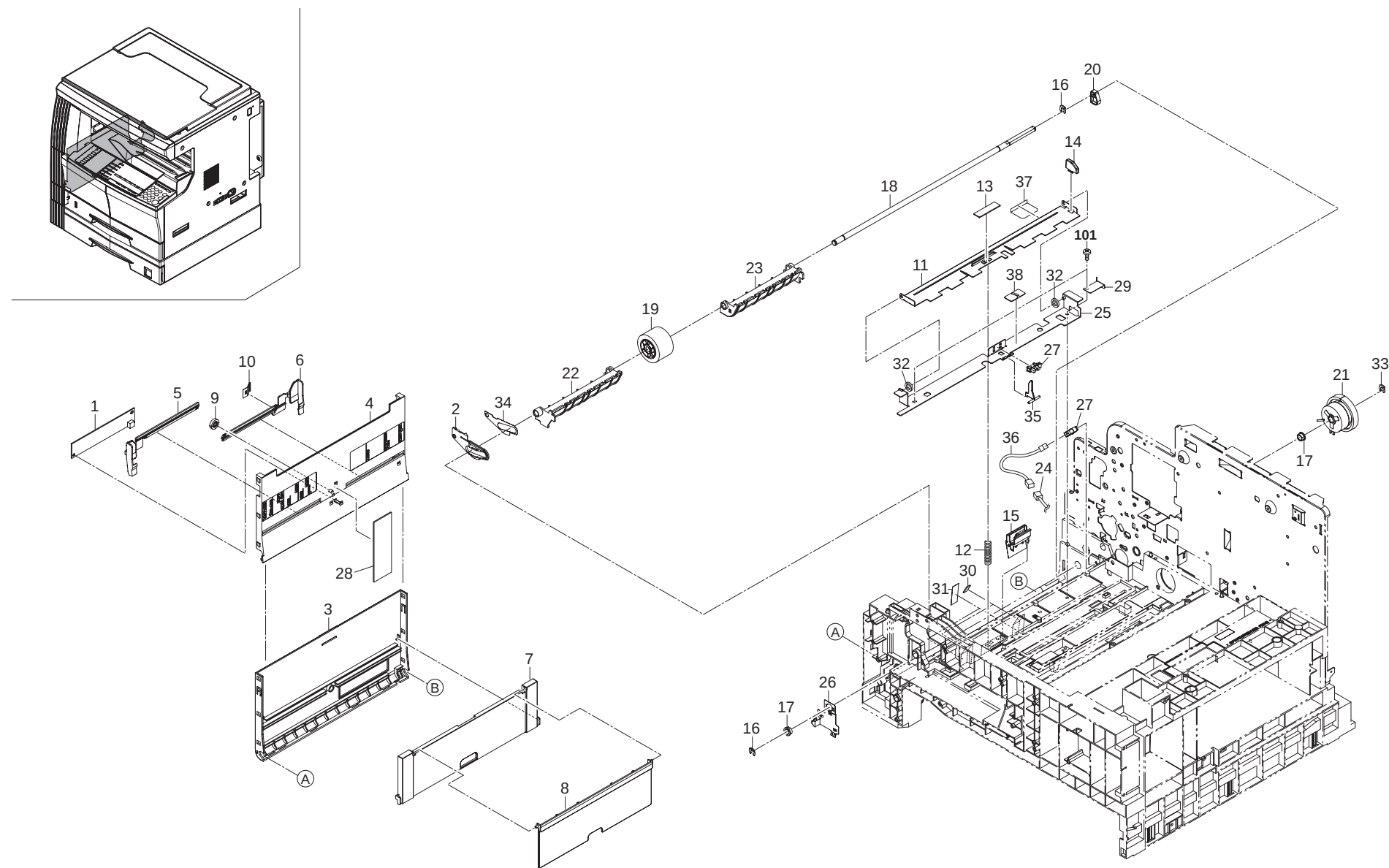
FIG. 8 Bypass Section
