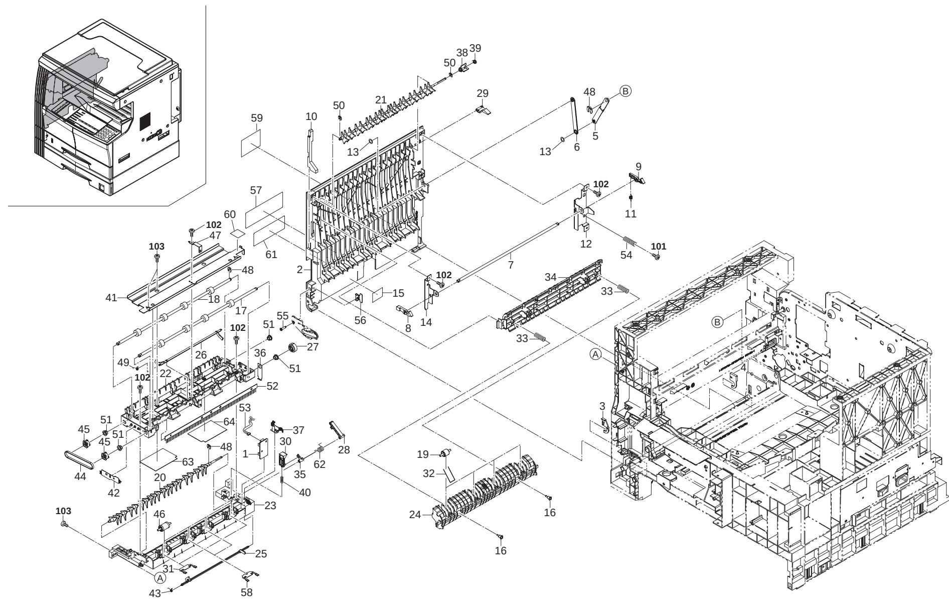
FIG. 9 Exit Section
