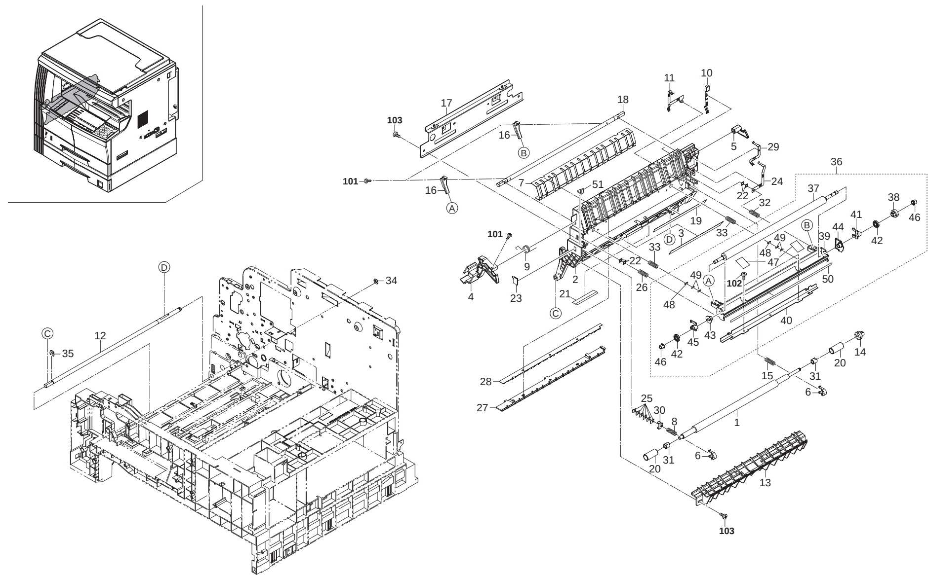
FIG. 6 Conveying Section
