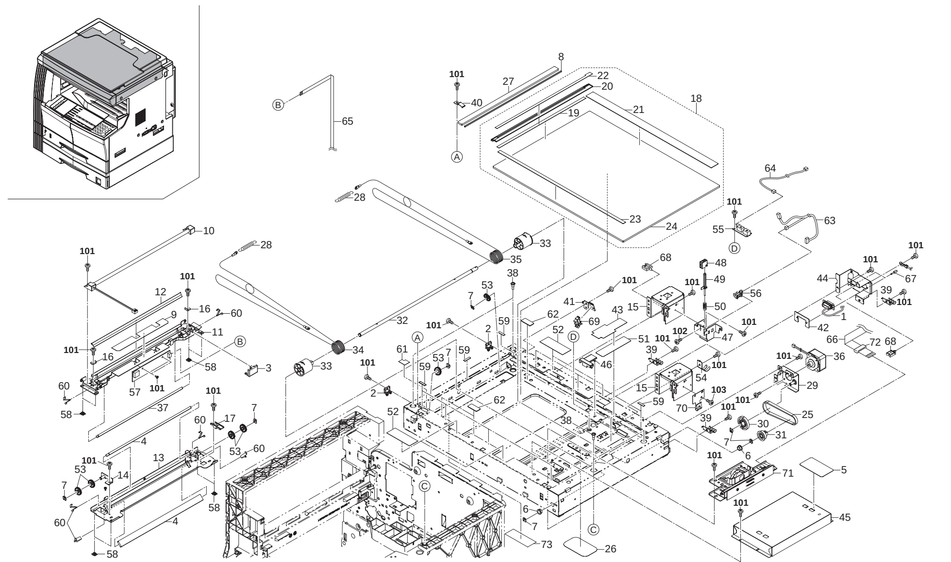
FIG. 10 Scanner Section
