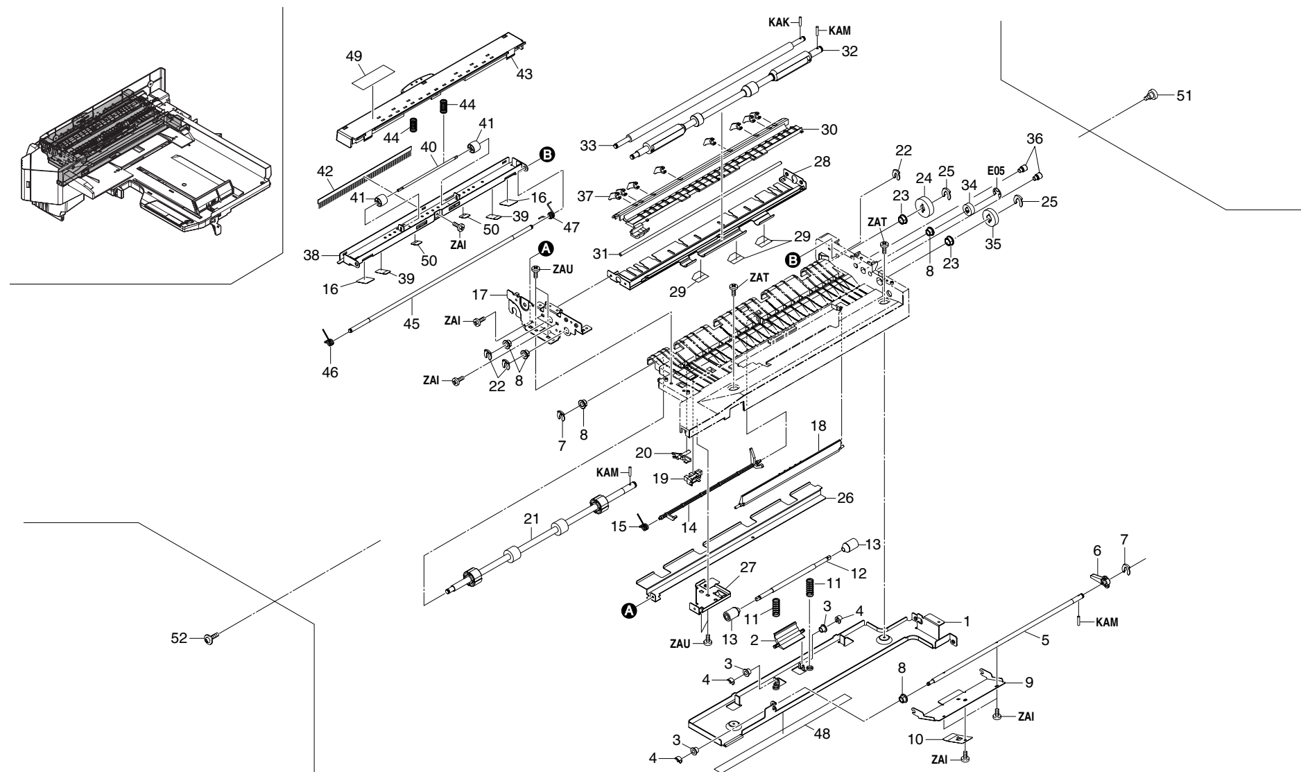
FIG. 1 BASE SECTION
