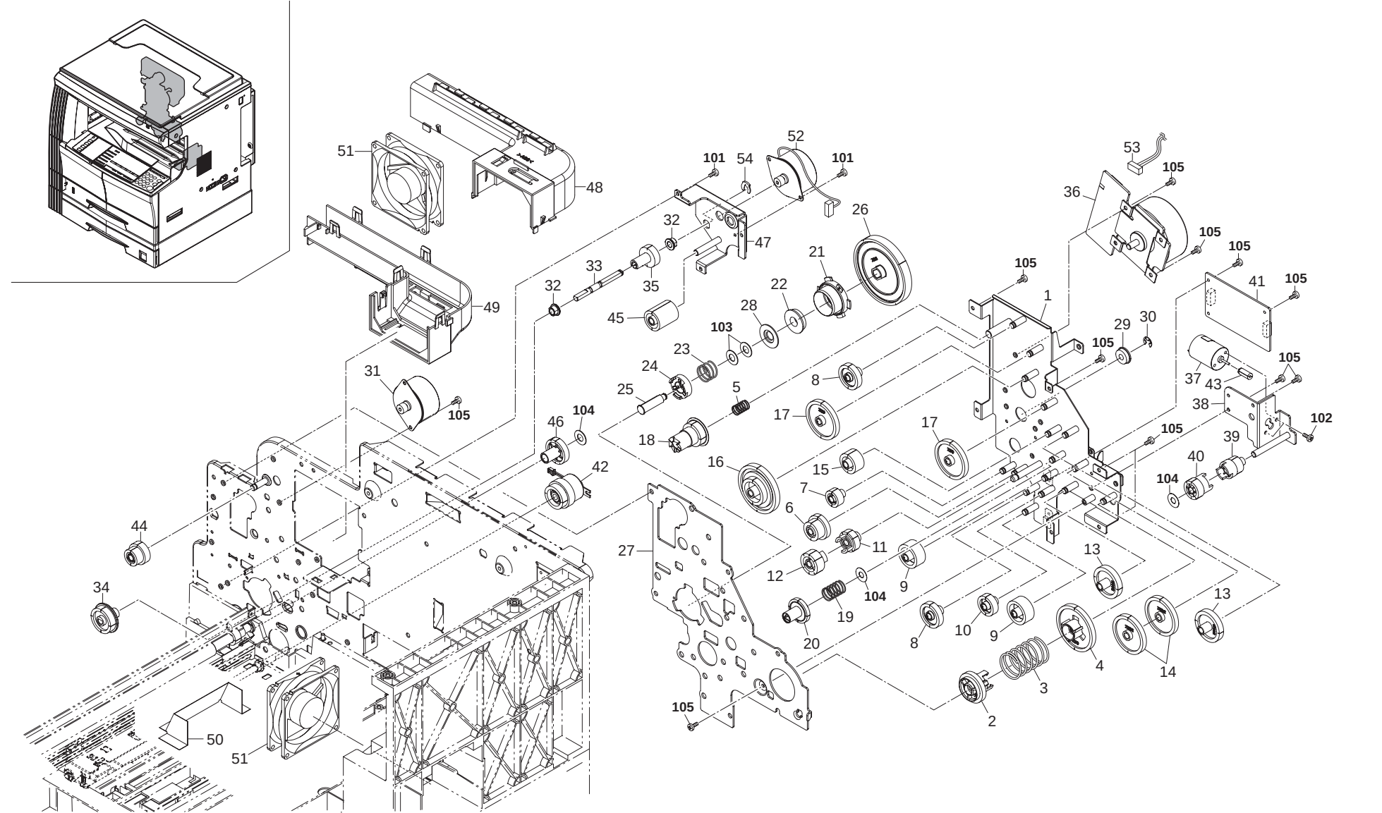
FIG. 13 Driving & Cooling Section
