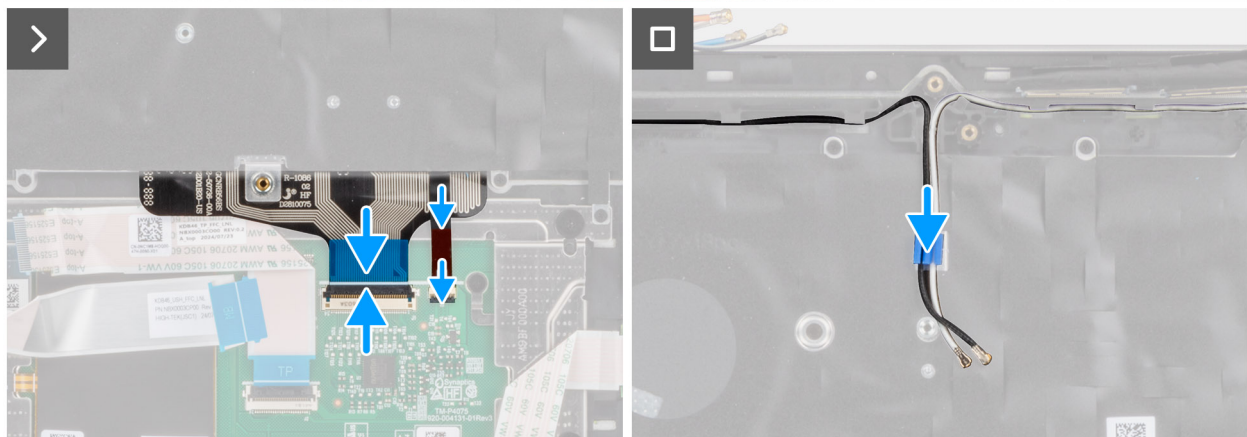
Figure 84. Installing the keyboard
