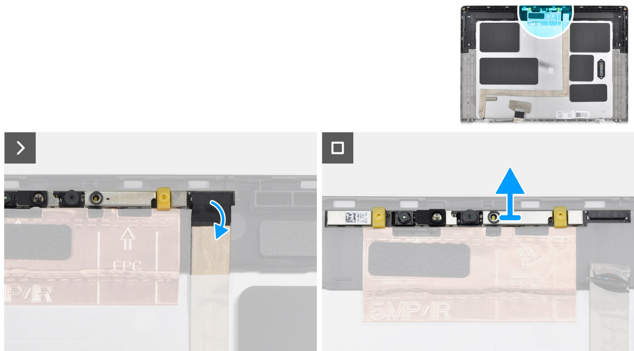
Figure 75. Removing the RGB/IR camera
