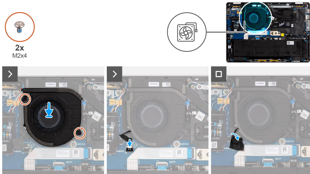
Figure 40. Installing the fan
