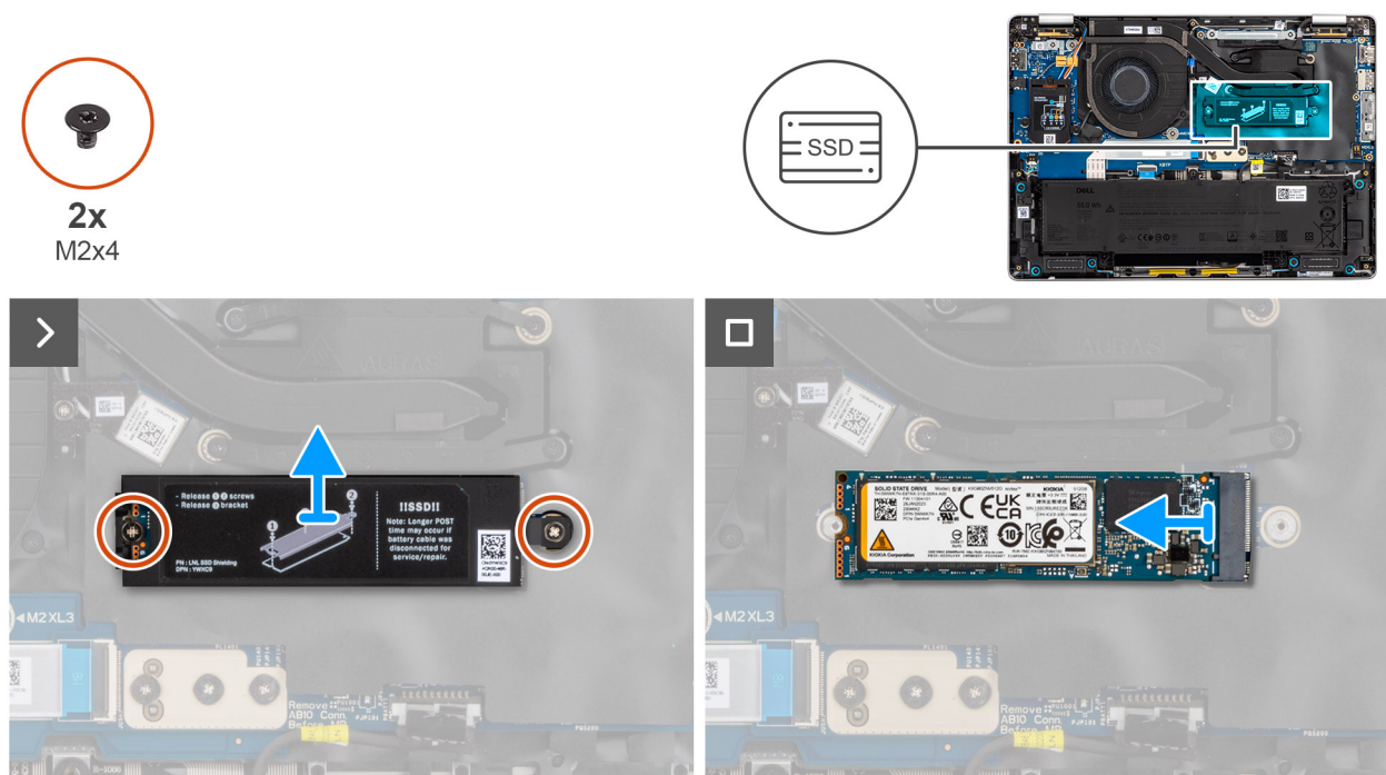
Figure 35. Removing the M.2 2280 SSD
