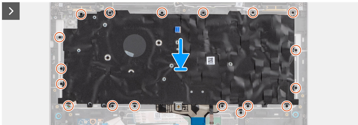
Figure 83. Installing the keyboard
