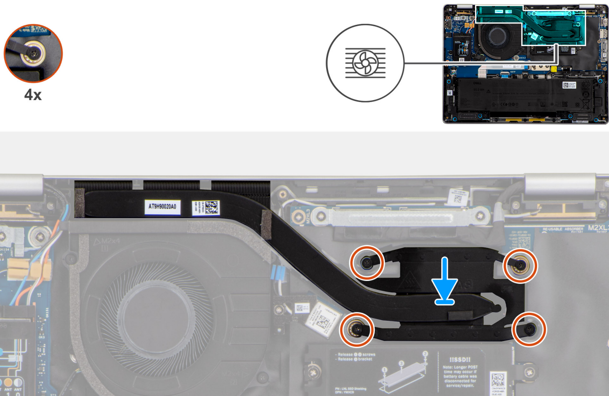
Figure 42. Installing the heat-sink
