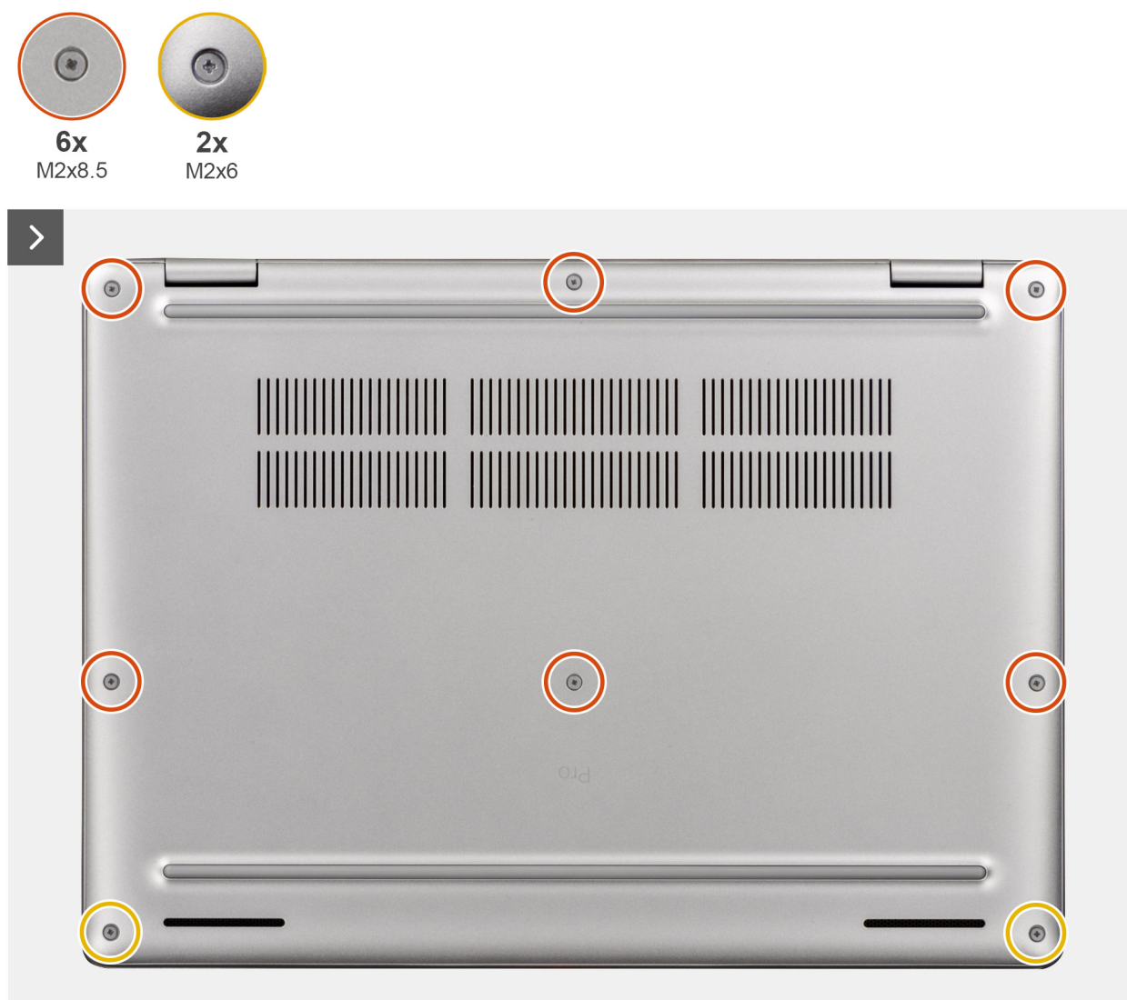
Figure 22. Removing the base cover
