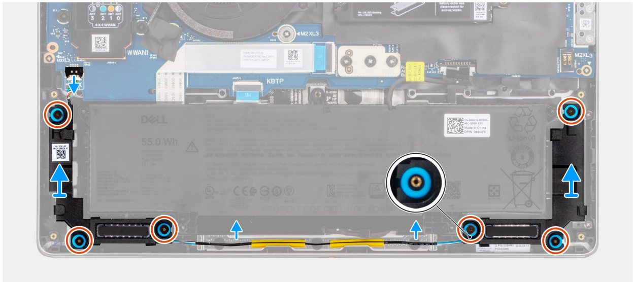
Figure 37. Removing the speakers
