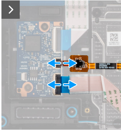
Figure 43. Removing the USH board
