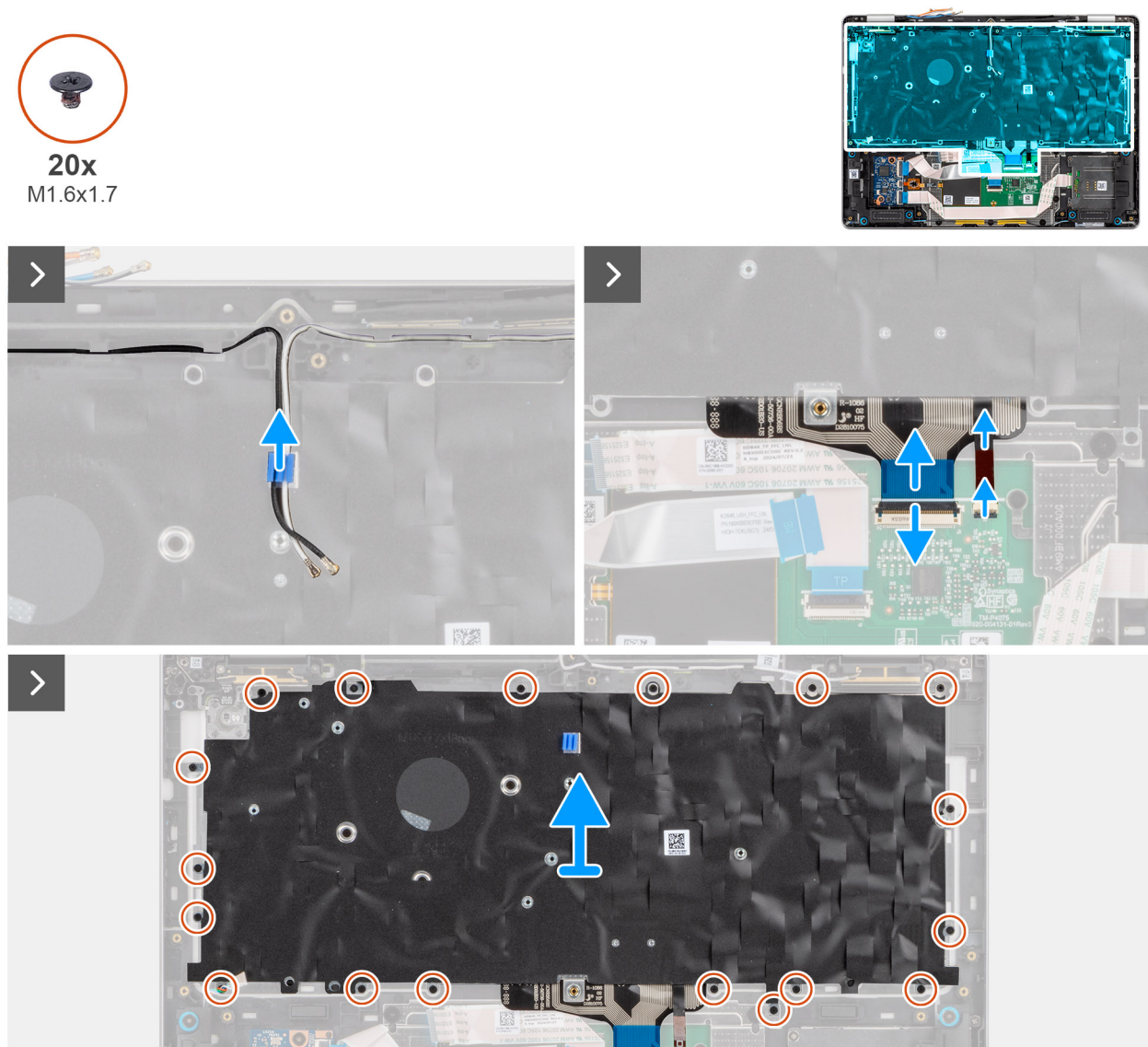
Figure 81. Removing the keyboard
