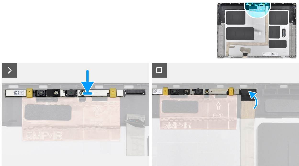
Figure 76. Installing the RGB/IR camera
