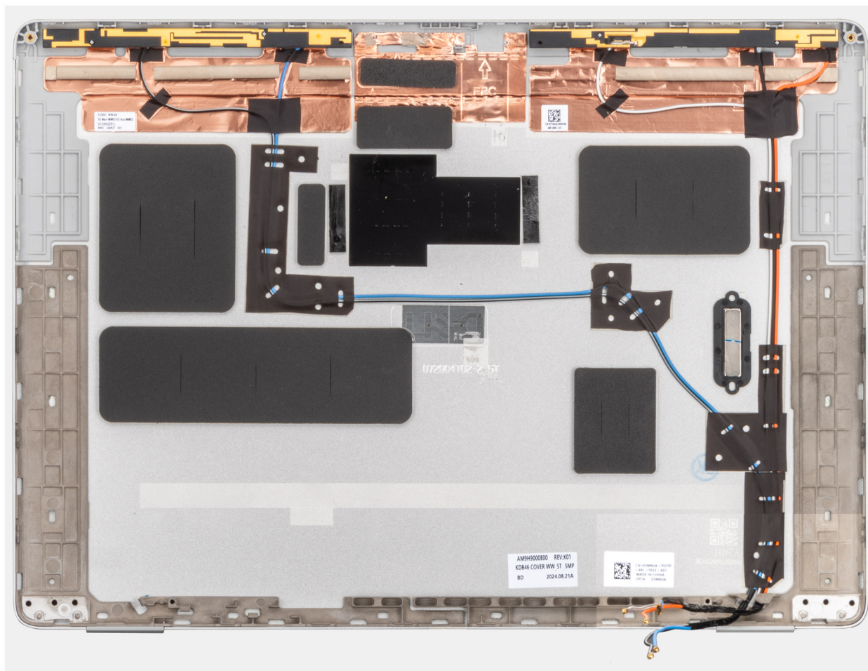
Figure 80. Display back-cover and antenna assembly
