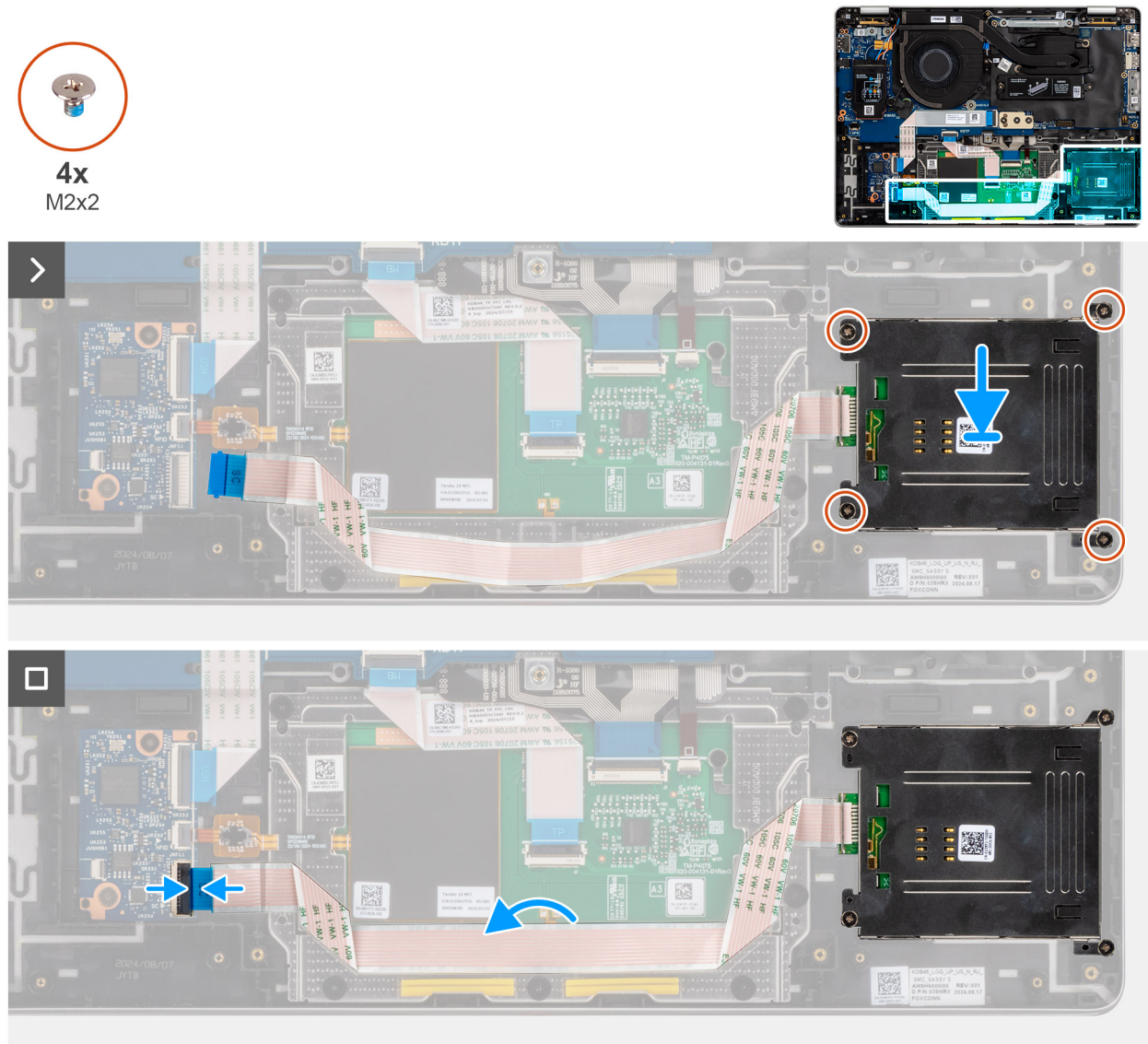
Figure 46. Installing the smart card reader
