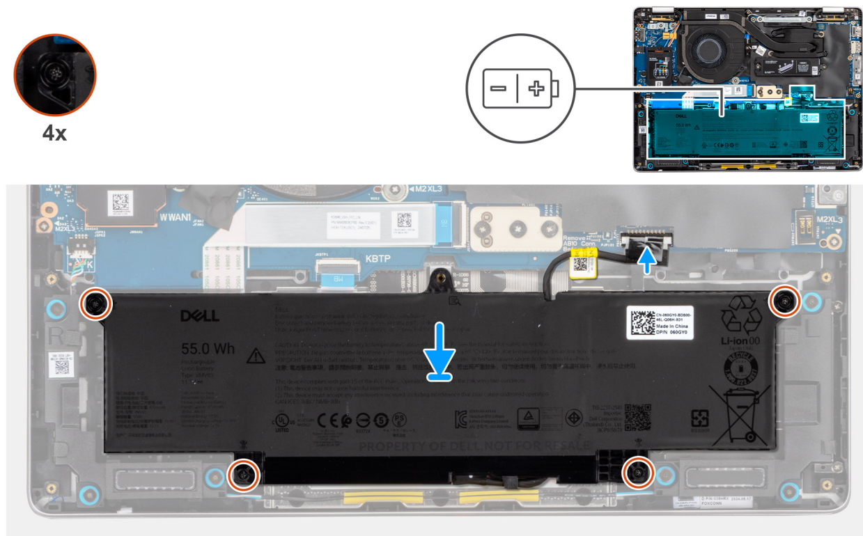
Figure 28. Installing the battery
