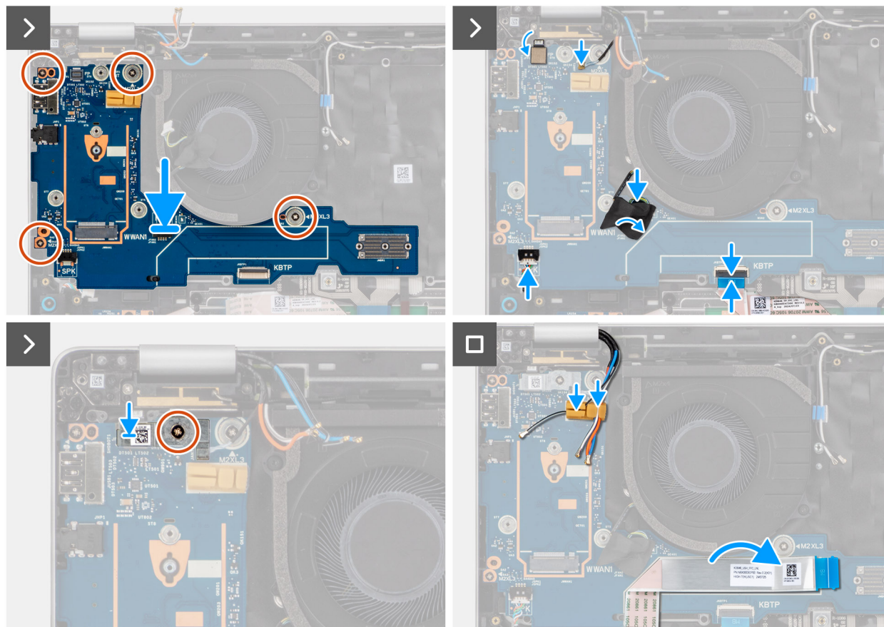
Figure 54. Installing the I/O board
