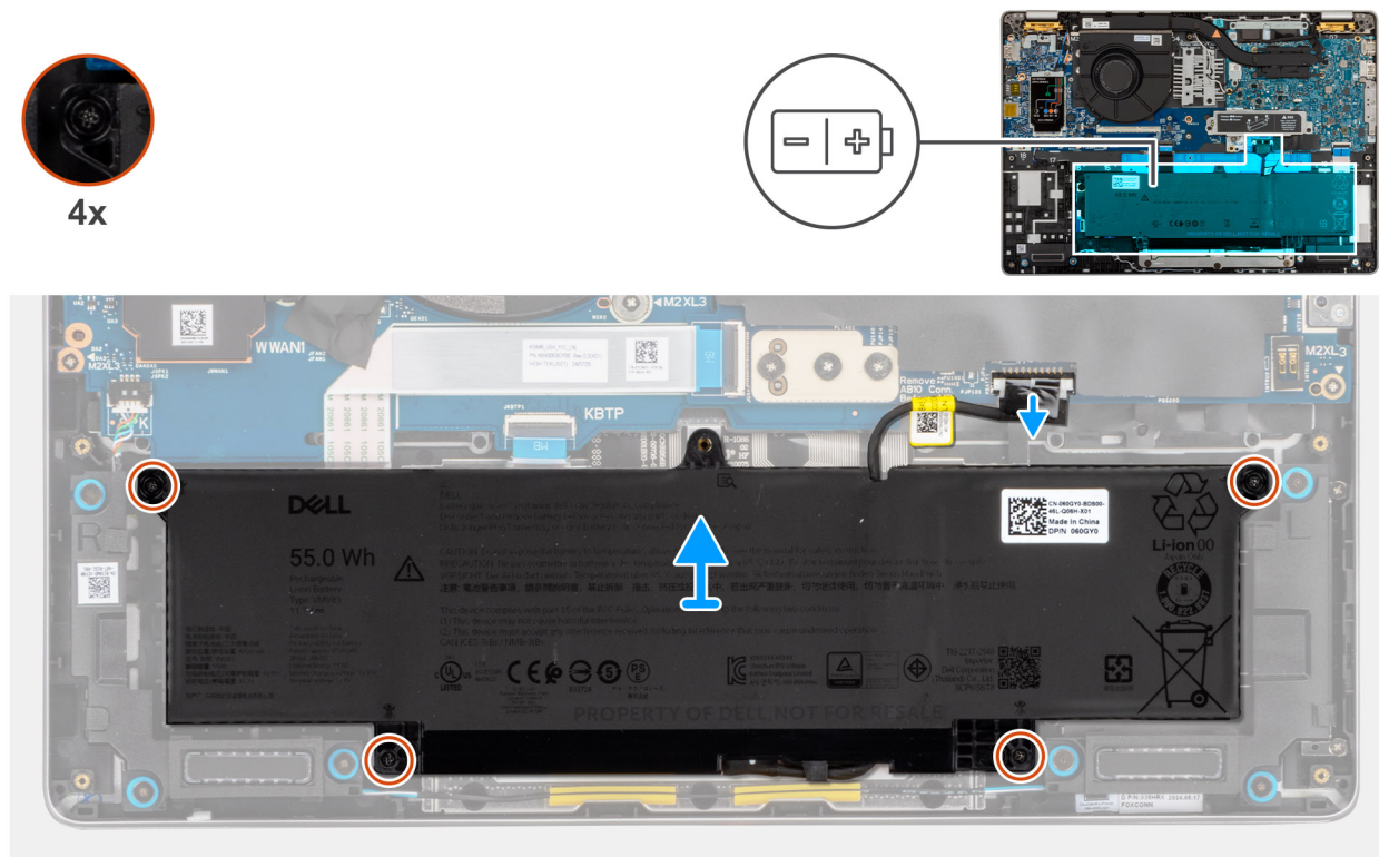
Figure 27. Removing the battery
