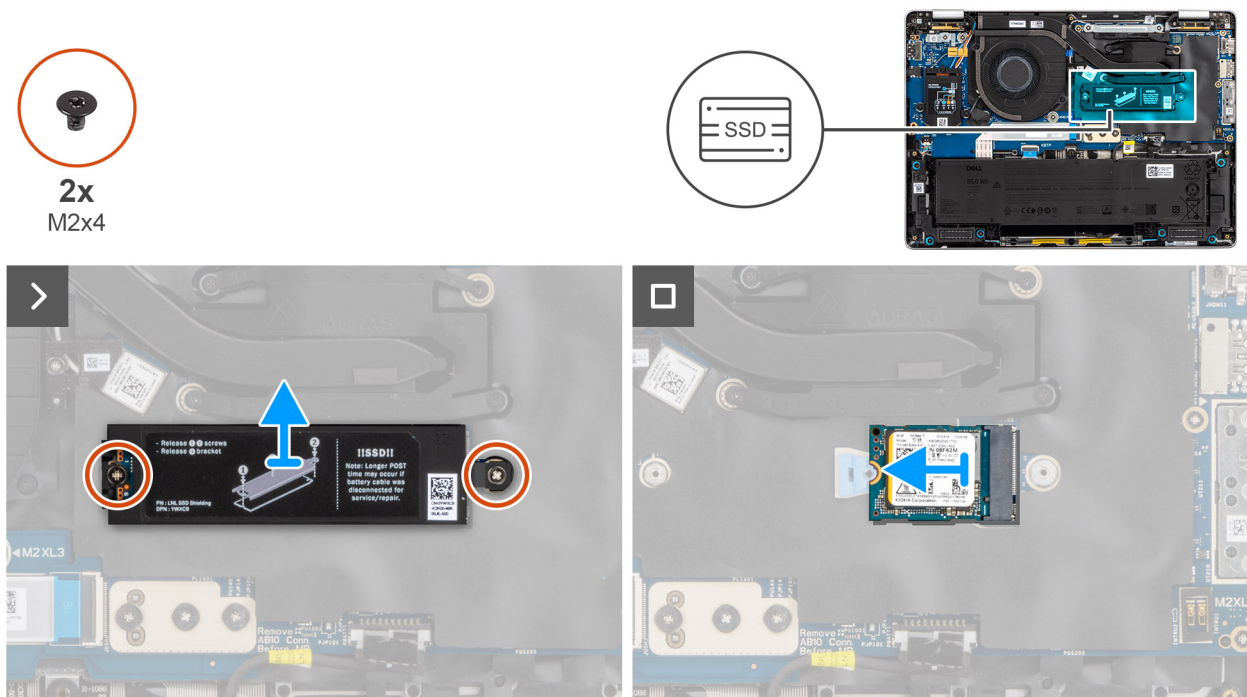
Figure 33. Removing the M.2 2230 SSD
