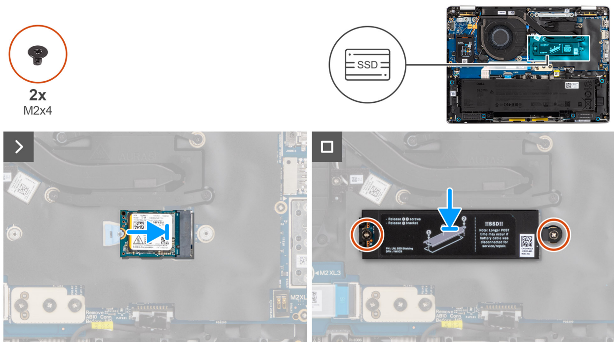
Figure 34. Installing the M.2 2230 SSD
