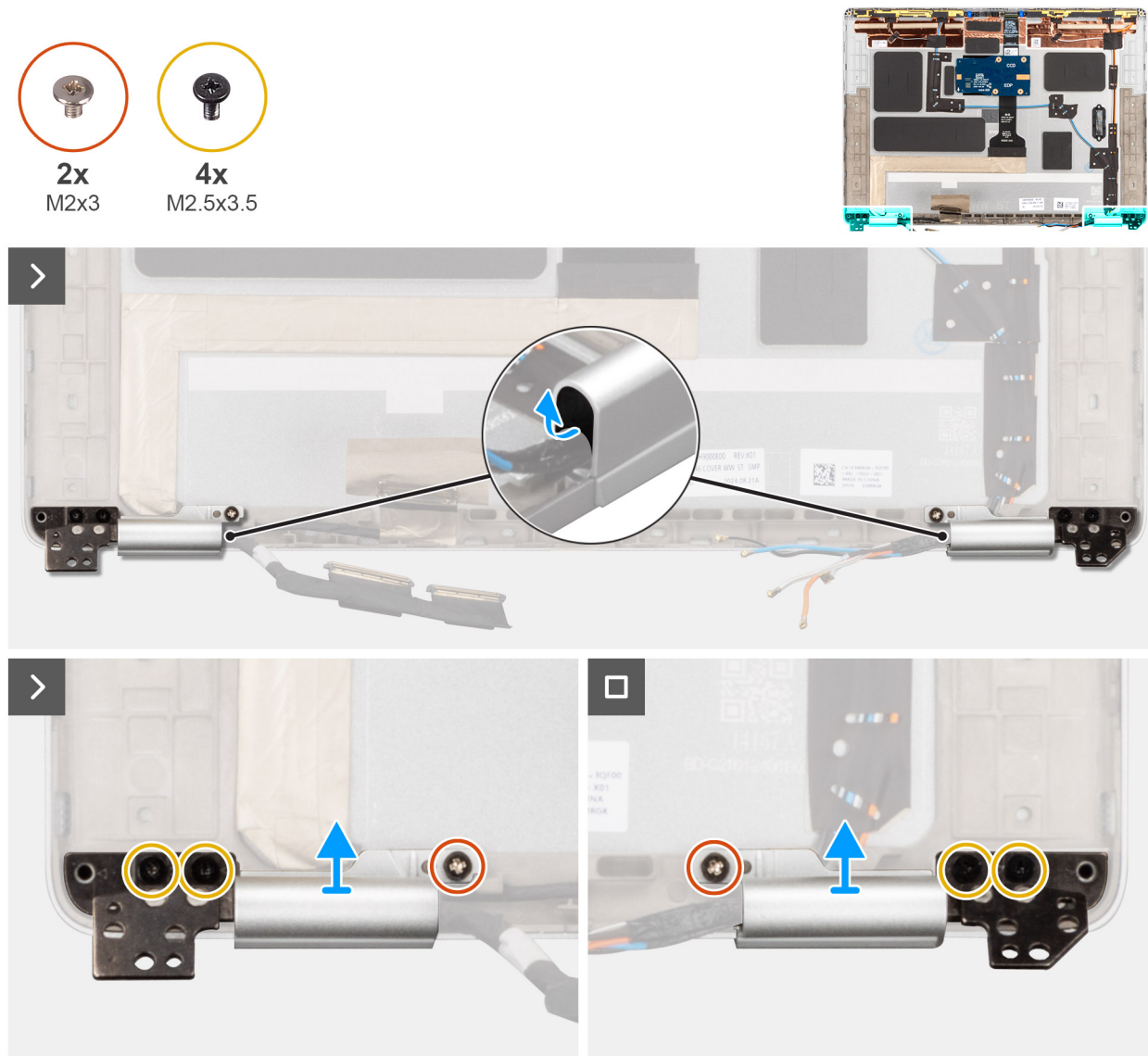
Figure 73. Removing the display hinge caps
