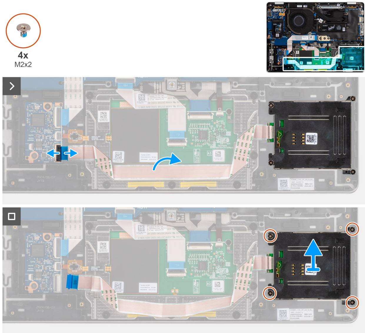
Figure 45. Removing the smart card reader
