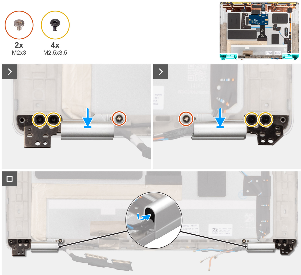
Figure 74. Installing the display hinge caps
