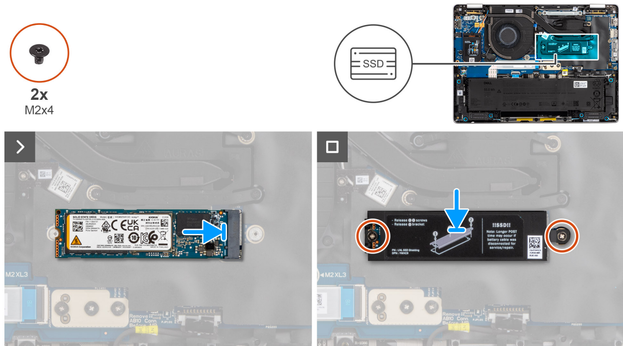
Figure 36. Installing the M.2 2280 SSD
