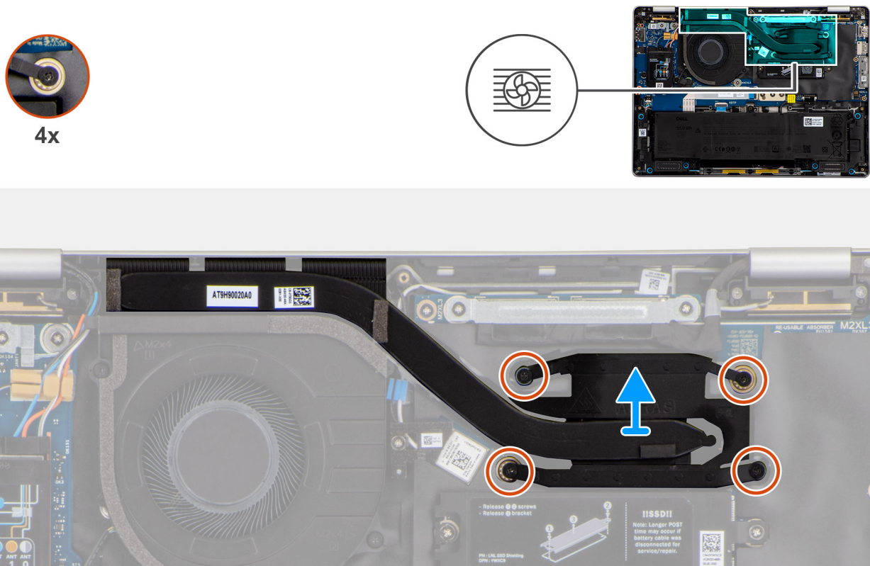
Figure 41. Removing the heat-sink
