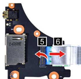
Figure 22. Separate the USB board cable from the USB board
