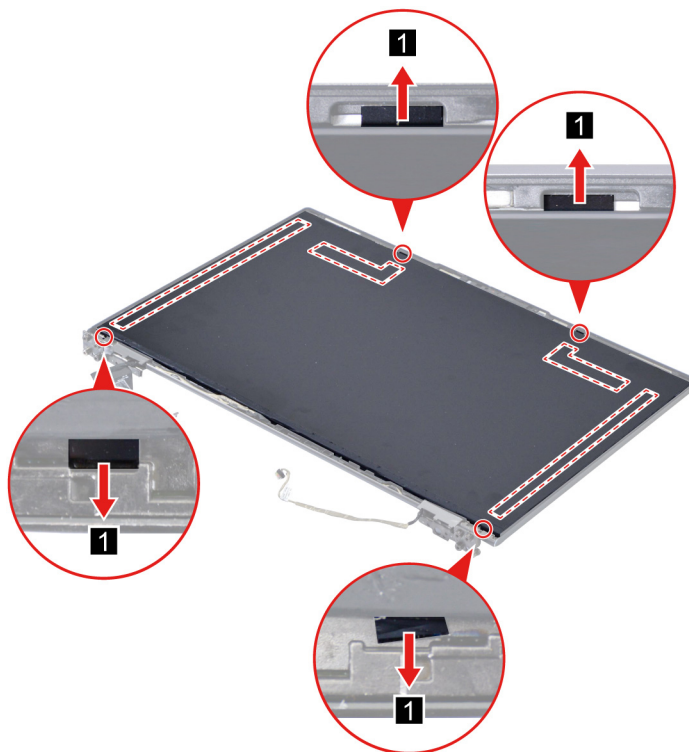
Figure 44. Remove the four pieces of removable tape with tweezers
