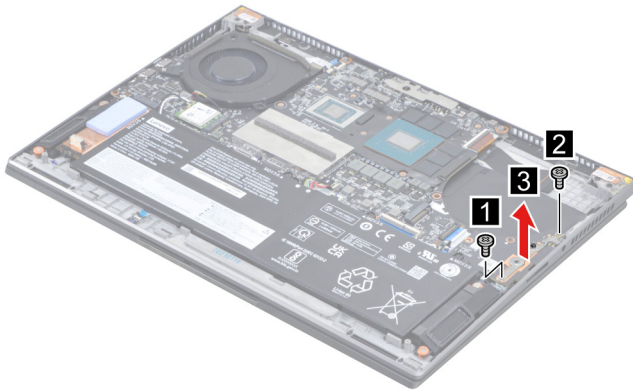
Figure 19. Remove the SSD bracket
