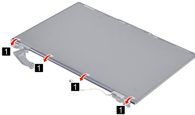
Figure 43. Remove the hinge cover
