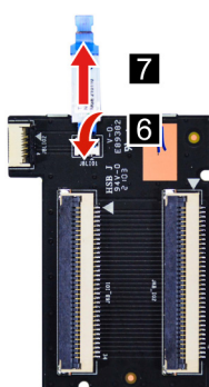
Figure 35. Separate the keyboard backlight cable from the connector board
