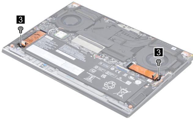
Figure 7. Remove two screws
