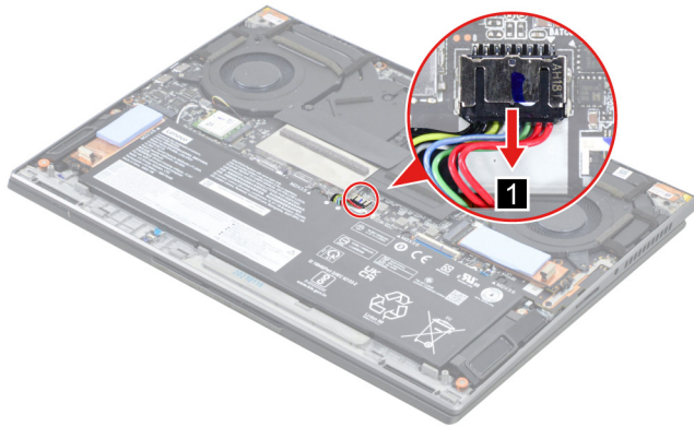
Figure 5. Disconnect the battery pack cable.
