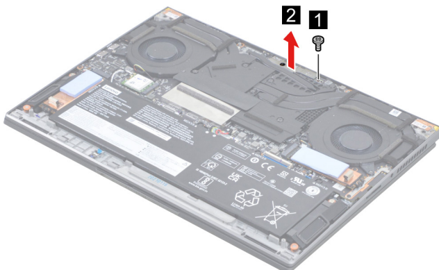
Figure 13. Remove the DC-in bracket.
