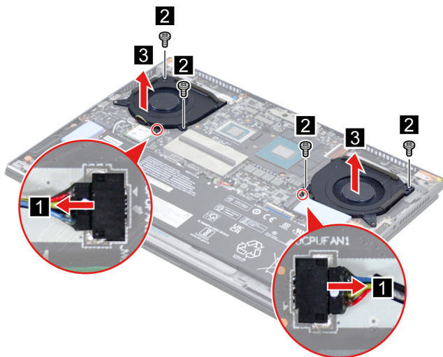
Figure 18. Remove the fans
