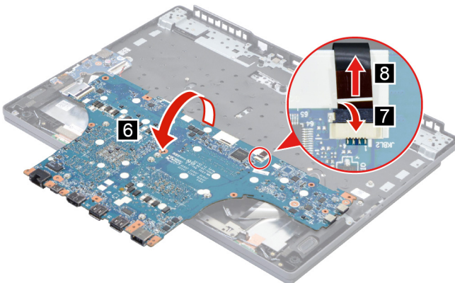
Figure 25. Remove the system board with the I/O board cable
