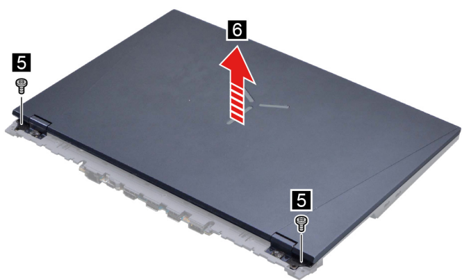
Figure 31. Lift the LCD module
