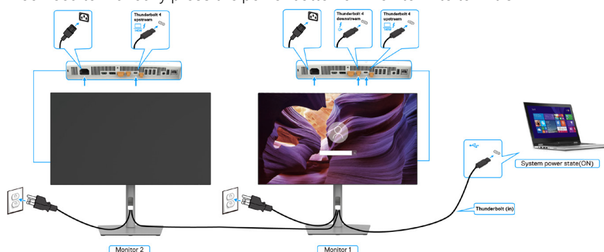
Figure 52. Connecting the monitor for Thunderbolt 4 daisy chain function-on
