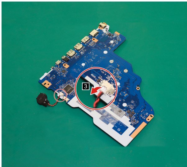
Figure 24. Remove the backup battery
