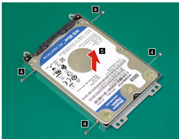
Figure 7. Remove the screws and detach the HDD bracket
