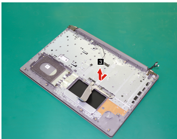
Figure 29. Remove the upper case
