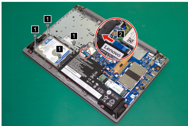
Figure 5. Remove the screws and detach the HDD board connector
