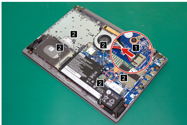
Figure 8. Detach the battery pack connector and remove the screws
