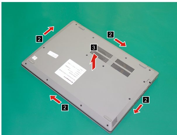
Figure 4. Remove the base cover
