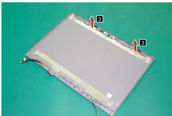
Figure 43. Remove the antenna assembly
