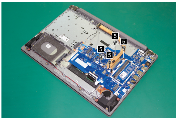
Figure 18. Remove the screws
