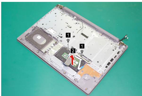
Figure 26. Remove the screws and detach the touchpad
