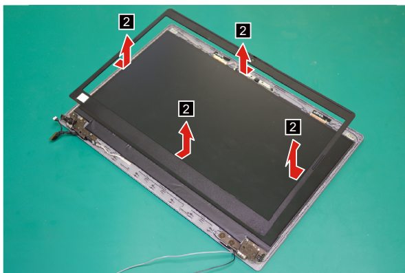
Figure 31. Remove the LCD front bezel
