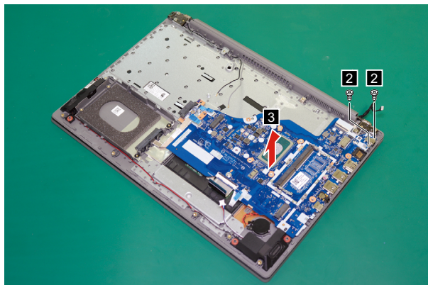
Figure 22. Remove the screws and system board
