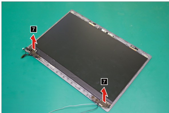
Figure 38. Remove the LCD hinges
