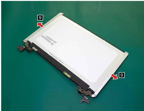
Figure 40. Remove the hinge modules
