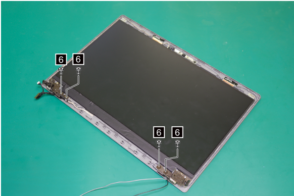
Figure 33. Remove the screws
