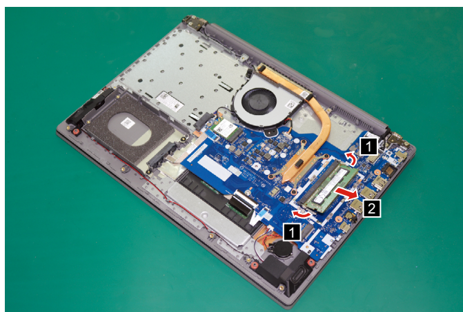
Figure 12. Release the latches and unplug the DIMM
