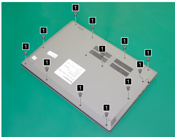
Figure 3. Remove the screws
