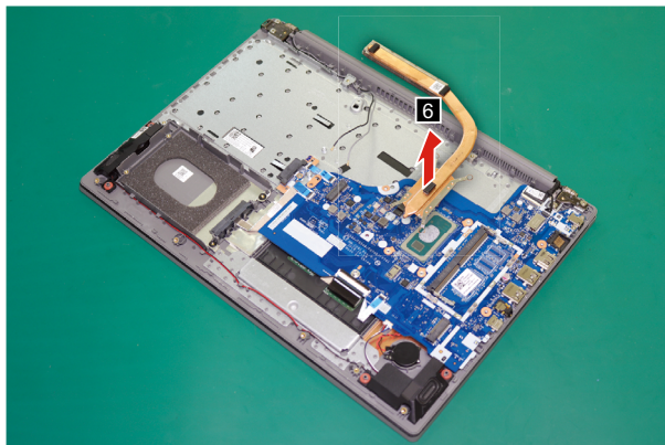
Figure 19. Remove the heat sink
