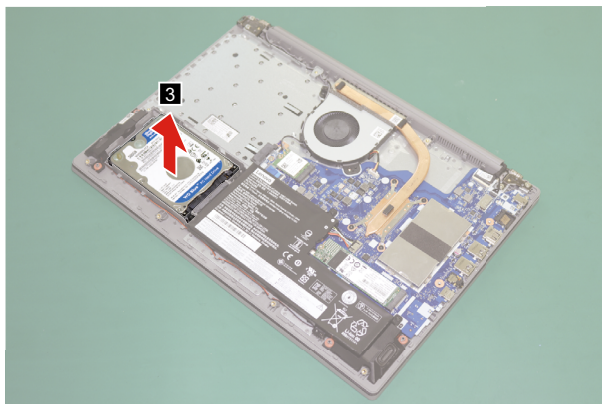
Figure 6. Remove the hard disk drive
