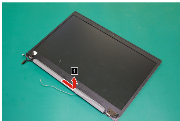
Figure 30. Remove the hinge cap
