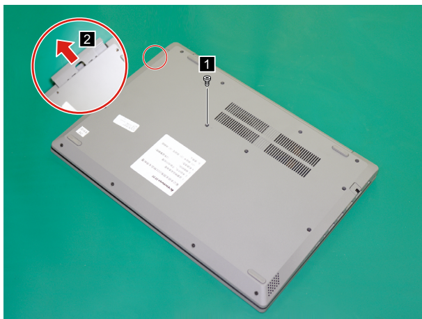
Figure 1. Remove the optical drive
