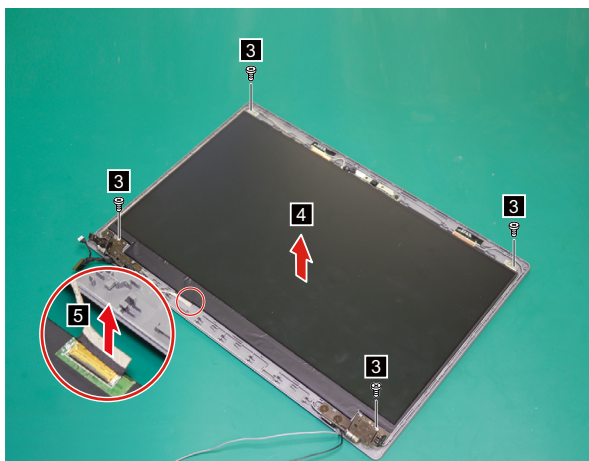
Figure 32. Remove the screws and LCD module connector
