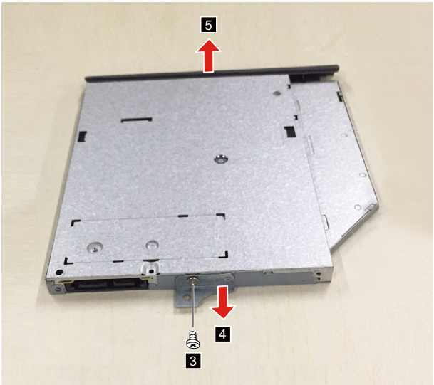
Figure 2. Remove the optical drive bracket and bezel
