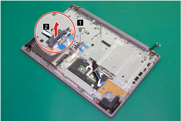
Figure 23. Remove the ODD transfer board
