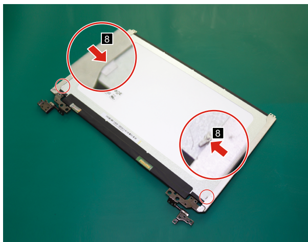
Figure 39. Pull out the adhesive tapes securing the hinge modules
