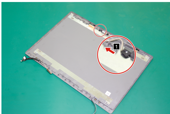
Figure 41. Detach the camera connector
