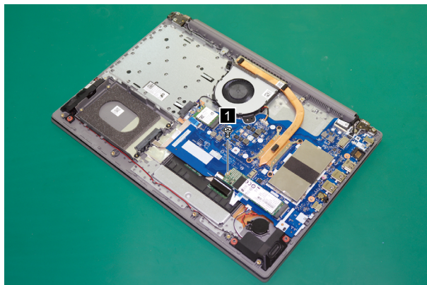
Figure 10. Remove the screw
