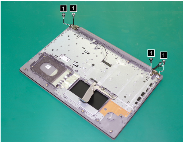
Figure 27. Remove the screws
