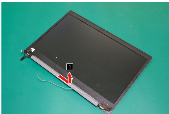
Figure 35. Remove the hinge cap
