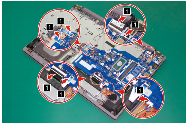
Figure 21. Disconnect the connectors
