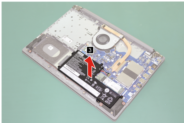
Figure 9. Remove the battery pack
