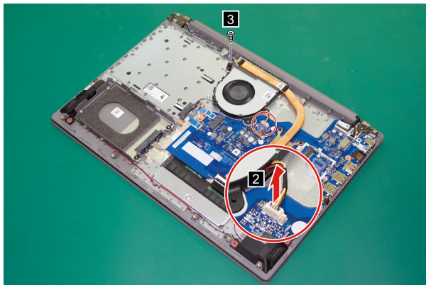
Figure 16. Unplug the fan connector and remove the screw
