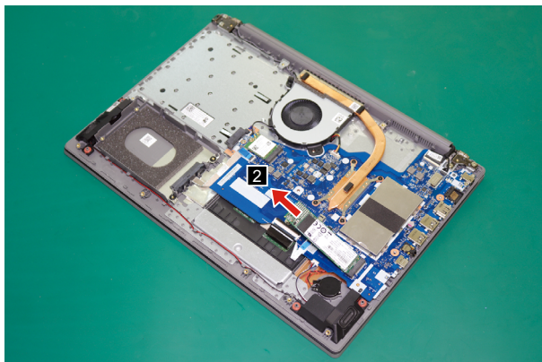
Figure 11. Remove the SSD card
