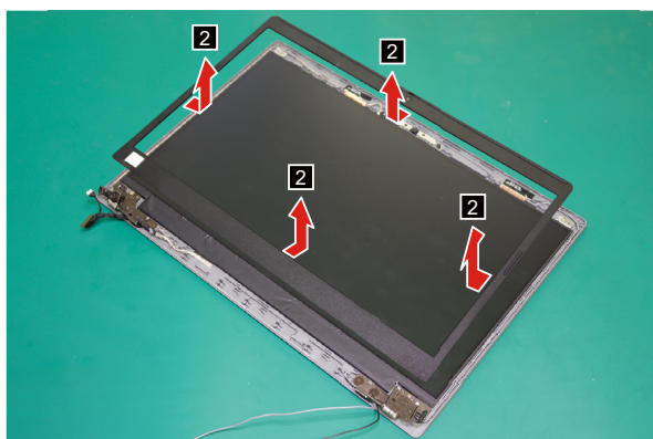
Figure 36. Remove the LCD front bezel
