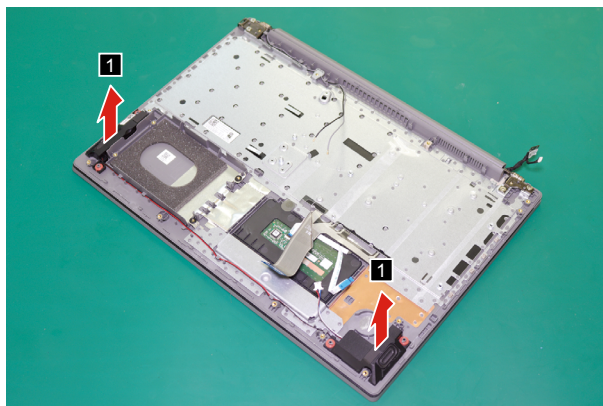
Figure 25. Remove the speakers
