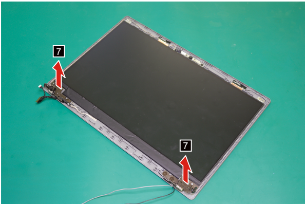
Figure 34. Remove the LCD hinges
