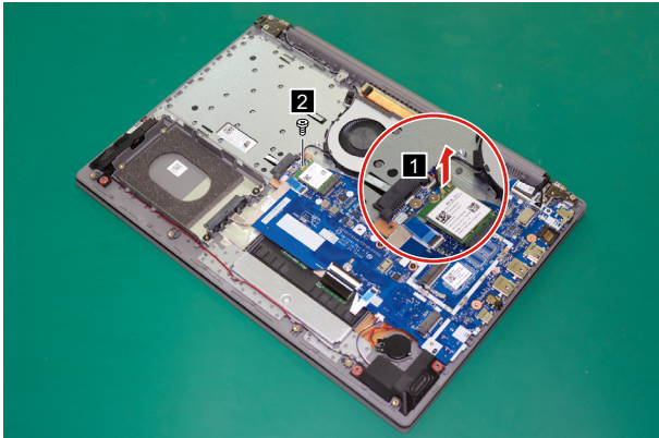
Figure 13. Disconnect the two wireless LAN cables and remove the screw
