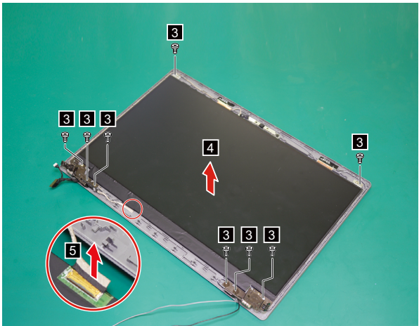
Figure 37. Remove the screws and LCD module connector
