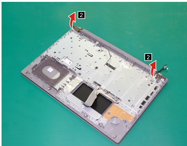
Figure 28. Open the hinge
