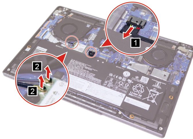
Figure 18. Disconnect cables
