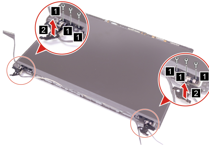
Figure 29. Remove six screws and hinges
