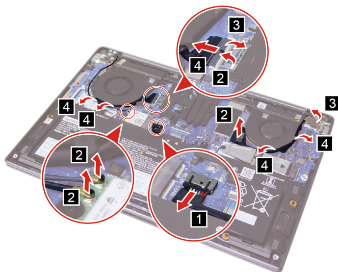
Figure 25. Disconnect cables
