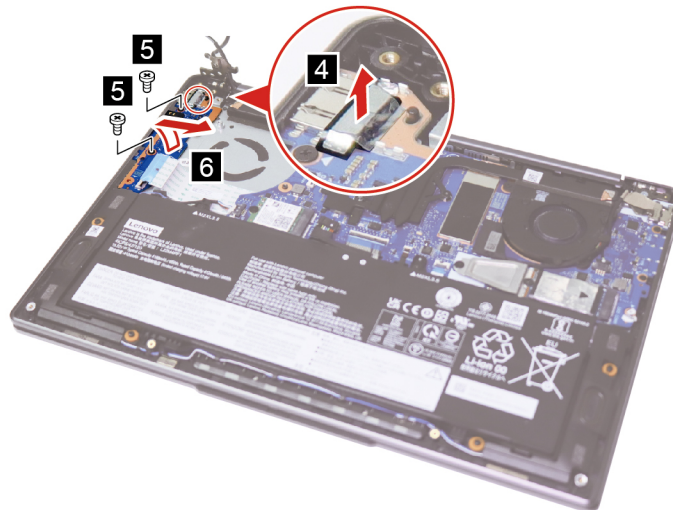
Figure 17. Remove two screws and remove the I/O board
