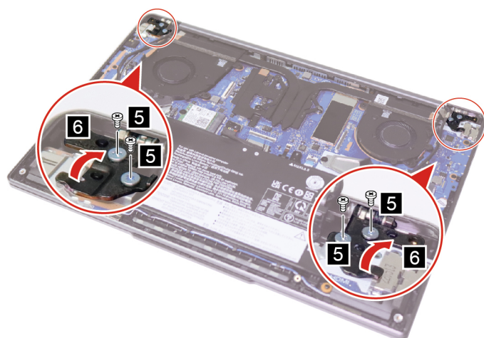
Figure 26. Remove four screws and open two hinges
