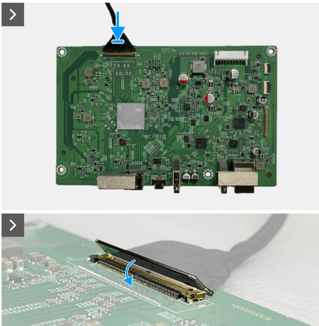
Figure 99. Installation de la carte interface
