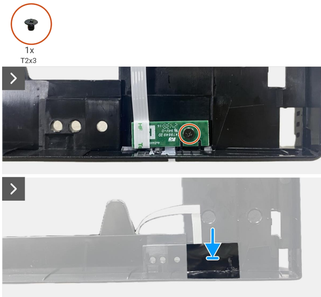
Figure 59. Installation de la carte LED
