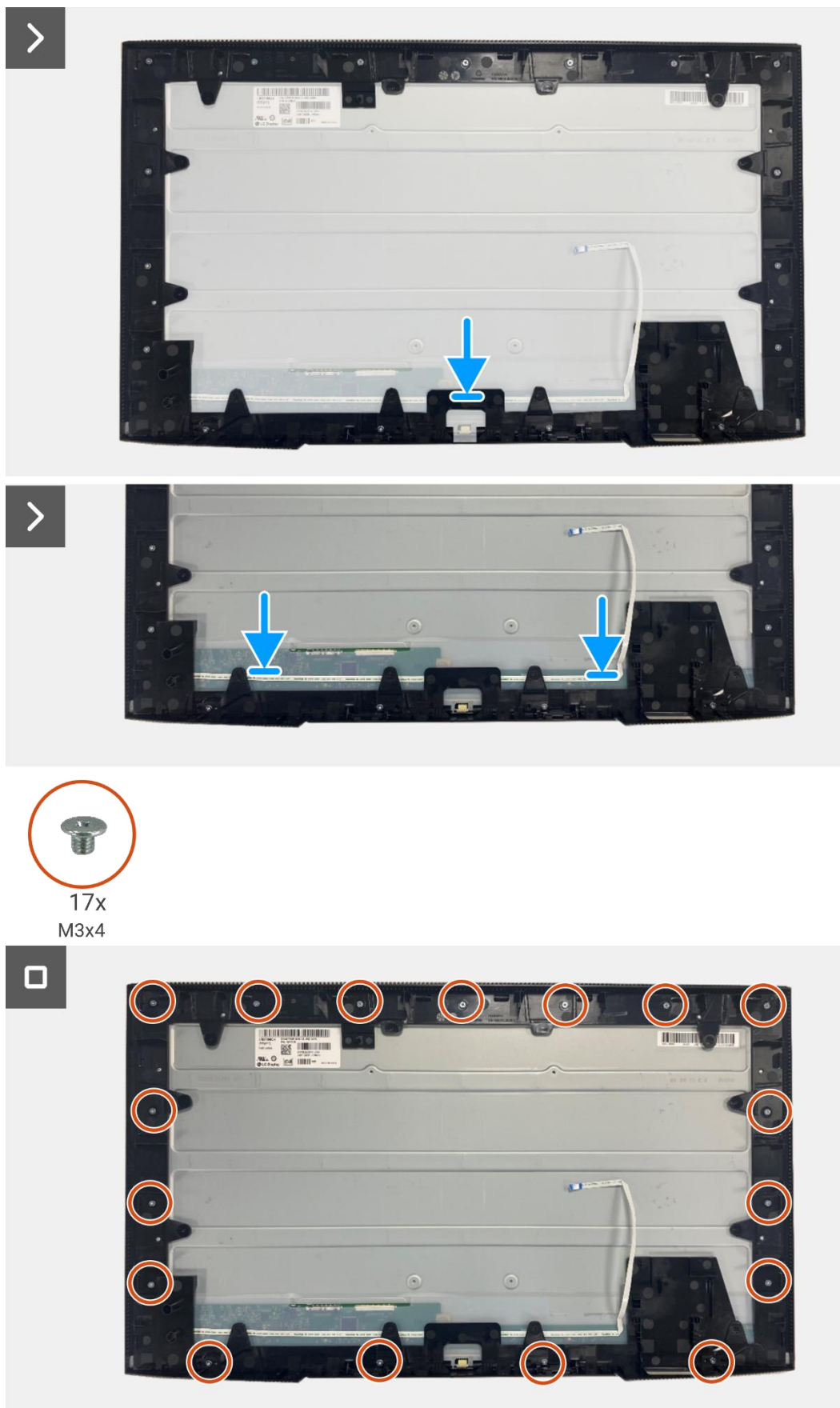
Figure 60. Installation de la carte LED
