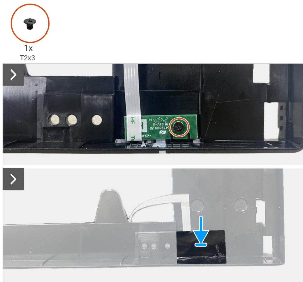
Figure 29. Installation de la carte LED
