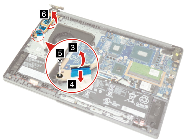
Figure 20. Disconnect the USB board cable, remove one screw and the USB board
