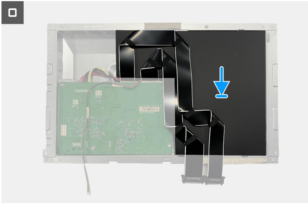
Figure 71. Installation de la carte interface
