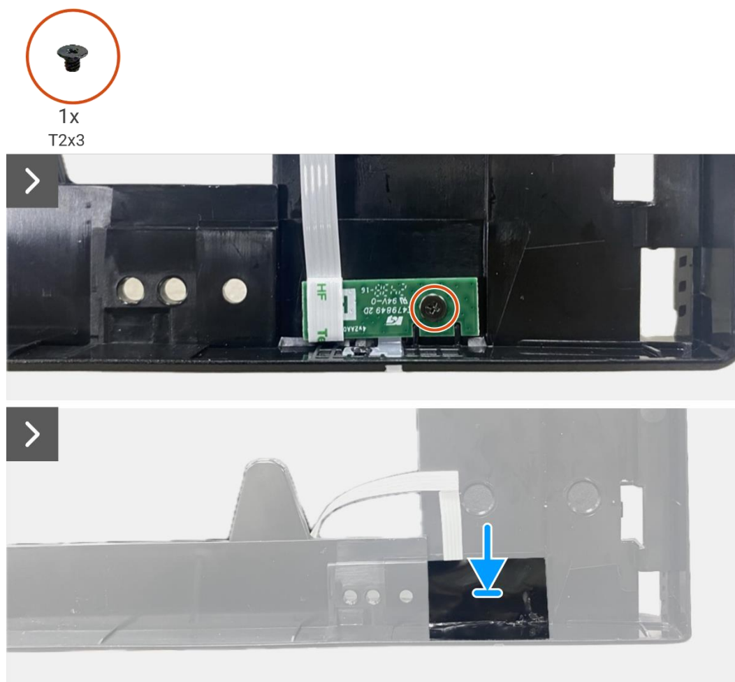
Figure 76. Installation de la carte LED
