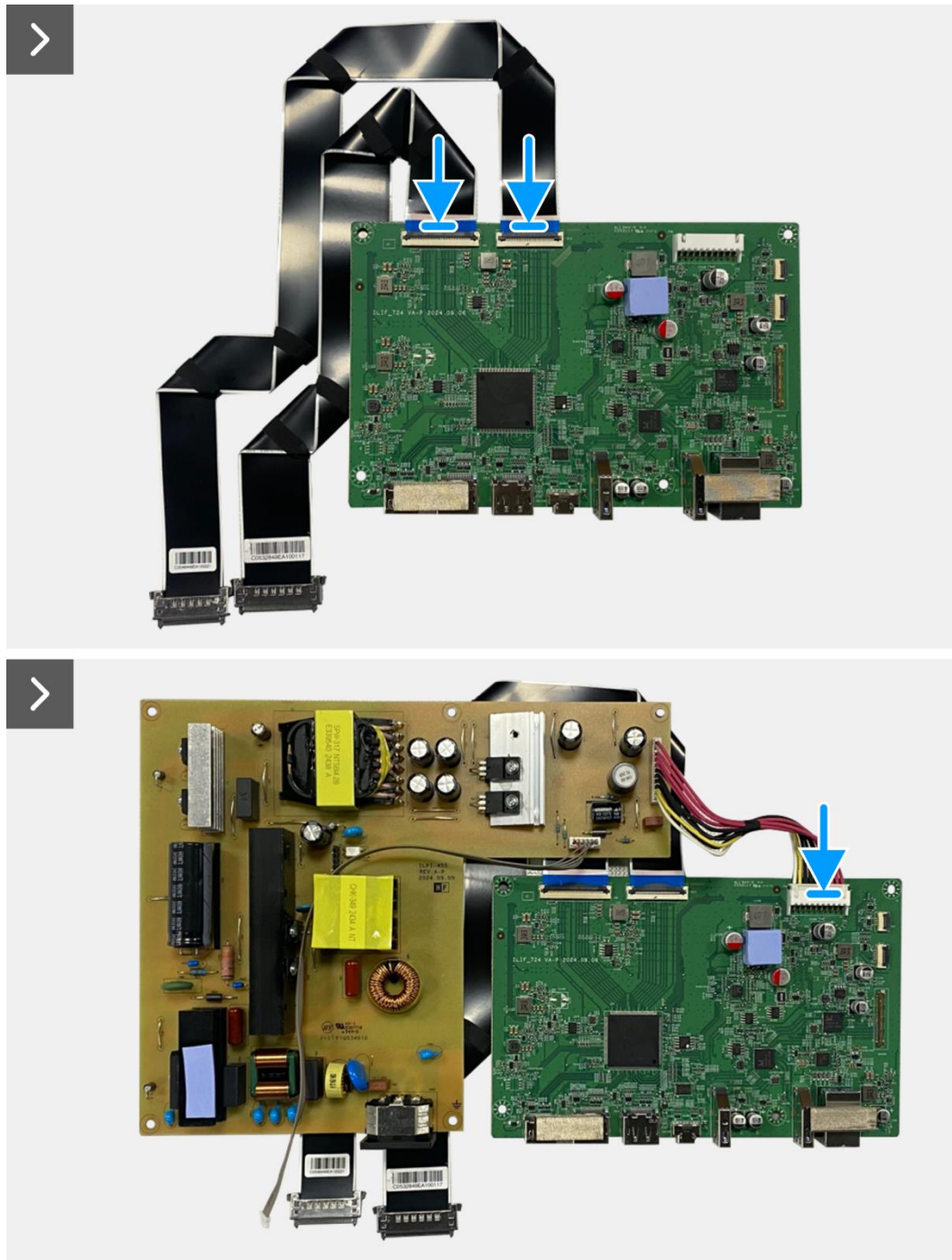
Figure 69. Installation de la carte interface
