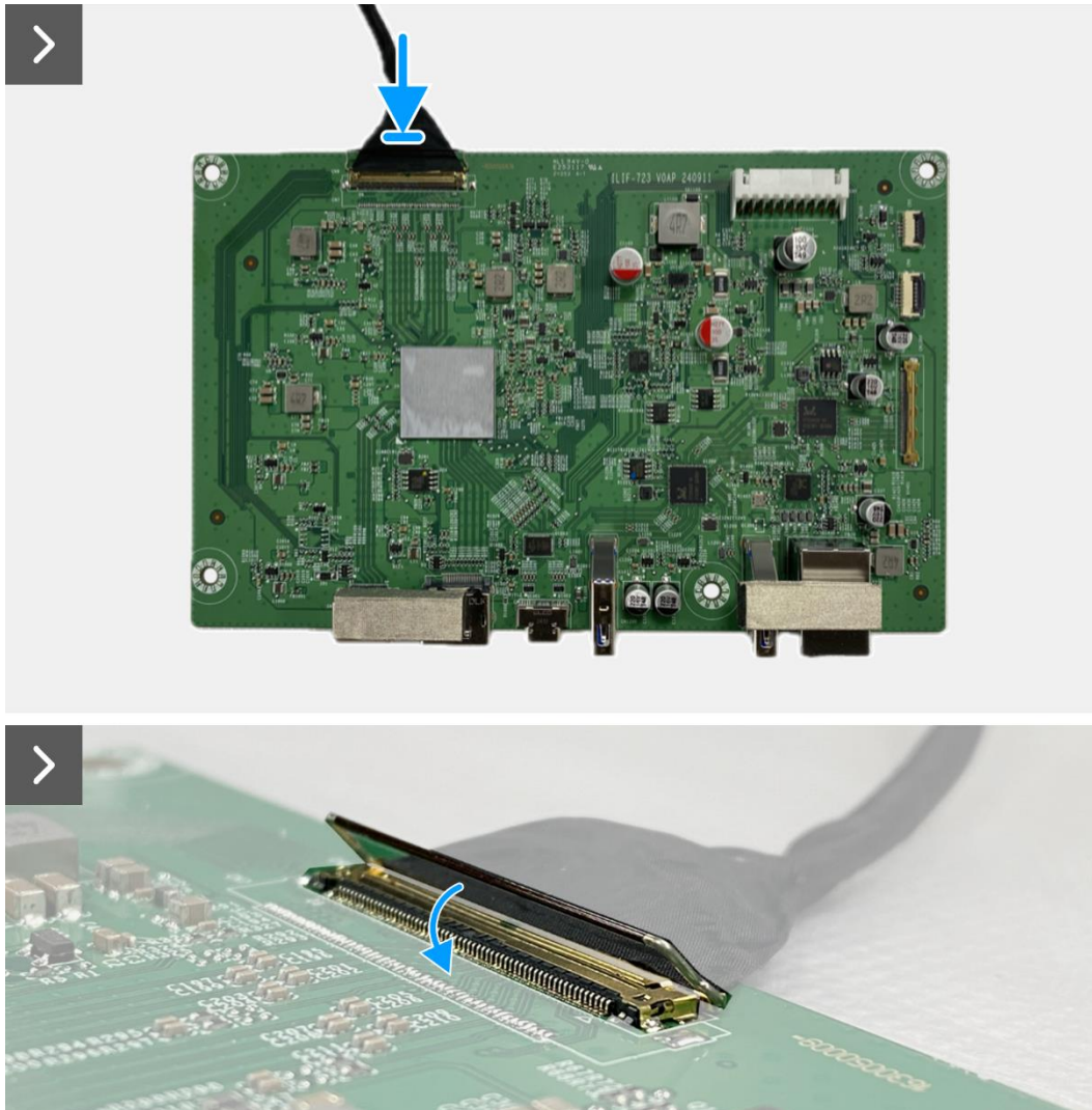
Figure 99. Installation de la carte interface
