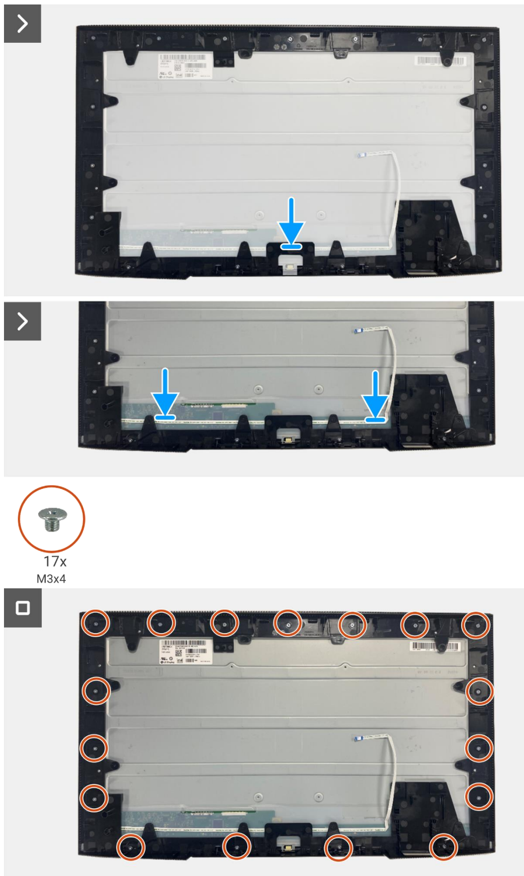
Figure 47. Installation de la carte LED
