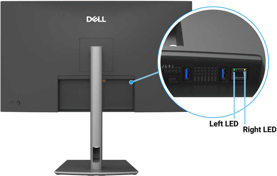
Figura 12. Color de LED RJ45
