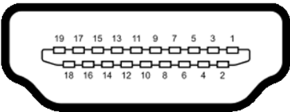
Figura 7. Puerto HDMI
