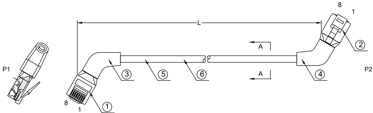
PIN OUT
