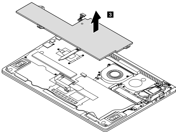
Figure 2. Removal steps of battery pack (continued)
