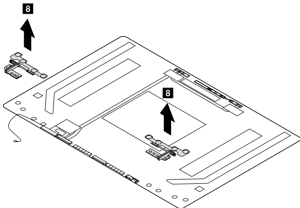
Figure 10. Removal steps of LCD unit and LCD cable (continued)
