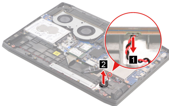
Figure 20. Remove the RTC battery
