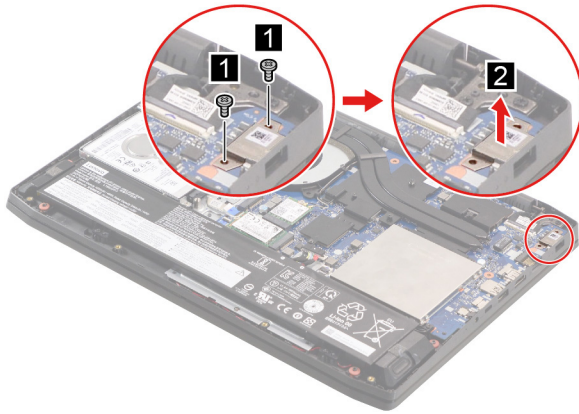
Figure 21. Remove two screws and then remove the DC-in bracket
