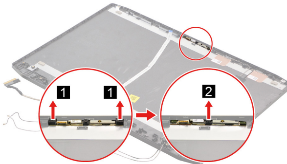
Figure 33. Remove the microphone rubber and then remove the camera
