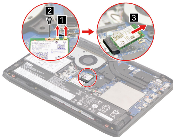
Figure 8. Remove the Wi-Fi card
