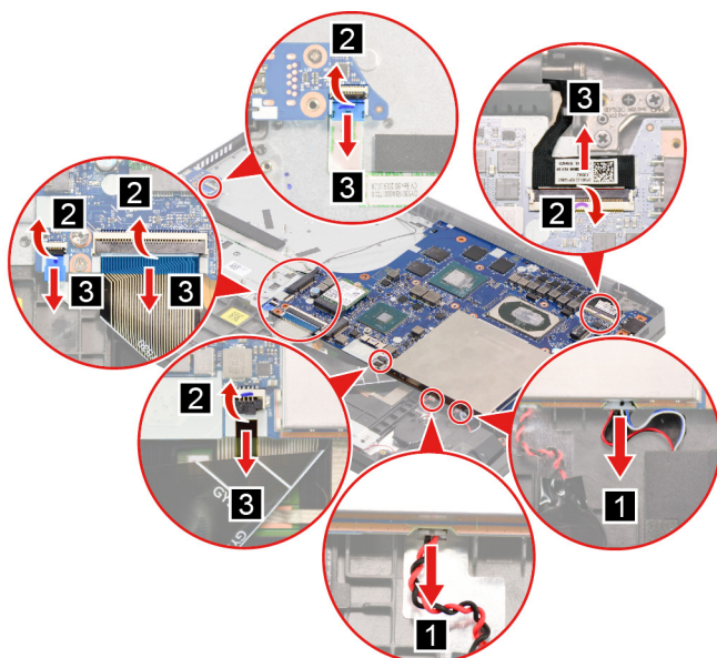
Figure 22. Disconnect cables connected to the system board
