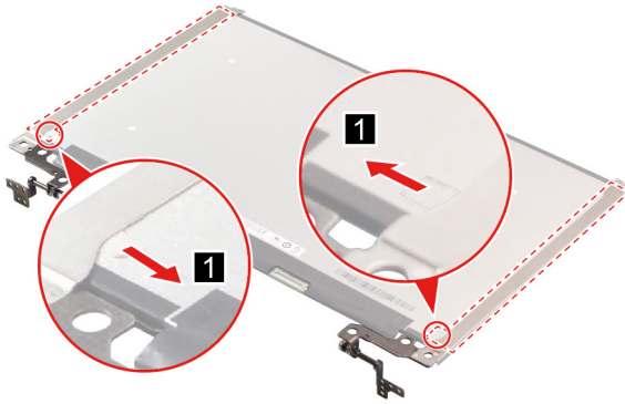
Figure 34. Pull out the removable tape with tweezers
