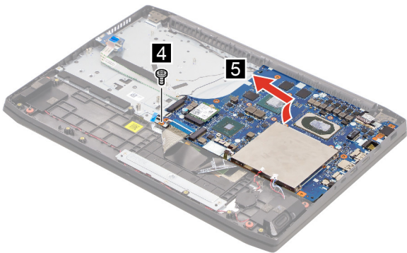
Figure 23. Remove one screw and then remove the system board
