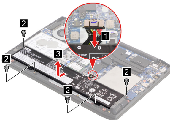
Figure 5. Remove the battery pack
