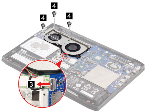
Figure 16. Disconnect the fan cable from the system board and then remove three screws
