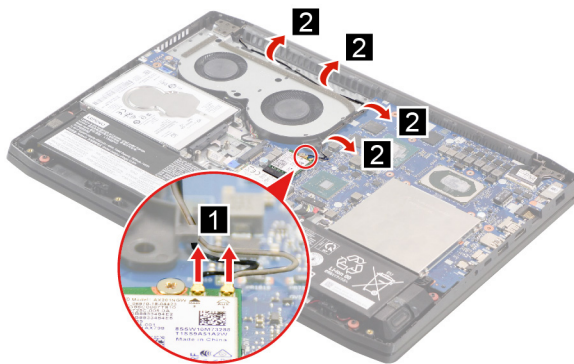
Figure 25. Detach the antenna cable connectors and release the antenna cable from the cable guide
