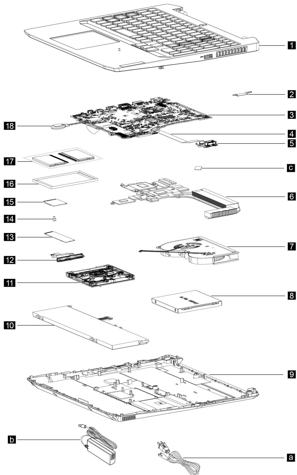
Figure 1. IdeaPad Gaming 3 (15", 05) exploded view
