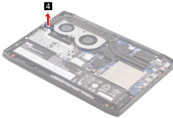
Figure 19. Remove the I/O board
