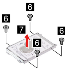
Figure 11. Remove four screws and then separate the HDD bracket and the HDD
