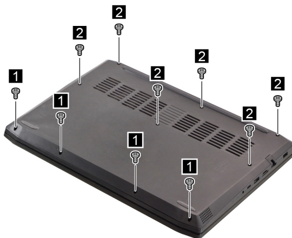
Figure 3. Remove ten screws
