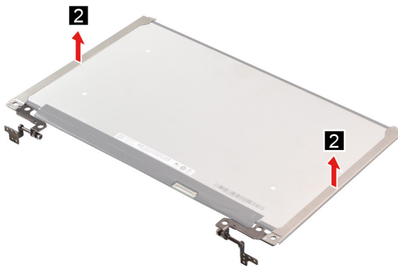
Figure 35. Remove the hinges
