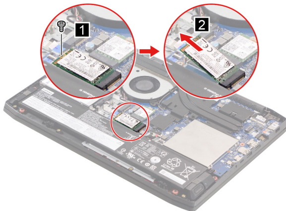
Figure 6. Remove the SSD
