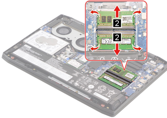
Figure 13. Remove the memory
