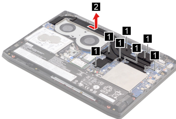
Figure 14. Loosen seven screws and then remove the heat sink
