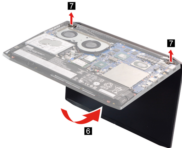
Figure 27. Remove the LCD module
