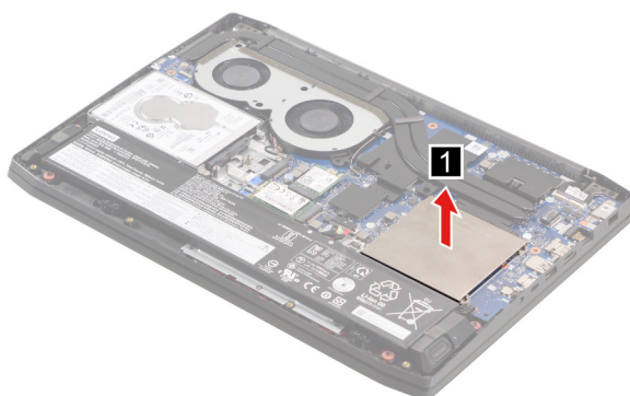
Figure 12. Remove the memory shielding
