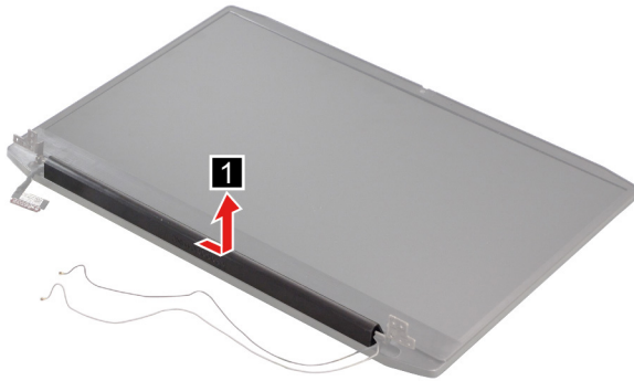
Figure 28. Remove the strip cover
