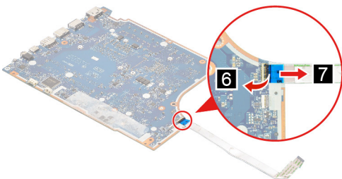
Figure 24. Remove the I/O board cable
