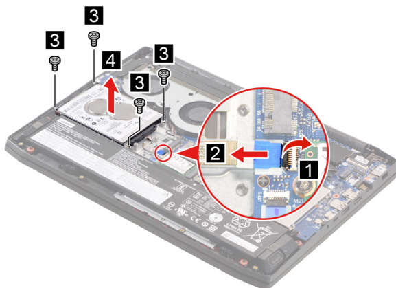
Figure 9. Remove the HDD module
