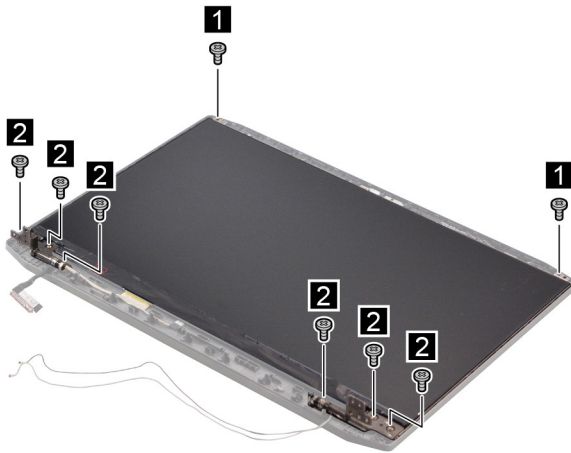
Figure 30. Remove eight screws
