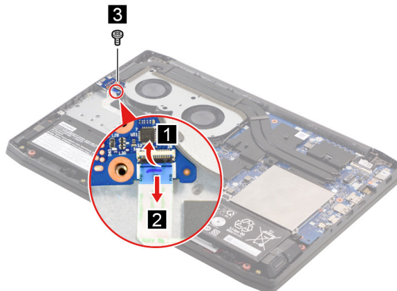
Figure 18. Detach the I/O board cable and remove one screw
