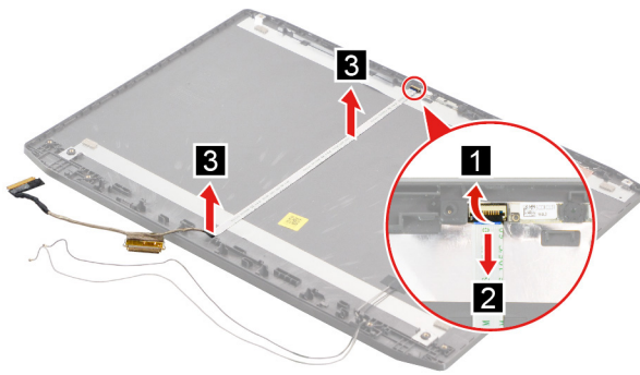
Figure 32. Remove the EDP cable
