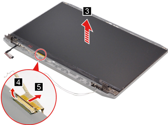
Figure 31. Remove the LCD panel
