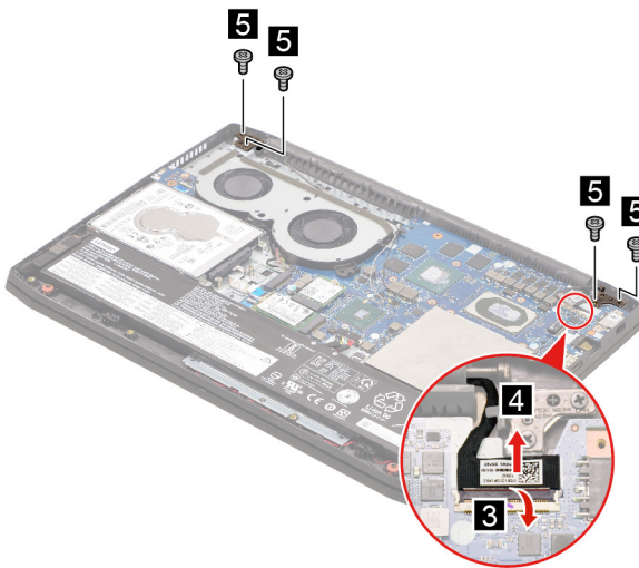
Figure 26. Disconnect the EDP cable from the system board and remove four screws
