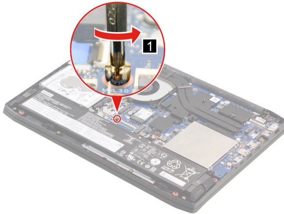
Figure 7. Remove the SSD stand off
