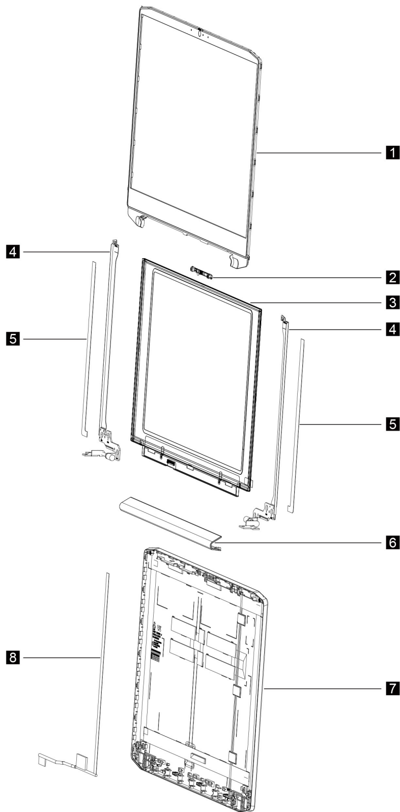
Figure 2. IdeaPad Gaming 3 (15", 05) LCD module - exploded view
