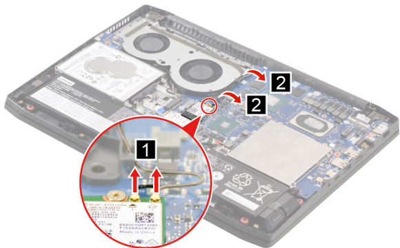
Figure 15. Release the antenna cable
