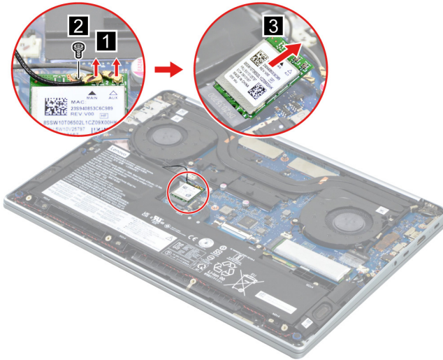
Figure 7. Remove the Wi-Fi card
