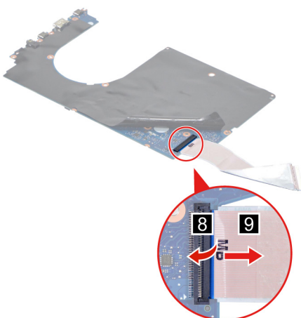
Figure 20. Remove the USB board cable
