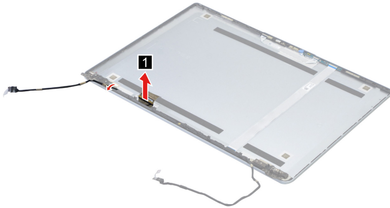
Figure 30. Remove the EDP cable
