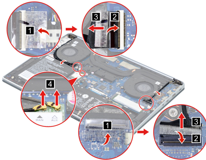
Figure 21. Disconnect cables and detach the main and auxiliary antenna cable connectors
