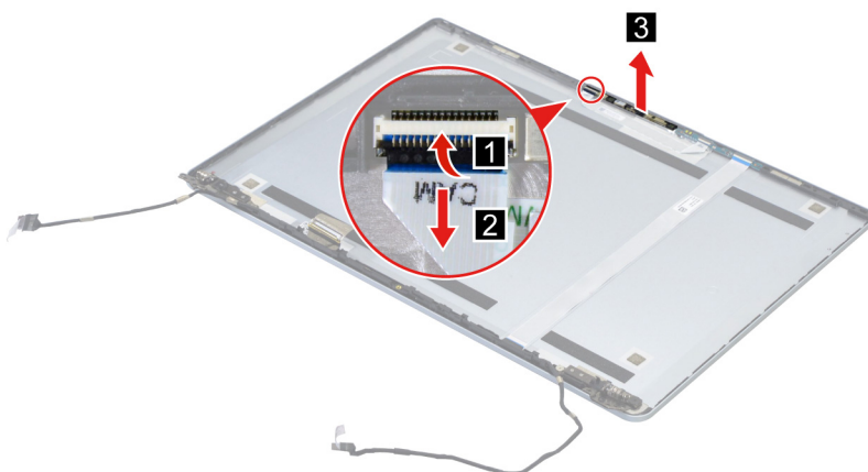
Figure 34. Disconnect the D-Mic cable and remove the camera
