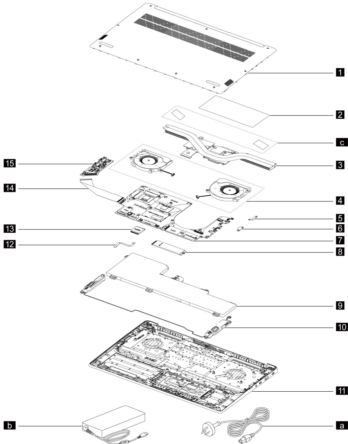
Figure 1. IdeaPad 5 Pro 16IHU6 exploded view
