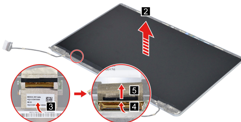
Figure 28. Disconnect the EDP cable and remove the LCD panel
