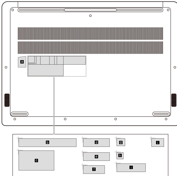
Figure 35. Label layout on the back side of the base cover
