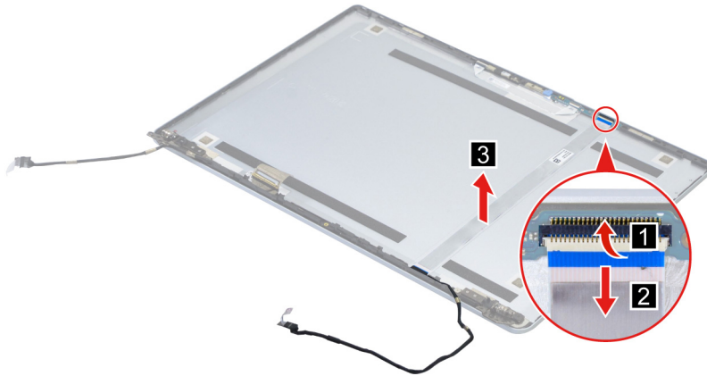
Figure 32. Remove the camera cable
