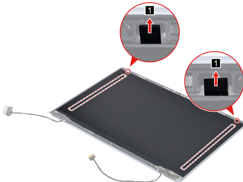
Figure 27. Remove the two pieces of removable tape with tweezers
