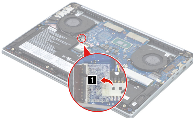
Figure 14. Peel off the tape
