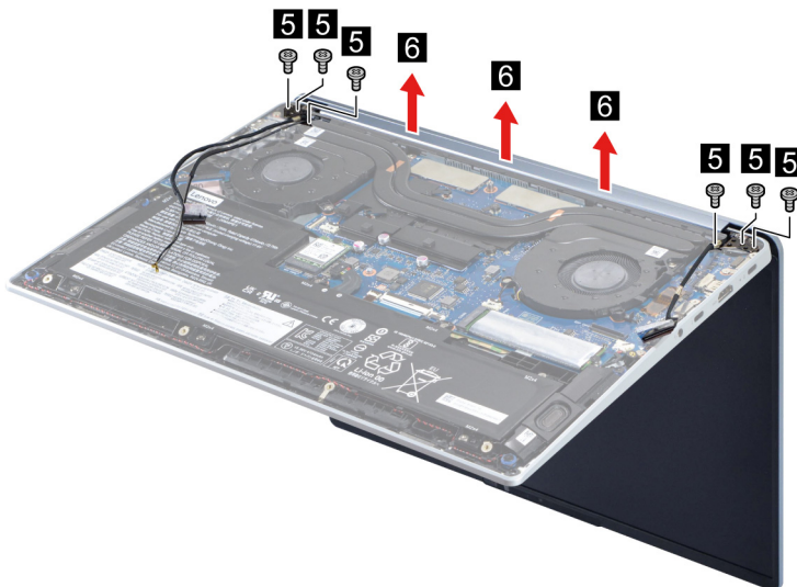
Figure 22. Rotate the LCD unit and remove the LCD unit
