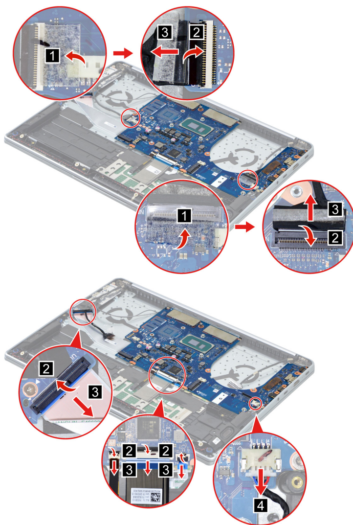
Figure 17. Disconnect cables
