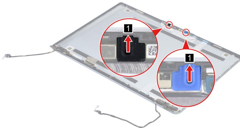
Figure 29. Remove the microphone rubbers
