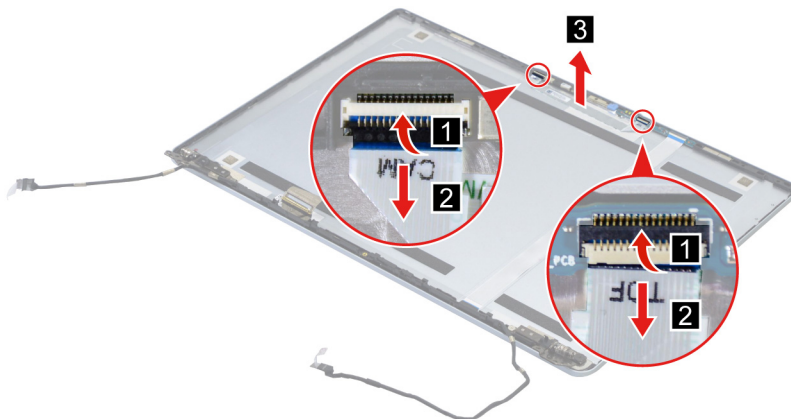
Figure 31. Remove the D-Mic cable
