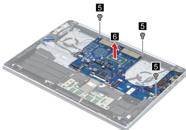
Figure 18. Remove the system board
