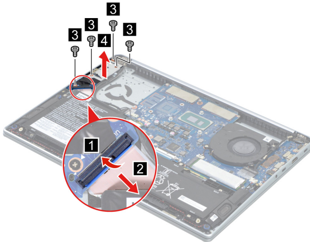
Figure 16. Disconnect the USB board cable and remove the USB board
