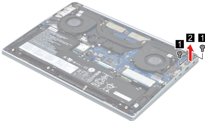
Figure 10. Remove the upper I/O board bracket
