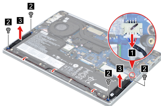
Figure 9. Remove the speakers
