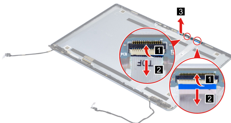
Figure 33. Remove the sensor board
