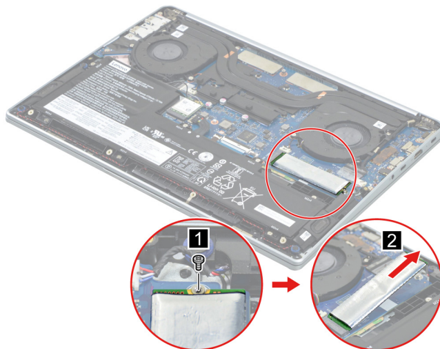
Figure 6. Remove the SSD
