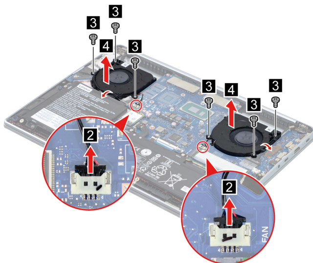
Figure 15. Disconnect the fan cables and remove the fans
