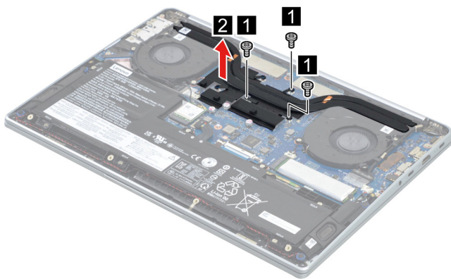
Figure 8. Remove the heat sink
