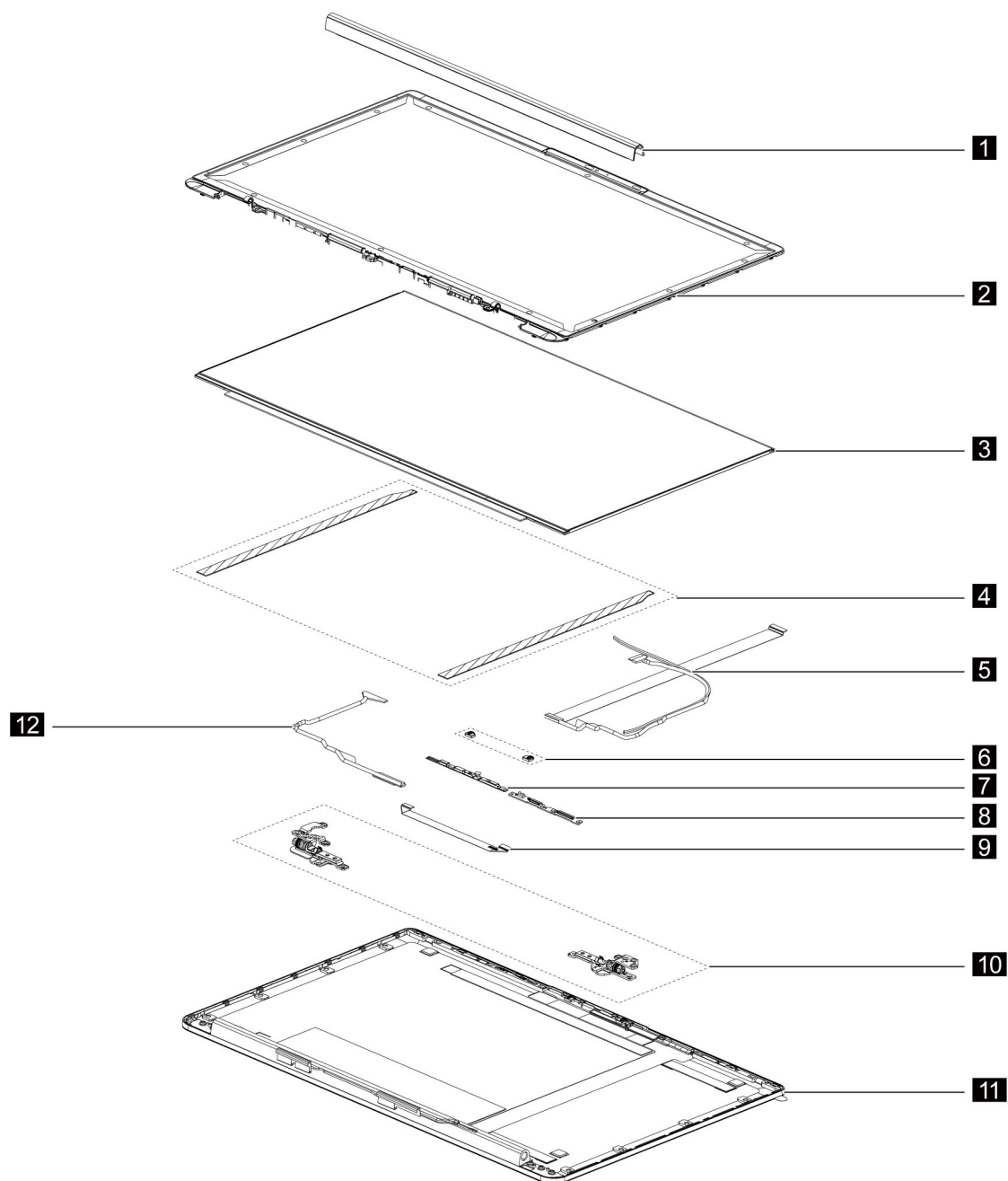
Figure 2. IdeaPad 5 Pro 16IHU6 LCD unit - exploded view
