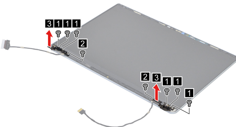
Figure 26. Remove the hinges
