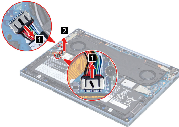
Figure 11. Remove the I/O board cable
