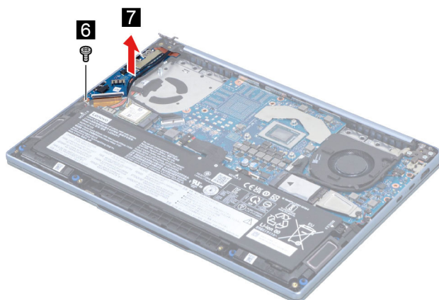
Figure 20. Remove the I/O board
