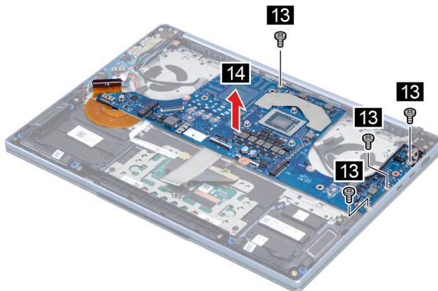
Figure 23. Remove the system board
