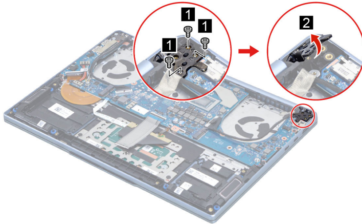
Figure 21. Open the hinge
