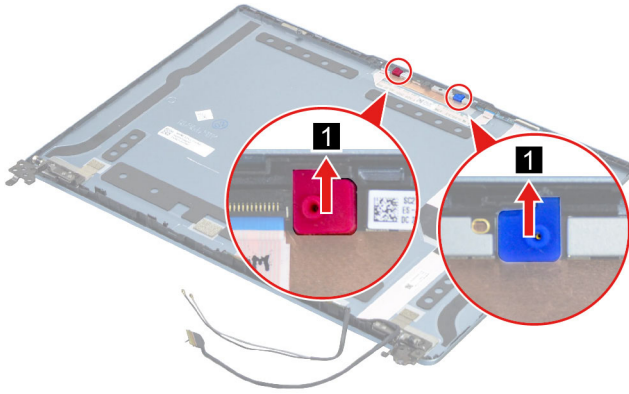
Figure 34. Remove the microphone rubber
