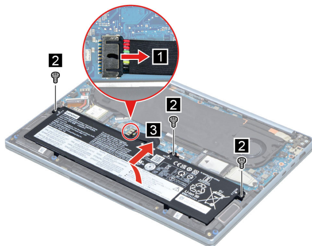
Figure 5. Remove the battery pack
