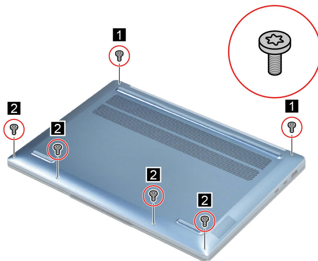
Figure 3. Remove six screws
