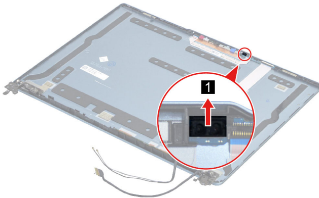
Figure 35. Remove the ToF rubber
