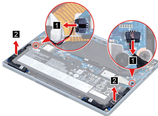
Figure 10. Remove the speakers
