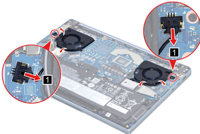
Figure 16. Detach the fan cable connectors and release cables
