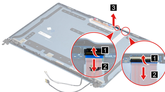
Figure 38. Remove the sensor board
