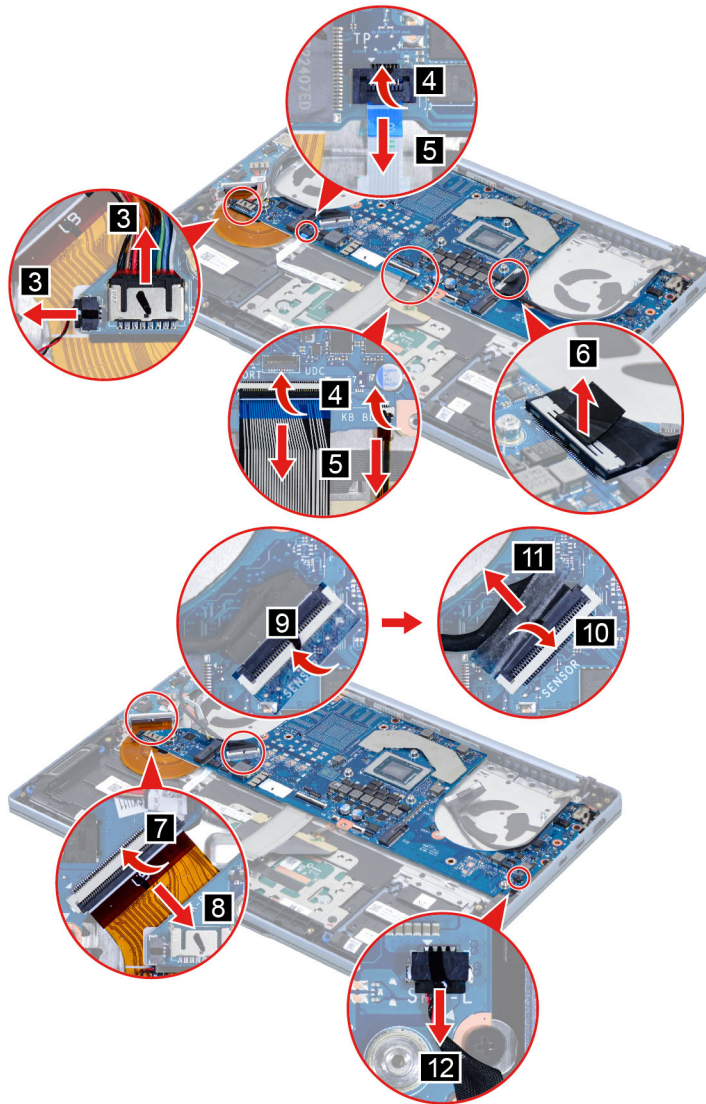
Figure 22. Disconnect cables connected to the system board
