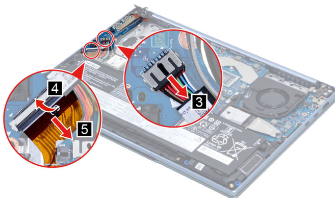
Figure 19. Disconnect cables connected to the I/O board
