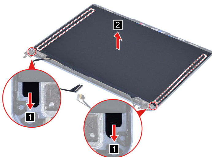
Figure 31. Remove the LCD panel
