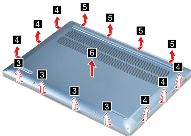
Figure 4. Remove the lower case
