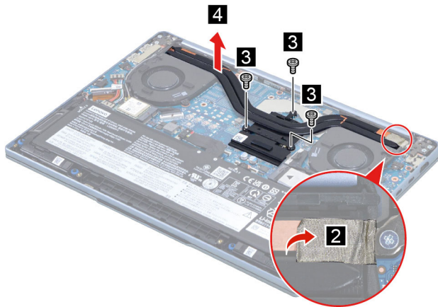
Figure 15. Remove the heat sink
