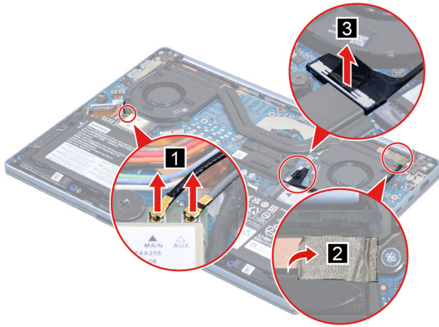
Figure 25. Disconnect the antenna cables and EDP cable
