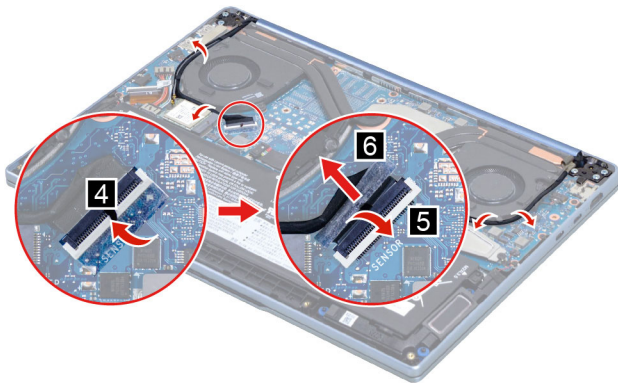
Figure 26. Disconnect the antenna cables and EDP cable
