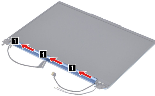
Figure 28. Remove the hinge cover
