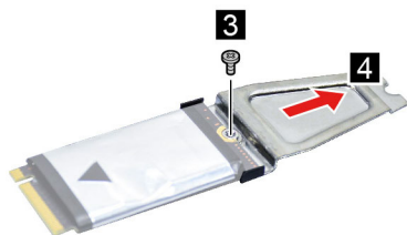
Figure 7. Remove the SSD bracket
