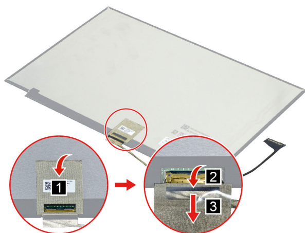
Figure 32. Remove the EDP cable
