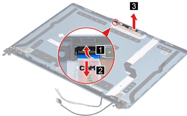
Figure 39. Remove the camera board
