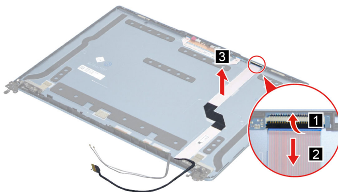
Figure 37. Remove the sensor board cable
