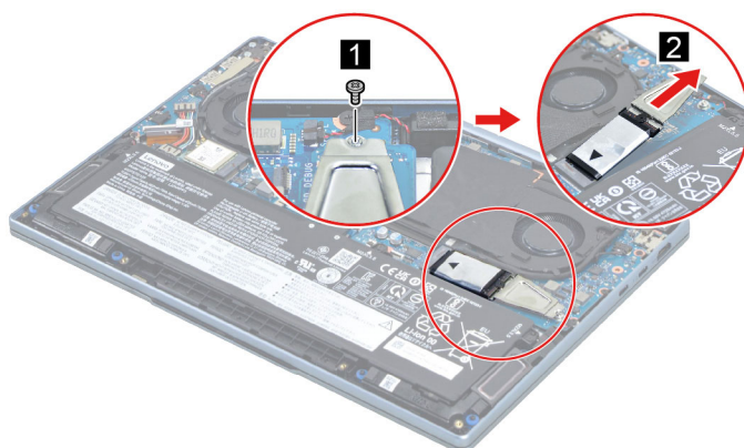
Figure 6. Remove the SSD
