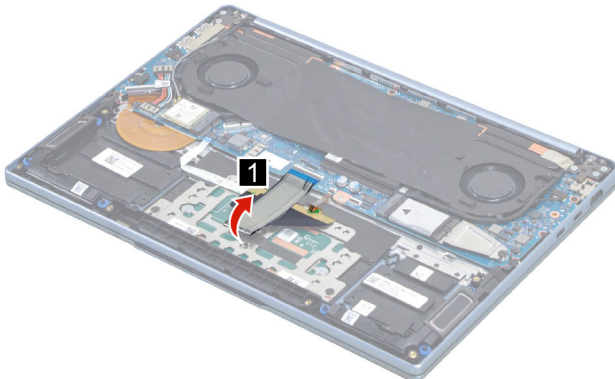
Figure 12. Peel back the keyboard FPC
