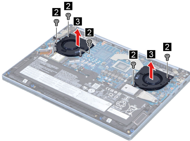
Figure 17. Remove the fans
