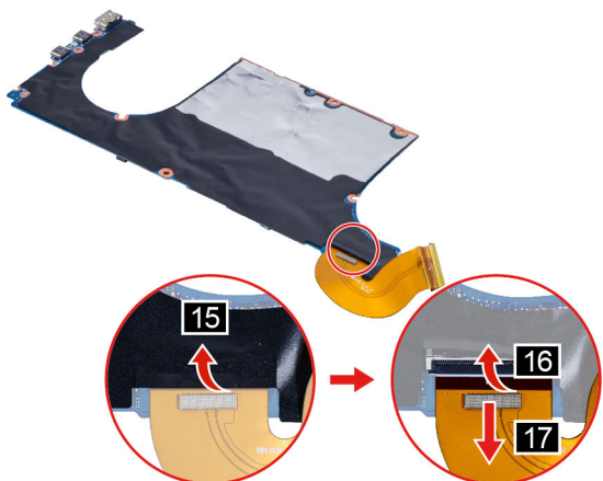
Figure 24. Remove the I/O board FPC
