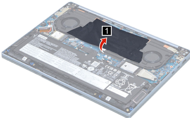
Figure 14. Peel off the system mylar
