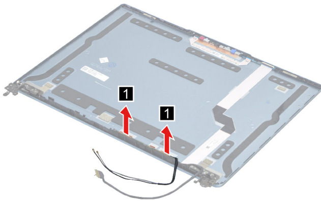
Figure 33. Remove the antenna
