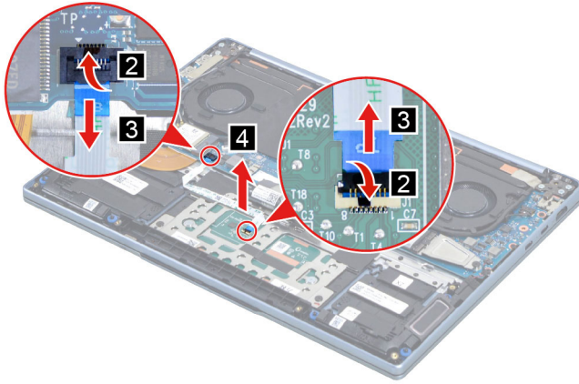
Figure 13. Remove the touchpad board cable
