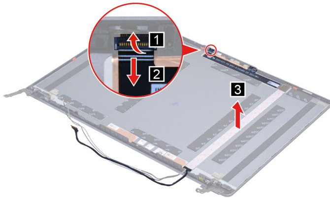
Figure 32. Remove the camera cable
