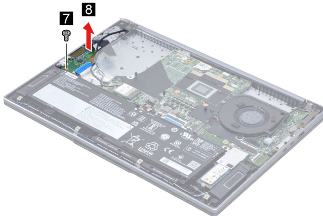
Figure 17. Remove the I/O board
