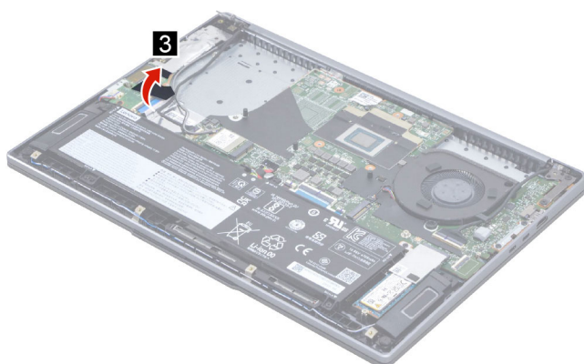
Figure 15. Peel back the I/O board mylar
