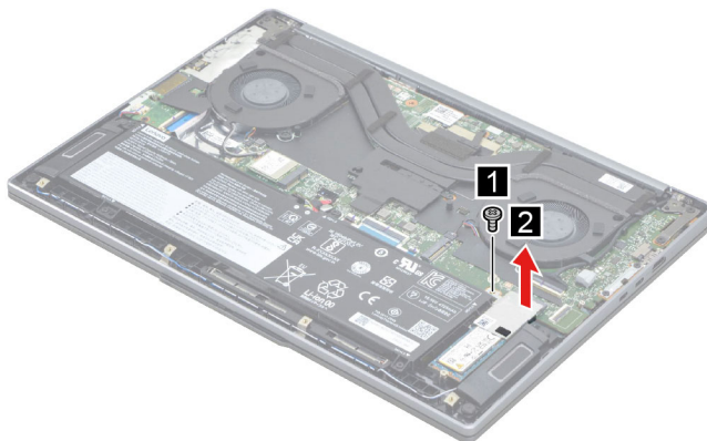
Figure 6. Remove the SSD plate
