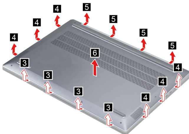
Figure 4. Remove the lower case
