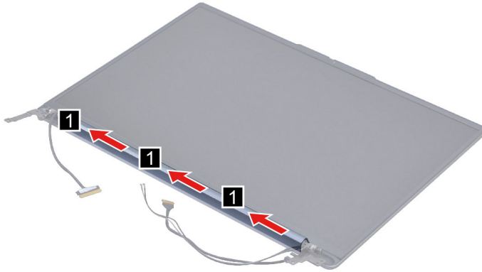
Figure 25. Remove the hinge cover
