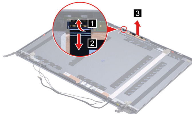
Figure 33. Remove the camera board
