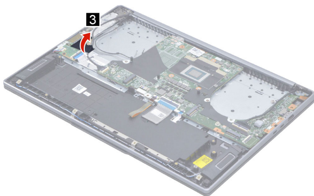
Figure 20. Peel back the I/O board mylar
