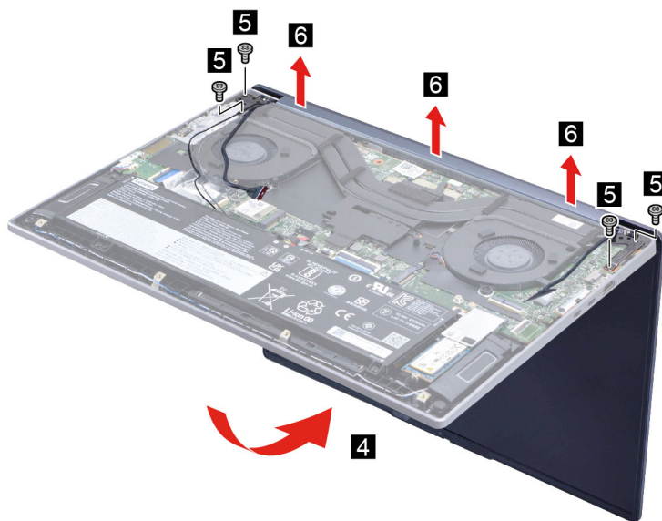
Figure 24. Remove the LCD module
