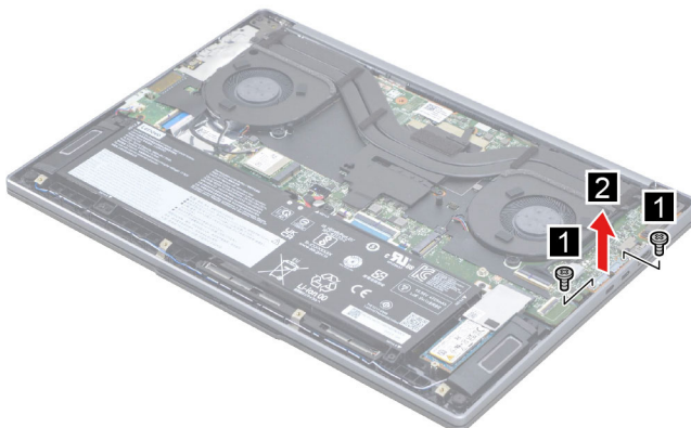
Figure 10. Remove the Type-C bracket
