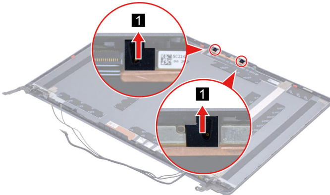
Figure 30. Remove the microphone rubber
