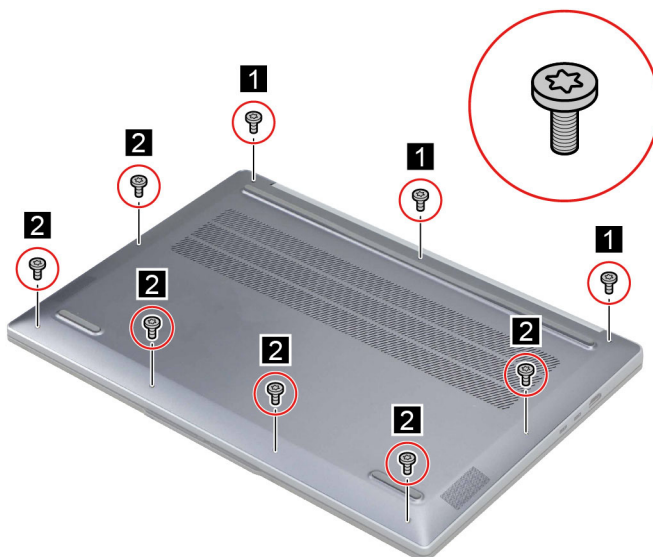
Figure 3. Remove nine screws
