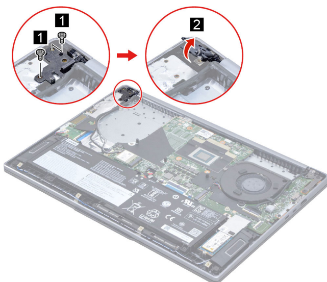
Figure 14. Remove two screws and then open the hinge
