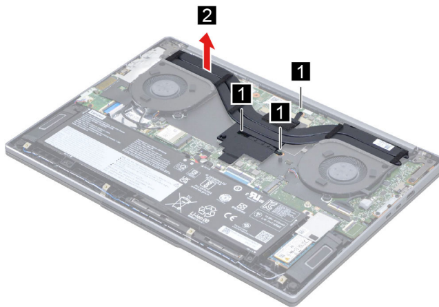
Figure 11. Remove the heat sink
