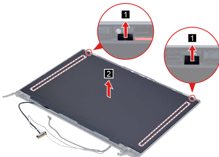
Figure 28. Remove the LCD panel
