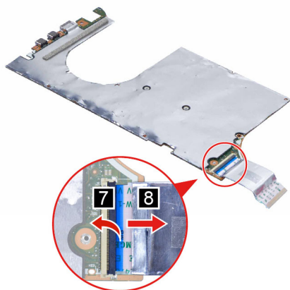
Figure 22. Remove the I/O board cable
