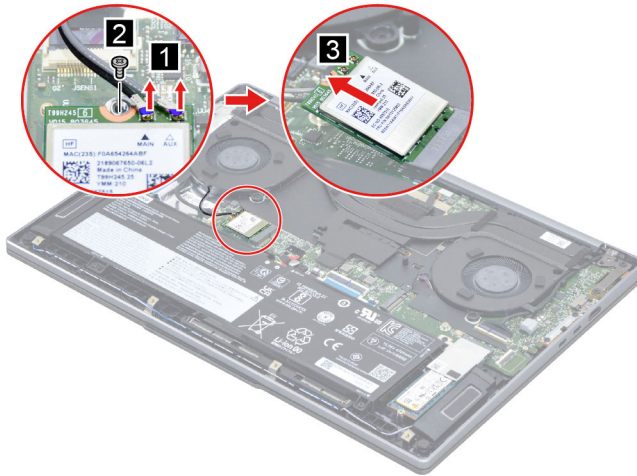
Figure 9. Remove the Wi-Fi card
