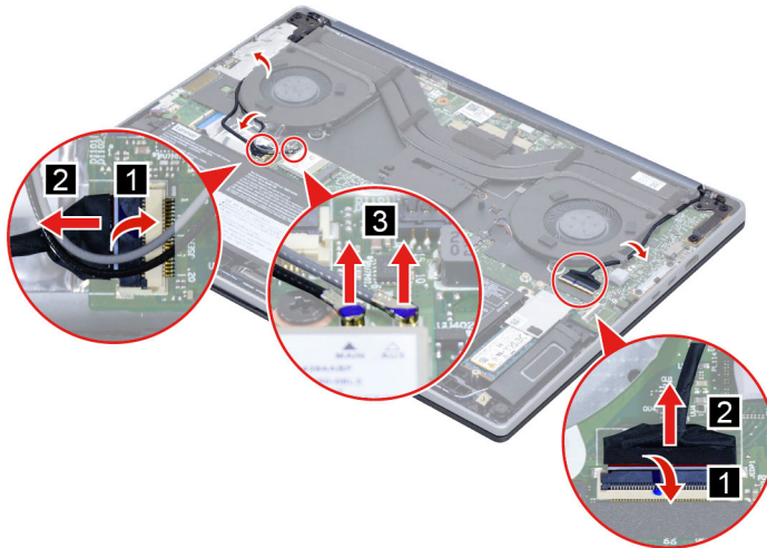
Figure 23. Disconnect the antenna cables, EDP cable and camera cable
