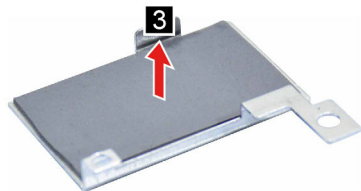
Figure 7. Remove the SSD thermalpad
