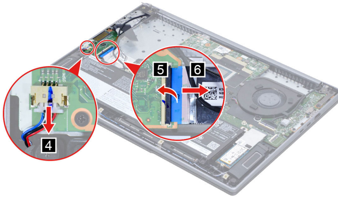
Figure 16. Disconnect cables connected to the I/O board
