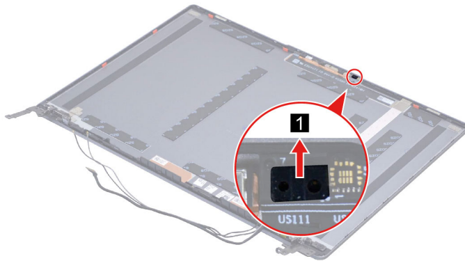
Figure 31. Remove the ToF rubber
