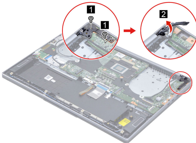
Figure 19. Open the hinge
