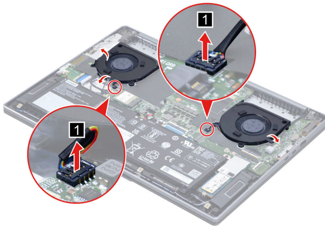
Figure 12. Detach the fan cable connectors and release cables
