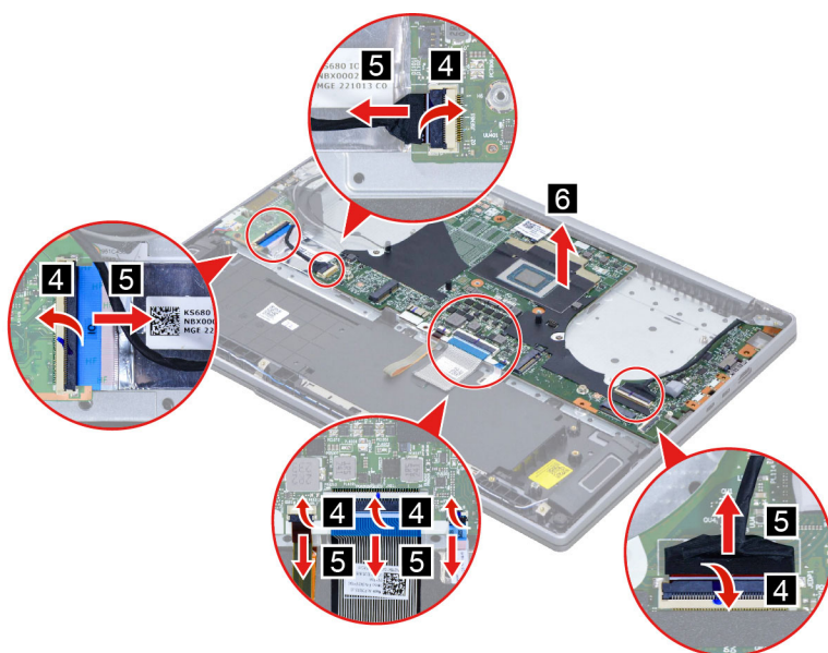
Figure 21. Remove the system board
