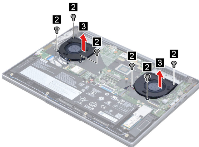
Figure 13. Remove the fans
