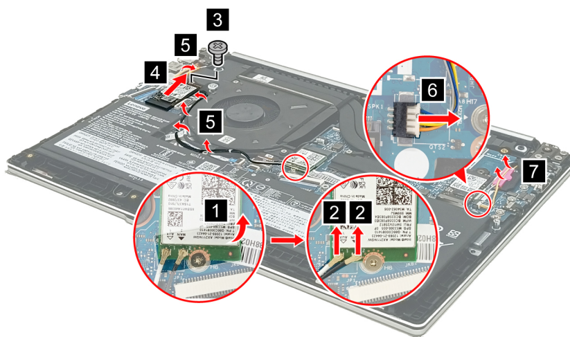
Figure 31. Disconnect and remove the antennas and the speaker cable
