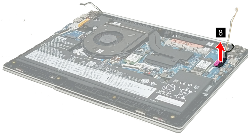
Figure 32. Disconnect the EDP cable from the system board
