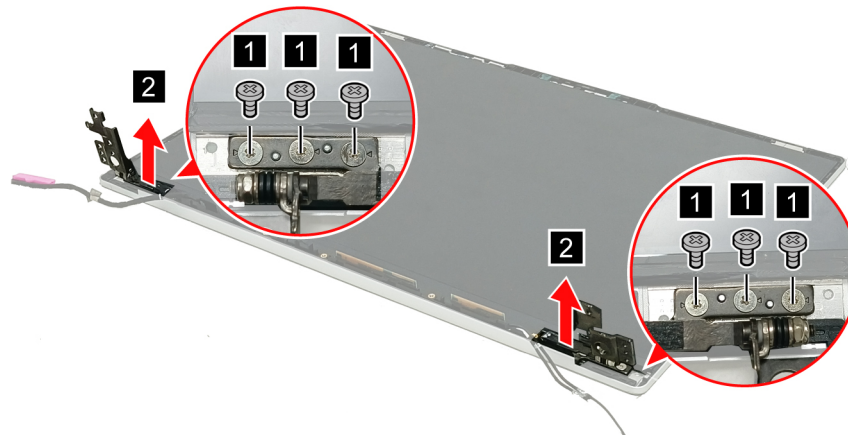
Figure 37. Remove the hinges
