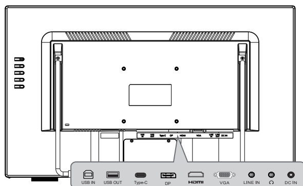
Figure.2. Connecting to a PC
