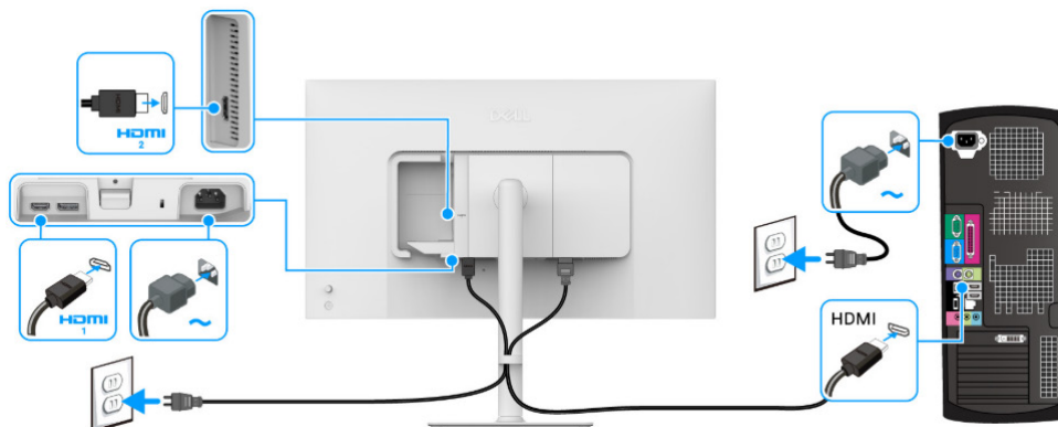
Figure 7. Connexion HDMI
