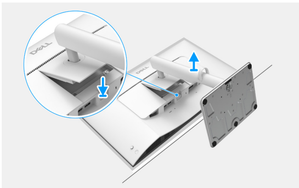
Figure 9. Retirer le pied
