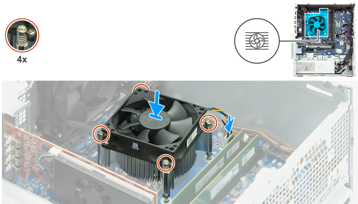
Figure 93. Installing the processor fan and heat-sink assembly
