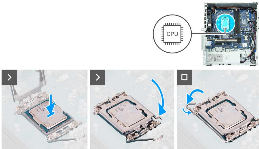
Figure 95. Installing the processor
