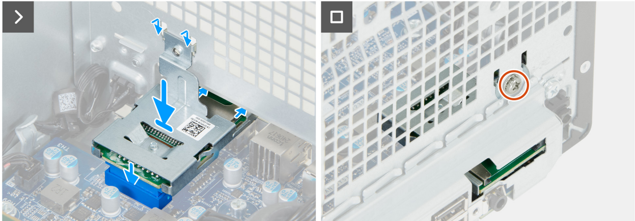
Figure 85. Installing the media-card reader
