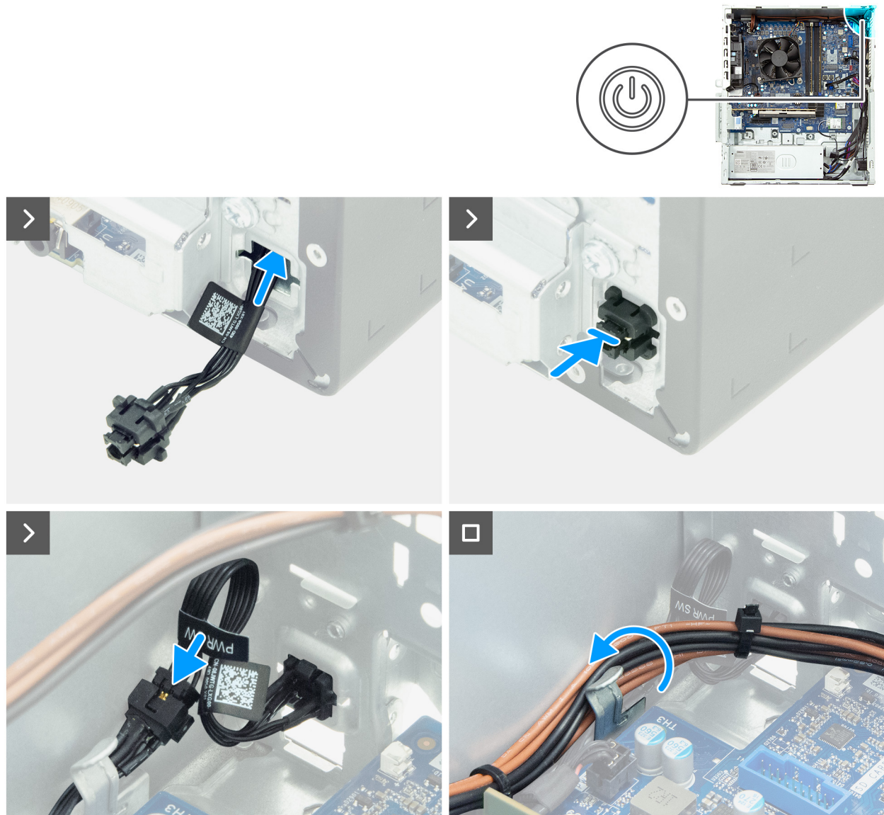
Figure 74. Installing the power button
