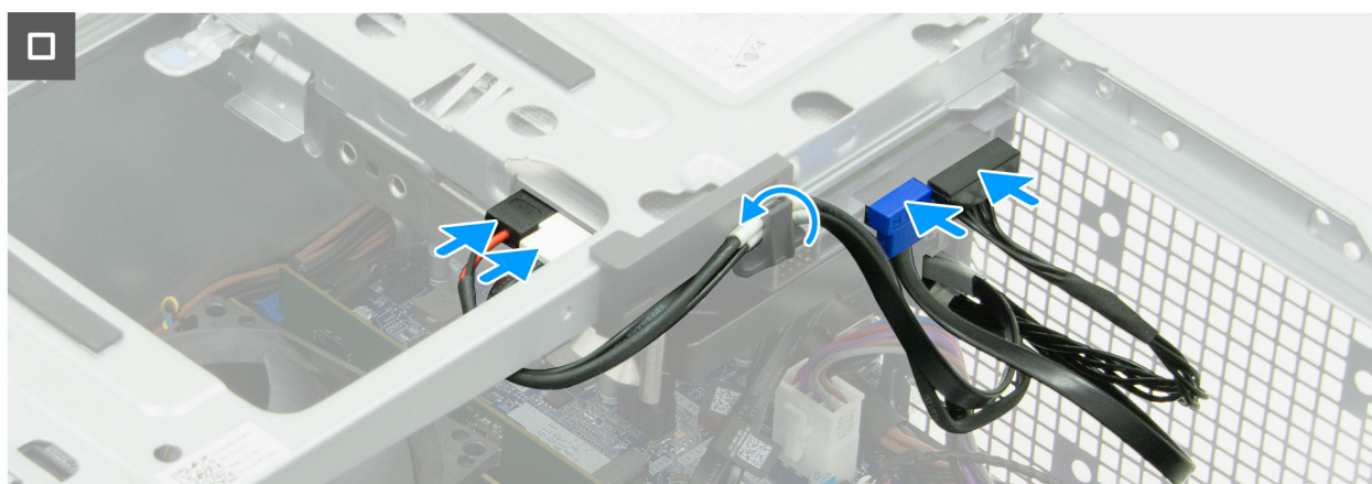
Figure 62. Installing the drive bay
