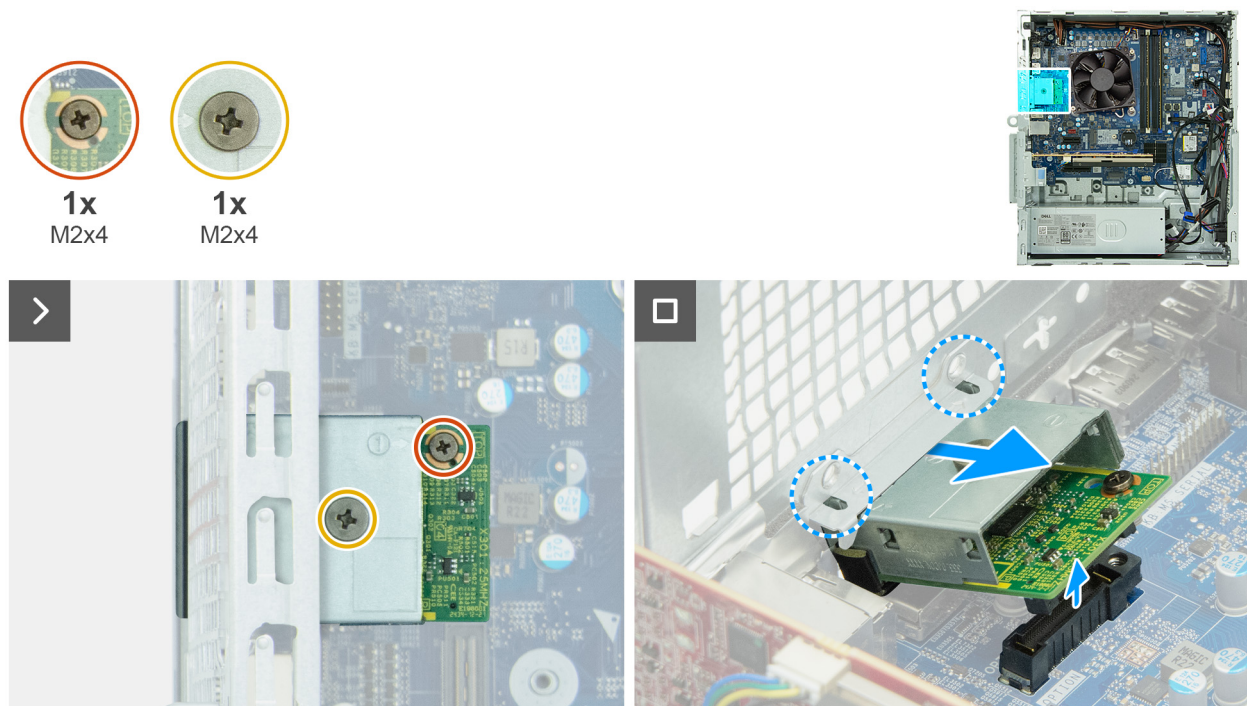
Figure 75. Removing the optional-port module
