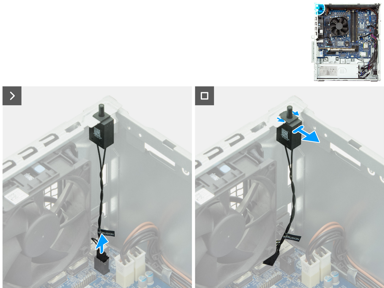
Figure 65. Removing the intrusion switch
