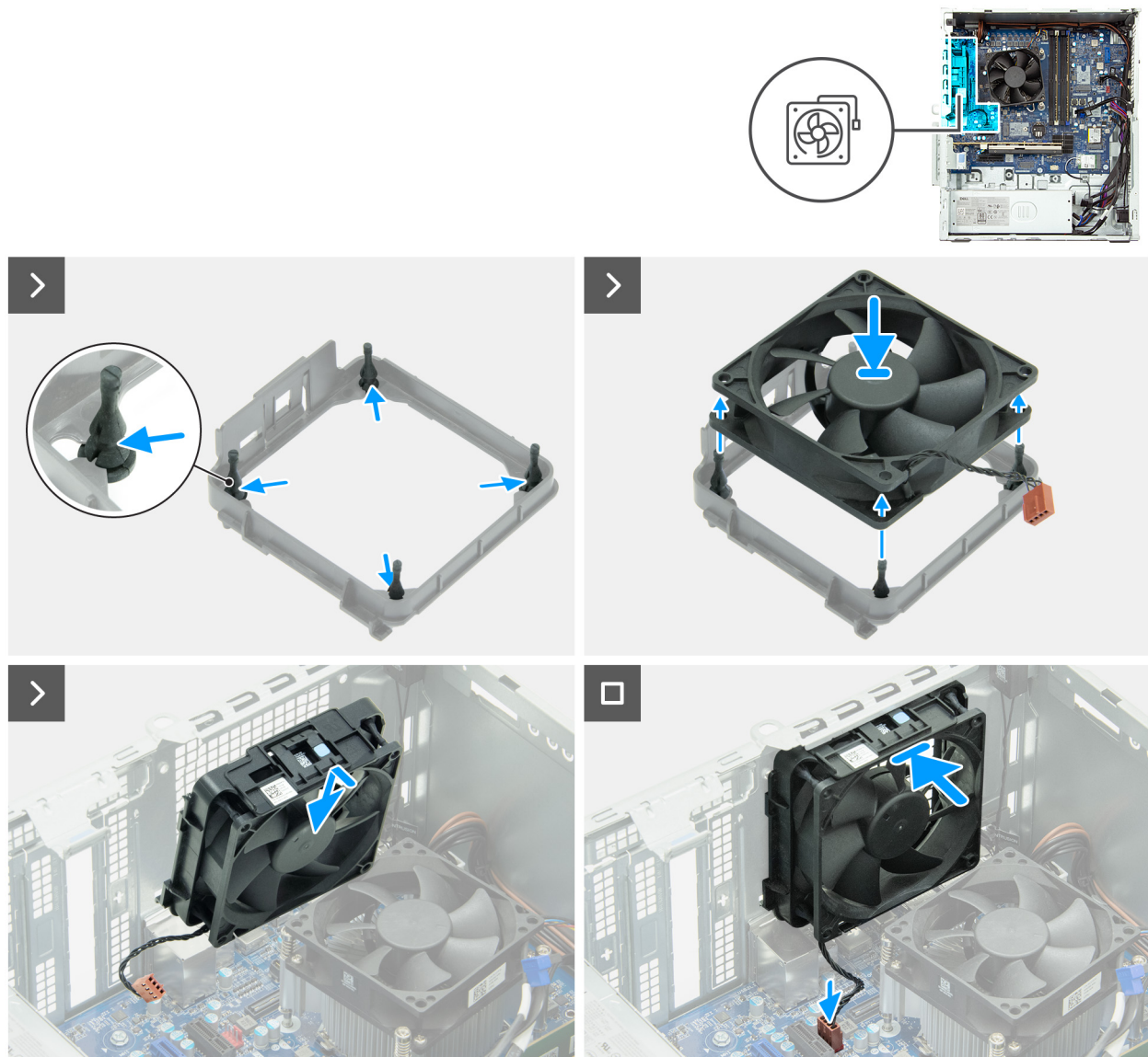
Figure 68. Installing the fan
