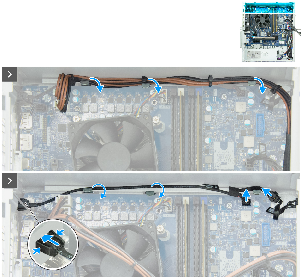
Figure 69. Removing the remote-power switch cable
