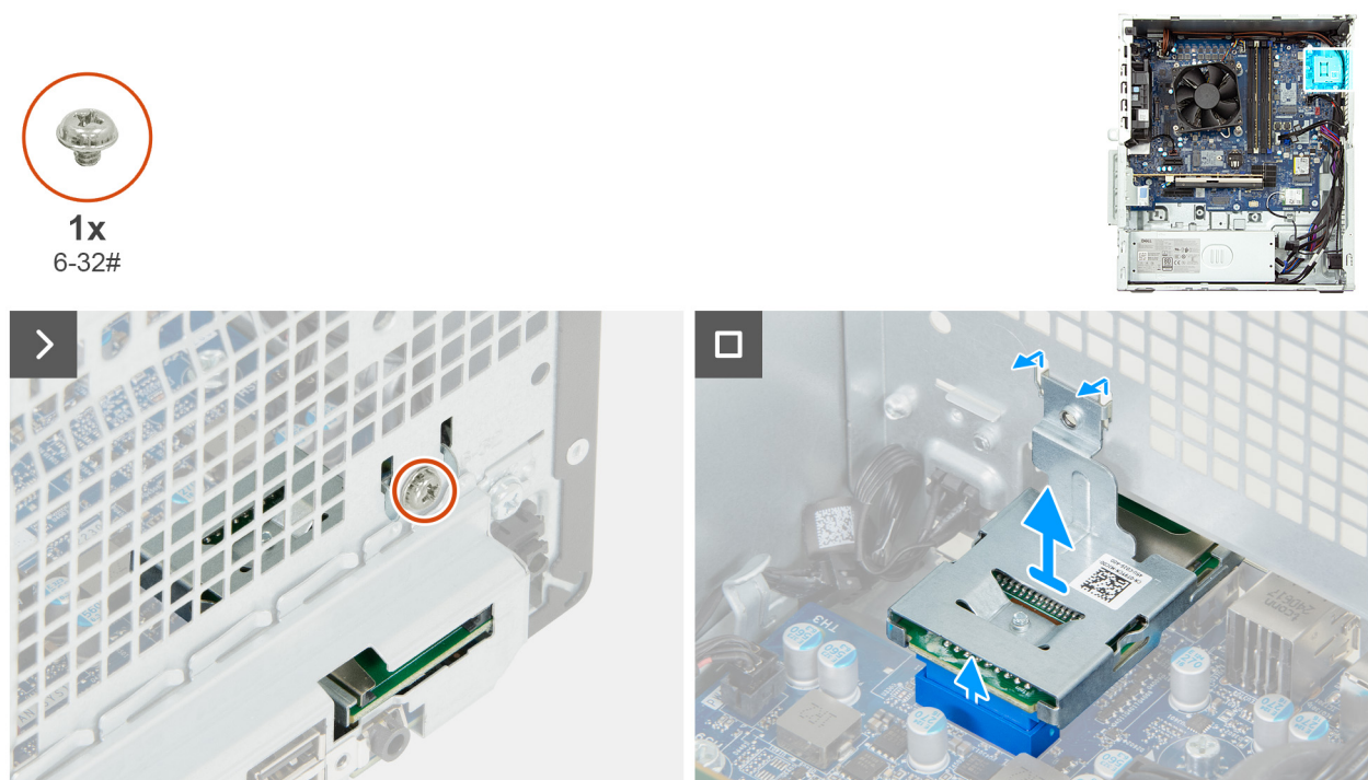
Figure 84. Removing the media-card reader
