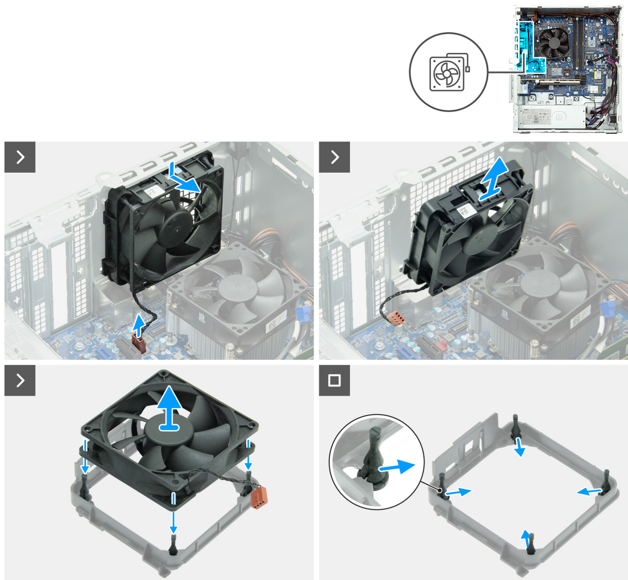
Figure 67. Removing the fan
