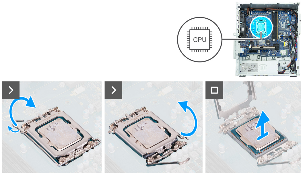
Figure 94. Removing the processor
