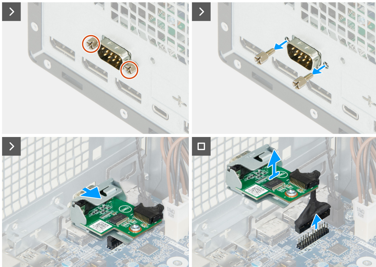
Figure 81. Removing the serial-port module
