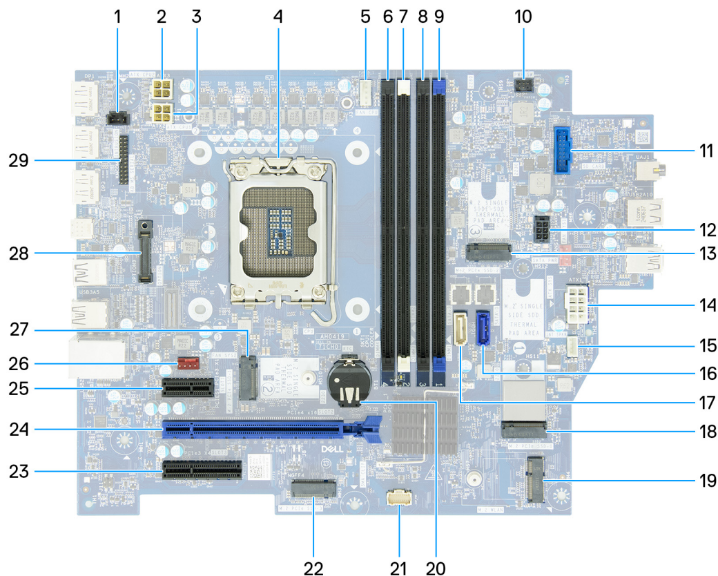
Figure 101. System board callouts
