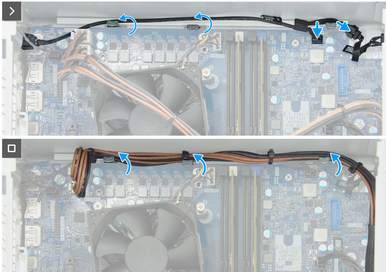
Figure 72. Installing the remote-power switch cable
