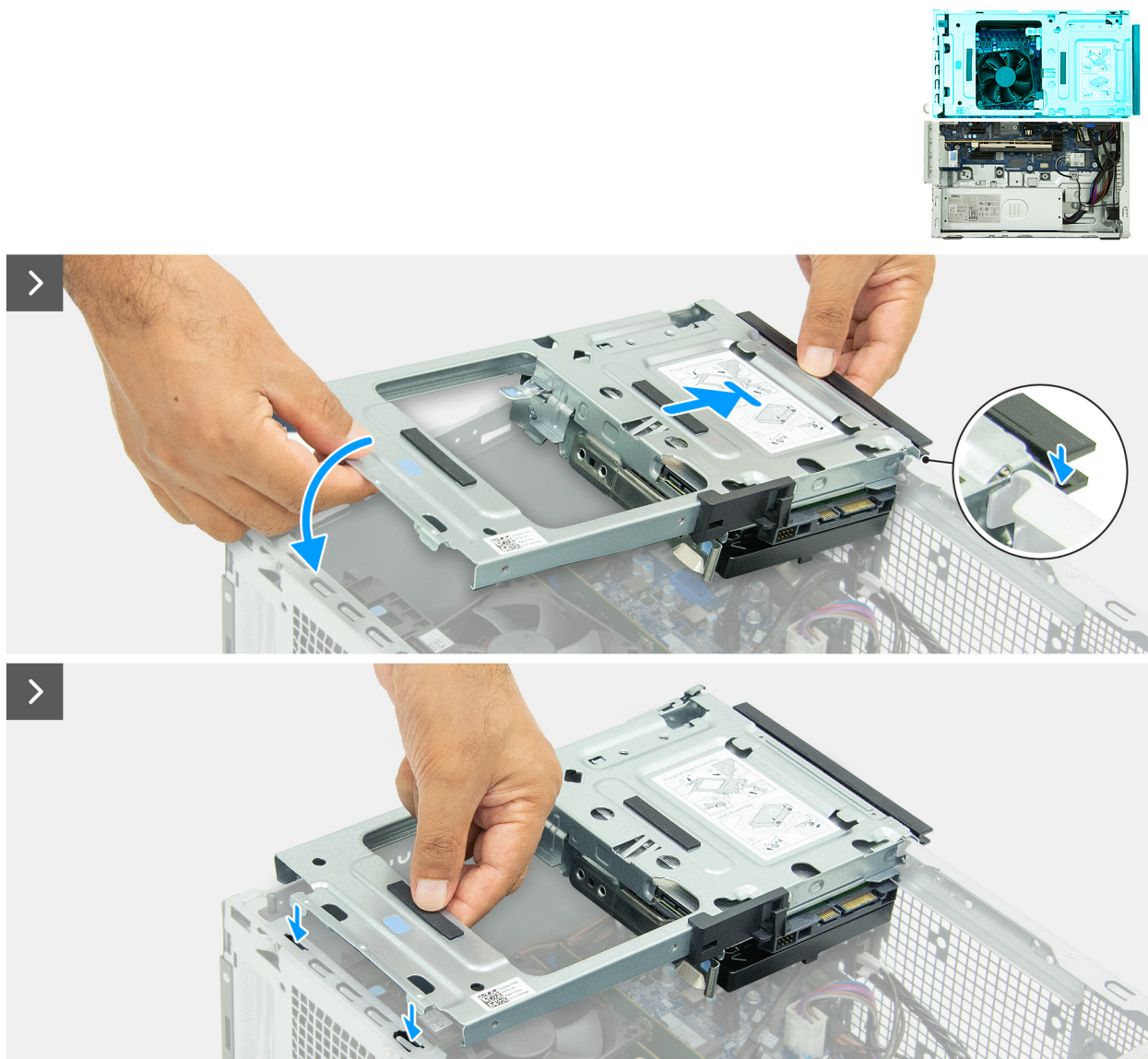
Figure 61. Installing the drive bay
