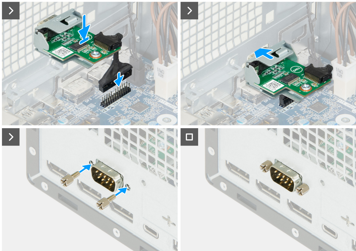
Figure 83. Installing the serial-port module
