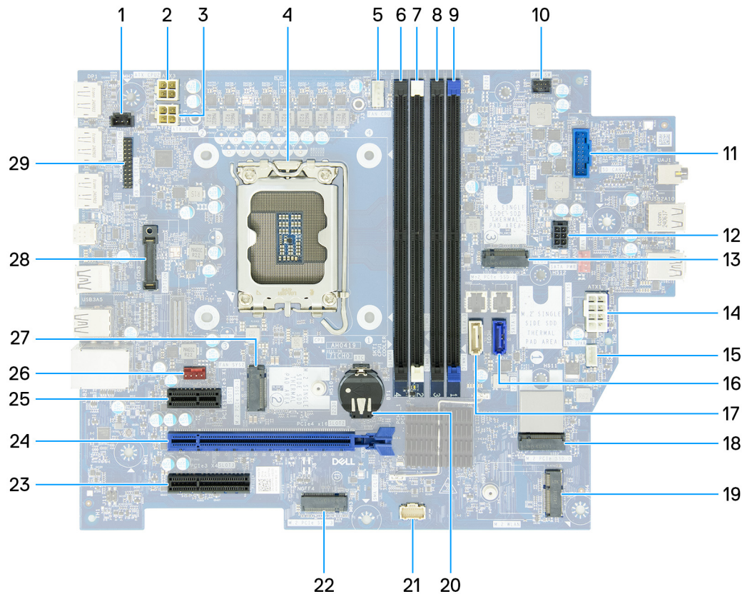
Figure 96. System board callouts
