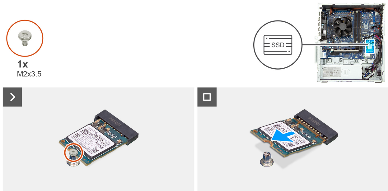
Figure 29. Removing the M.2 2230 solid-state drive in slot 0
