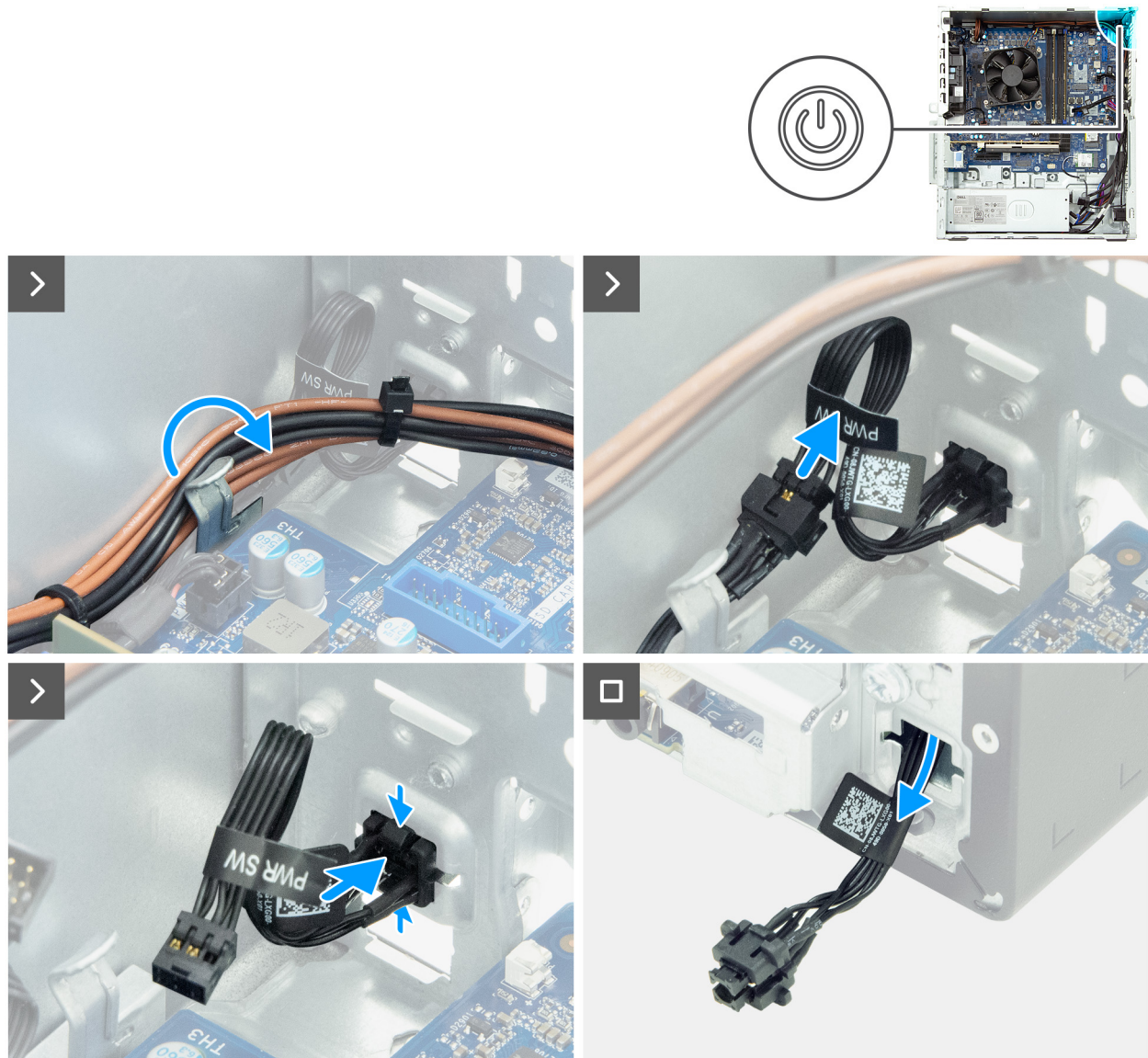
Figure 73. Removing the power button
