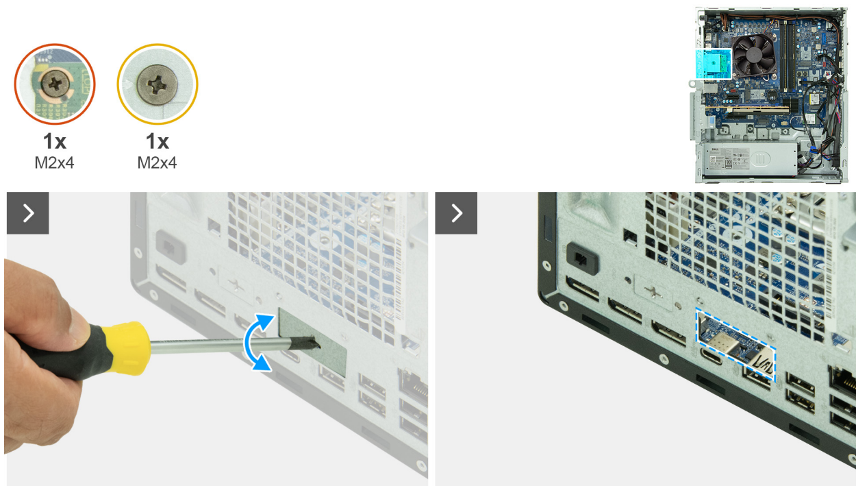
Figure 76. Installing the optional-port module
