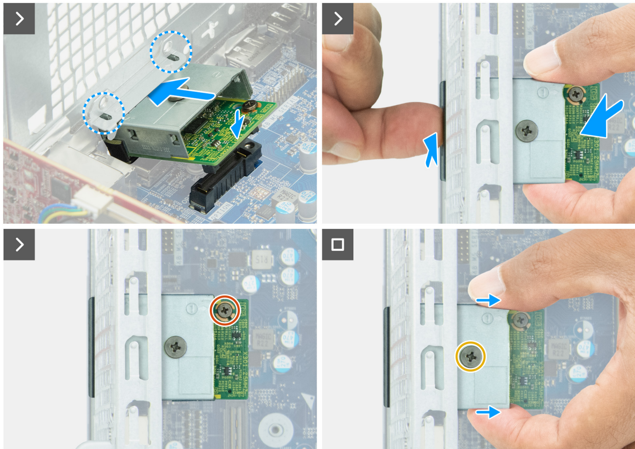
Figure 77. Installing the optional-port module
