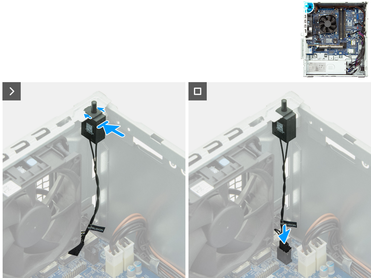
Figure 66. Installing the intrusion switch
