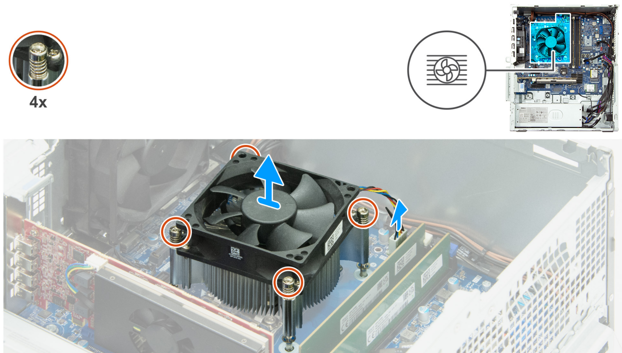
Figure 92. Removing the processor fan and heat-sink assembly
