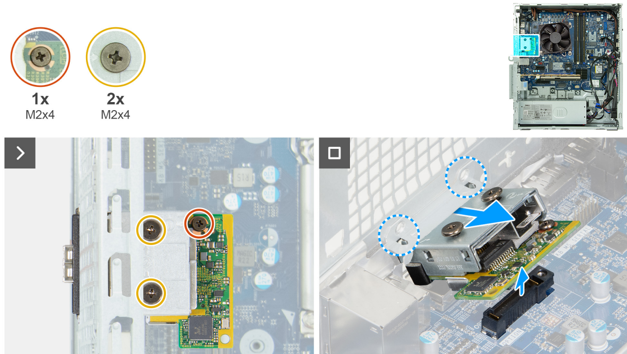
Figure 78. Removing the fiber-optic port module
