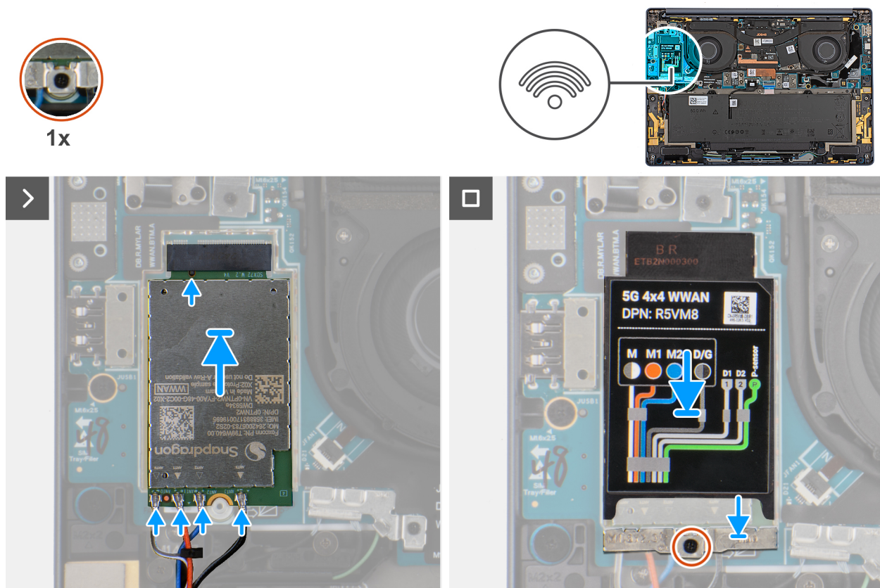
Figure 29. Installing the WWAN card
