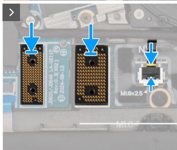
Figure 42. Installing the left I/O-board
