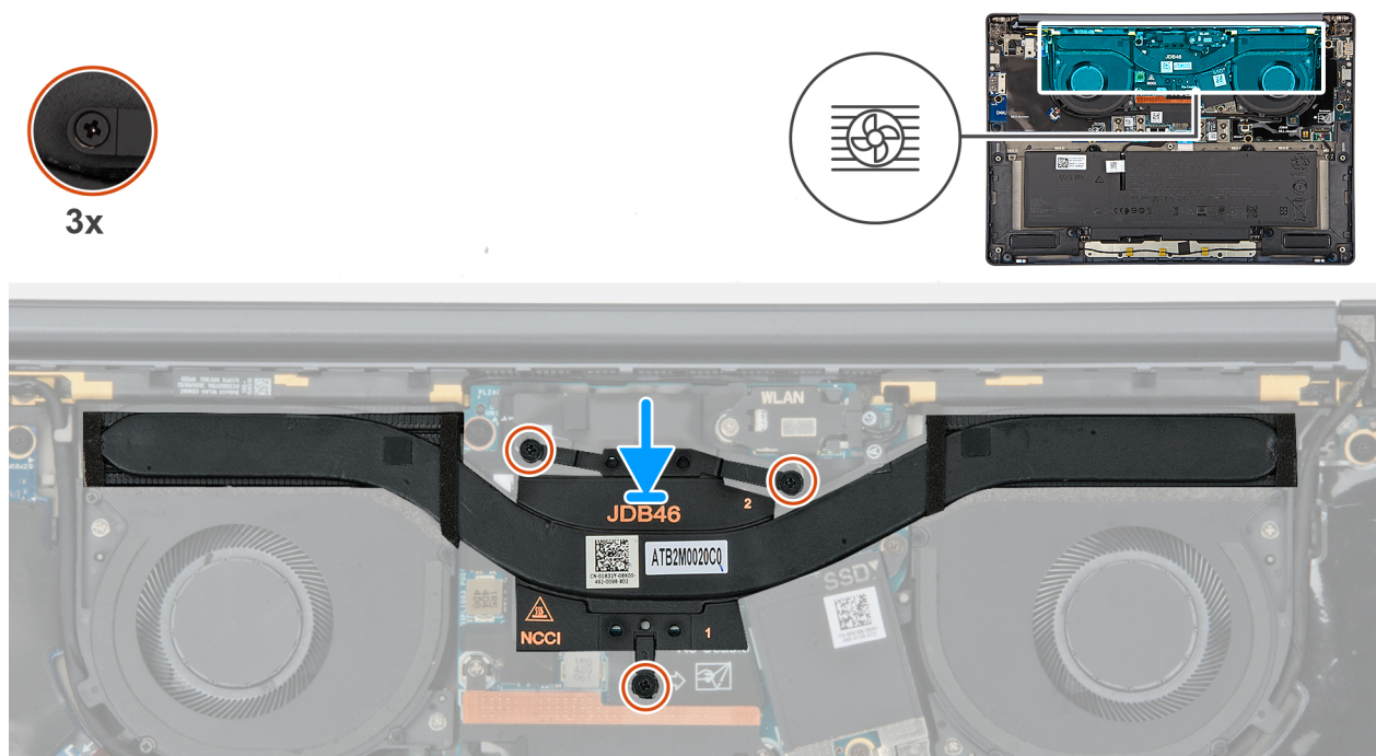
Figure 39. Installing the heat sink
