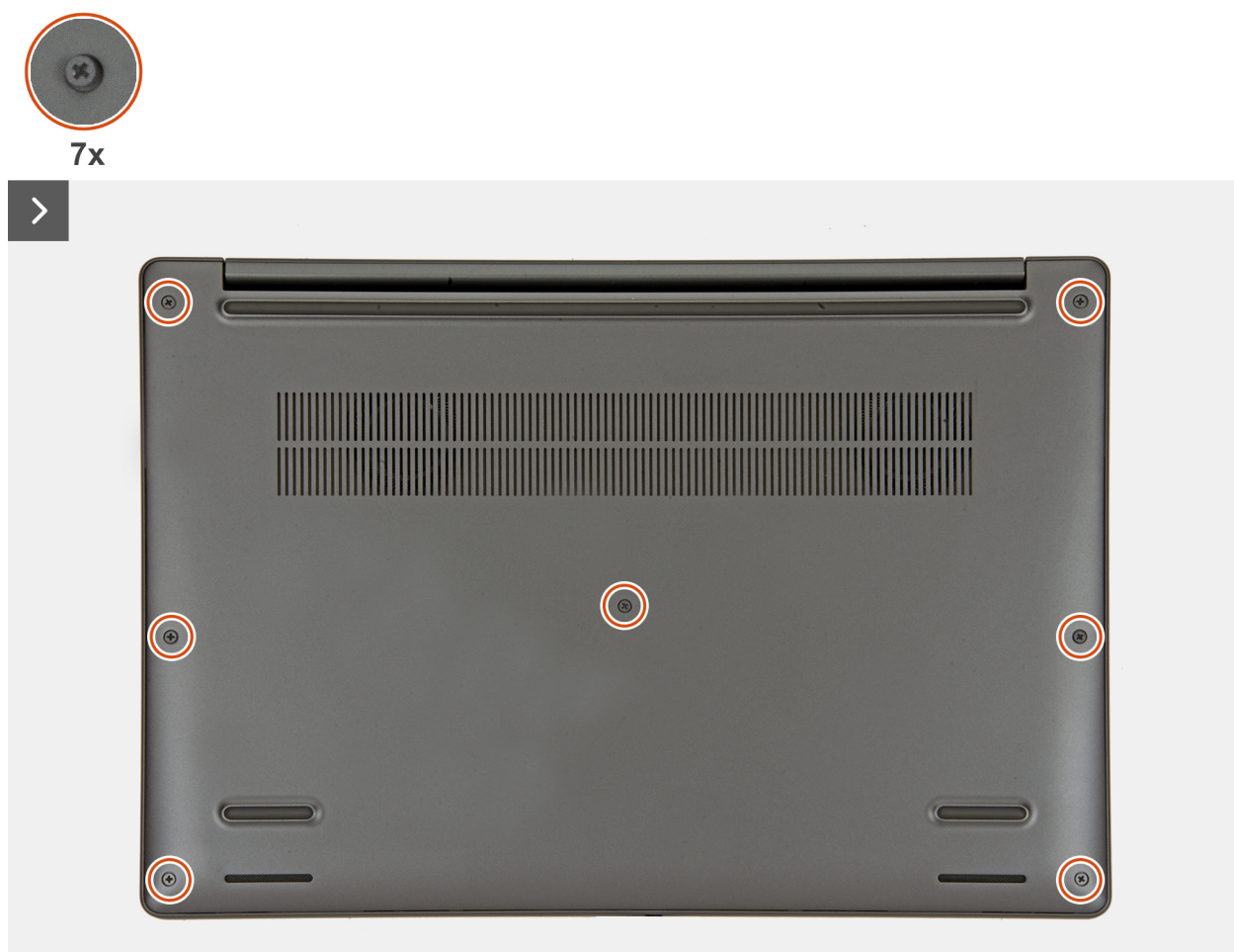
Figure 16. Loosen the captive screws
