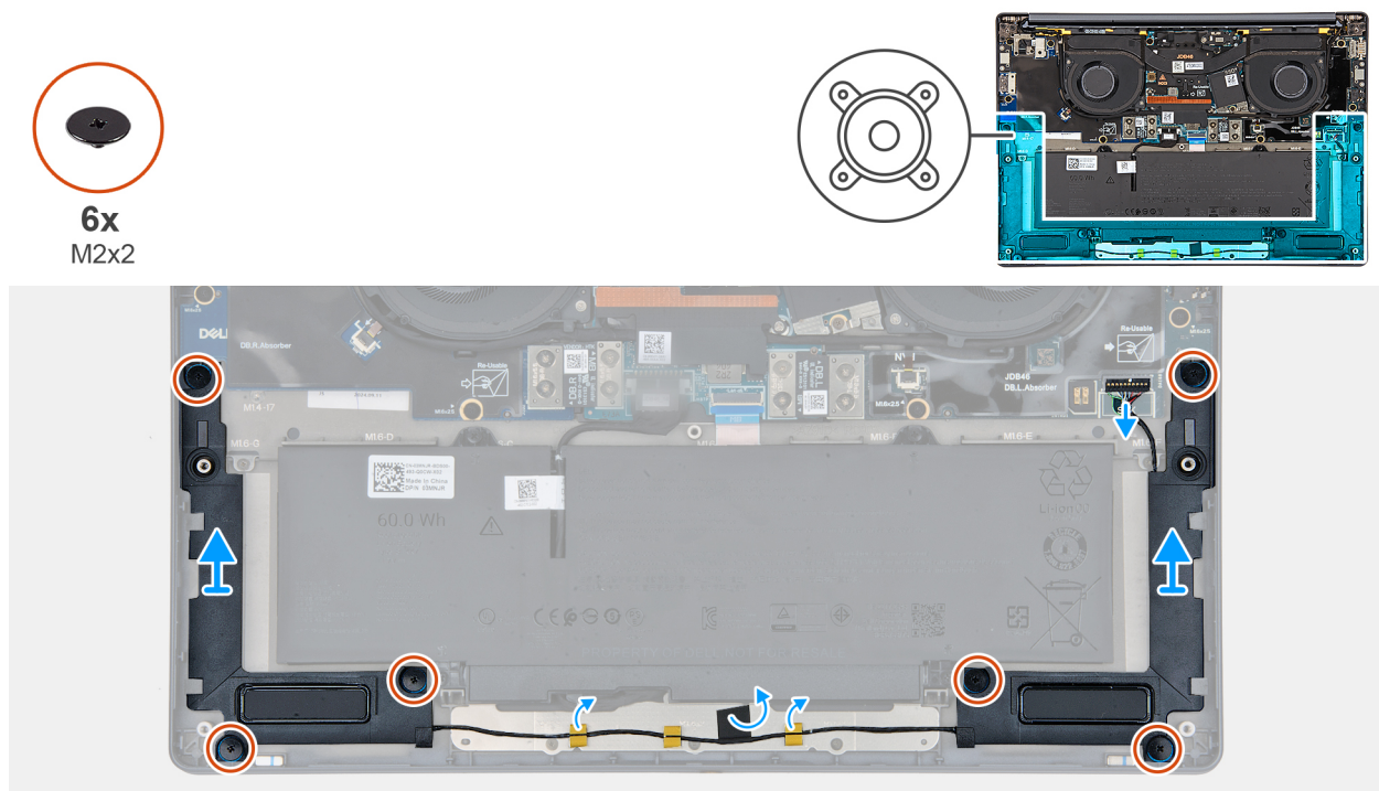
Figure 34. Removing the speakers without antenna (WLAN configuration)
