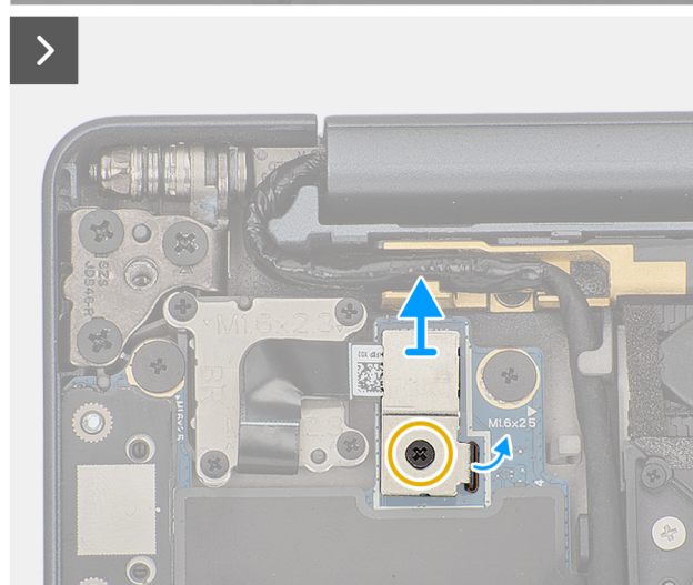
Figure 44. Removing the screws
