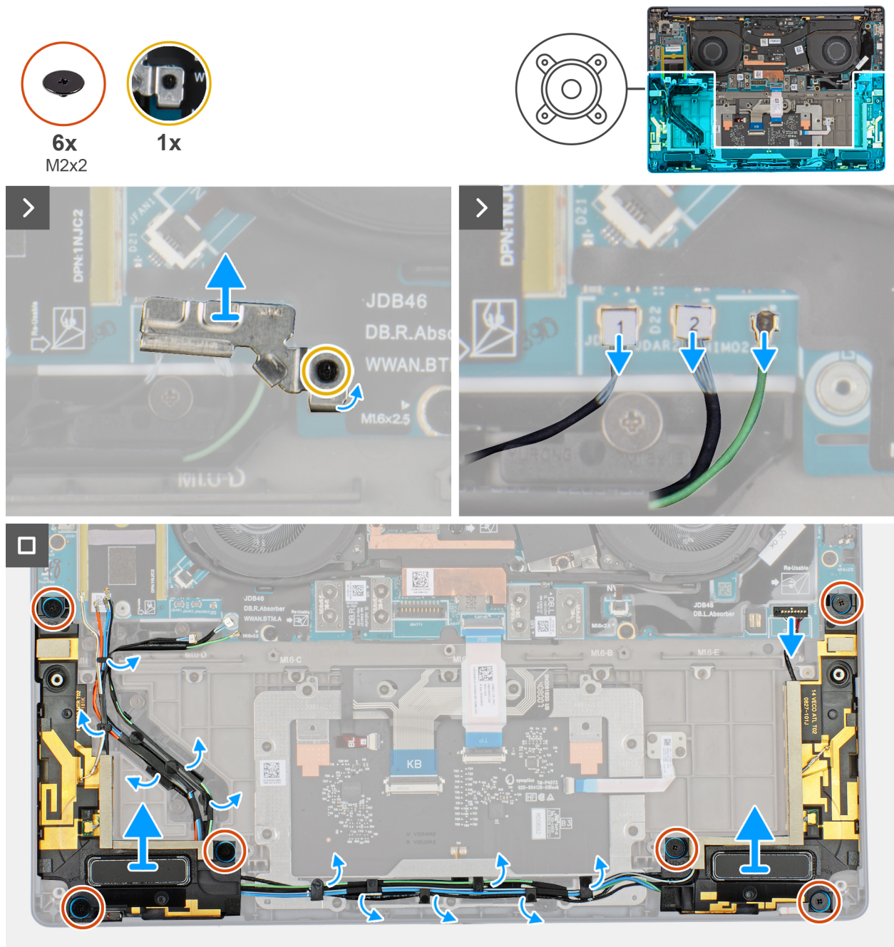
Figure 36. Removing the speakers with antennas (WWAN configuration)
