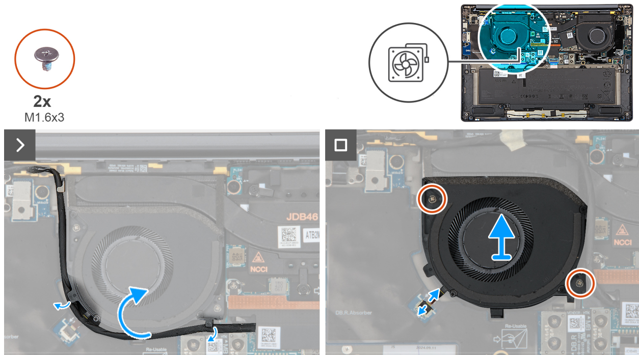
Figure 32. Removing the right fan
