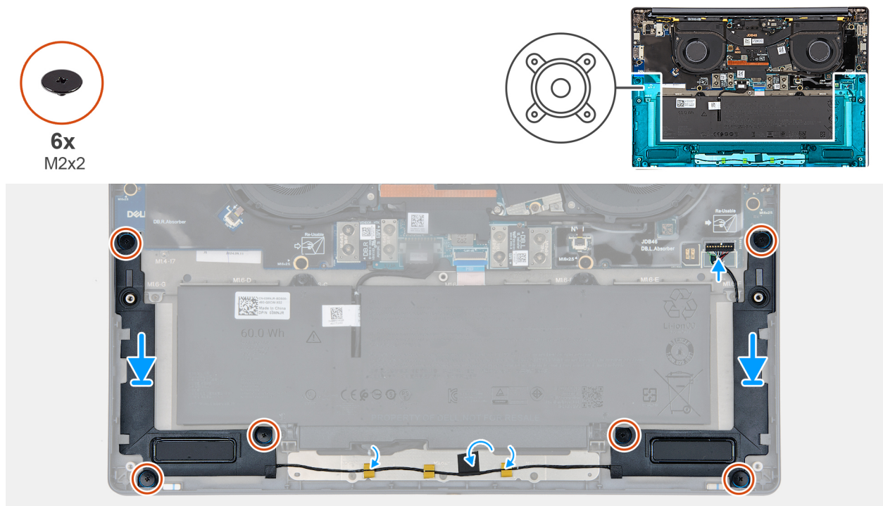
Figure 35. Installing the speakers (without WWAN)
