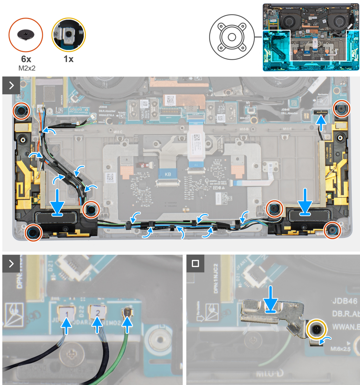
Figure 37. Installing the speakers with antennas (WWAN configuration)
