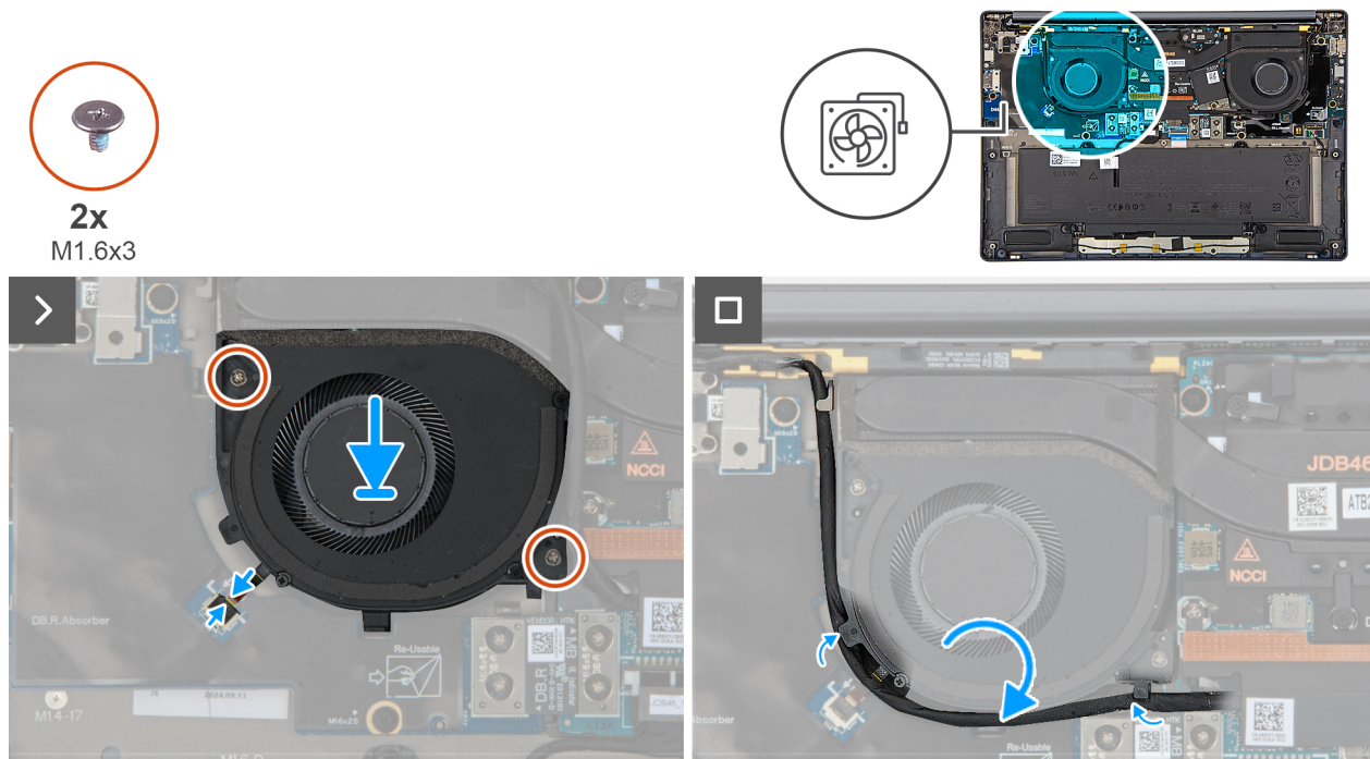
Figure 33. Installing the right fan
