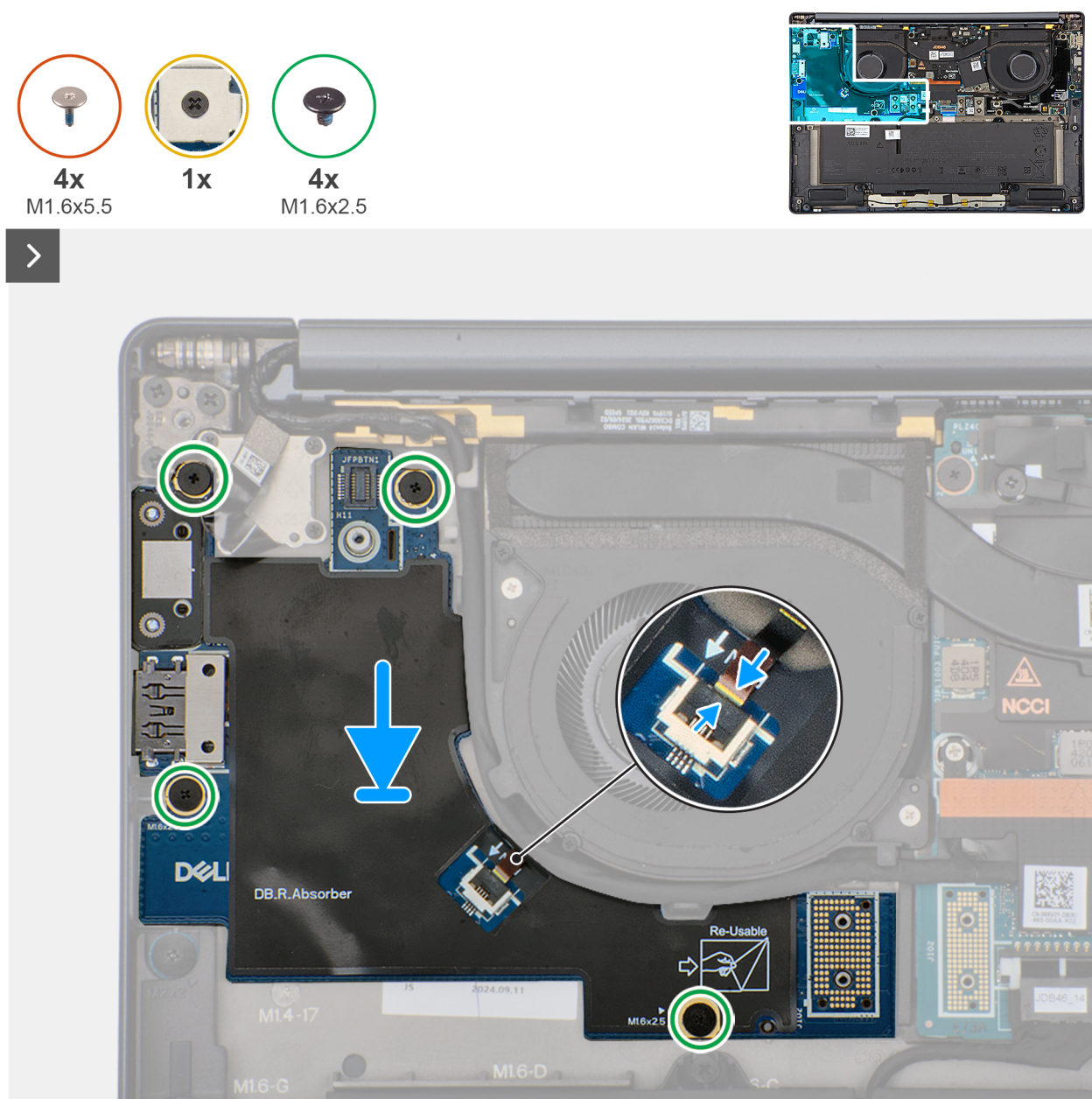
Figure 48. Installing the right I/O board (without WWAN antennas)
