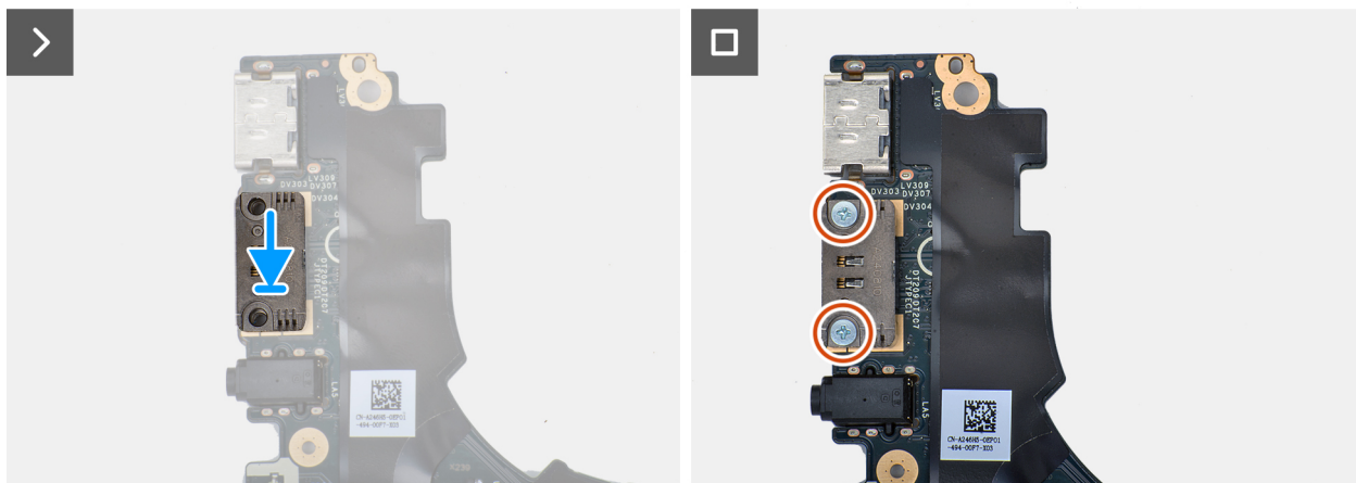
Figure 58. Removing the right USB Type-C module
