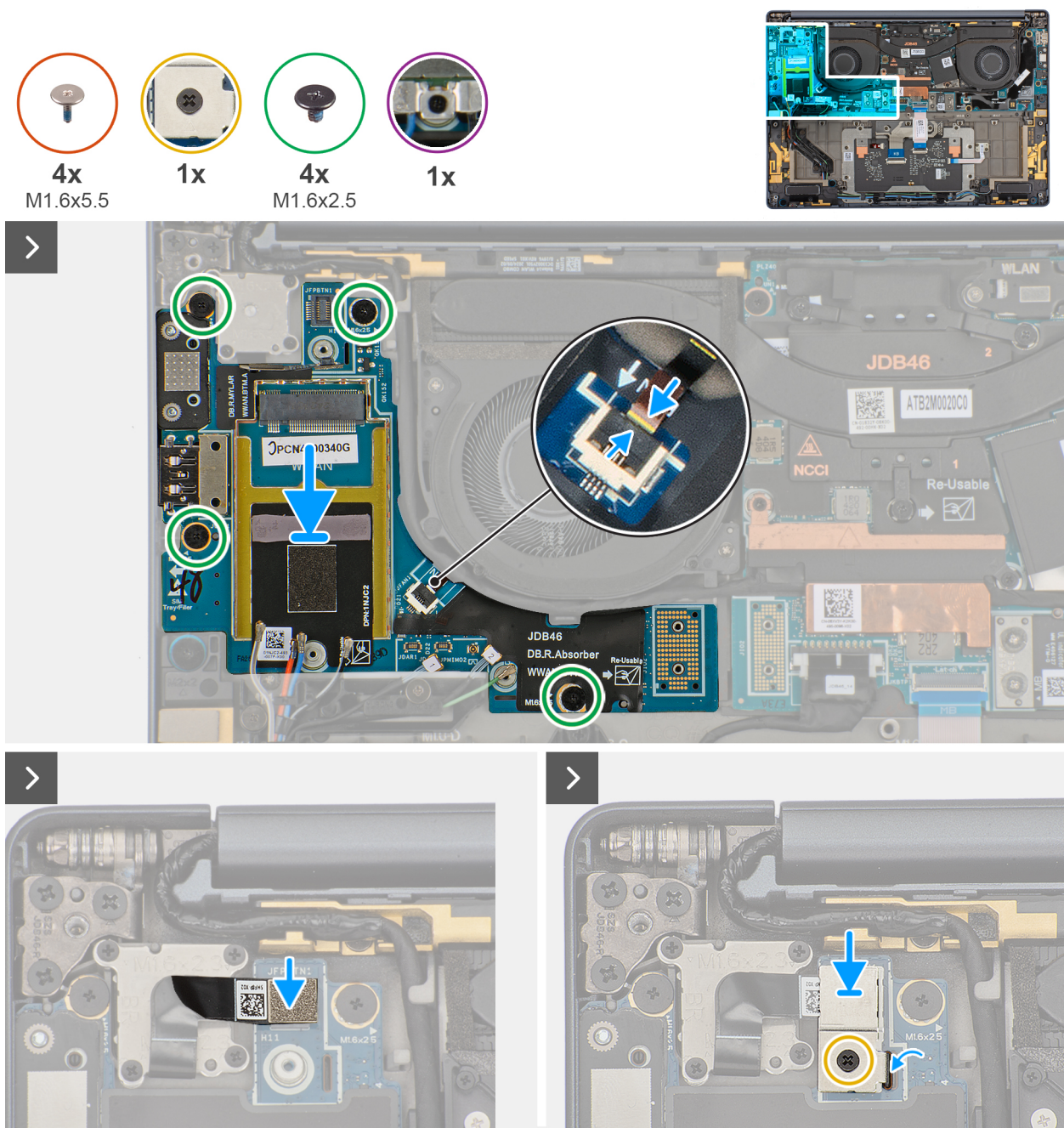
Figure 53. Installing the screws
