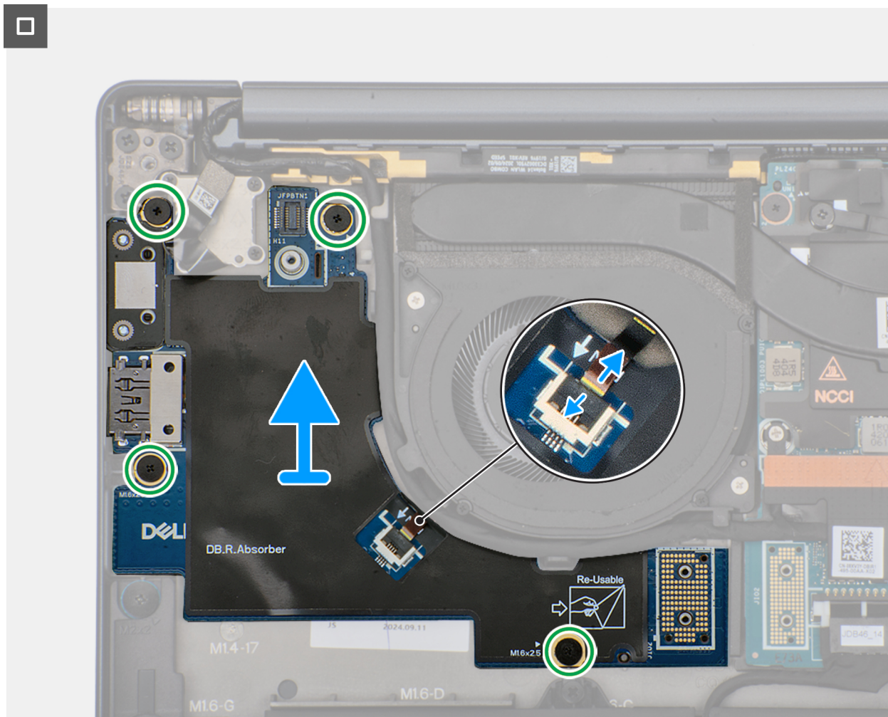
Figure 45. Removing the right I/O-board (without WWAN antennas)
