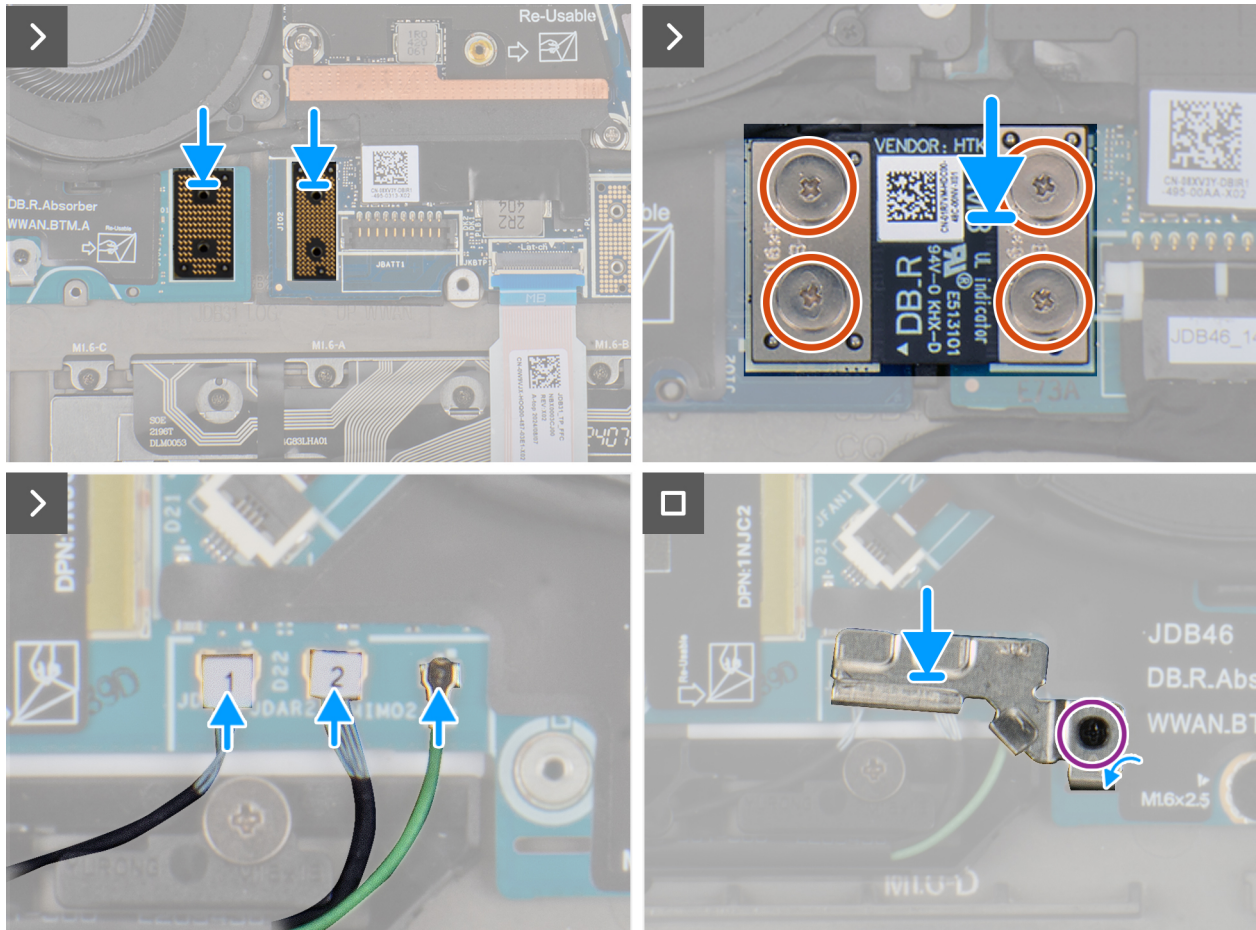
Figure 54. Installing the right I/O-board (with WWAN)
