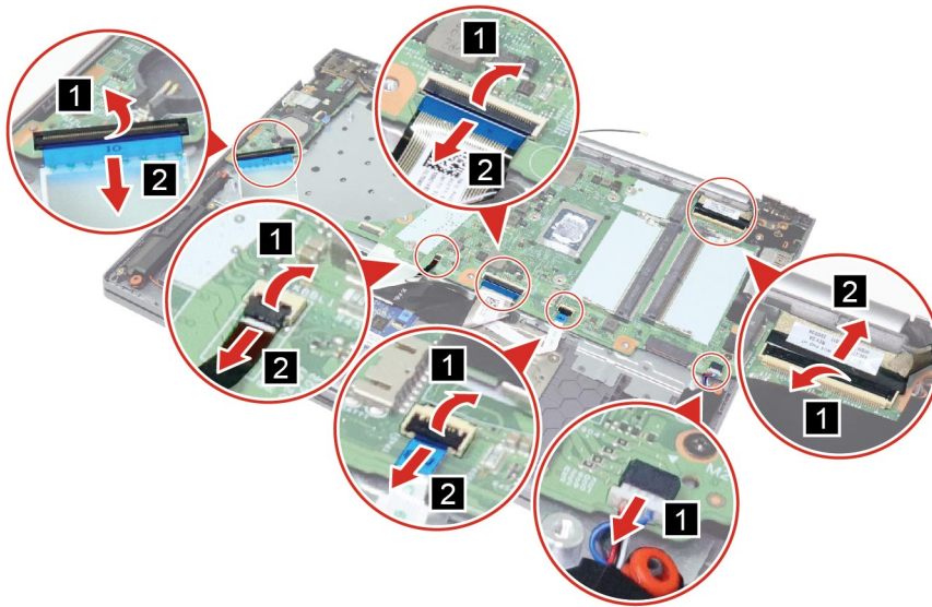
Figure 30. Disconnect cables
