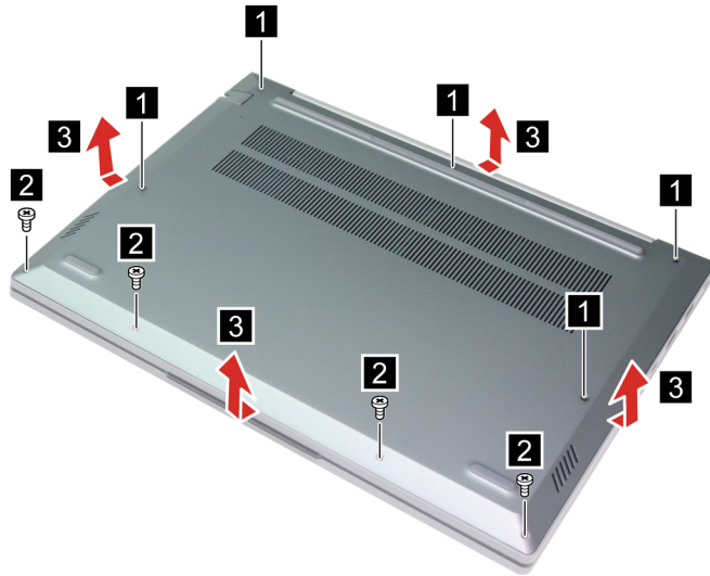
Figure 5. Loosen five screws, remove four screws and the lower case
