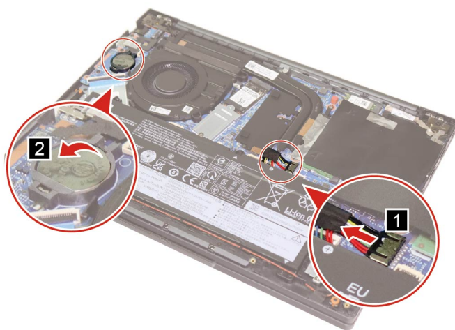
Figure 17. Remove the coin-cell battery
