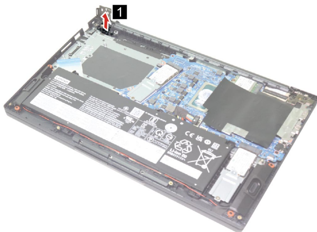
Figure 29. Remove the power button
