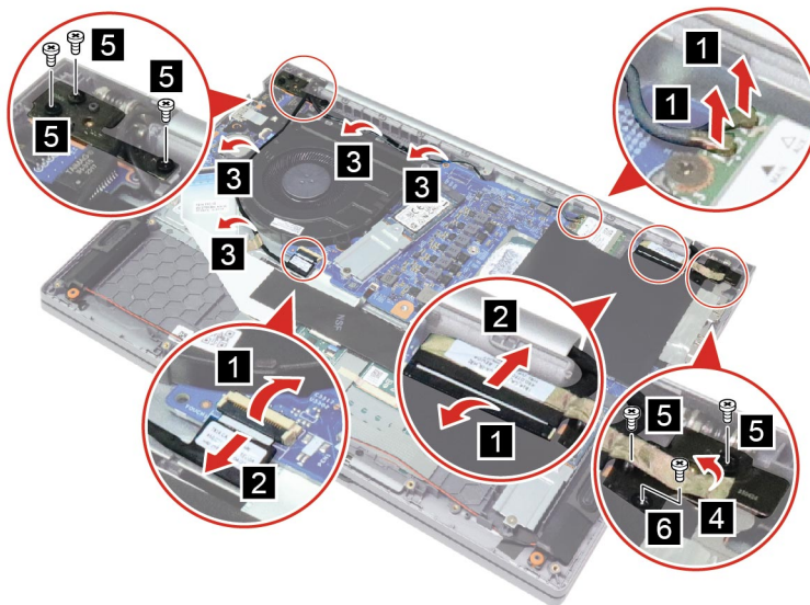
Figure 33. Disconnect cables and remove six screws
