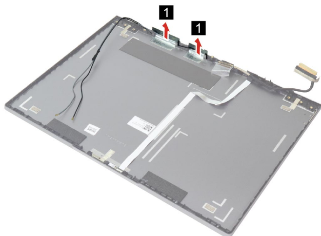
Figure 44. Remove the antennas
