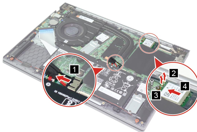
Figure 8. Remove the Wi-Fi card
