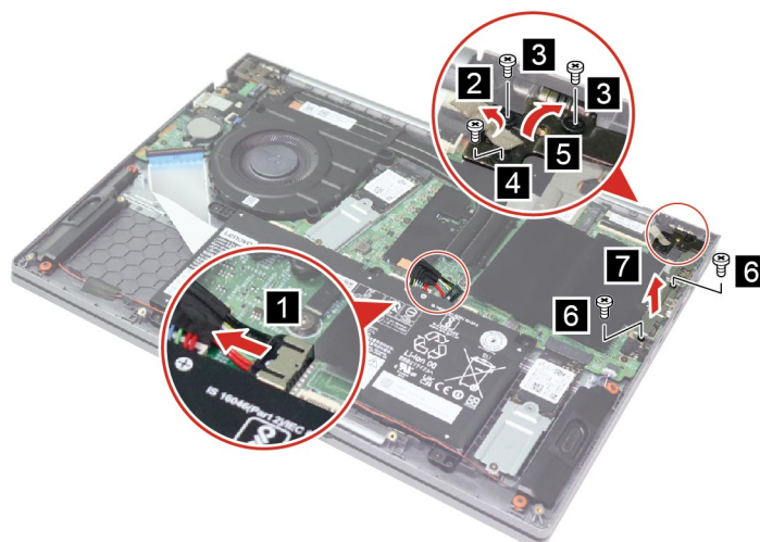
Figure 9. Remove the I/O bracket
