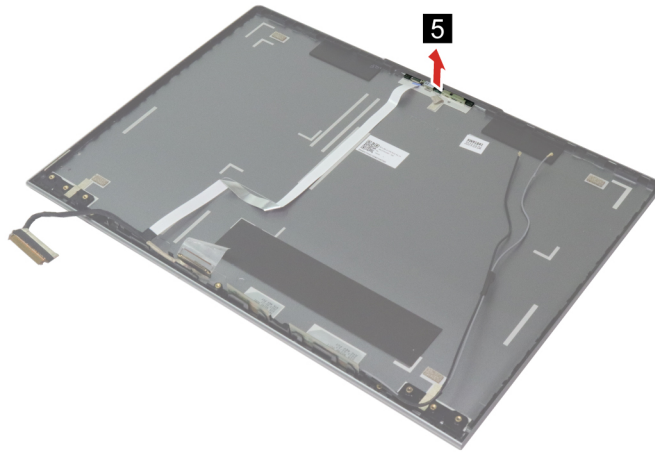
Figure 43. Remove the camera board
