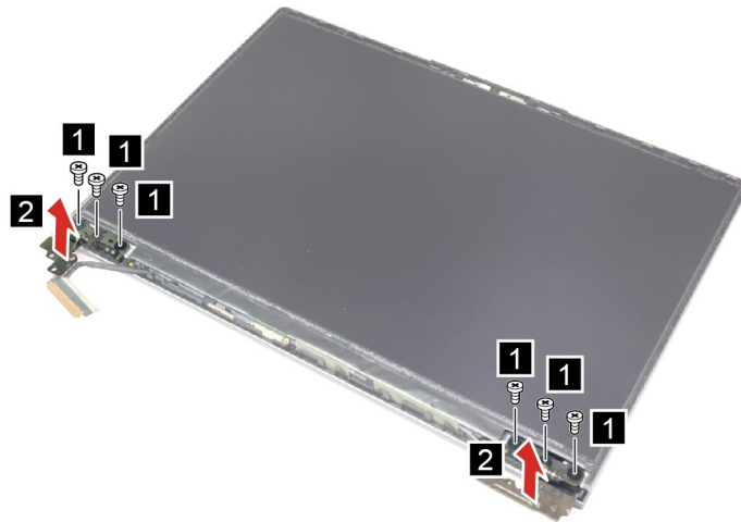
Figure 37. Remove six screws and remove the hinges
