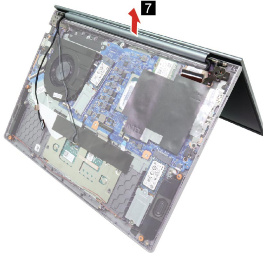
Figure 34. Rotate and remove LCD module
