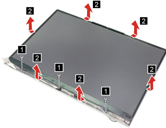
Figure 36. Remove three screws and remove the LCD bezel
