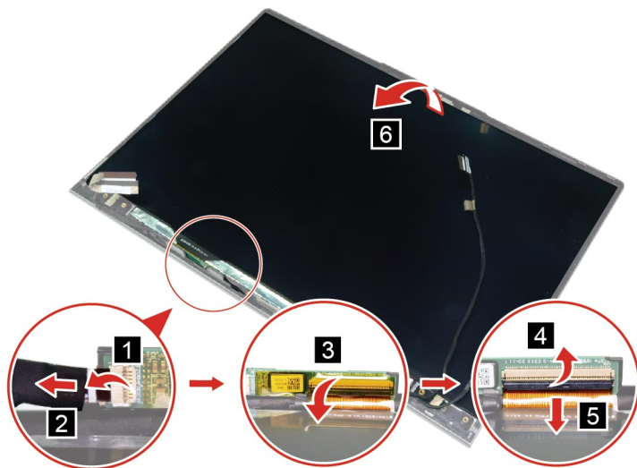
Figure 38. Disconnect the touch board and LCD panel cable
