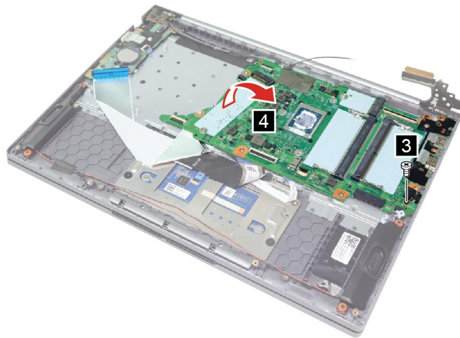
Figure 31. Remove one screw and remove the system board
