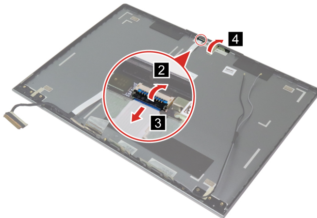
Figure 42. Disconnect the camera board cable
