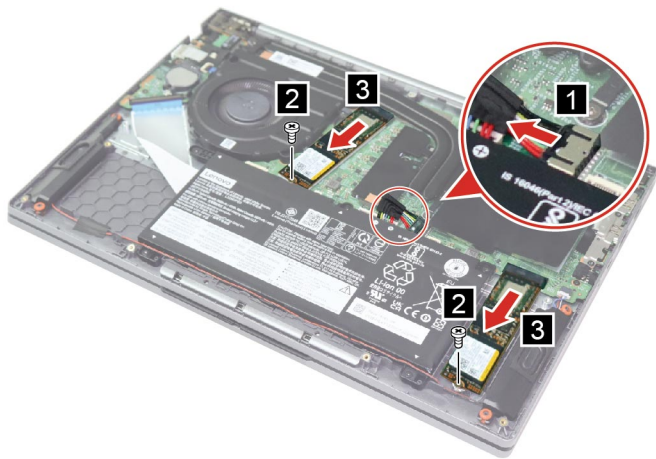
Figure 13. Remove the 2280 solid-state drives
