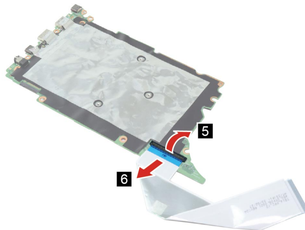
Figure 32. Disconnect the I/O board cable from the system board
