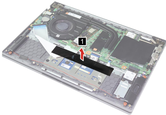
Figure 7. Remove the battery protective sponge
