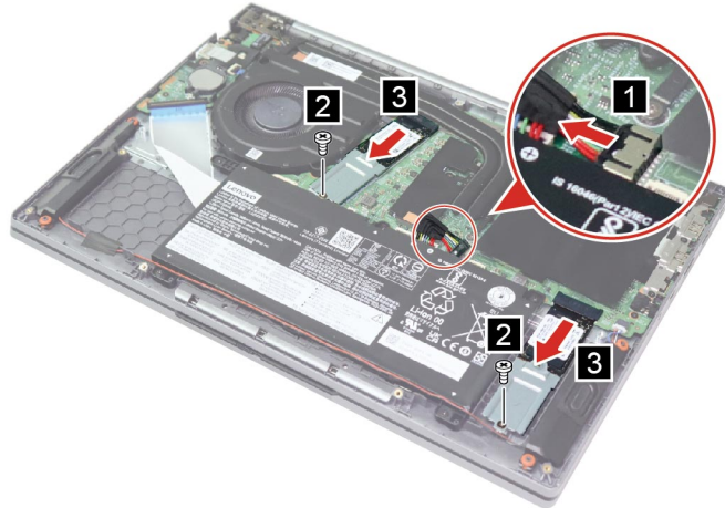
Figure 10. Remove the 2242 solid-state drives
