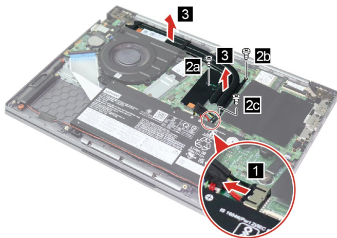
Figure 16. Remove three screws and remove the heat sink
