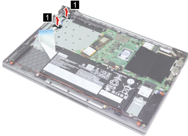
Figure 26. Remove the acetate tapes
