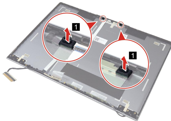
Figure 40. Remove the microphone rubbers
