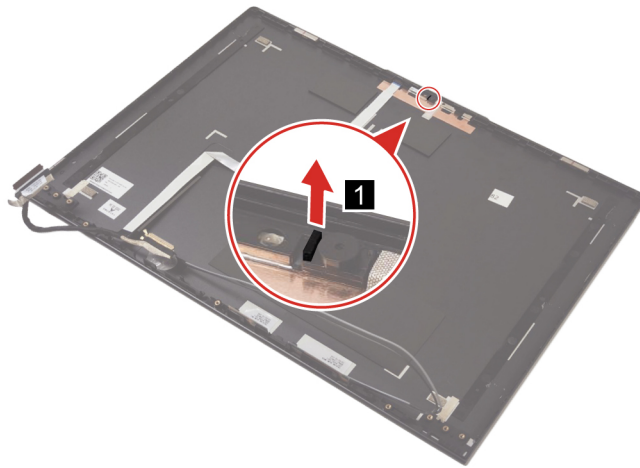
Figure 41. Remove the camera board sponge
