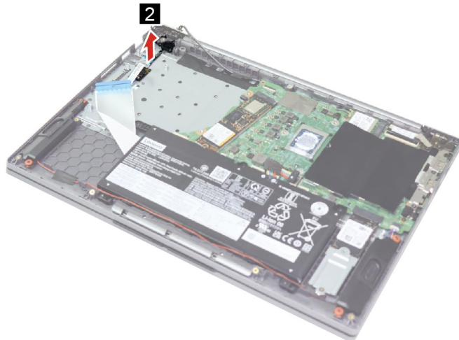
Figure 27. Remove the fingerprint reader module
