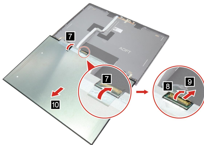
Figure 39. Peel back the camera board cable and EDP cables. Then, remove the LCD panel
