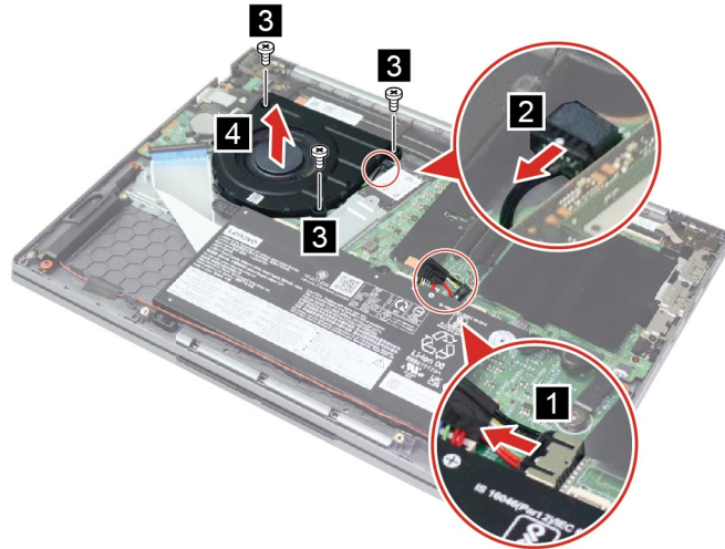
Figure 15. Remove three screws and the fan
