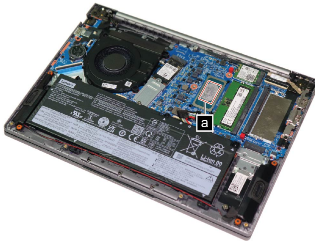
Figure 4. Area on the system board where thermal interface materials are applied
