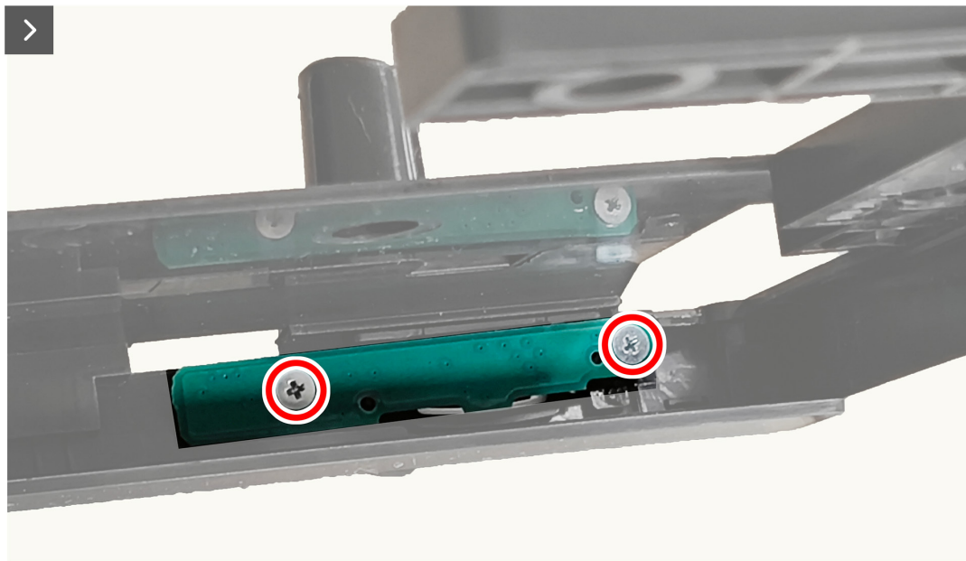
Figure 28. Removing the power-button board
