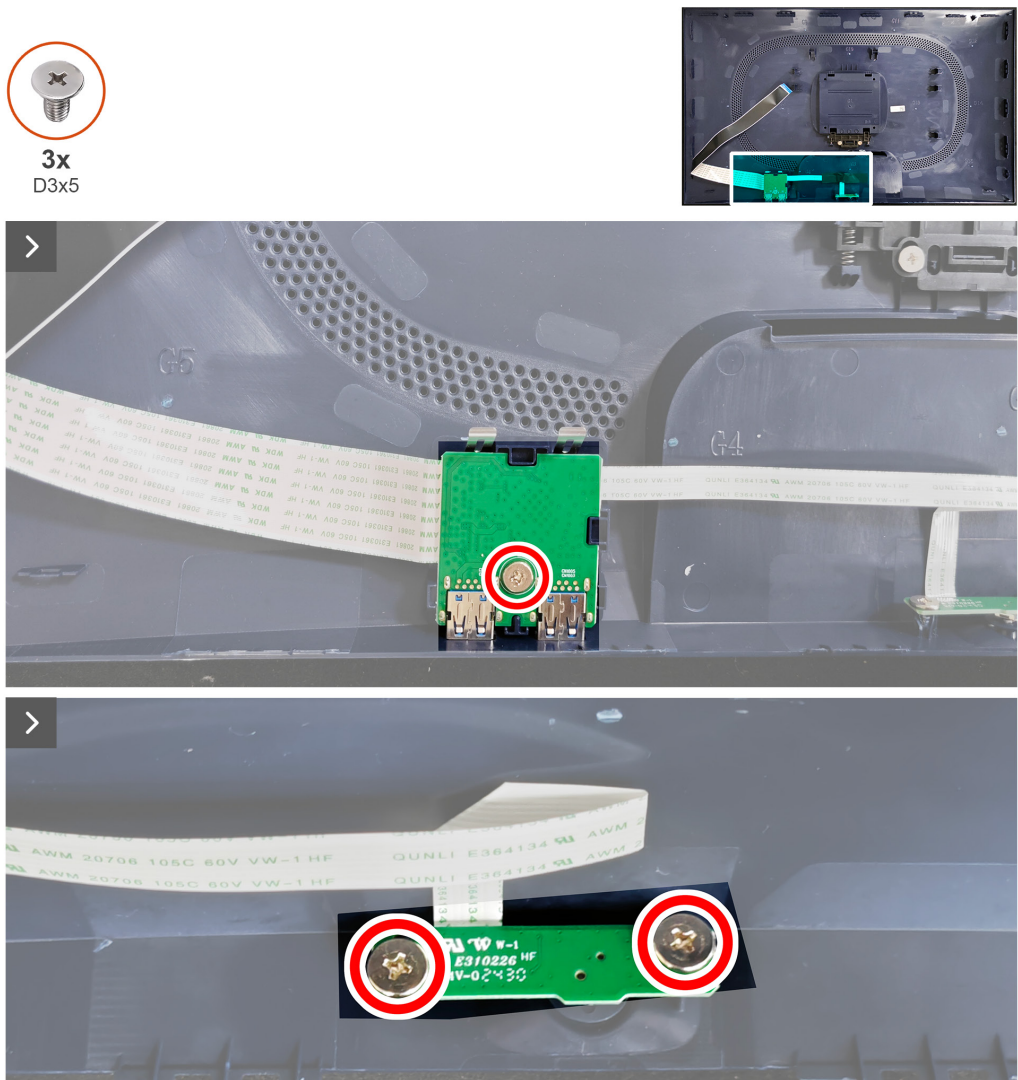
Figure 31. Removing the I/O board and joystick-button board
