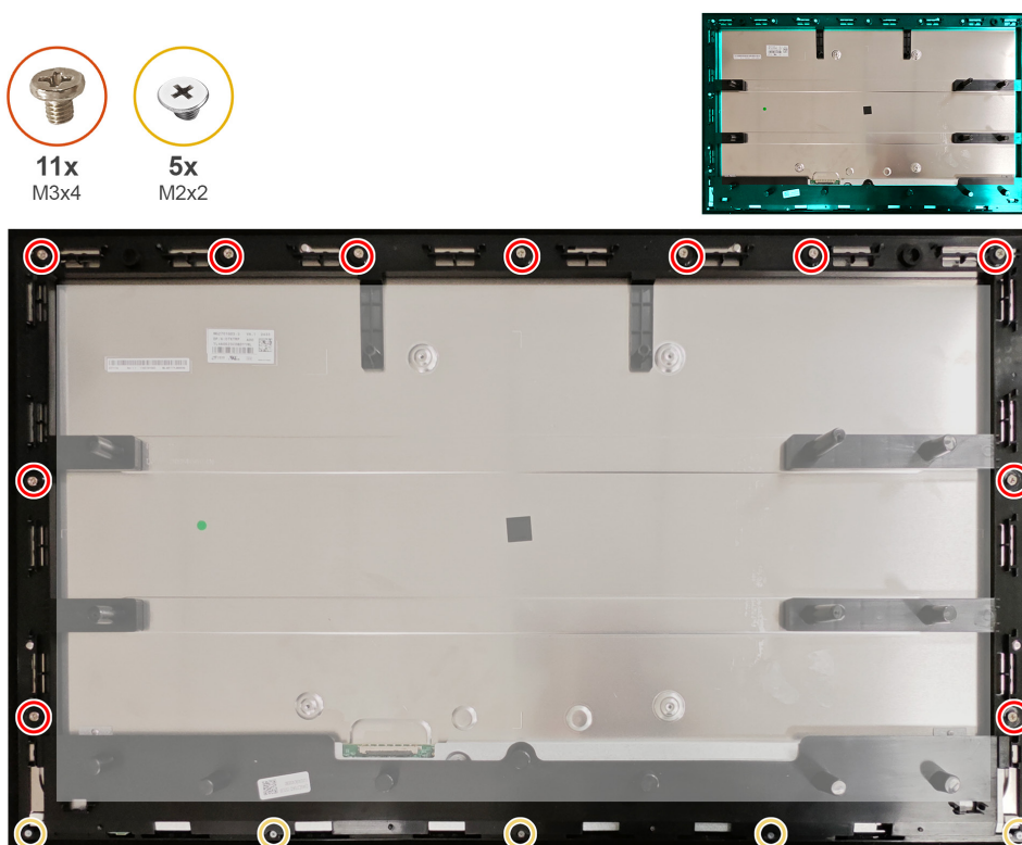
Figure 27. Installing the middle frame
