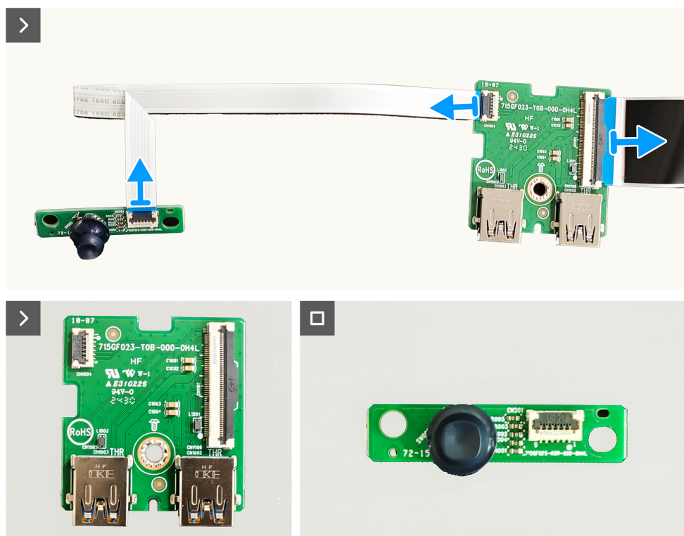
Figure 32. Removing the I/O board and joystick-button board
