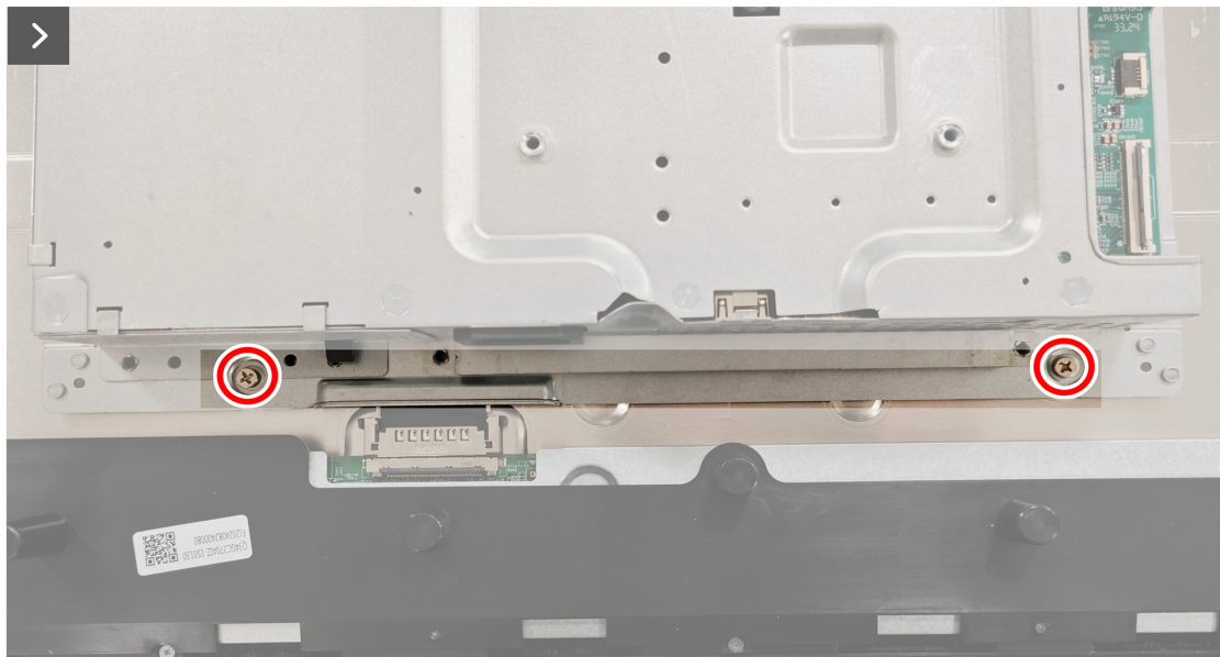
Figure 17. Installing the metal shield
