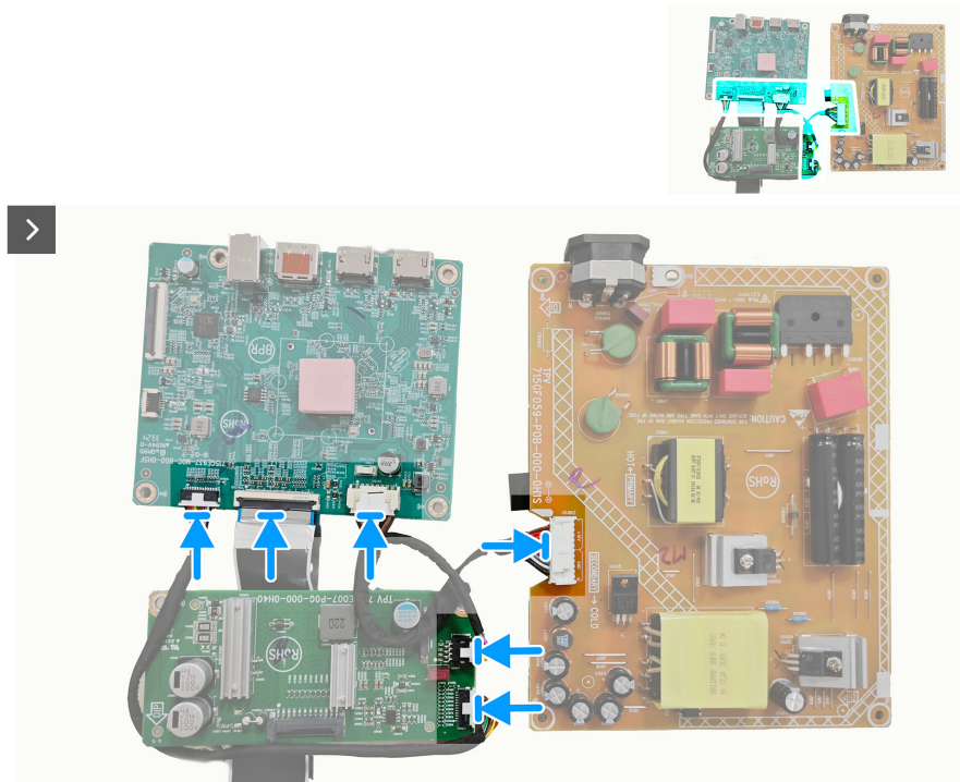
Figure 23. Installing the system board and power board
