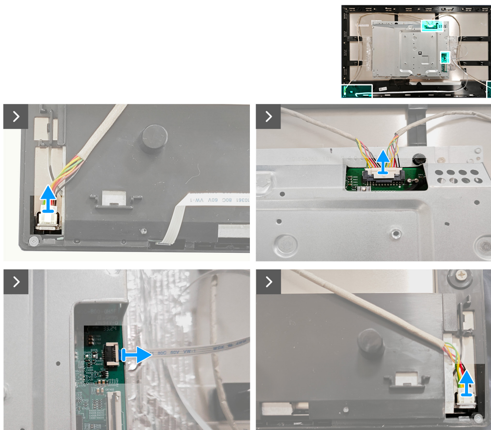
Figure 11. Removing the metal shield
