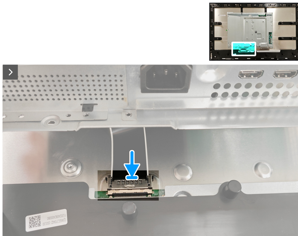
Figure 15. Installing the metal shield
