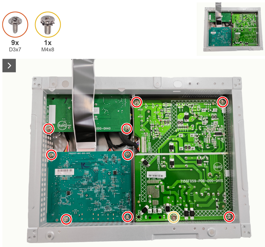
Figure 24. Installing the system board and power board
