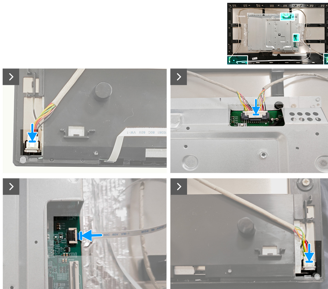
Figure 18. Installing the metal shield
