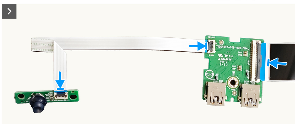
Figure 33. Installing the I/O board and joystick-button board
