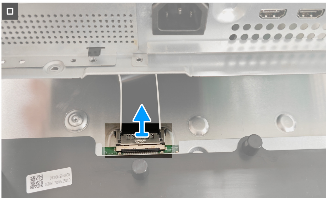
Figure 14. Removing the metal shield
