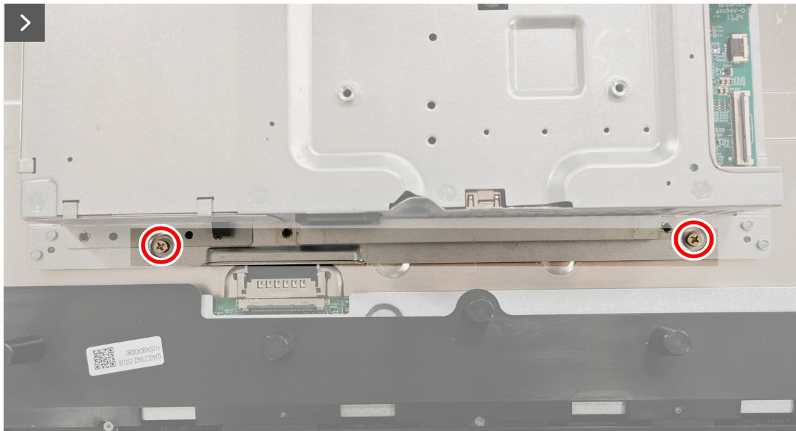
Figure 13. Removing the metal shield
