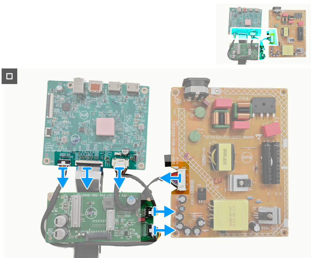
Figure 22. Removing the system board and power board
