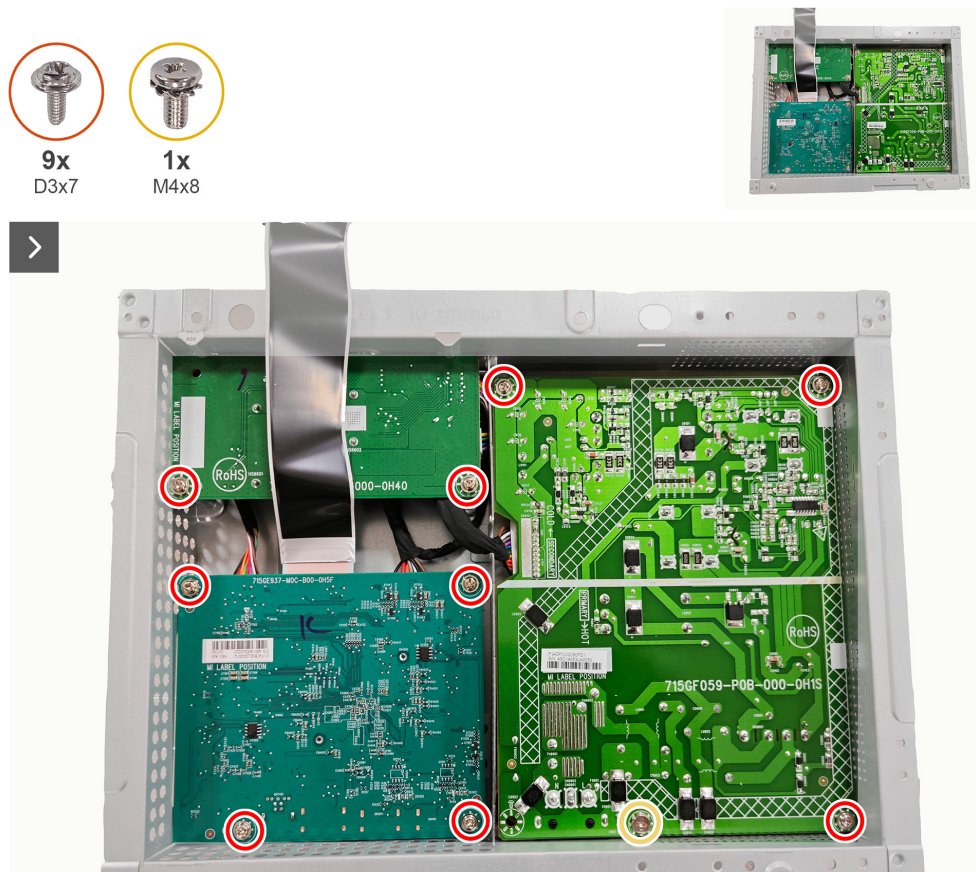
Figure 21. Removing the system board and power board
