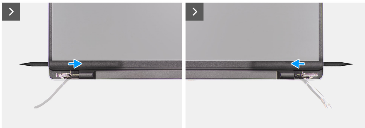
Figure 60. Removing the display bezel
