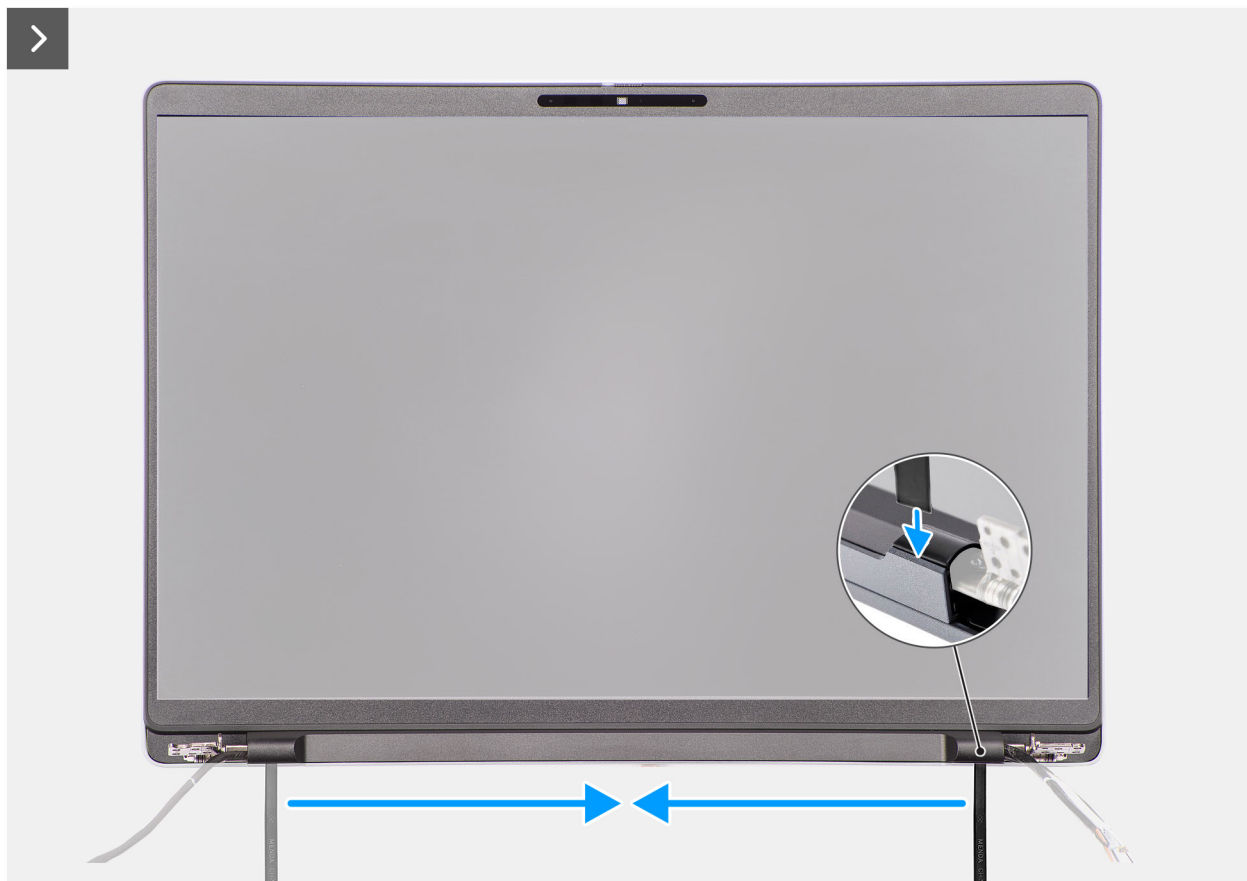
Figure 59. Removing the display bezel
