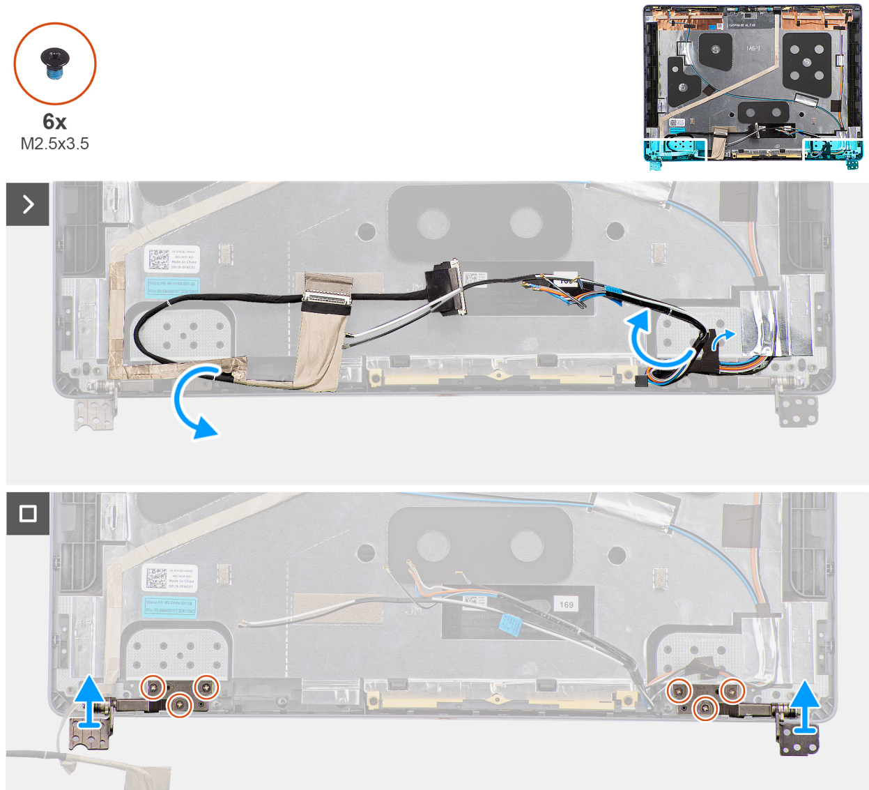
Figure 70. Removing the display hinges
