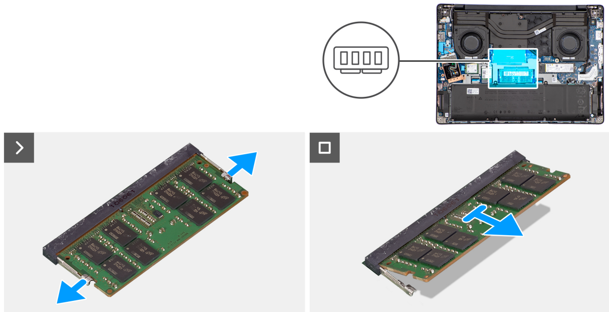
Figure 19. Removing the memory module
