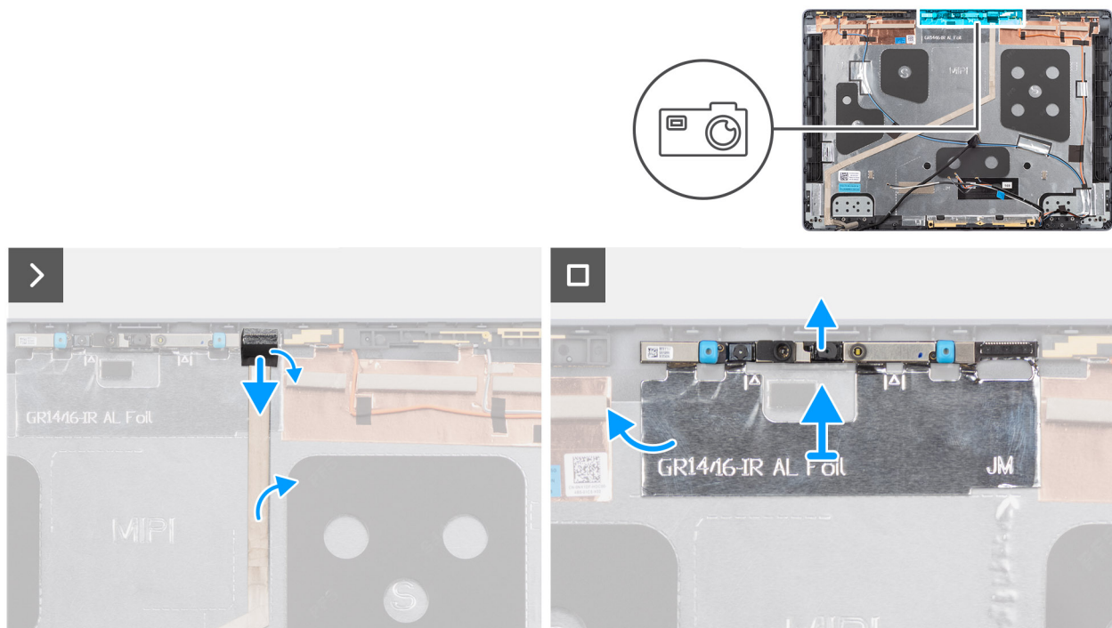
Figure 74. Removing the camera
