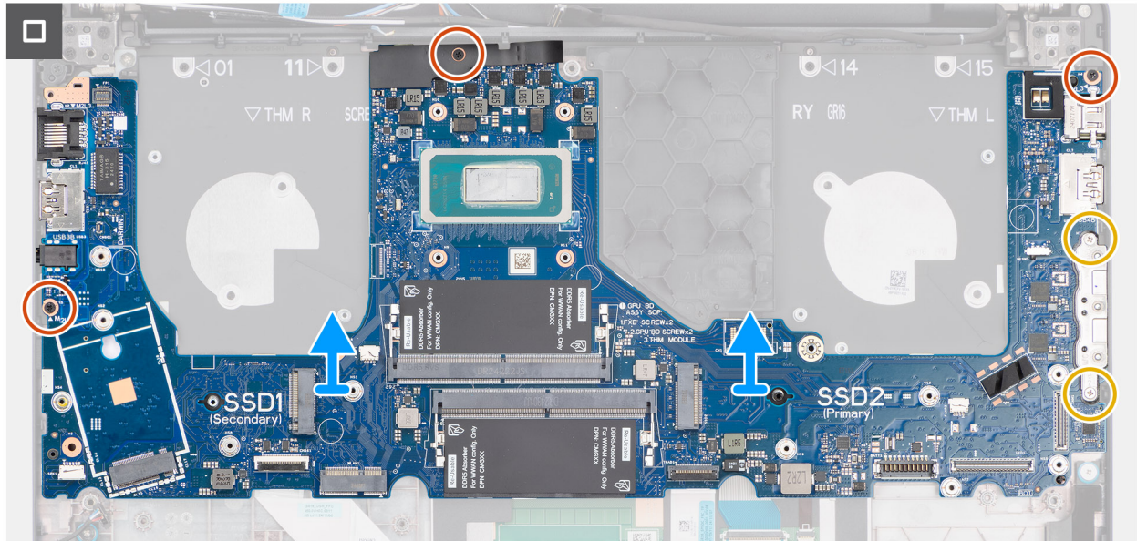
Figure 80. Removing the system board
