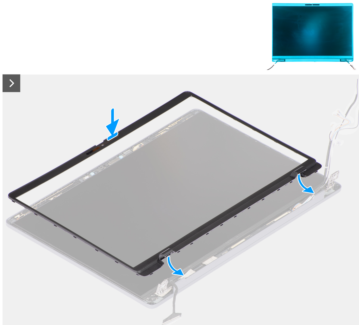
Figure 62. Installing the display bezel
