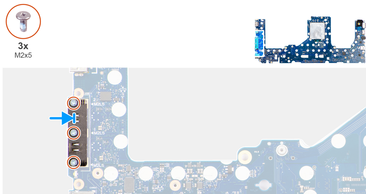
Figure 85. Installing the USB Type-C module
