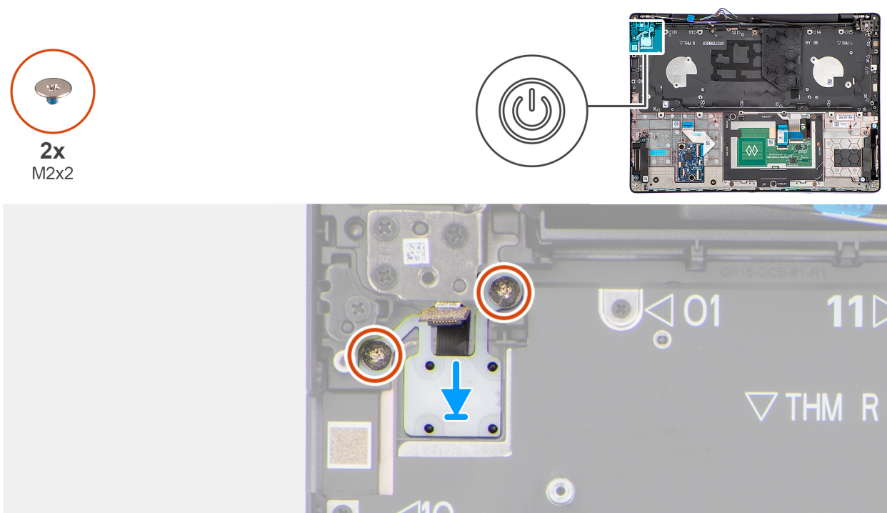
Figure 87. Installing the power button
