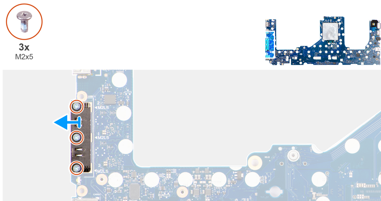
Figure 84. Removing the USB Type-C module
