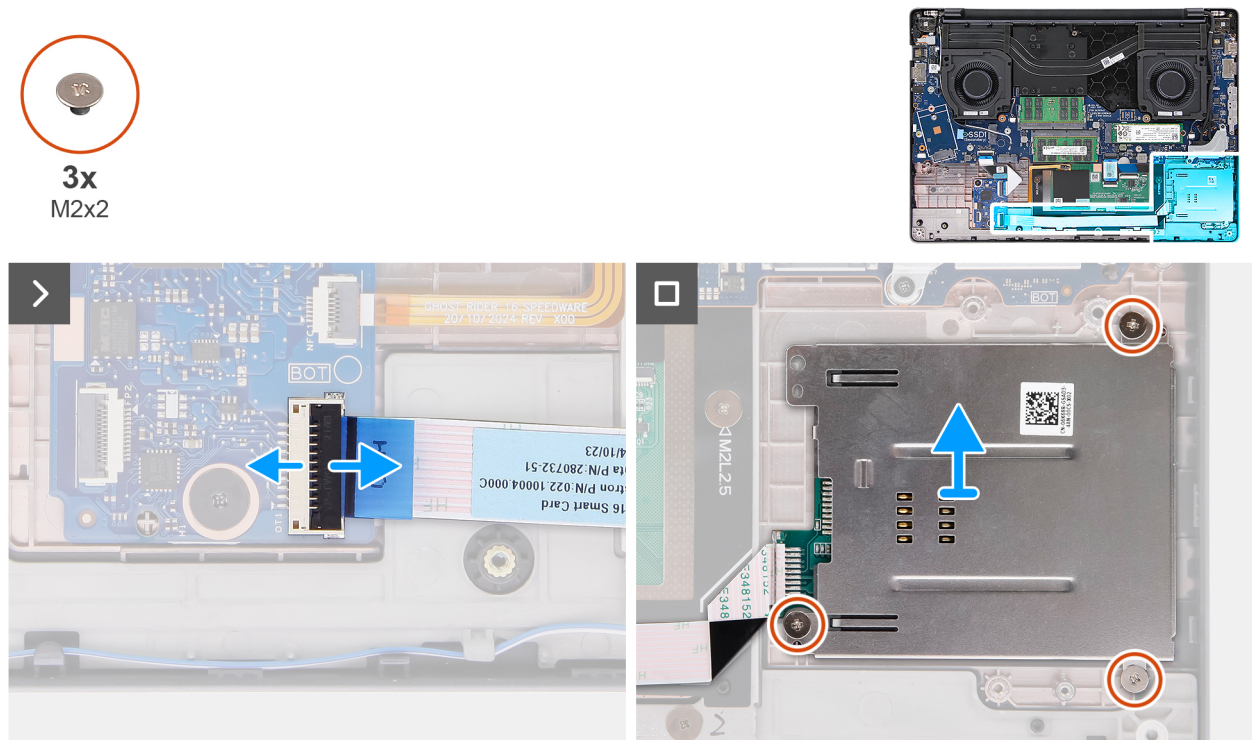
Figure 48. Removing the smart-card reader
