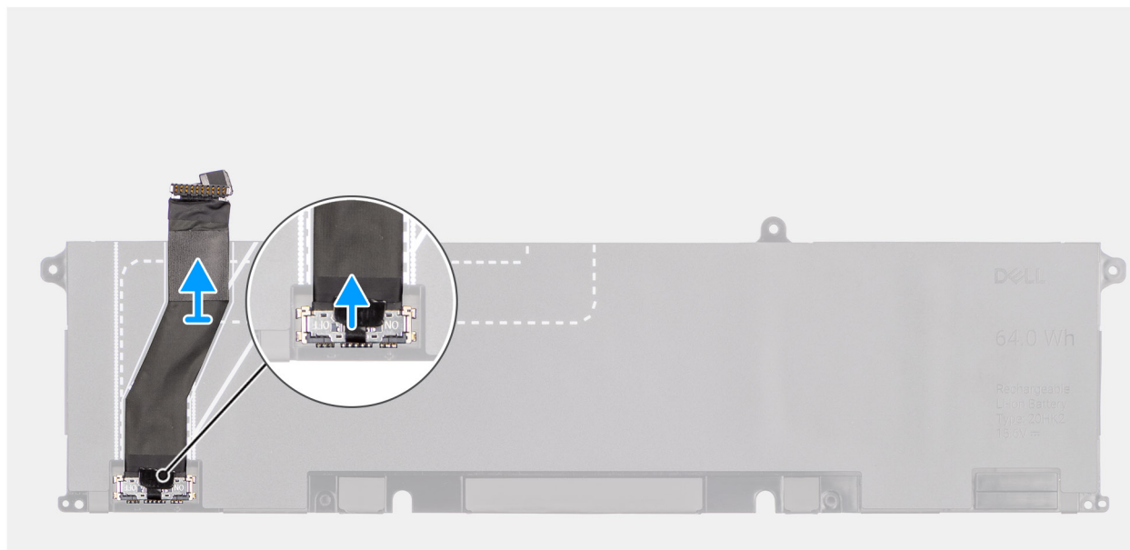
Figure 38. Disconnecting the battery cable
