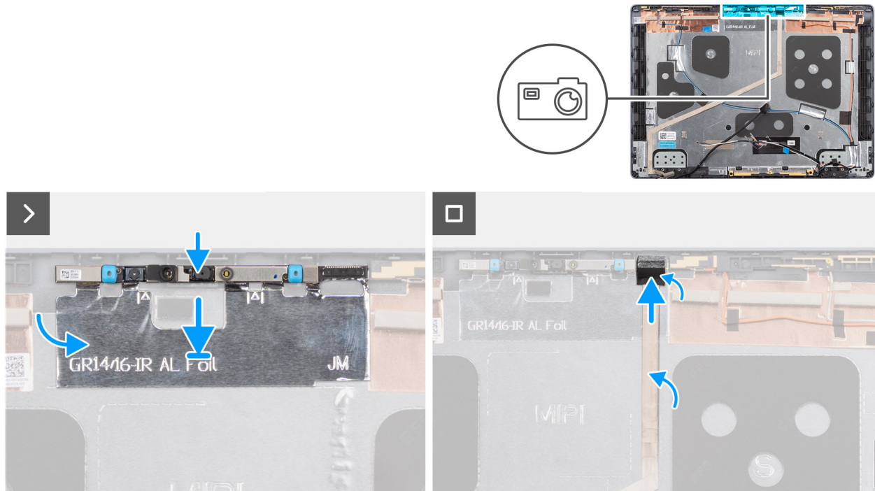
Figure 75. Installing the camera
