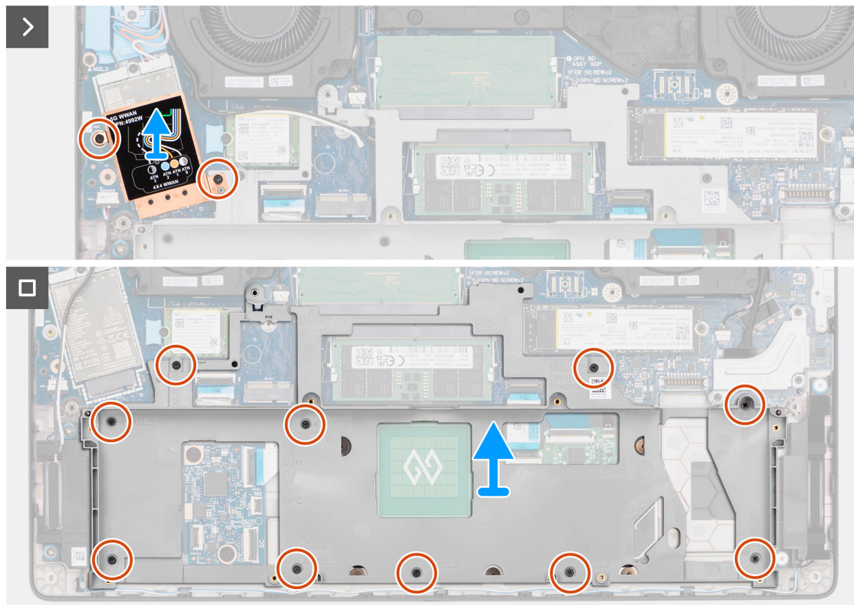
Figure 44. Removing the battery frame
