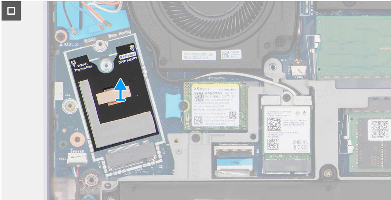
Figure 28. Removing the WWAN module
