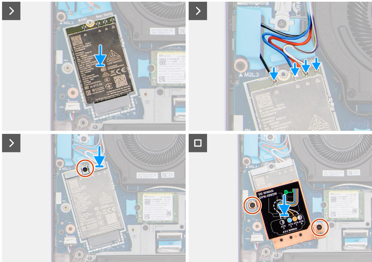
Figure 30. Installing the WWAN module
