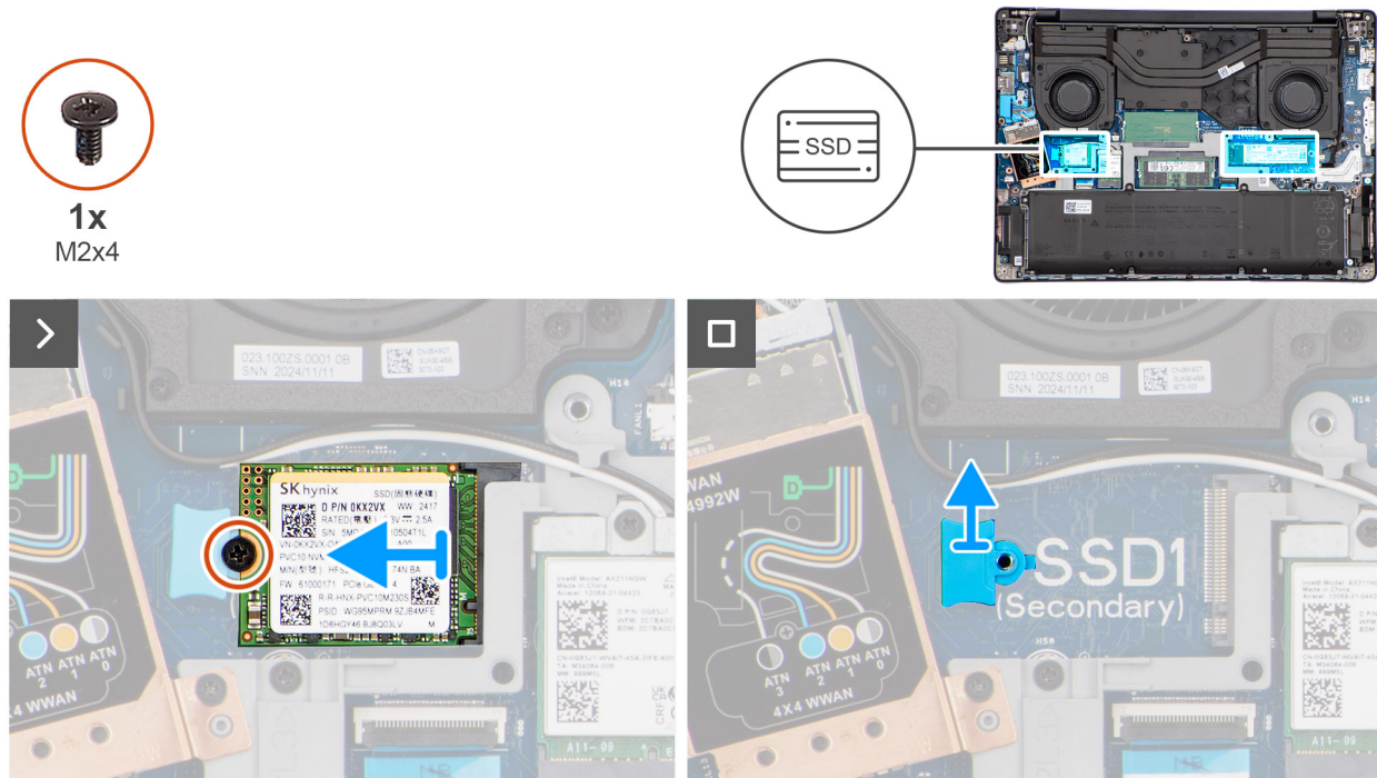
Figure 21. Removing the M.2 2230 solid state drive
