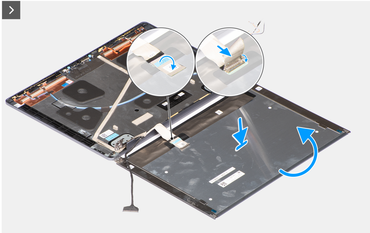
Figure 68. Installing the display panel
