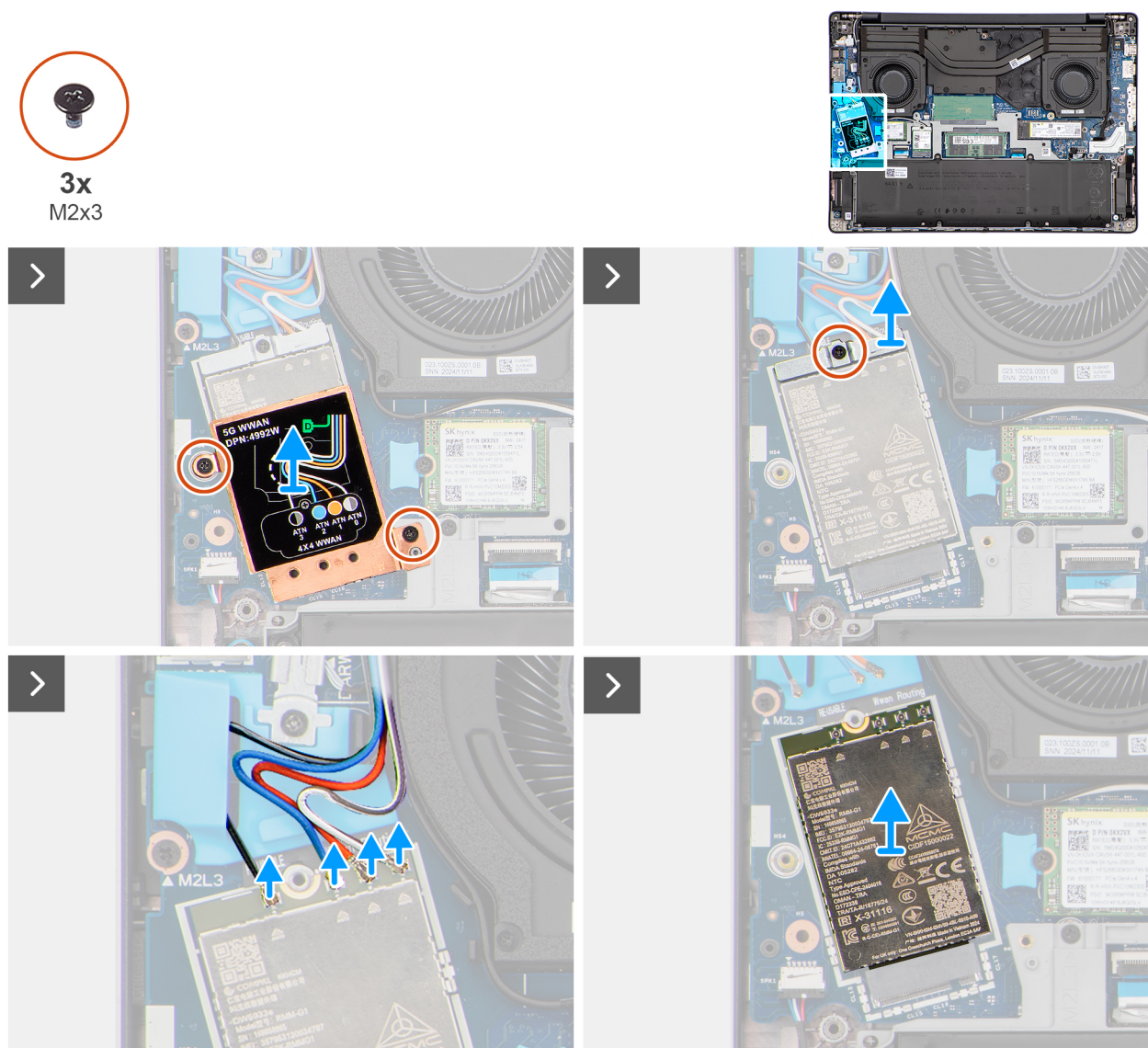
Figure 27. Removing the WWAN module
