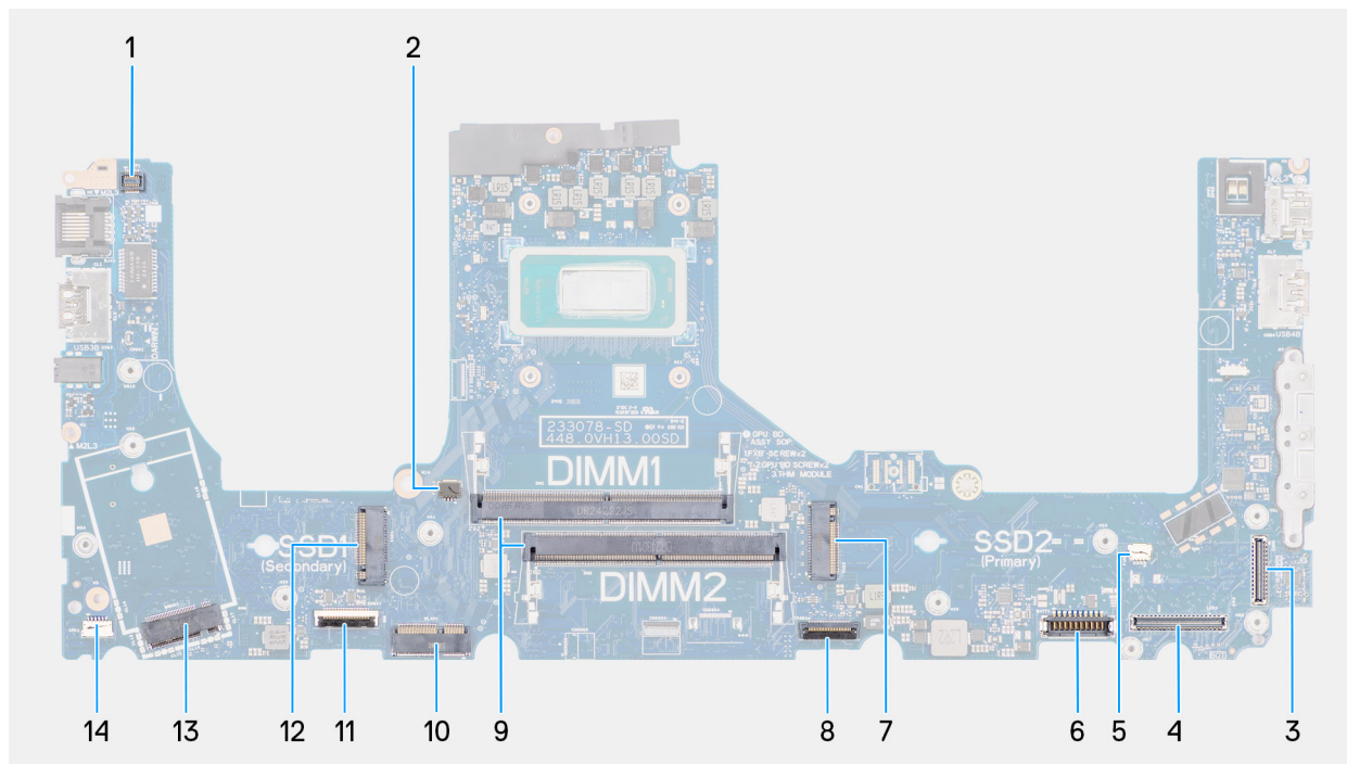
Figure 81. System board connectors
