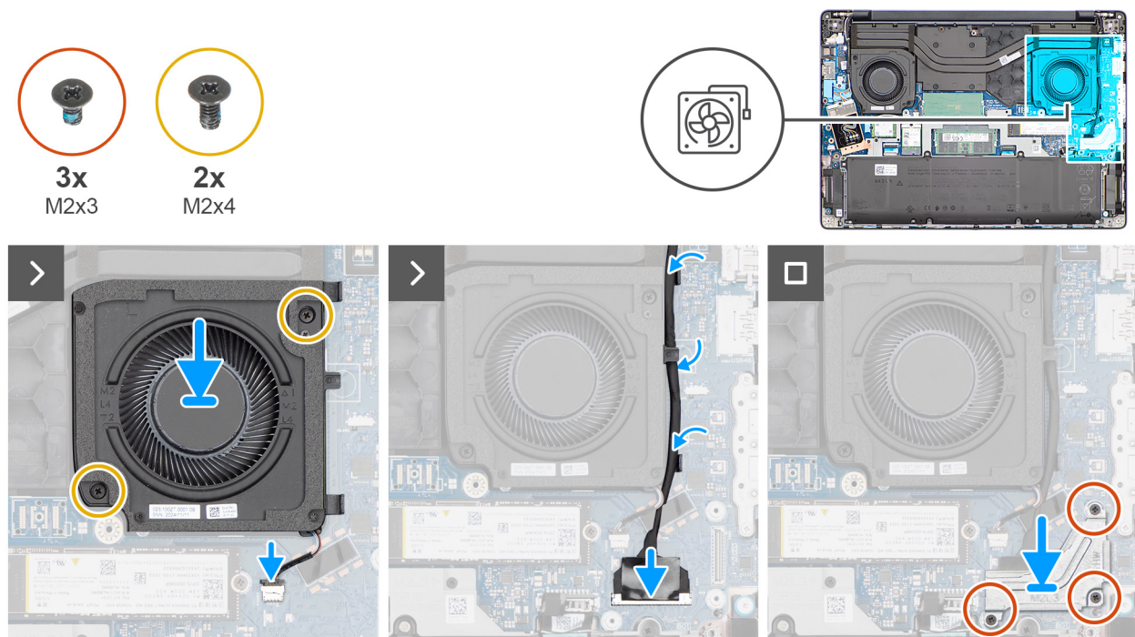
Figure 37. Installing the left/video fan
