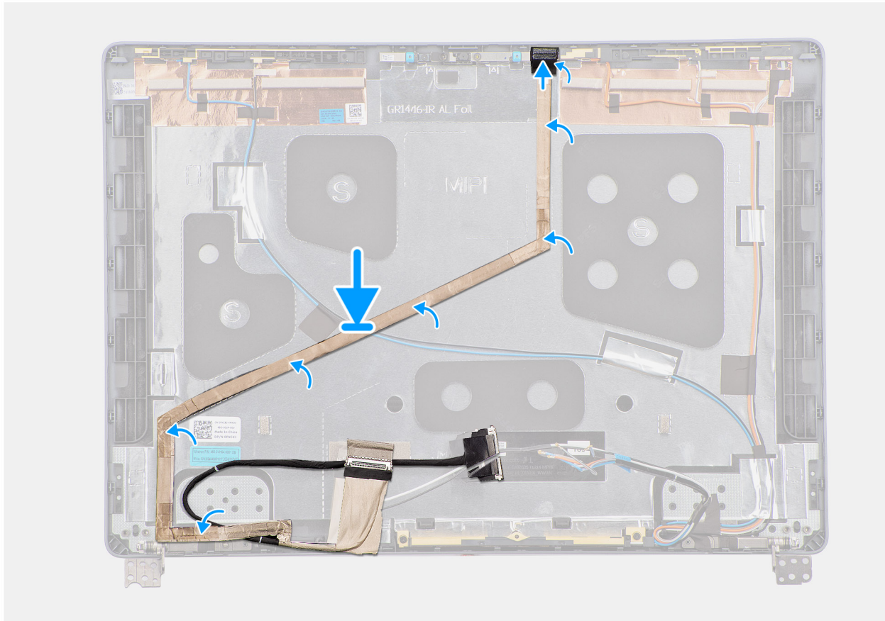
Figure 73. Installing the display cable
