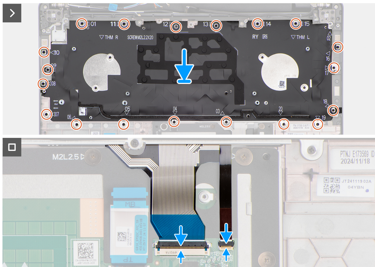
Figure 91. Installing the keyboard
