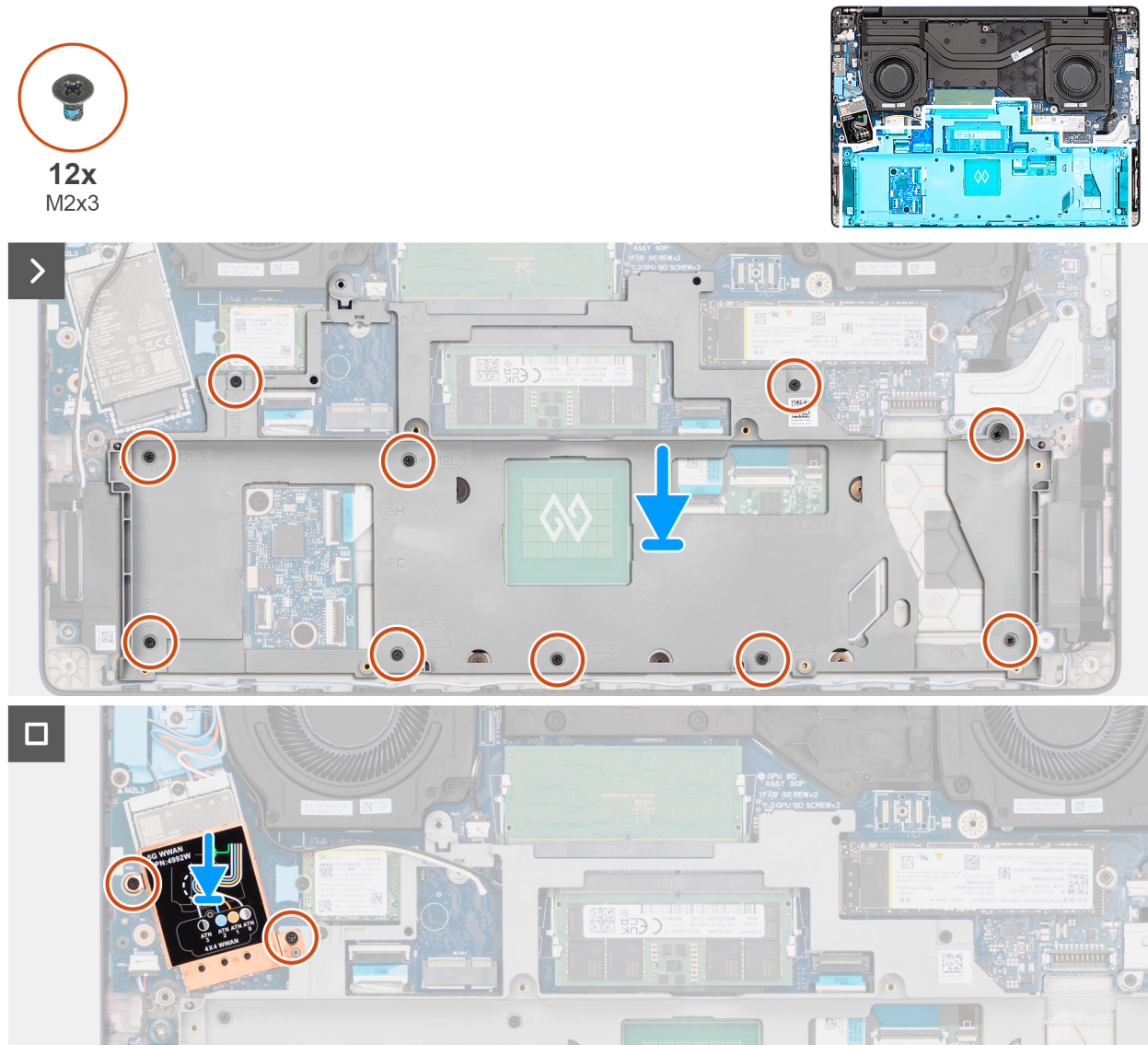
Figure 45. Installing the battery frame
