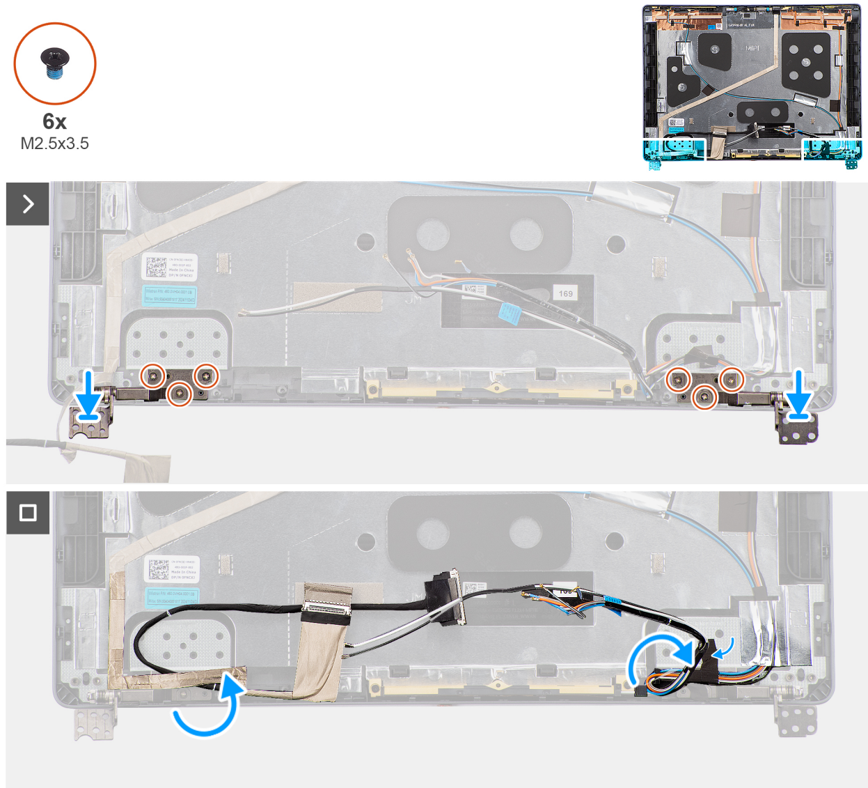
Figure 71. Installing the display hinges
