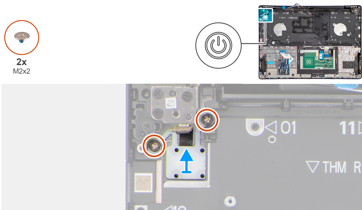
Figure 86. Removing the power button
