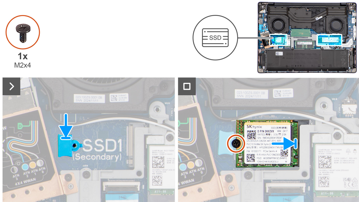
Figure 22. Installing the M.2 2230 solid state drive
