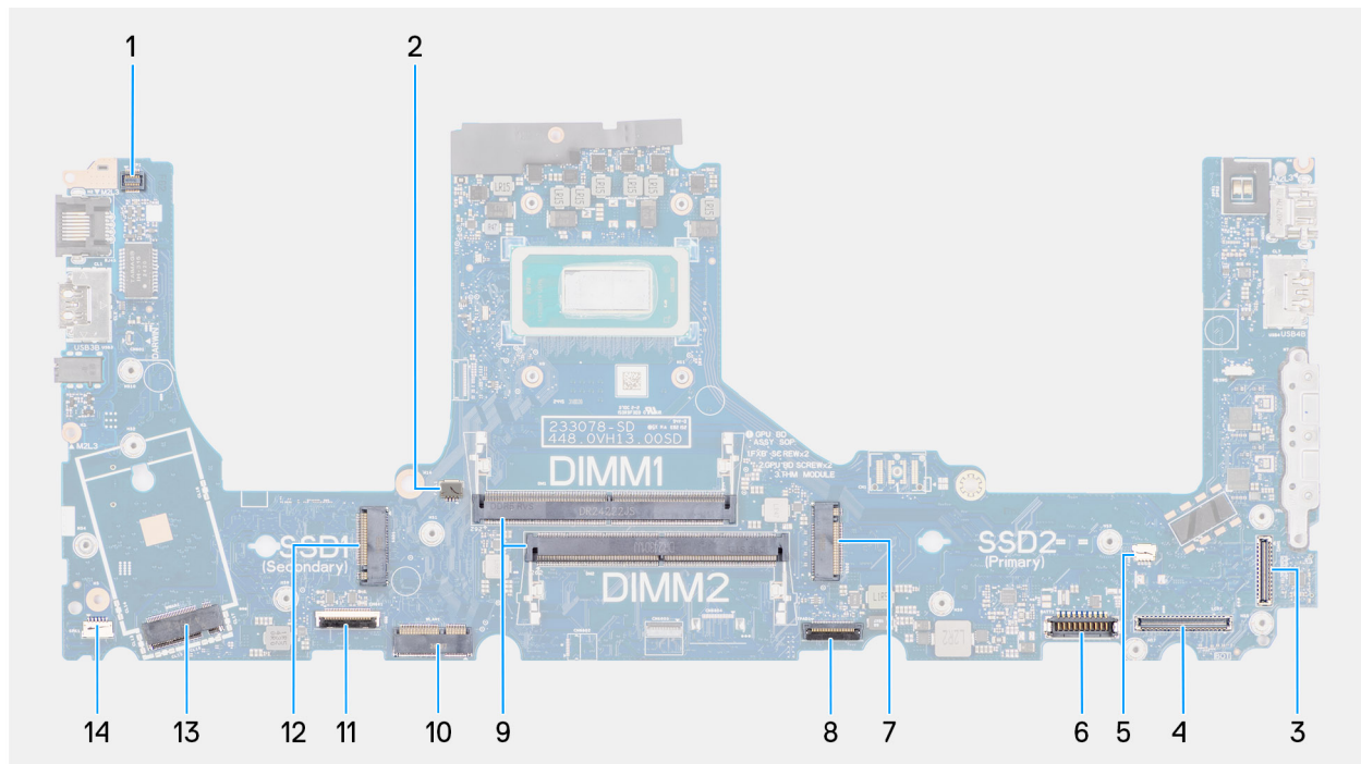
Figure 78. System board connectors
