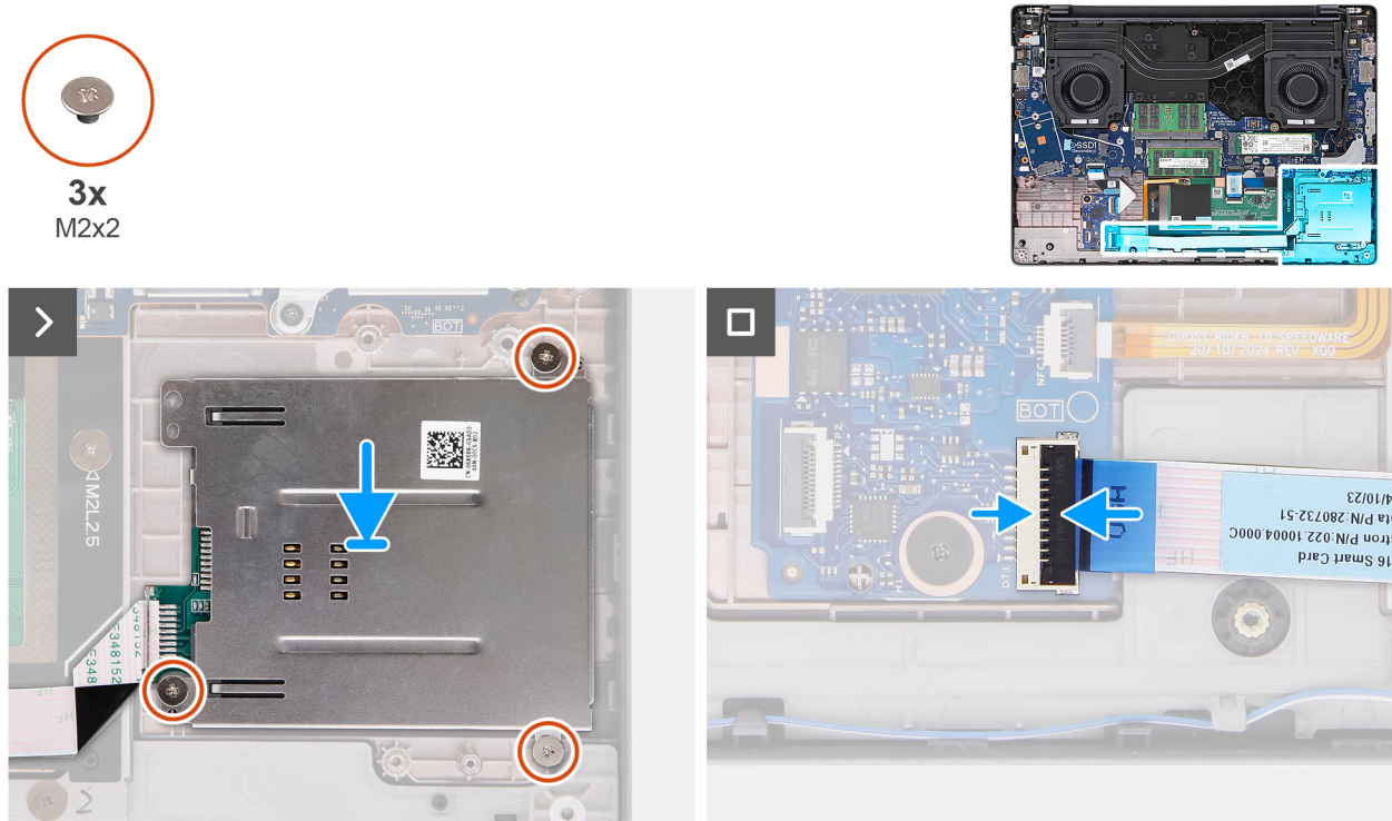
Figure 49. Installing the smart-card reader
