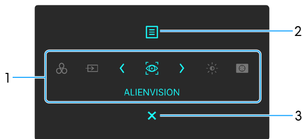
Figure 36. Menu Launcher
