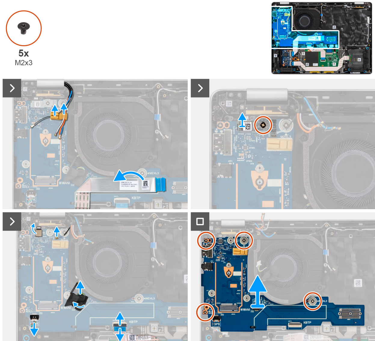
Figure 52. Removing the I/O board
