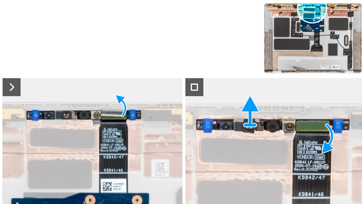
Figure 76. Removing the MIPI camera
