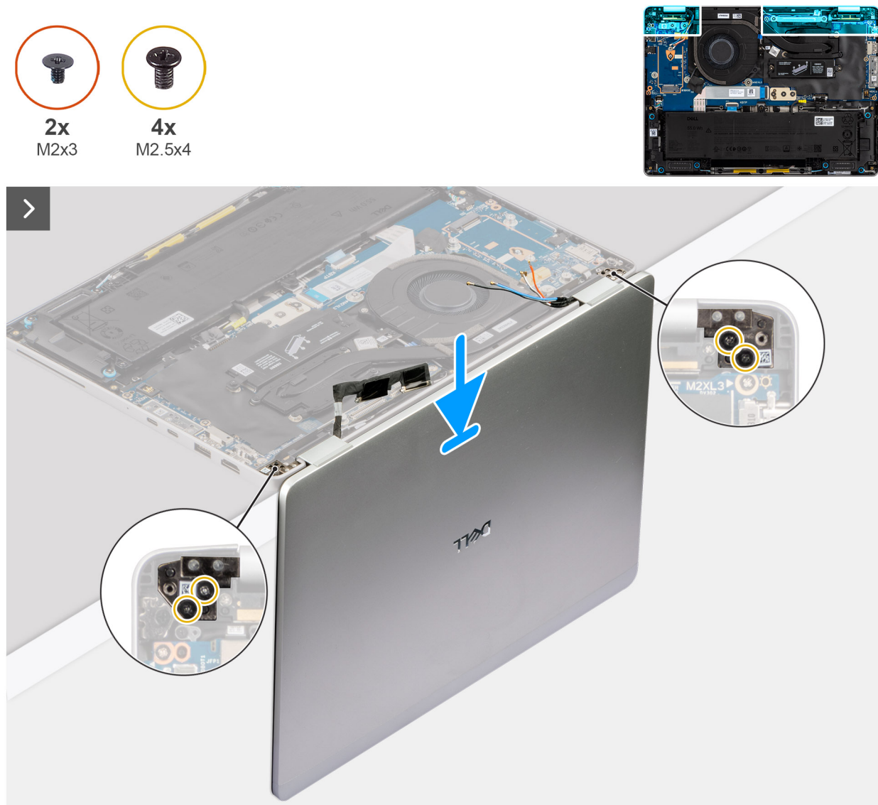
Figure 58. Installing the display assembly
