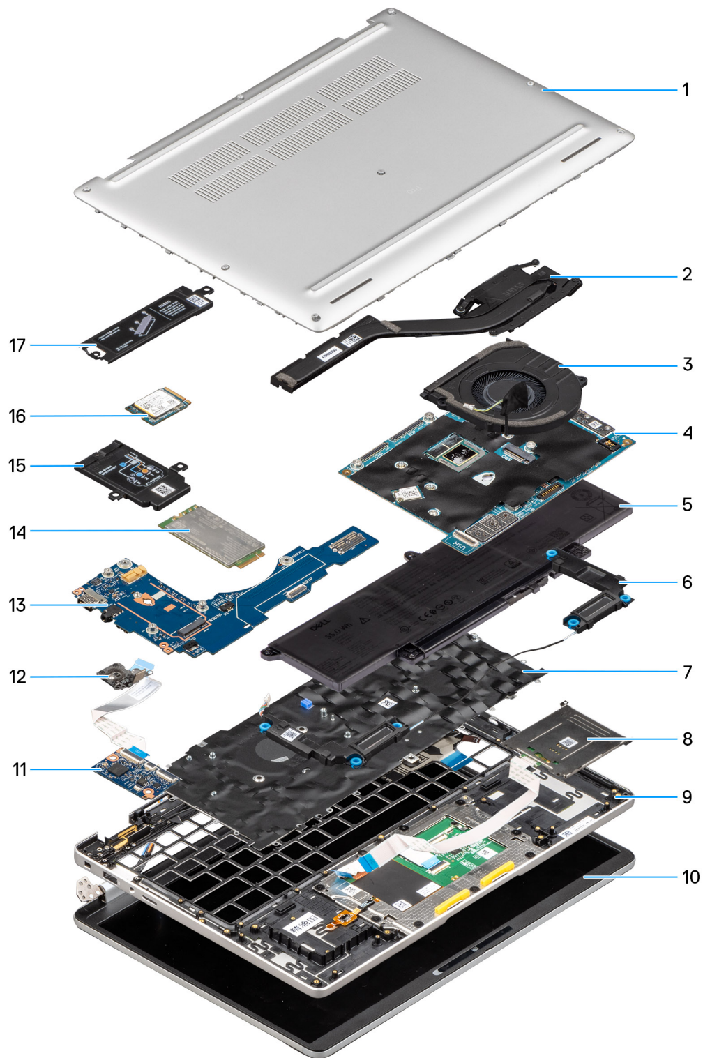
Figure 18. Explode view
