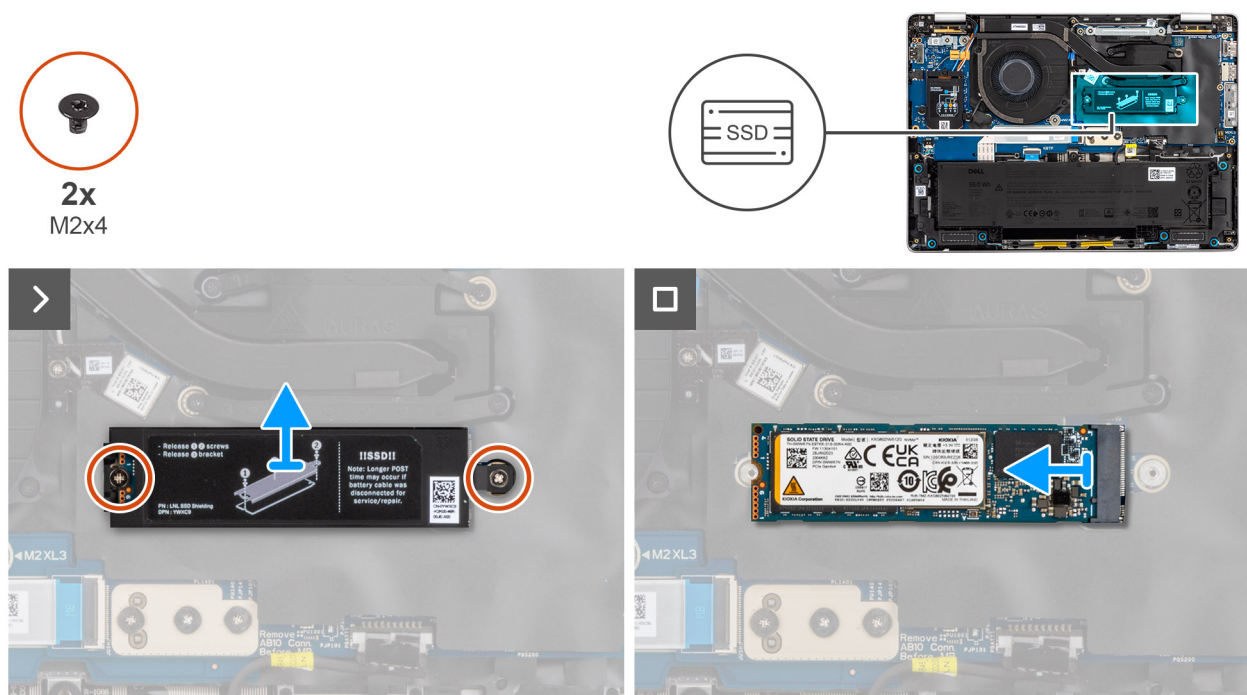
Figure 34. Removing the M.2 2280 SSD
