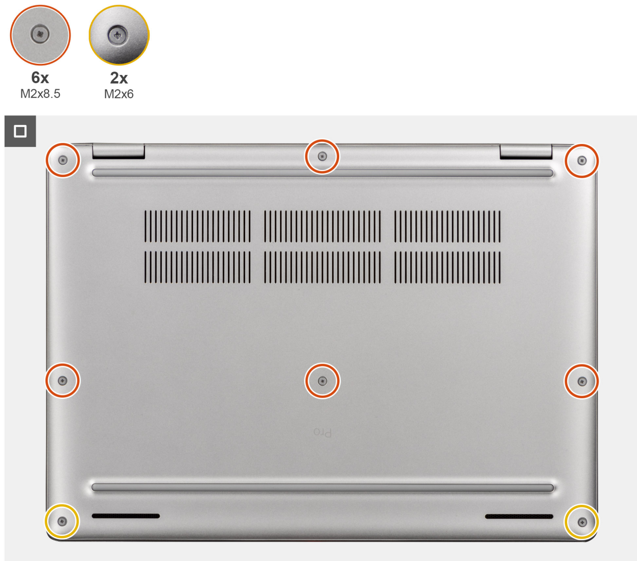
Figure 25. Installing the base cover
