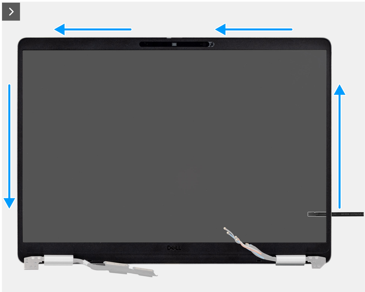
Figure 63. Removing the display bezel
