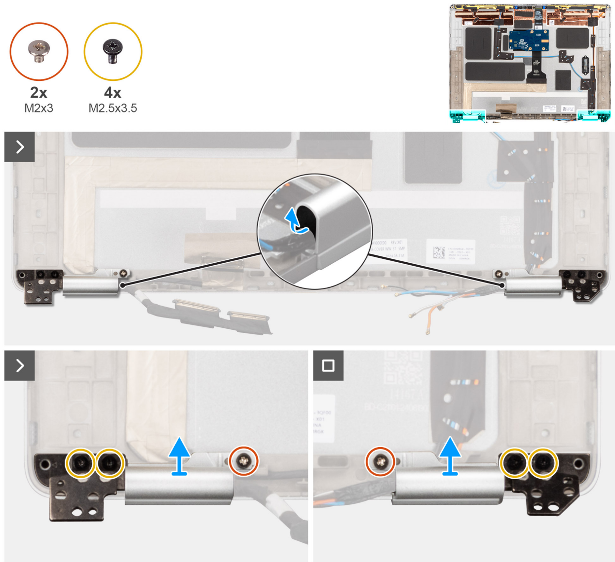
Figure 72. Removing the display hinge caps
