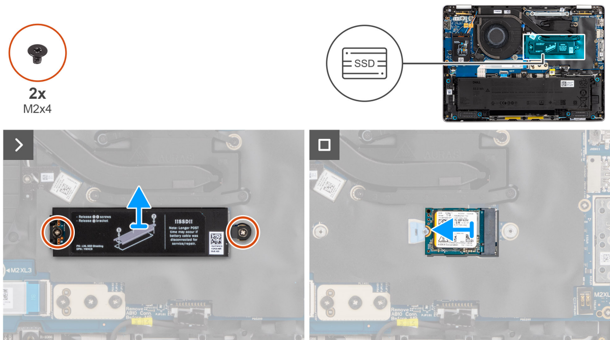
Figure 32. Removing the M.2 2230 SSD
