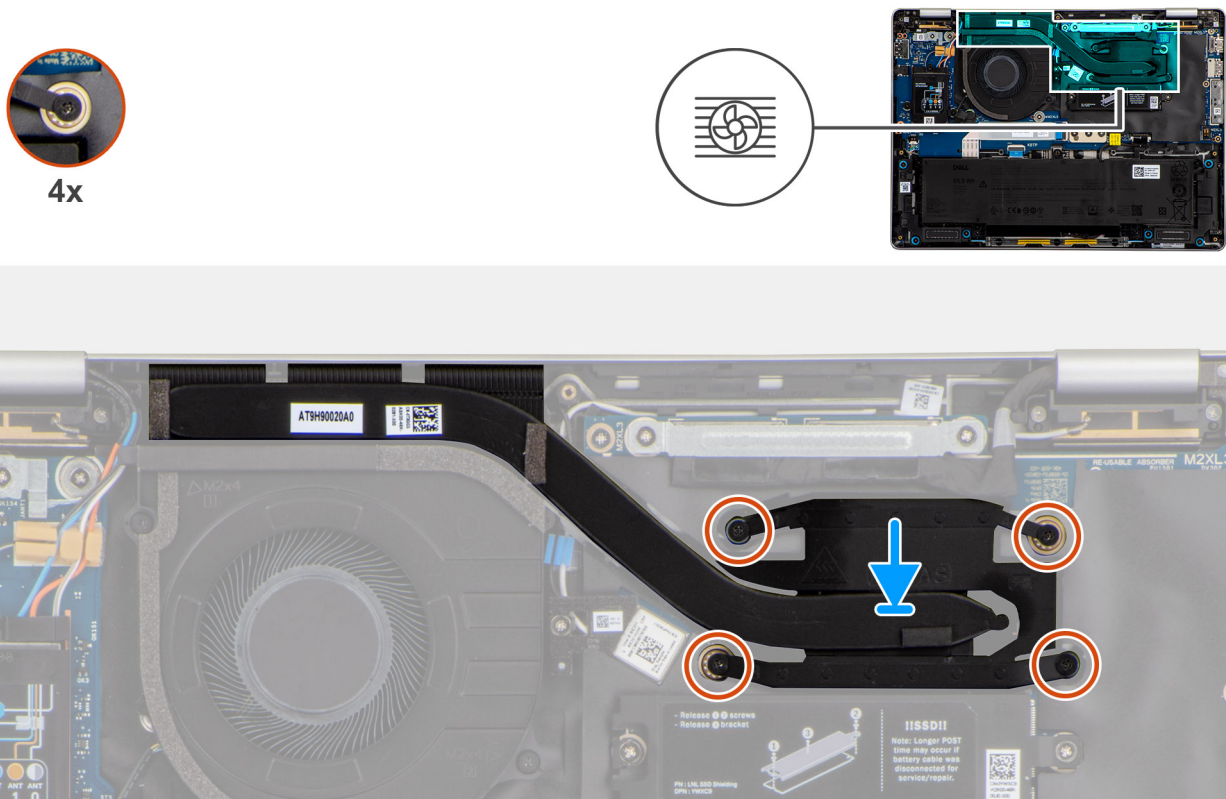
Figure 41. Installing the heat-sink
