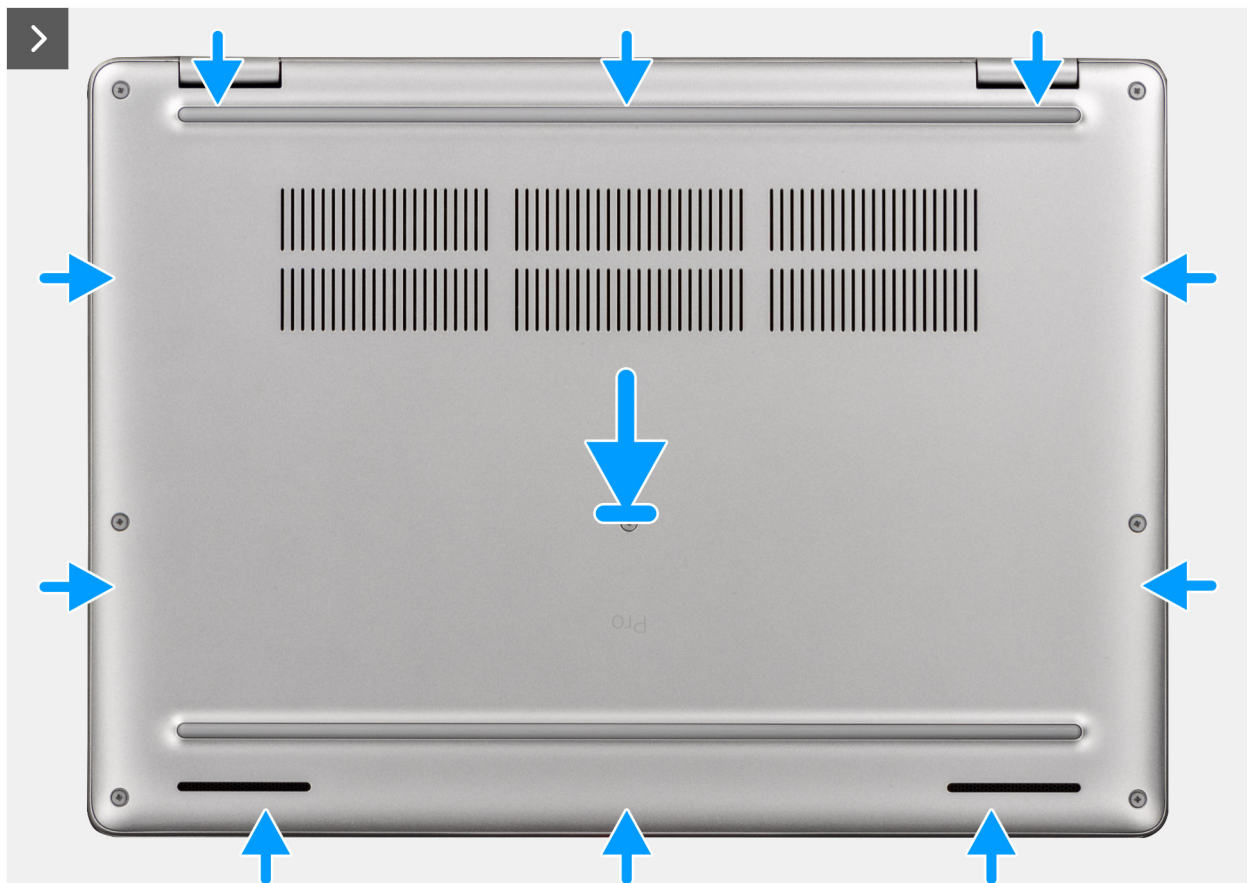
Figure 24. Installing the base cover
