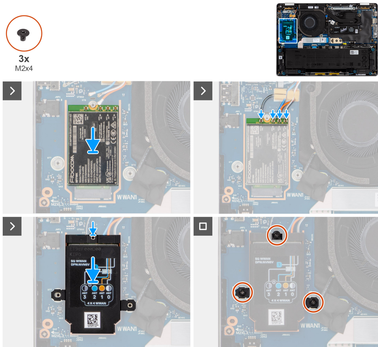
Figure 31. Installing the WWAN card
