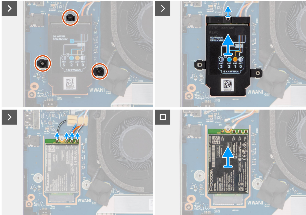
Figure 30. Removing the WWAN card
