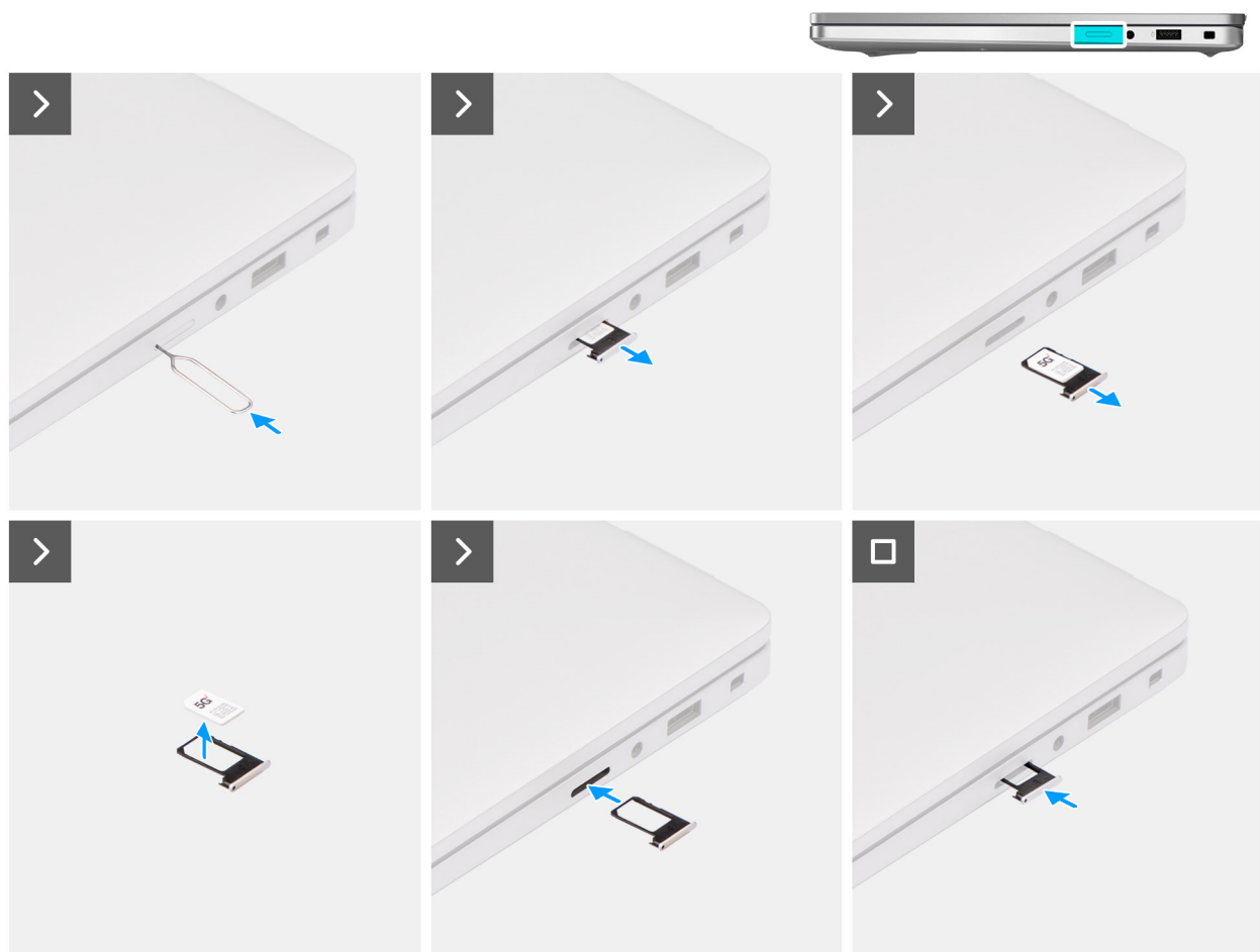
Figure 19. Removing the SIM-card tray
