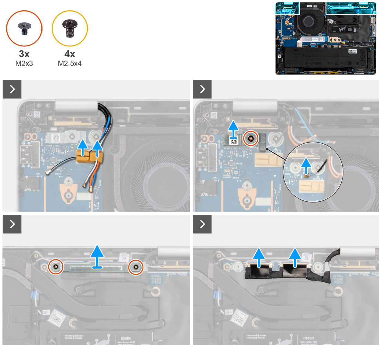
Figure 56. Removing the display assembly
