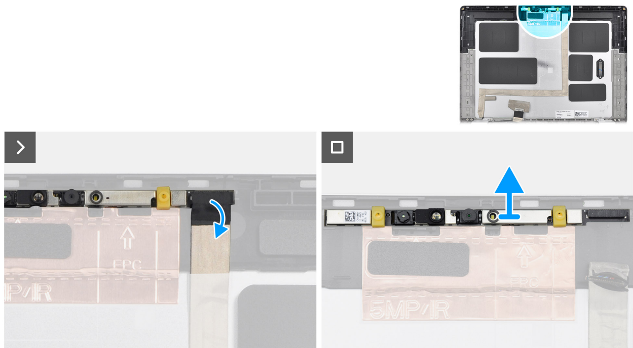
Figure 74. Removing the RGB/IR camera
