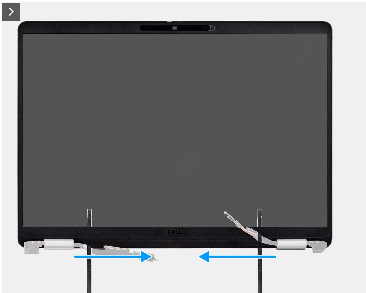
Figure 61. Removing the display bezel
