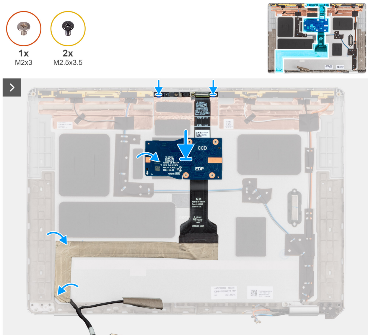
Figure 75. Installing the camera and display cable
