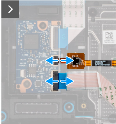
Figure 42. Removing the USH board
