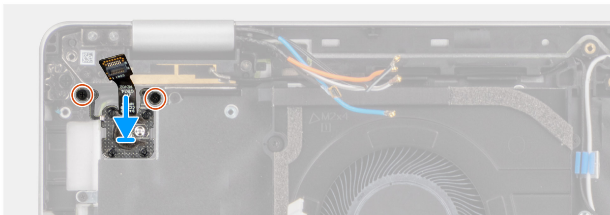
Figure 55. Installing the power button with optional fingerprint reader
