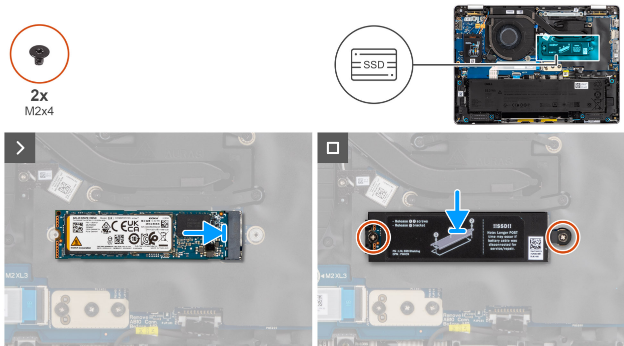
Figure 35. Installing the M.2 2280 SSD
