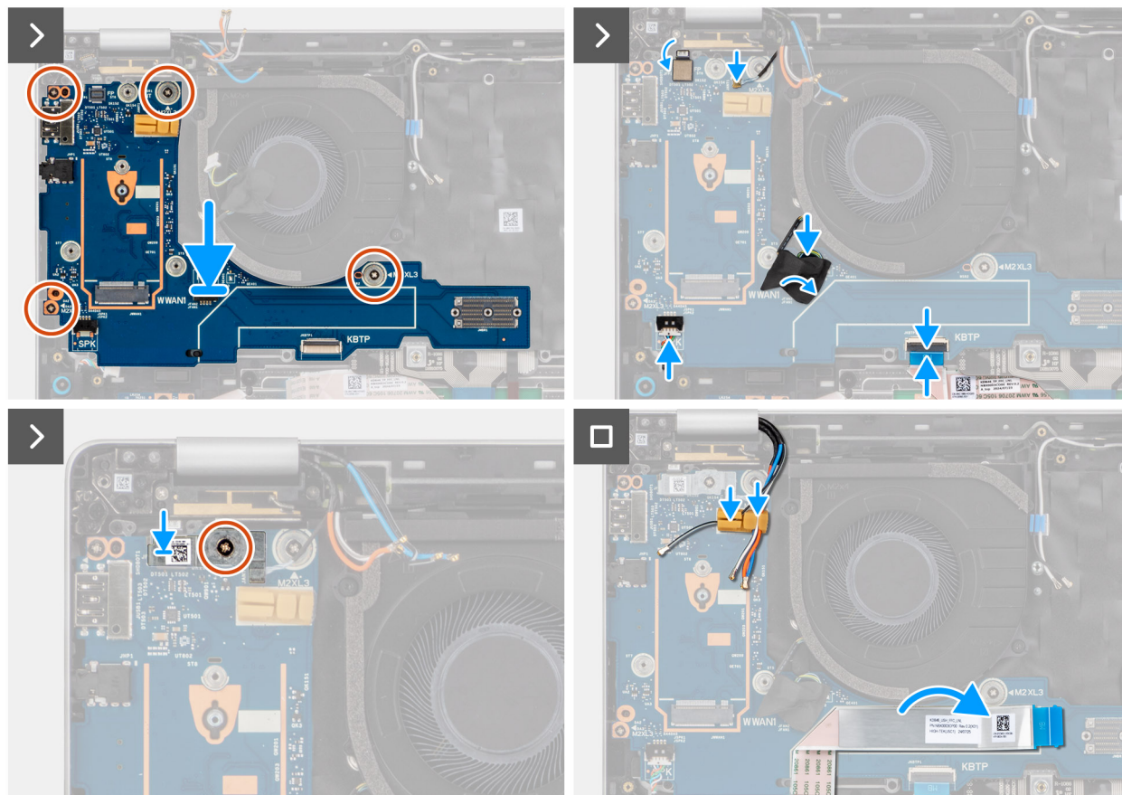
Figure 53. Installing the I/O board
