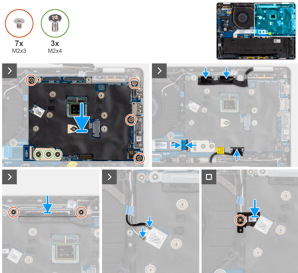
Figure 49. Installing the system board
