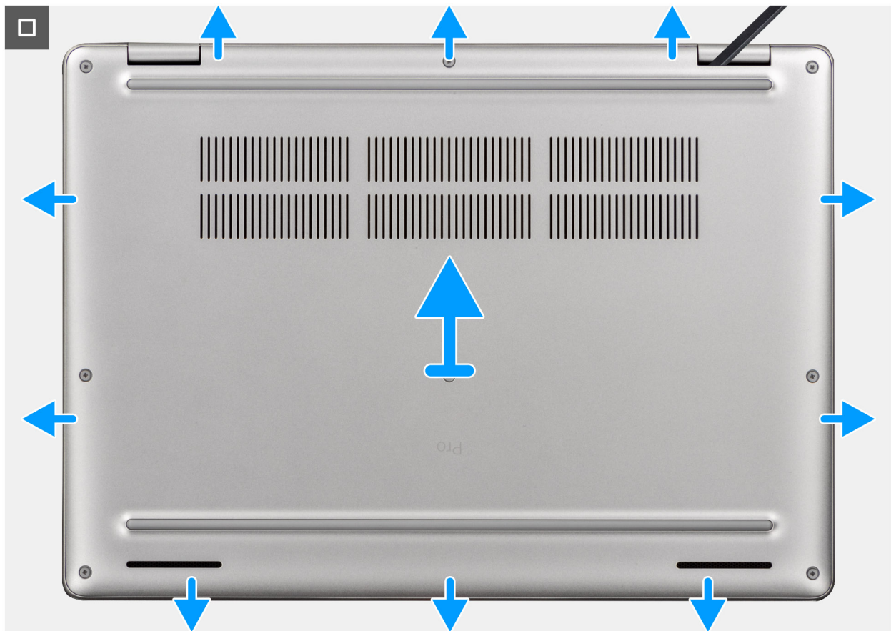
Figure 22. Removing the base cover
