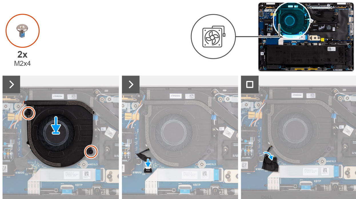
Figure 39. Installing the fan
