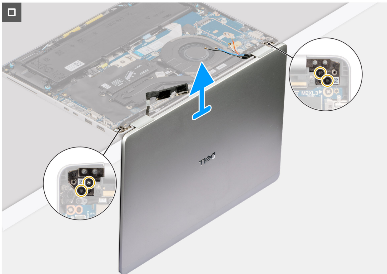
Figure 57. Removing the display assembly
