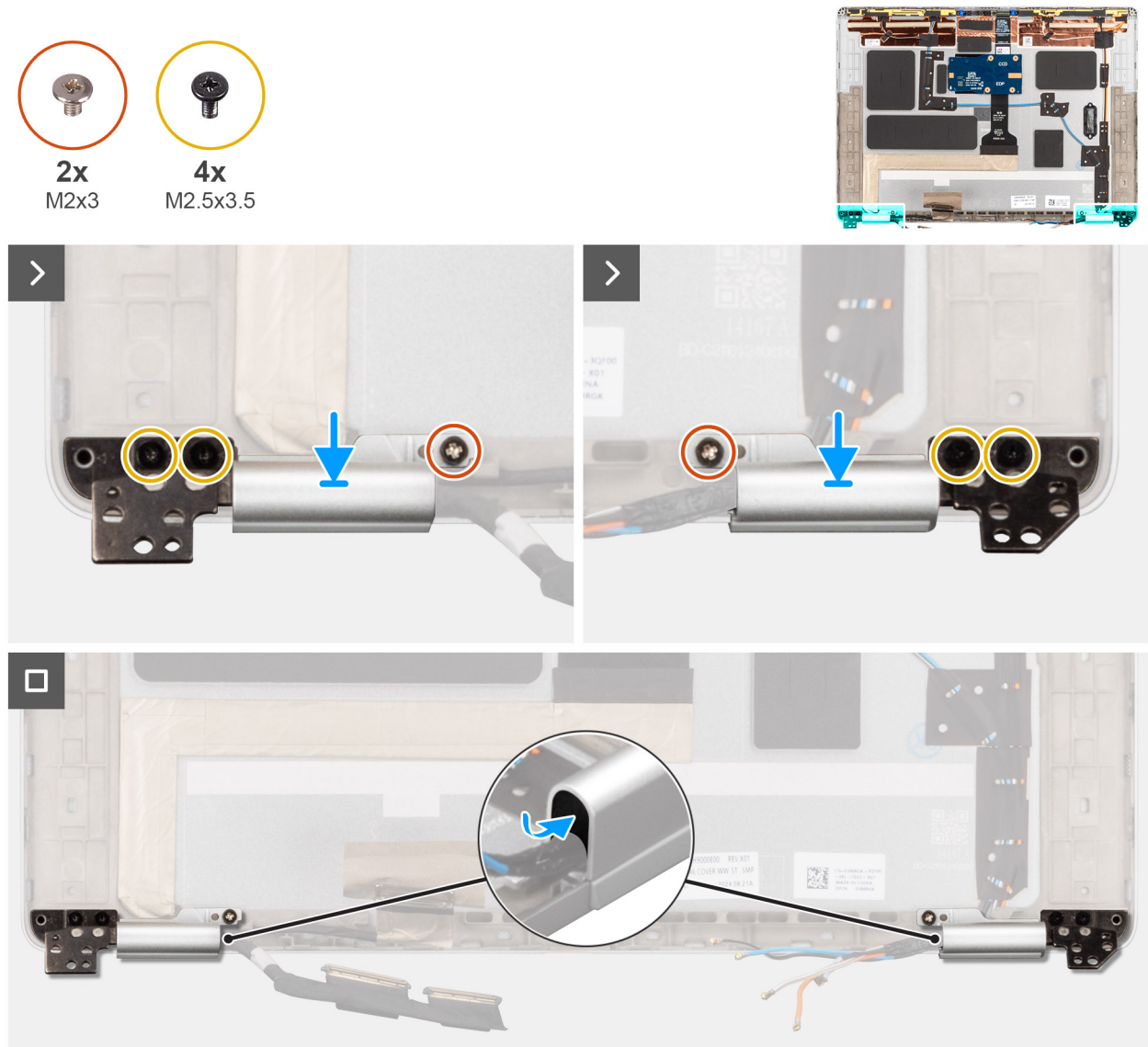
Figure 73. Installing the display hinge caps
