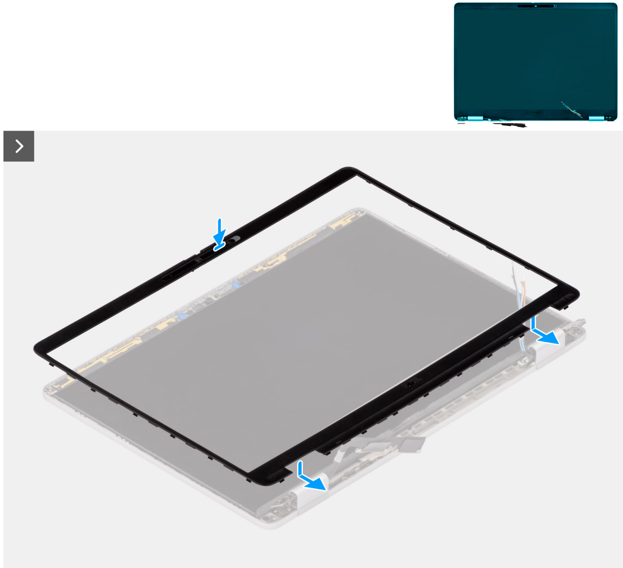
Figure 65. Installing the display bezel
