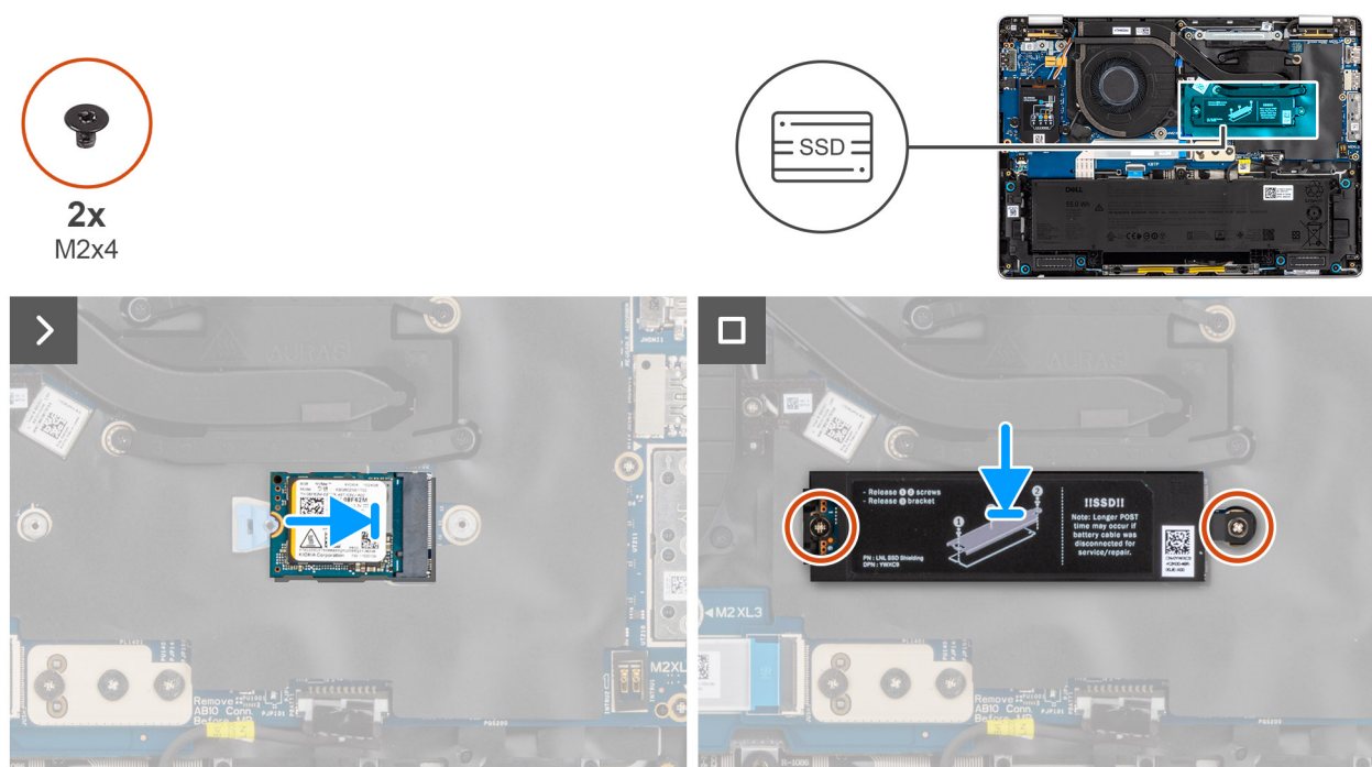
Figure 33. Installing the M.2 2230 SSD
