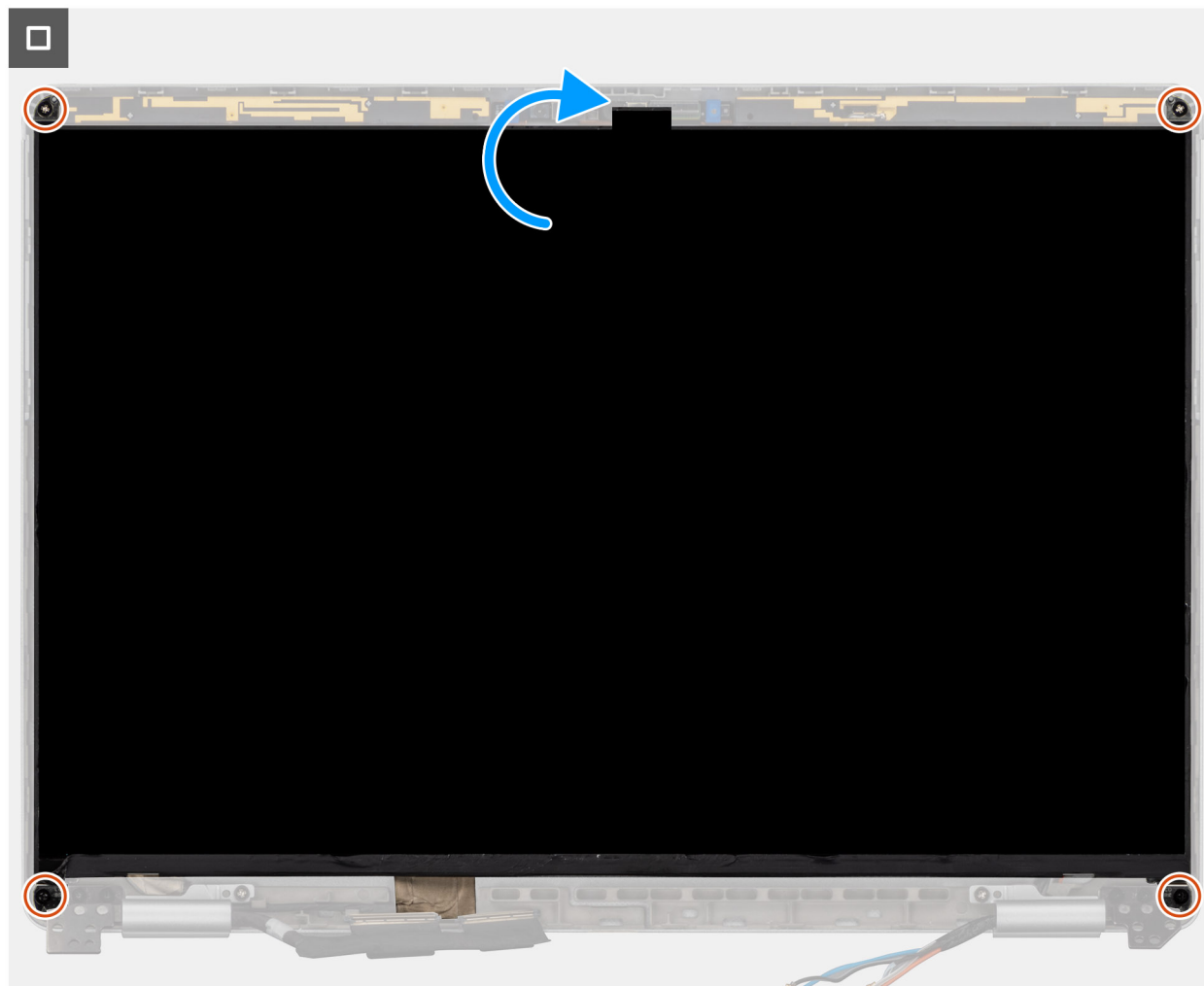
Figure 71. Installing the display panel
