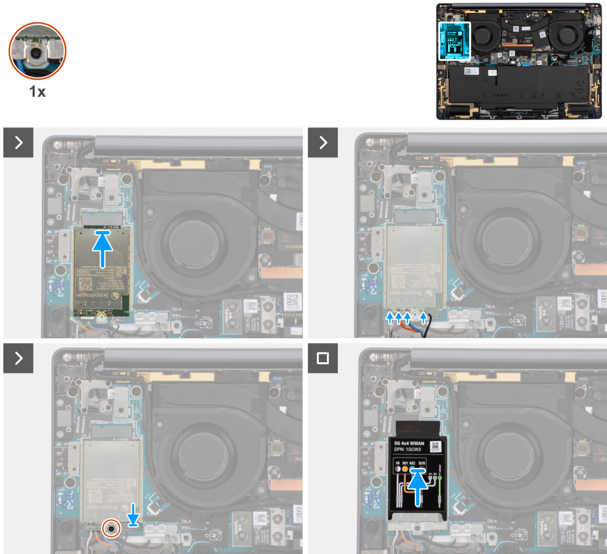
Figure 27. Installing the WWAN card
