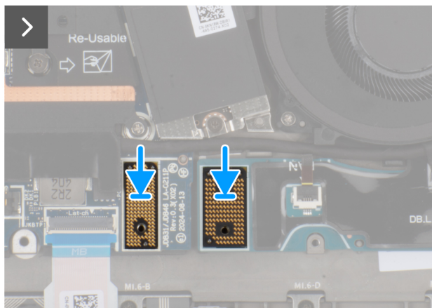
Figure 40. Installing the left I/O-board
