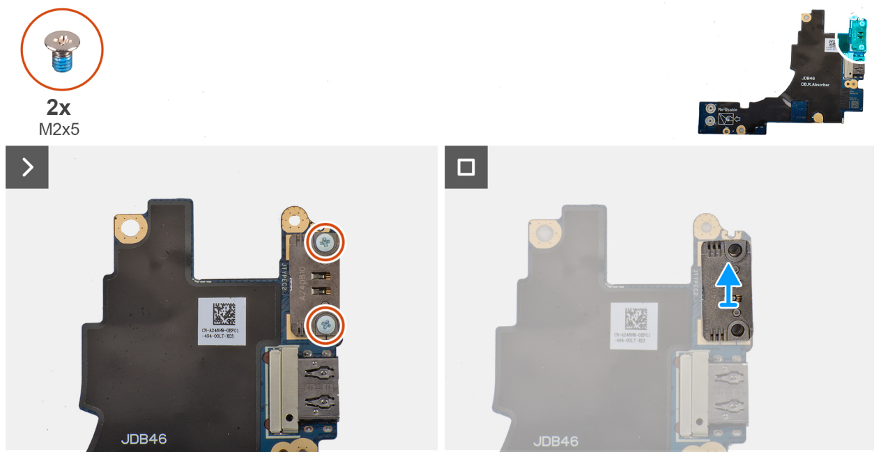
Figure 50. Removing the left USB Type-C module
