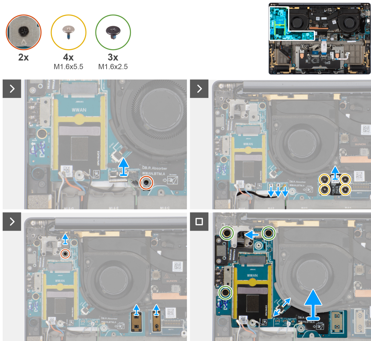
Figure 46. Removing the right I/O-board (with WWAN)
