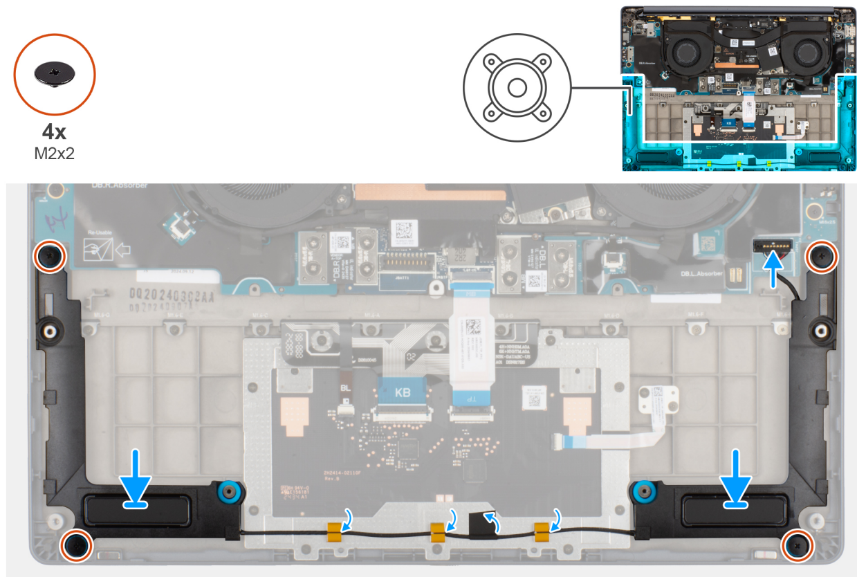
Figure 33. Installing the speakers (without WWAN)
