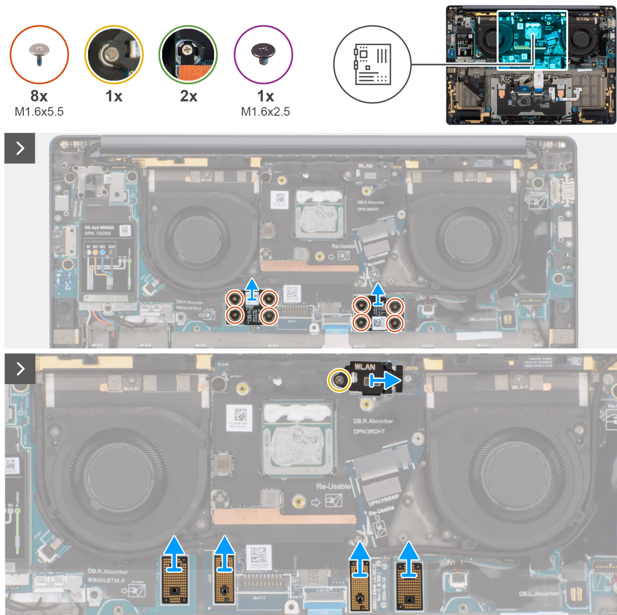
Figure 62. Removing the system board
