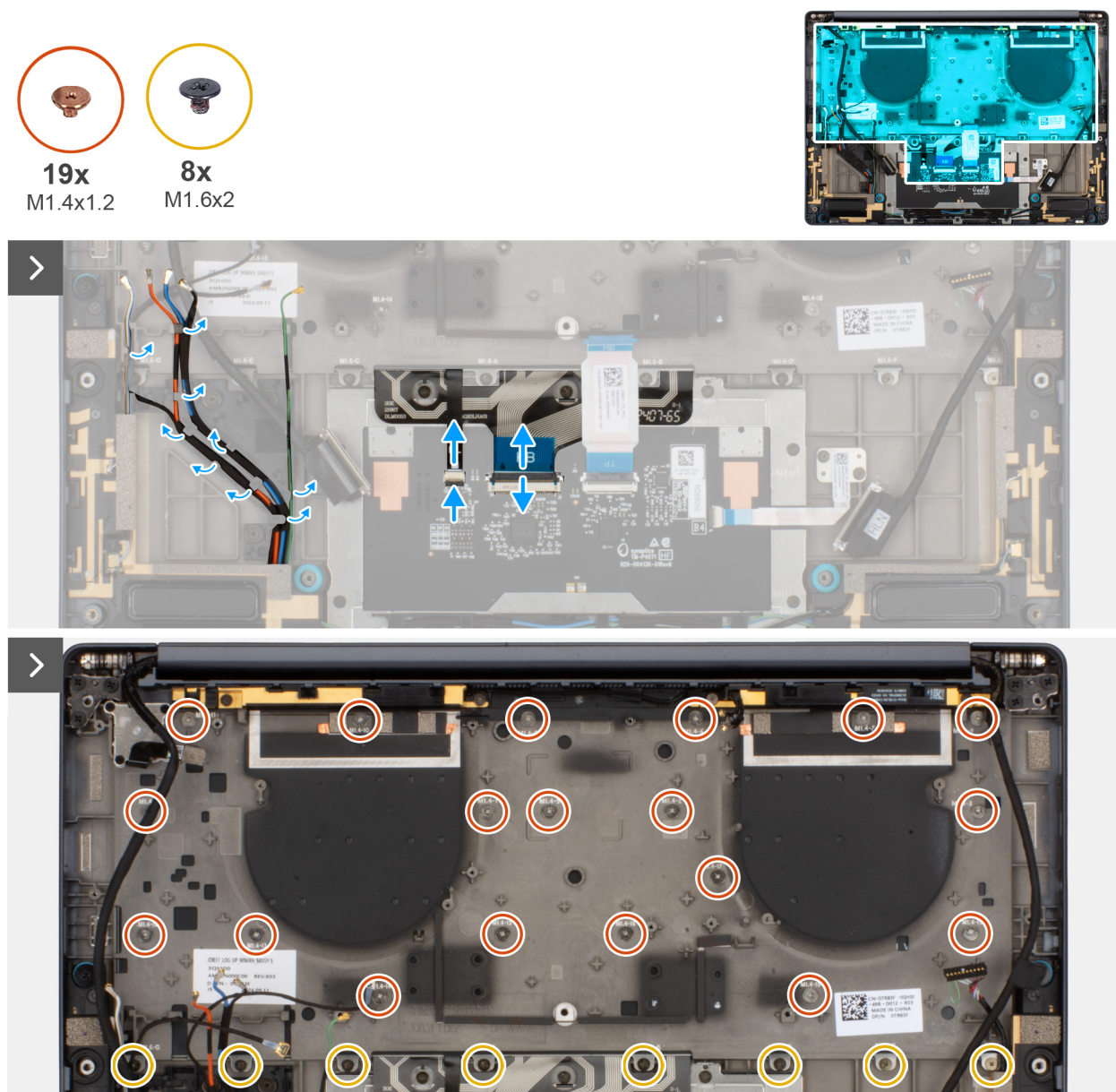
Figure 71. Removing the keyboard assembly
